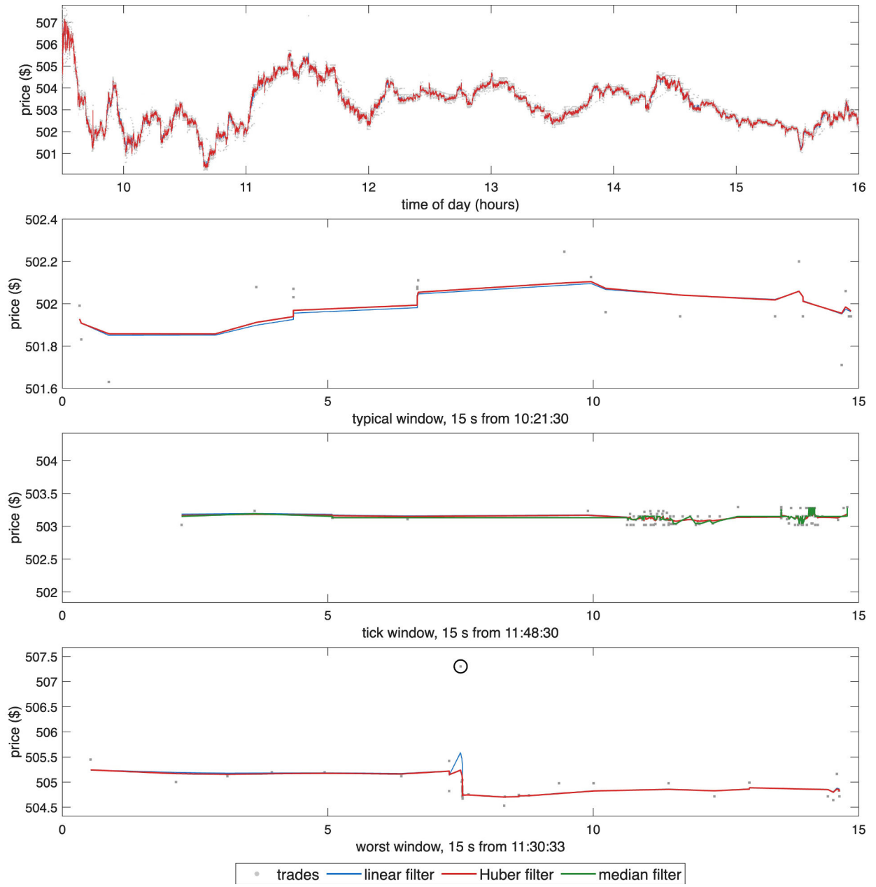
Figure 1: ADBE trades (grey points), the linear filter and the Huber filter, 16 October 2024. Top: full trading day. 2nd: 15-second window at the day's median trade count, from 10:21:30. 3rd: 15-second window at 11:48:30 in which the price reverses direction most often, with the median filter m_t added. Bottom: 15-second window around the largest Huber residual after 09:45, circled.
