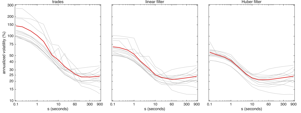
Figure 4: Volatility signature curves for ADBE over the 12 trading days in Oct 2024. The annualized vol \hat{\sigma}100\sqrt{252} from the returns \hat{X}_t - \hat{X}_{t,s} of Table 2, against the lag s in seconds, both axes on log scales, for: raw trades, linear filter & Huber filter. Grey lines are the individual trading days & the red line is the square root of the 12 day average of their squares. The linear & Huber returns carry the finite-sample correction c_{t,s} of the paper; the raw trades are unaffected by it.
