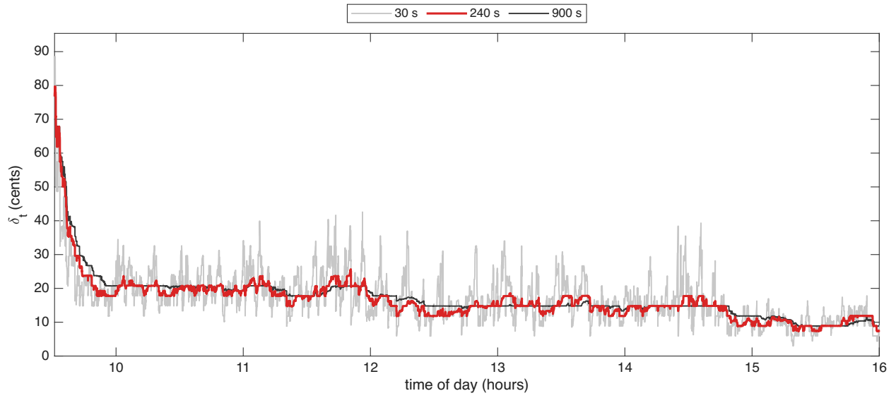
Figure 2: The Huber threshold \delta_t in cents for ADBE on 16 October 2024, with half-lives of 30, 240, 900 seconds. The 240-second half-life, in red, is used.
