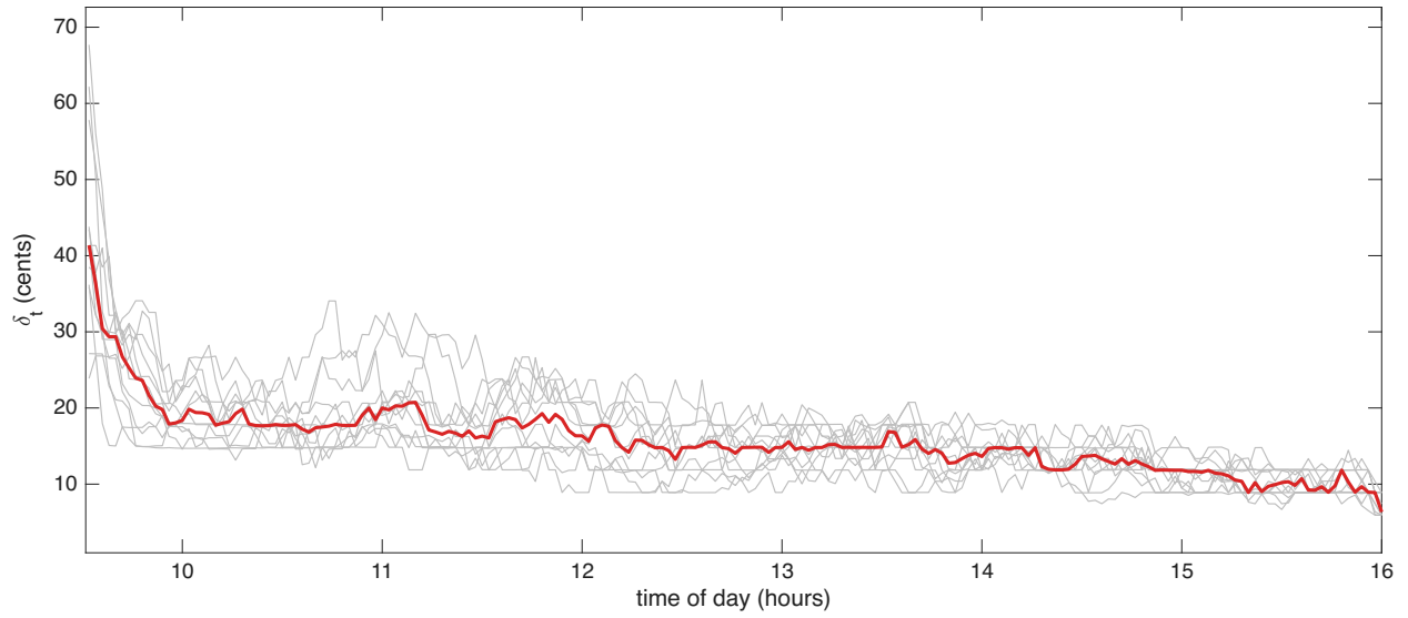
Figure 3: Huber threshold \delta_t in cents through the trading day, for 12 ADBE trading days in Oct 2024 (grey lines) and their median (red line).
