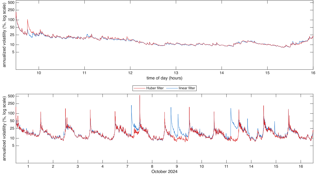
Figure 5: Filtered spot volatility for ADBE over 12 trading days in Oct 2024, the diurnally adjusted estimator \hat{\sigma}(u)100\sqrt{252} at s = 1 second with hyperbolic weights, Mandelbrot parameter a = 61 , with the input prices computed using the Huber & linear filters, shown as annualized volatility in percent on a log10 scale. Top: 16 October 2024, bottom: 12 days.
