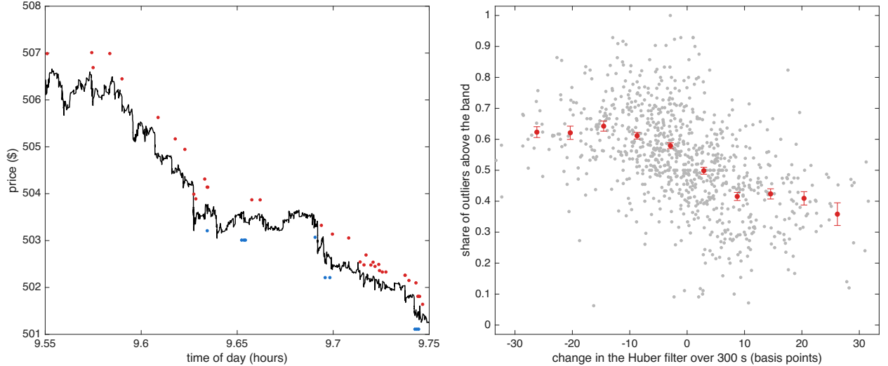
Figure 7: Outliers & robust price for ADBE on 16 October 2024. Left: the 12 minutes with the largest move in the Huber filter that day; outliers above Y_t - \theta_t > \delta_{t-1} in red, outliers below Y_t - \theta_t < -\delta_{t-1} in blue, Huber filter in black. Right: over the 12 trading days, the 300 second empirical conditional probability that outliers are above (rather than below) the Huber band against the 300 second change in the Huber filter in basis points: light points are single bins, the line & bars are means & s.e.
