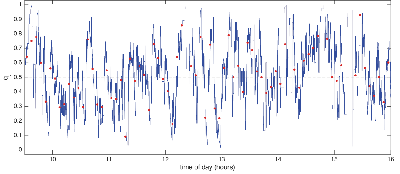
Figure 8: The directional conditional probability for ADBE, 16 October 2024. The filtered conditional probability q_t that an outlier lies above the robust Huber band, under exponential weights decaying in clock time with half life of 43 seconds; where fewer than two outliers remain in the weights it is drawn in grey. The dashed line marks 0.5. The red points are the empirical conditional probability using the 300 second bins of the previous figure.
