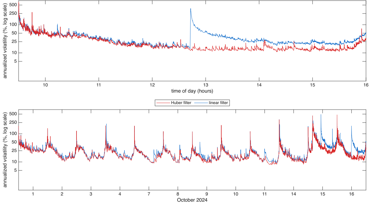
Figure 5: Filtered spot volatility for AMAT over 12 trading days in Oct 2024, the diurnally adjusted estimator \hat{\sigma}(u)100\sqrt{252} at s = 1 second with hyperbolic weights, Mandelbrot parameter a = 30 , with the input prices computed using the Huber & linear filters, shown as annualized volatility in percent on a log10 scale. Top: 16 October 2024, bottom: 12 days.
