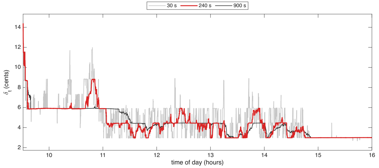
Figure 2: The Huber threshold \delta_t in cents for AMAT on 16 October 2024, with half-lives of 30, 240, 900 seconds. The 240-second half-life, in red, is used.
