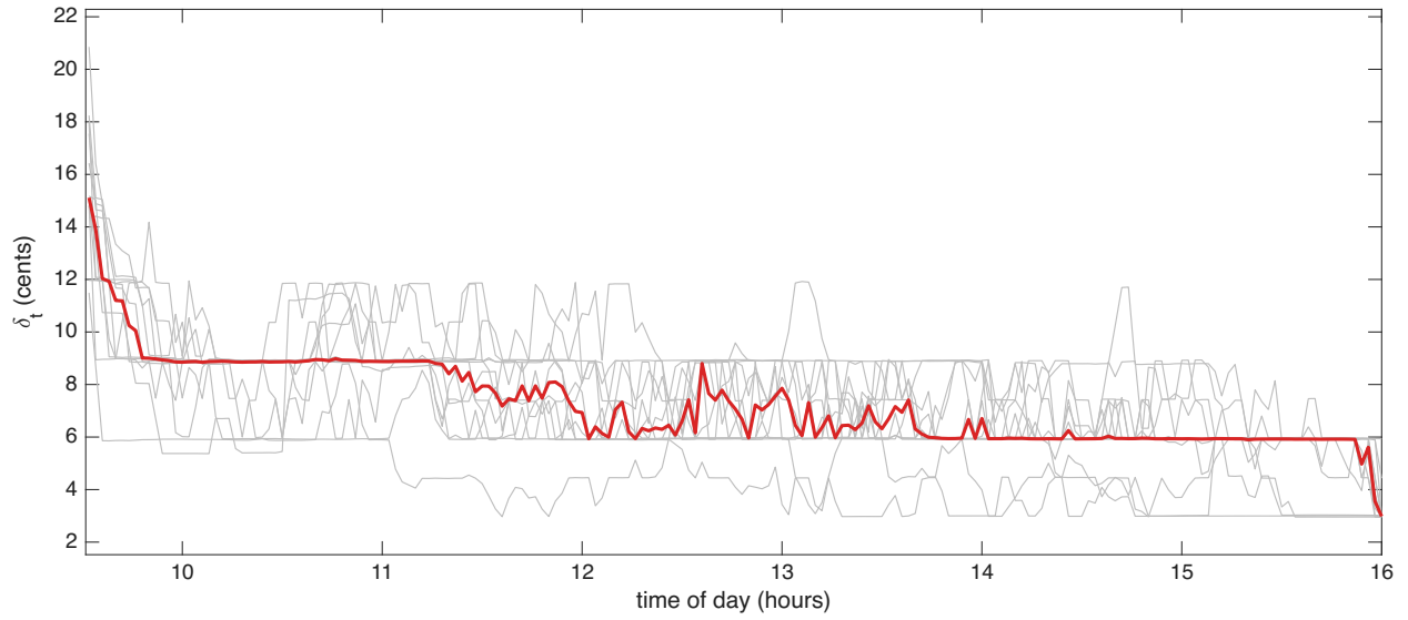
Figure 3: Huber threshold \delta_t in cents through the trading day, for 12 AMAT trading days in Oct 2024 (grey lines) and their median (red line).
