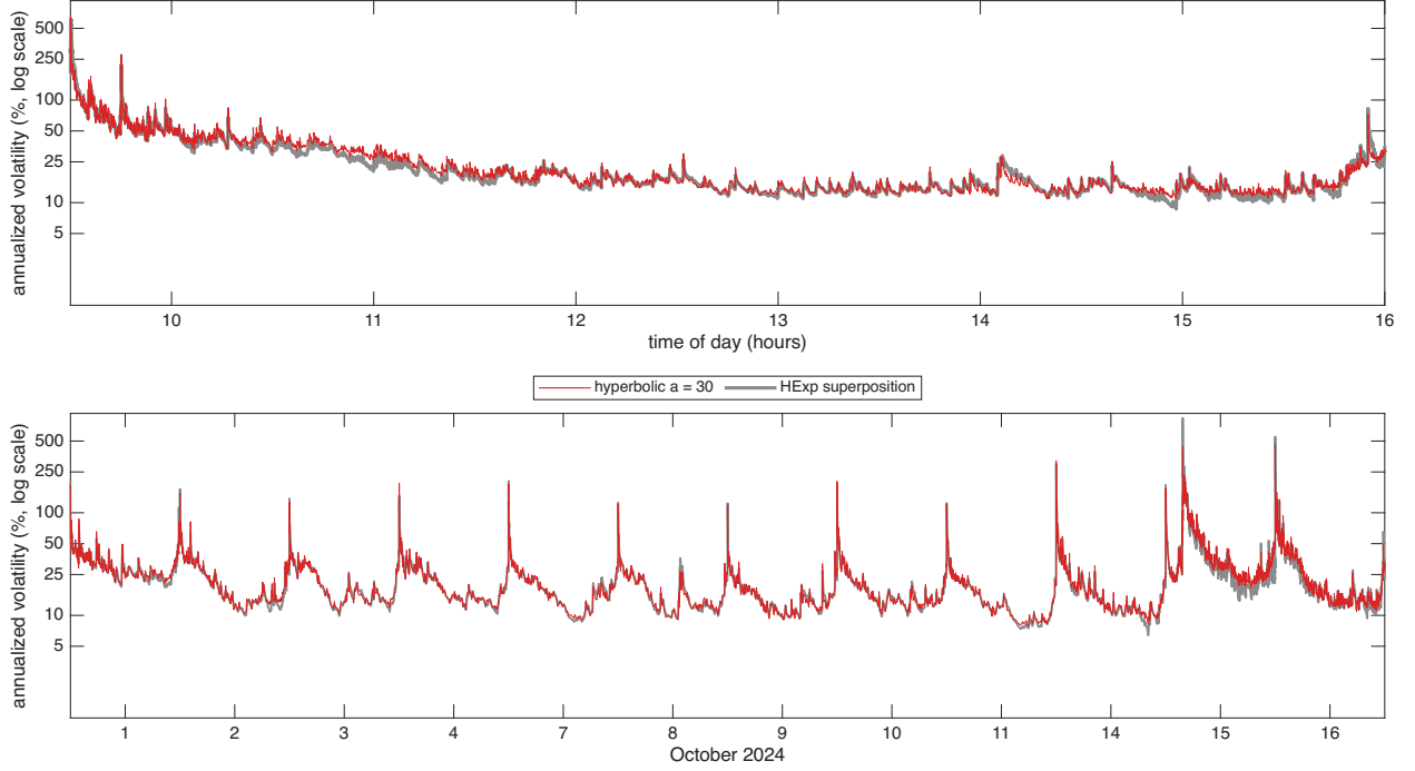
Figure 6: Hyperbolic against superposition weights for AMAT over 12 trading days in Oct 2024, the diurnally adjusted \hat{\sigma}(u)100\sqrt{252} at s = 1 second from the Huber filter, shown as annualized vol in % on a log10 scale. The only difference between the 2 paths is the weight function: the hyperbolic weights with a = 30 in red, drawn on top, and the HExp superposition in grey, 4 exponential components with half lives of 2, 20, 200, 2000 seconds. Hyperparameters minimize the QLIKE objective. Top: 16 October 2024, bottom: 12 days.
