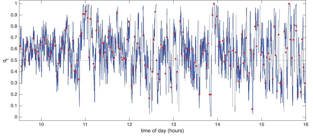
Figure 8: The directional conditional probability for AMAT, 16 October 2024. The filtered conditional probability q_t that an outlier lies above the robust Huber band, under exponential weights decaying in clock time with half life of 21 seconds; where fewer than two outliers remain in the weights it is drawn in grey. The dashed line marks 0.5. The red points are the empirical conditional probability using the 120 second bins of the previous figure.
