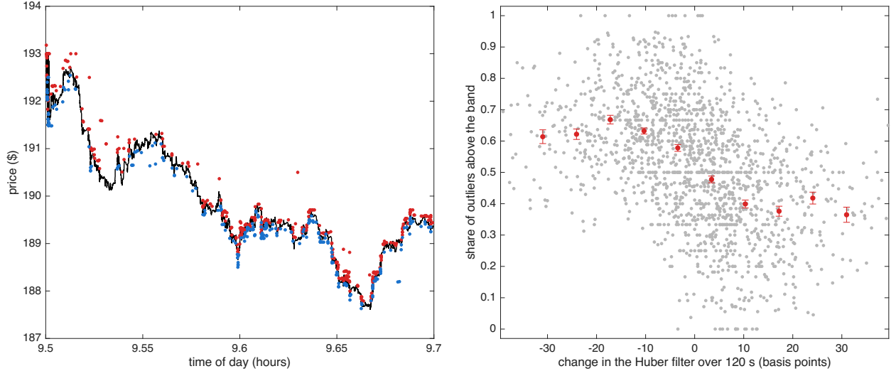
Figure 7: Outliers & robust price for AMAT on 16 October 2024. Left: the 12 minutes with the largest move in the Huber filter that day; outliers above Y_t - \theta_t > \delta_{t-1} in red, outliers below Y_t - \theta_t < -\delta_{t-1} in blue, Huber filter in black. Right: over the 12 trading days, the 120 second empirical conditional probability that outliers are above (rather than below) the Huber band against the 120 second change in the Huber filter in basis points: light points are single bins, the line & bars are means & s.e.
