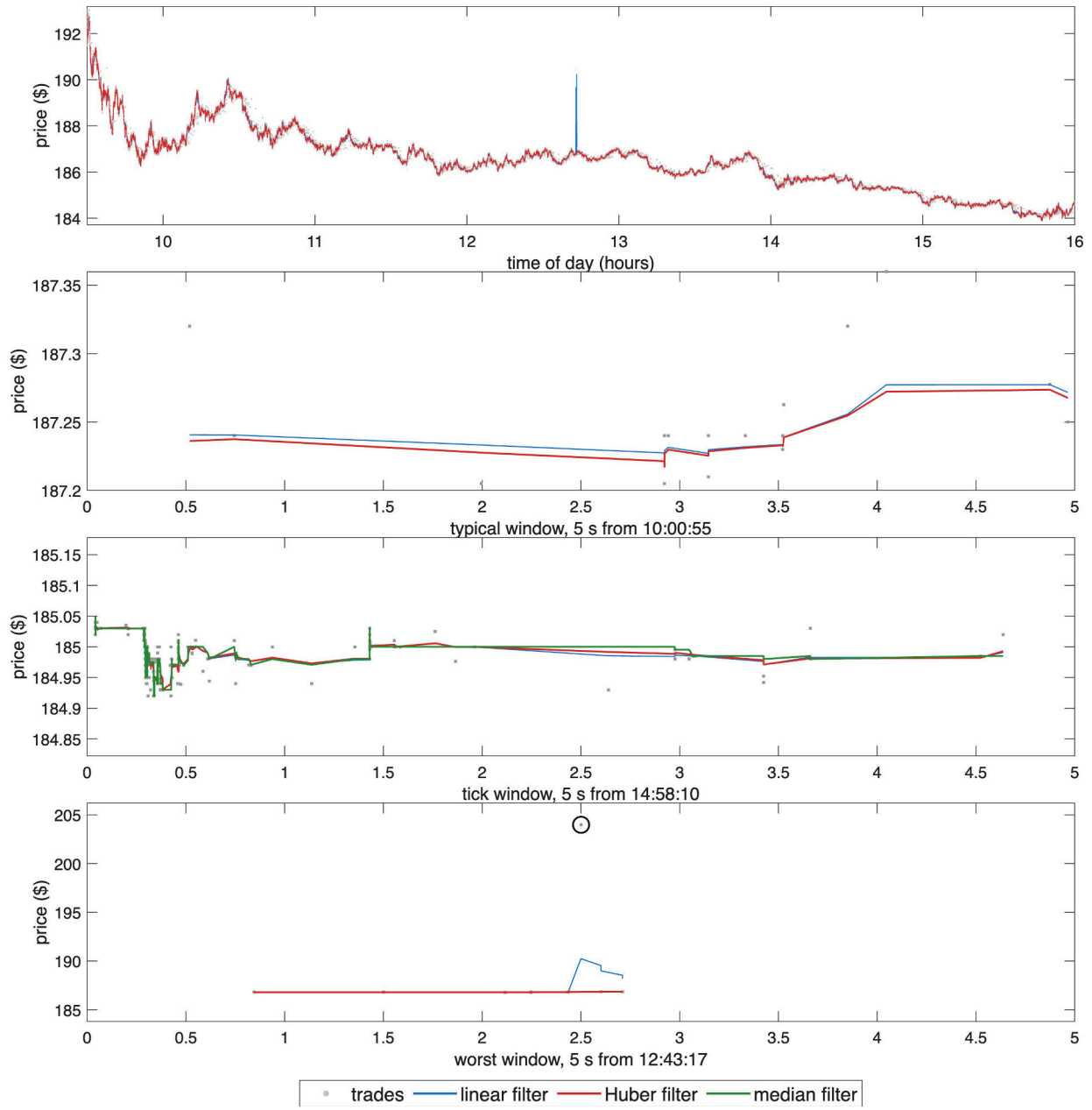
Figure 1: AMAT trades (grey points), the linear filter and the Huber filter, 16 October 2024. Top: full trading day. 2nd: 5-second window at the day's median trade count, from 10:00:55. 3rd: 5-second window at 14:58:10 in which the price reverses direction most often, with the median filter m_t added. Bottom: 5-second window around the largest Huber residual after 09:45, circled.
