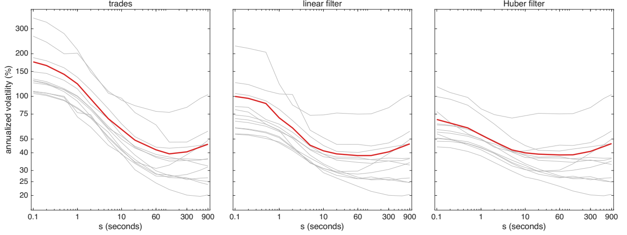
Figure 4: Volatility signature curves for AMAT over the 12 trading days in Oct 2024. The annualized vol \hat{\sigma}100\sqrt{252} from the returns \hat{X}_t - \hat{X}_{t,s} of Table 2, against the lag s in seconds, both axes on log scales, for: raw trades, linear filter & Huber filter. Grey lines are the individual trading days & the red line is the square root of the 12 day average of their squares. The linear & Huber returns carry the finite-sample correction c_{t,s} of the paper; the raw trades are unaffected by it.
