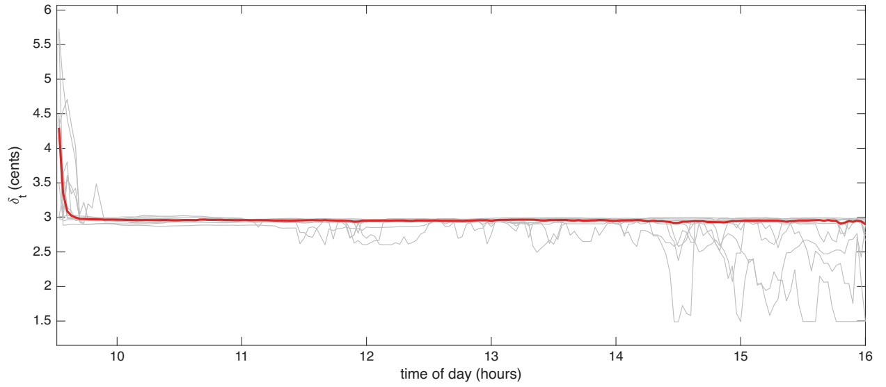
Figure 3: Huber threshold \delta_t in cents through the trading day, for 12 AMD trading days in Oct 2024 (grey lines) and their median (red line).
