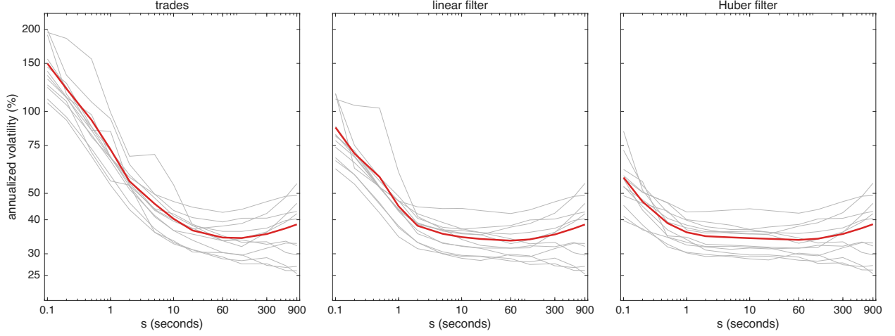
Figure 4: Volatility signature curves for AMD over the 12 trading days in Oct 2024. The annualized vol \hat{\sigma}100\sqrt{252} from the returns \hat{X}_t - \hat{X}_{t,s} of Table 2, against the lag s in seconds, both axes on log scales, for: raw trades, linear filter & Huber filter. Grey lines are the individual trading days & the red line is the square root of the 12 day average of their squares. The linear & Huber returns carry the finite-sample correction c_{t,s} of the paper; the raw trades are unaffected by it.
