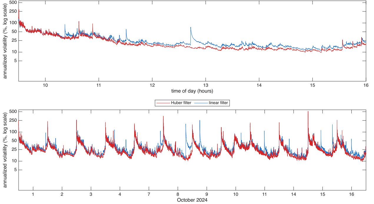
Figure 5: Filtered spot volatility for AMD over 12 trading days in Oct 2024, the diurnally adjusted estimator \hat{\sigma}(u)100\sqrt{252} at s = 1 second with hyperbolic weights, Mandelbrot parameter a = 106 , with the input prices computed using the Huber & linear filters, shown as annualized volatility in percent on a log10 scale. Top: 16 October 2024, bottom: 12 days.
