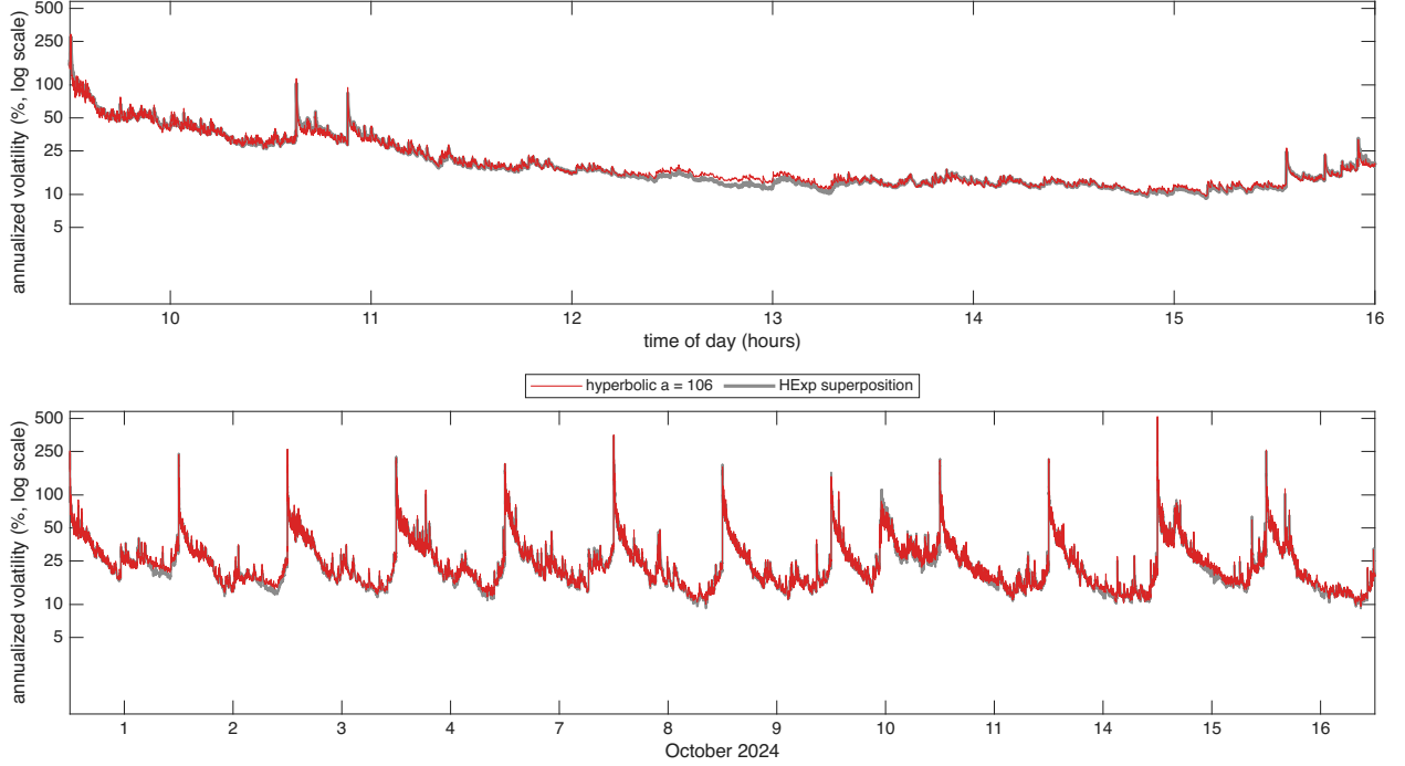
Figure 6: Hyperbolic against superposition weights for AMD over 12 trading days in Oct 2024, the diurnally adjusted \hat{\sigma}(u)100\sqrt{252} at s = 1 second from the Huber filter, shown as annualized vol in % on a log10 scale. The only difference between the 2 paths is the weight function: the hyperbolic weights with a = 106 in red, drawn on top, and the HExp superposition in grey, 4 exponential components with half lives of 2, 20, 200, 2000 seconds. Hyperparameters minimize the QLIKE objective. Top: 16 October 2024, bottom: 12 days.
