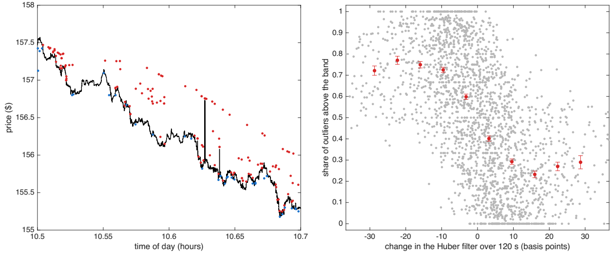
Figure 7: Outliers & robust price for AMD on 16 October 2024. Left: the 12 minutes with the largest move in the Huber filter that day; outliers above Y_t - \theta_t > \delta_{t-1} in red, outliers below Y_t - \theta_t < -\delta_{t-1} in blue, Huber filter in black. Right: over the 12 trading days, the 120 second empirical conditional probability that outliers are above (rather than below) the Huber band against the 120 second change in the Huber filter in basis points: light points are single bins, the line & bars are means & s.e.
