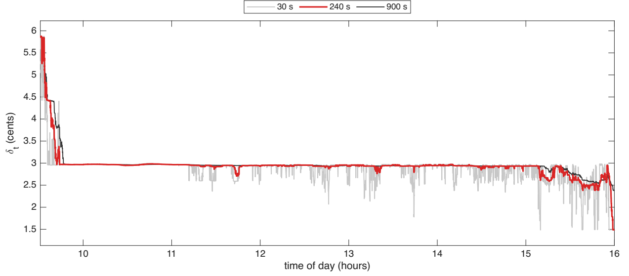
Figure 2: The Huber threshold \delta_t in cents for AMD on 16 October 2024, with half-lives of 30, 240, 900 seconds. The 240-second half-life, in red, is used.
