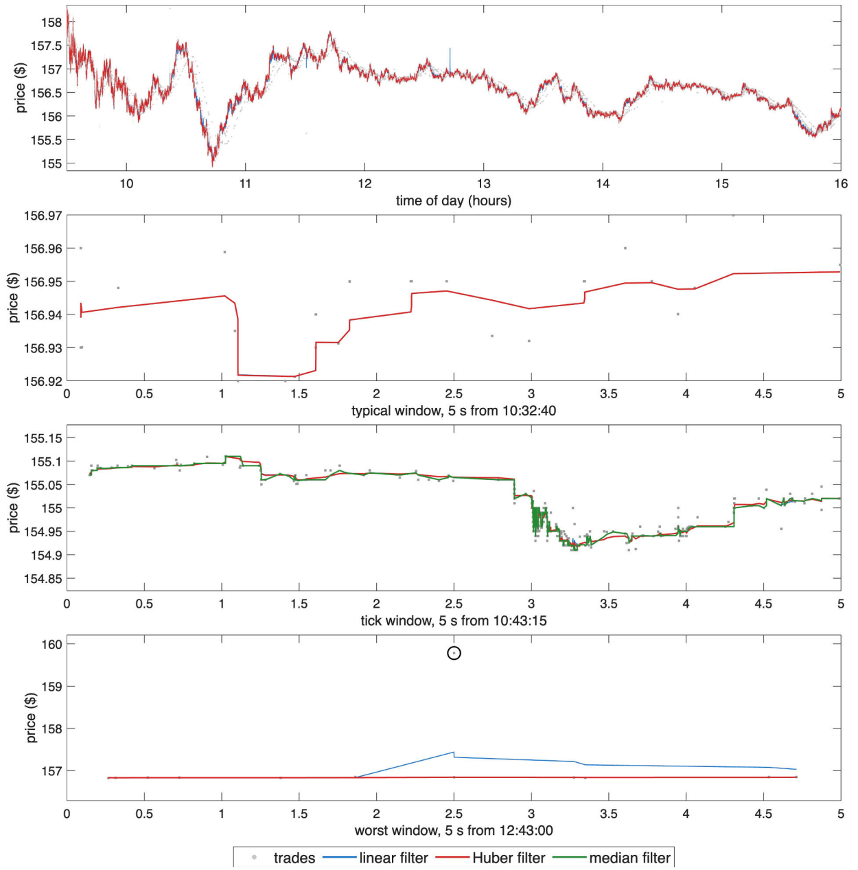
Figure 1: AMD trades (grey points), the linear filter and the Huber filter, 16 October 2024. Top: full trading day. 2nd: 5-second window at the day's median trade count, from 10:32:40. 3rd: 5-second window at 10:43:15 in which the price reverses direction most often, with the median filter m_t added. Bottom: 5-second window around the largest Huber residual after 09:45, circled.
