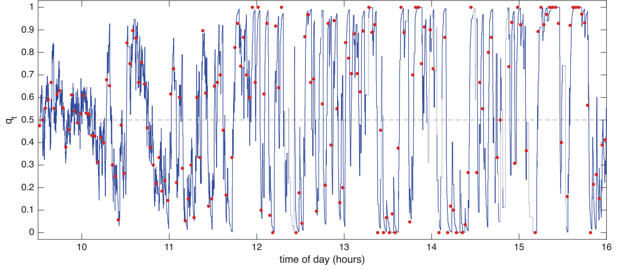
Figure 8: The directional conditional probability for AMD, 16 October 2024. The filtered conditional probability q_t that an outlier lies above the robust Huber band, under exponential weights decaying in clock time with half life of 29 seconds; where fewer than two outliers remain in the weights it is drawn in grey. The dashed line marks 0.5. The red points are the empirical conditional probability using the 120 second bins of the previous figure.
