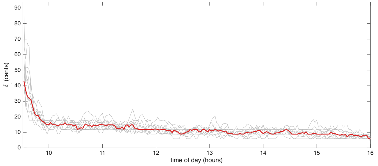
Figure 3: Huber threshold \delta_t in cents through the trading day, for 12 AMGN trading days in Oct 2024 (grey lines) and their median (red line).
