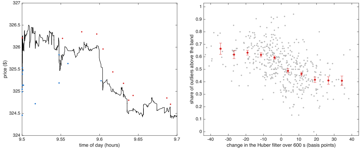
Figure 7: Outliers & robust price for AMGN on 16 October 2024. Left: the 12 minutes with the largest move in the Huber filter that day; outliers above Y_t - \theta_t > \delta_{t-1} in red, outliers below Y_t - \theta_t < -\delta_{t-1} in blue, Huber filter in black. Right: over the 12 trading days, the 600 second empirical conditional probability that outliers are above (rather than below) the Huber band against the 600 second change in the Huber filter in basis points: light points are single bins, the line & bars are means & s.e.
