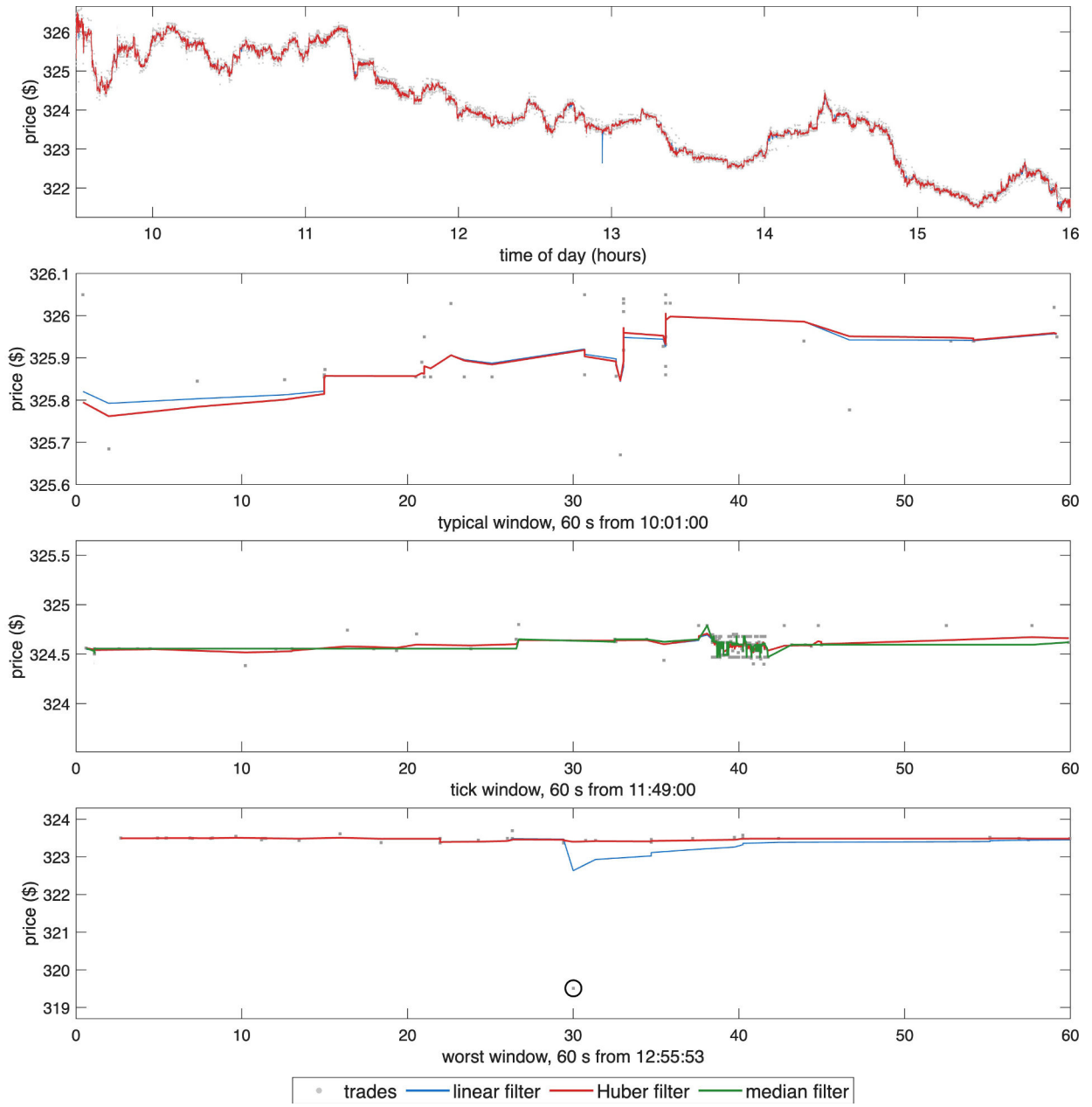
Figure 1: AMGN trades (grey points), the linear filter and the Huber filter, 16 October 2024. Top: full trading day. 2nd: 60-second window at the day's median trade count, from 10:01:00. 3rd: 60-second window at 11:49:00 in which the price reverses direction most often, with the median filter m_t added. Bottom: 60-second window around the largest Huber residual after 09:45, circled.
