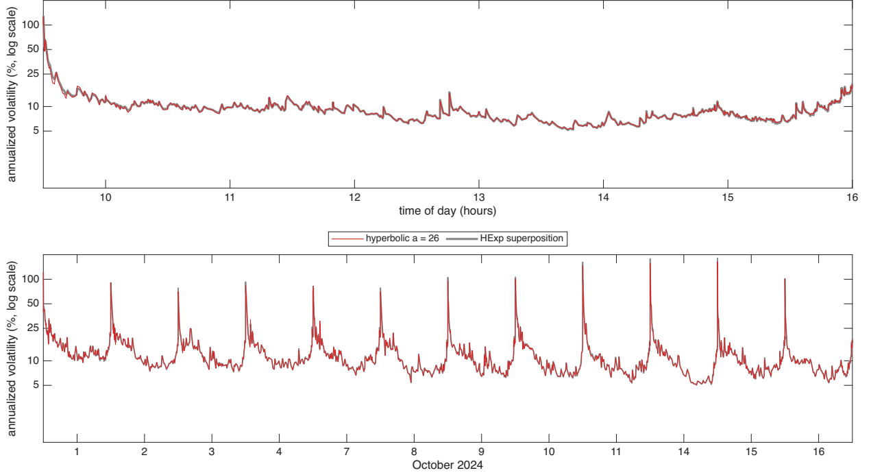
Figure 6: Hyperbolic against superposition weights for AMGN over 12 trading days in Oct 2024, the diurnally adjusted \hat{\sigma}(u)100\sqrt{252} at s = 1 second from the Huber filter, shown as annualized vol in % on a log10 scale. The only difference between the 2 paths is the weight function: the hyperbolic weights with a = 26 in red, drawn on top, and the HExp superposition in grey, 4 exponential components with half lives of 10, 100, 1000, 10000 seconds. Hyperparameters minimize the QLIKE objective. Top: 16 October 2024, bottom: 12 days.
