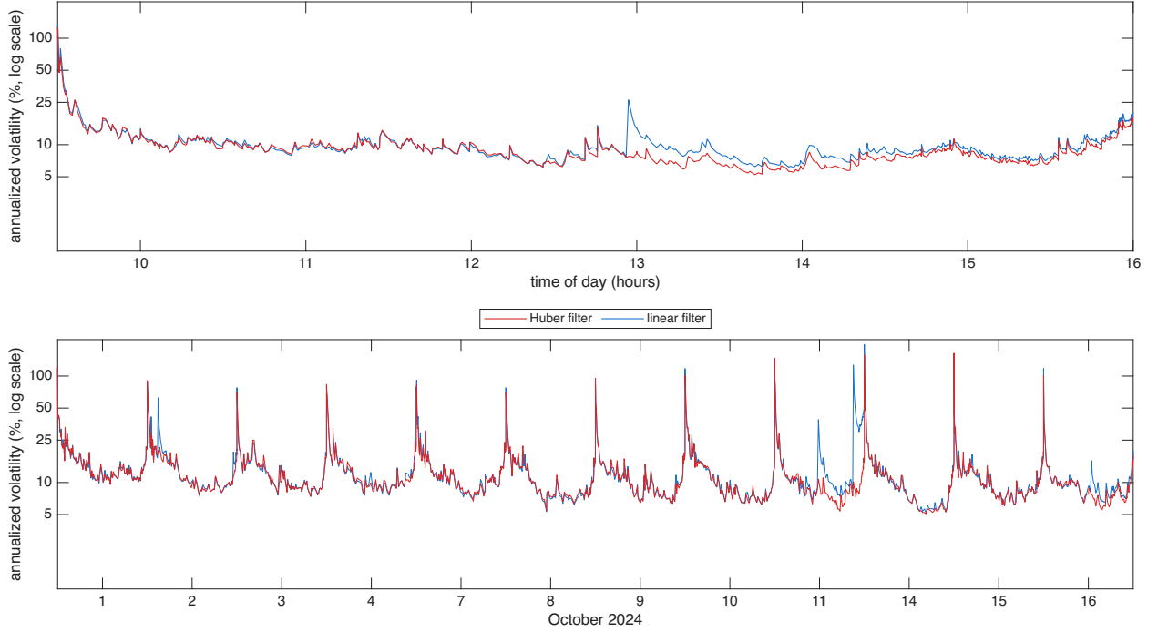
Figure 5: Filtered spot volatility for AMGN over 12 trading days in Oct 2024, the diurnally adjusted estimator \hat{\sigma}(u)100\sqrt{252} at s = 1 second with hyperbolic weights, Mandelbrot parameter a = 26 , with the input prices computed using the Huber & linear filters, shown as annualized volatility in percent on a log10 scale. Top: 16 October 2024, bottom: 12 days.
