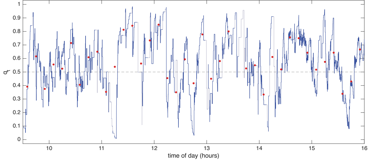
Figure 8: The directional conditional probability for AMGN , 16 October 2024. The filtered conditional probability q_t that an outlier lies above the robust Huber band, under exponential weights decaying in clock time with half life of 88 seconds; where fewer than two outliers remain in the weights it is drawn in grey. The dashed line marks 0.5. The red points are the empirical conditional probability using the 600 second bins of the previous figure.
