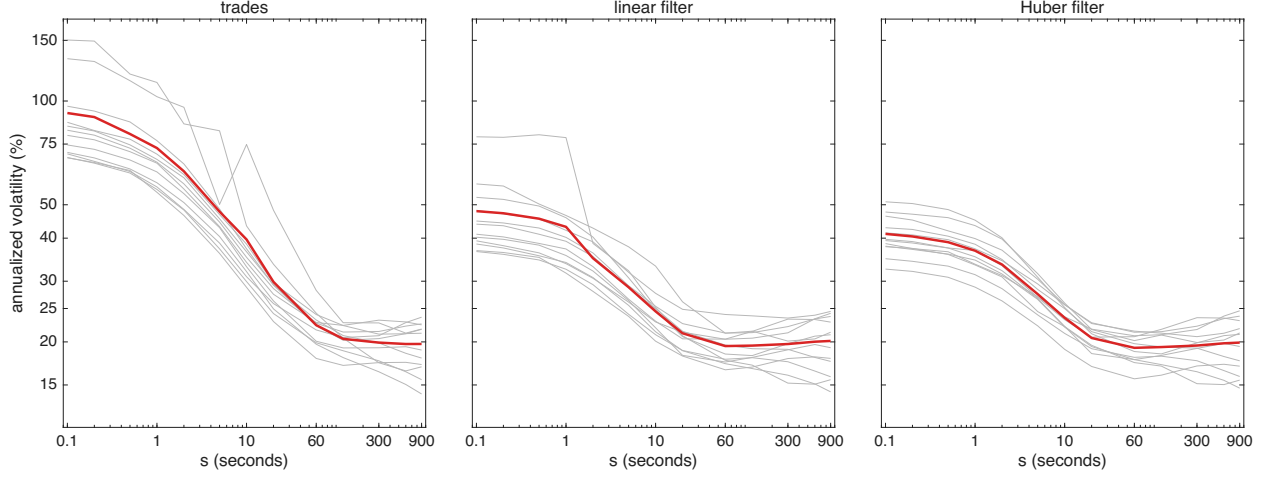
Figure 4: Volatility signature curves for AMGN over the 12 trading days in Oct 2024. The annualized vol \hat{\sigma}100\sqrt{252} from the returns \hat{X}_t - \hat{X}_{t,s} of Table 2, against the lag s in seconds, both axes on log scales, for: raw trades, linear filter & Huber filter. Grey lines are the individual trading days & the red line is the square root of the 12 day average of their squares. The linear & Huber returns carry the finite-sample correction c_{t,s} of the paper; the raw trades are unaffected by it.
