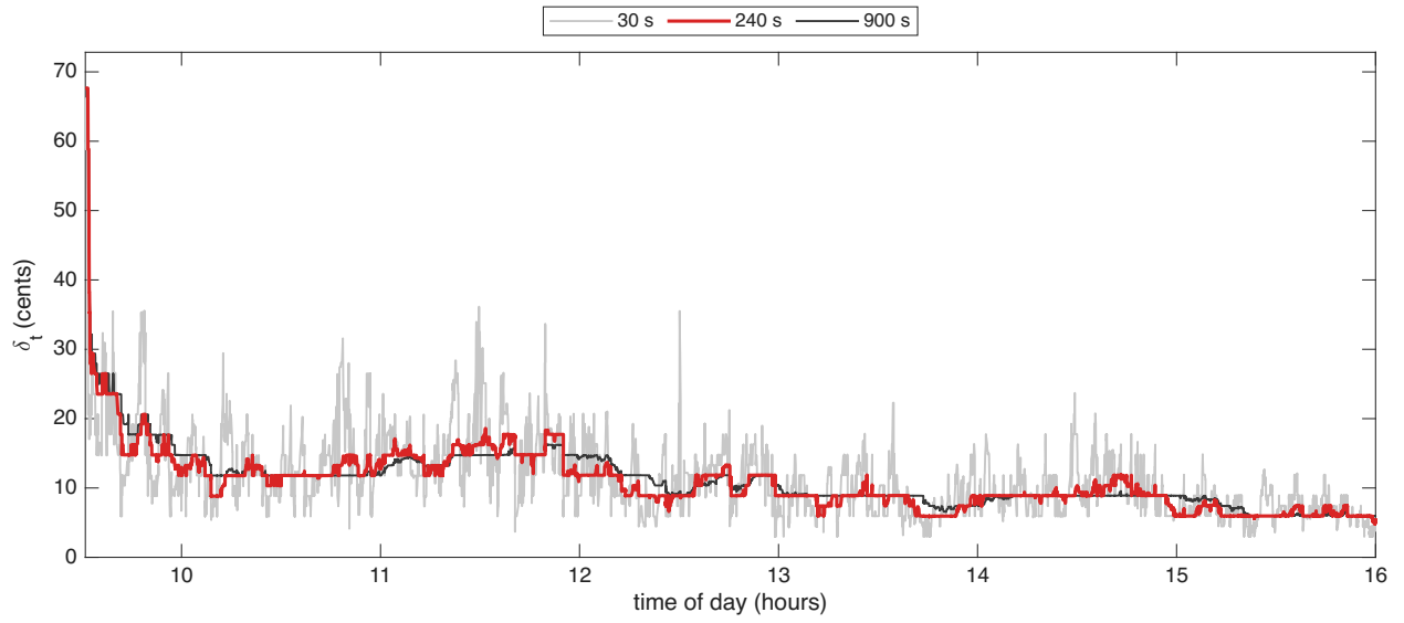
Figure 2: The Huber threshold \delta_t in cents for AMGN on 16 October 2024, with half-lives of 30, 240, 900 seconds. The 240-second half-life, in red, is used.
