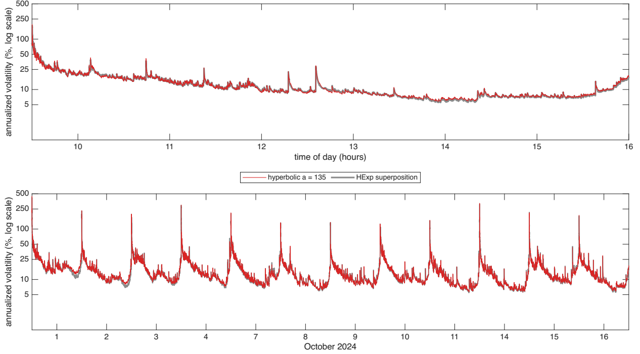
Figure 6: Hyperbolic against superposition weights for AMZN over 12 trading days in Oct 2024, the diurnally adjusted \hat{\sigma}(u)100\sqrt{252} at s = 1 second from the Huber filter, shown as annualized vol in % on a log10 scale. The only difference between the 2 paths is the weight function: the hyperbolic weights with a = 135 in red, drawn on top, and the HExp superposition in grey, 4 exponential components with half lives of 12, 50, 200, 800 seconds. Hyperparameters minimize the QLIKE objective. Top: 16 October 2024, bottom: 12 days.
