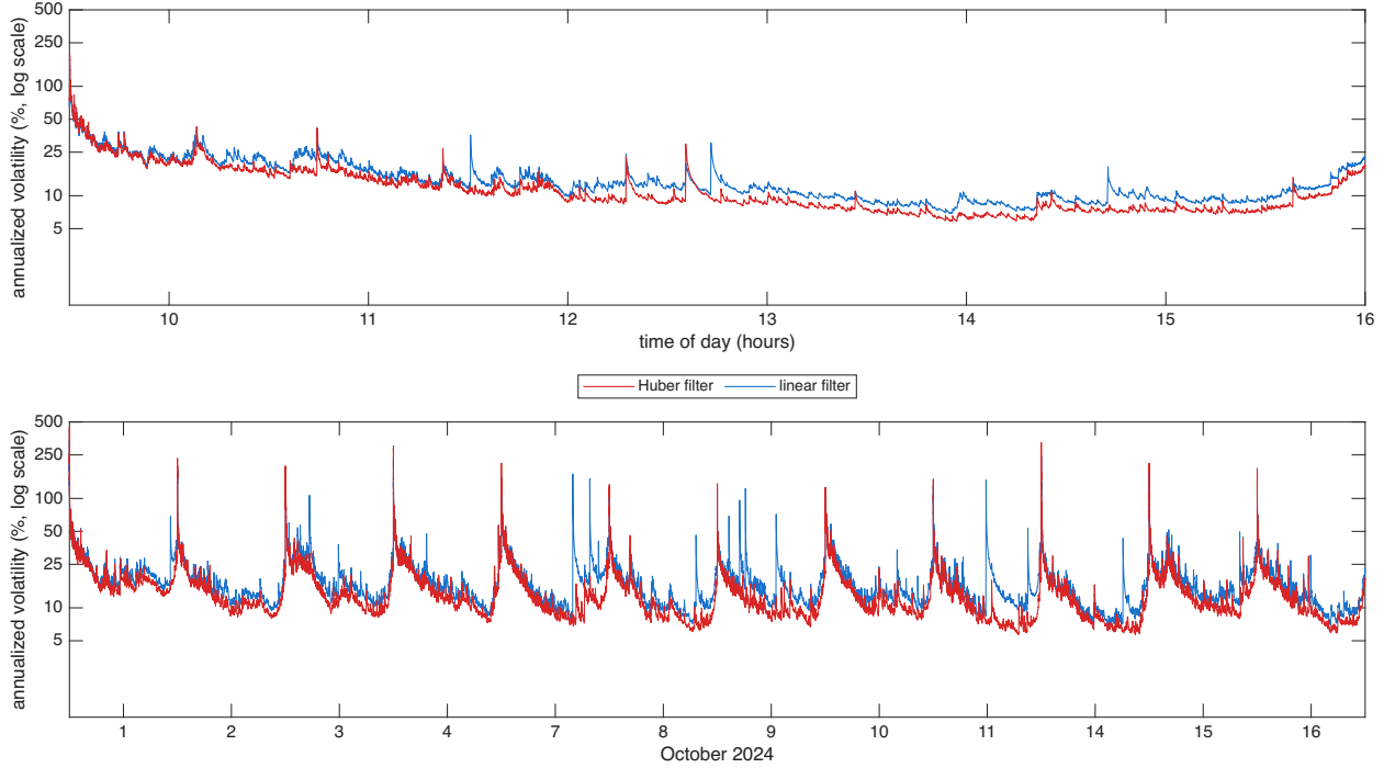
Figure 5: Filtered spot volatility for AMZN over 12 trading days in Oct 2024, the diurnally adjusted estimator \hat{\sigma}(u)100\sqrt{252} at s = 1 second with hyperbolic weights, Mandelbrot parameter a = 135 , with the input prices computed using the Huber & linear filters, shown as annualized volatility in percent on a log10 scale. Top: 16 October 2024, bottom: 12 days.
