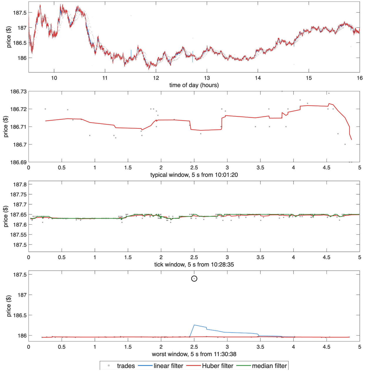
Figure 1: AMZN trades (grey points), the linear filter and the Huber filter, 16 October 2024. Top: full trading day. 2nd: 5-second window at the day's median trade count, from 10:01:20. 3rd: 5-second window at 10:28:35 in which the price reverses direction most often, with the median filter m_t added. Bottom: 5-second window around the largest Huber residual after 09:45, circled.
