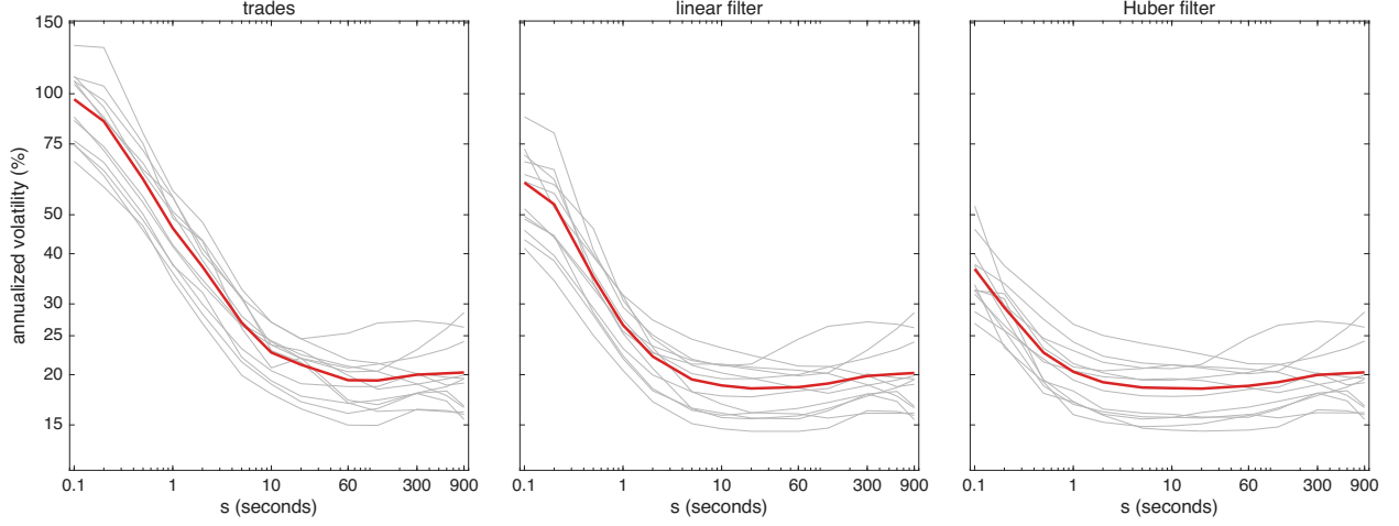
Figure 4: Volatility signature curves for AMZN over the 12 trading days in Oct 2024. The annualized vol \hat{\sigma}100\sqrt{252} from the returns \hat{X}_t - \hat{X}_{t,s} of Table 2, against the lag s in seconds, both axes on log scales, for: raw trades, linear filter & Huber filter. Grey lines are the individual trading days & the red line is the square root of the 12 day average of their squares. The linear & Huber returns carry the finite-sample correction c_{t,s} of the paper; the raw trades are unaffected by it.
