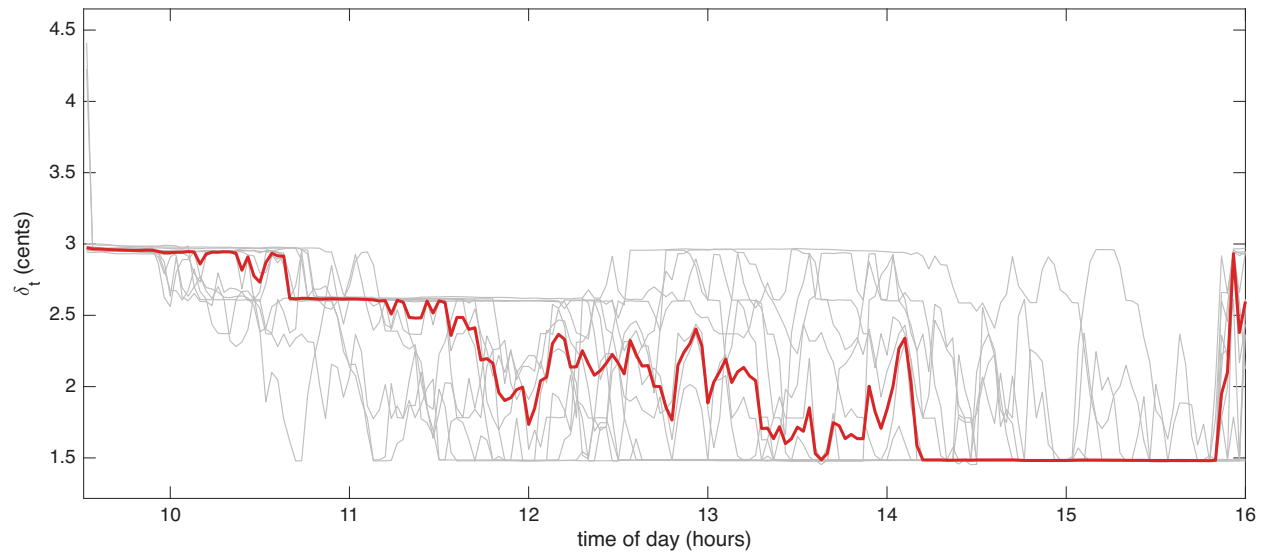
Figure 3: Huber threshold \delta_t in cents through the trading day, for 12 AMZN trading days in Oct 2024 (grey lines) and their median (red line).
