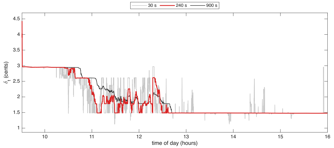
Figure 2: The Huber threshold \delta_t in cents for AMZN on 16 October 2024, with half-lives of 30, 240, 900 seconds. The 240-second half-life, in red, is used.
