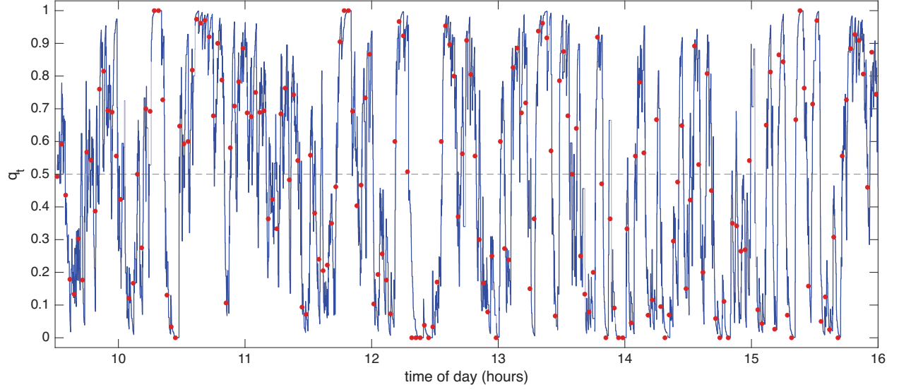
Figure 8: The directional conditional probability for AMZN, 16 October 2024. The filtered conditional probability q_t that an outlier lies above the robust Huber band, under exponential weights decaying in clock time with half life of 23 seconds; where fewer than two outliers remain in the weights it is drawn in grey. The dashed line marks 0.5. The red points are the empirical conditional probability using the 120 second bins of the previous figure.
