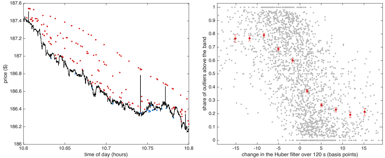
Figure 7: Outliers & robust price for AMZN on 16 October 2024. Left: the 12 minutes with the largest move in the Huber filter that day; outliers above Y_t - \theta_t > \delta_{t-1} in red, outliers below Y_t - \theta_t < -\delta_{t-1} in blue, Huber filter in black. Right: over the 12 trading days, the 120 second empirical conditional probability that outliers are above (rather than below) the Huber band against the 120 second change in the Huber filter in basis points: light points are single bins, the line & bars are means & s.e.
