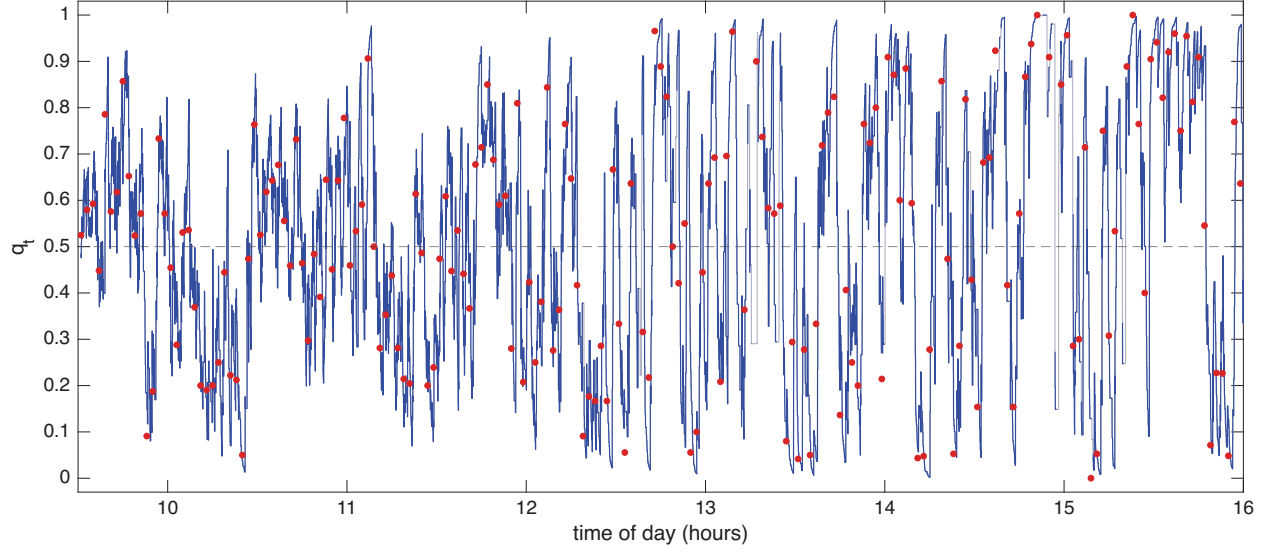
Figure 8: The directional conditional probability for AVGO , 16 October 2024. The filtered conditional probability q_t that an outlier lies above the robust Huber band, under exponential weights decaying in clock time with half life of 26 seconds; where fewer than two outliers remain in the weights it is drawn in grey. The dashed line marks 0.5. The red points are the empirical conditional probability using the 120 second bins of the previous figure.
