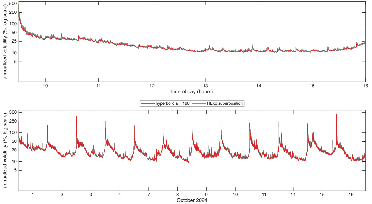
Figure 6: Hyperbolic against superposition weights for AVGO over 12 trading days in Oct 2024, the diurnally adjusted \hat{\sigma}(u)100\sqrt{252} at s = 1 second from the Huber filter, shown as annualized vol in % on a log10 scale. The only difference between the 2 paths is the weight function: the hyperbolic weights with a = 190 in red, drawn on top, and the HExp superposition in grey, 4 exponential components with half lives of 10, 100, 1000, 10000 seconds. Hyperparameters minimize the QLIKE objective. Top: 16 October 2024, bottom: 12 days.
