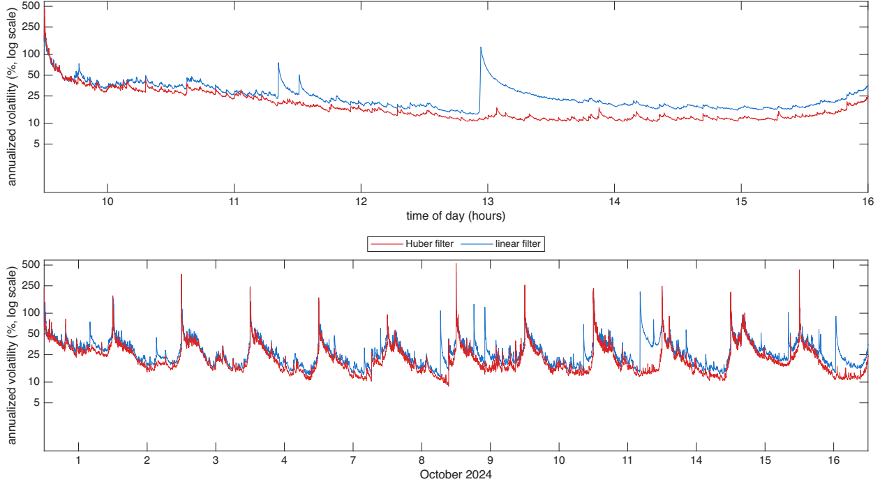
Figure 5: Filtered spot volatility for AVGO over 12 trading days in Oct 2024, the diurnally adjusted estimator \hat{\sigma}(u)100\sqrt{252} at s = 1 second with hyperbolic weights, Mandelbrot parameter a = 190 , with the input prices computed using the Huber & linear filters, shown as annualized volatility in percent on a log10 scale. Top: 16 October 2024, bottom: 12 days.
