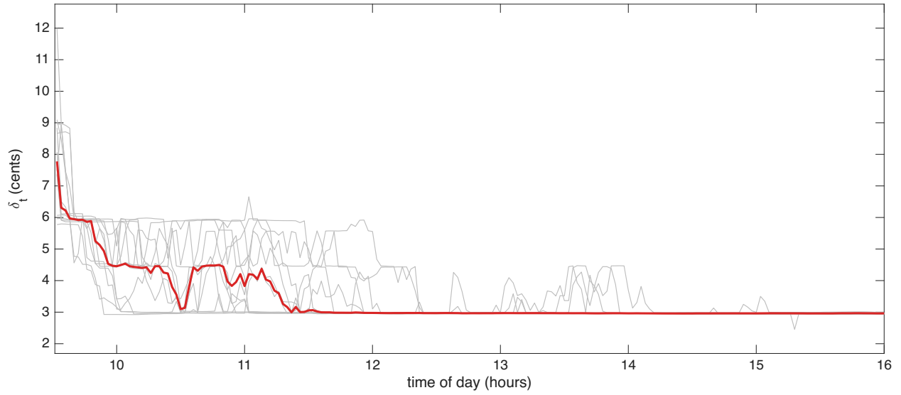
Figure 3: Huber threshold \delta_t in cents through the trading day, for 12 AVGO trading days in Oct 2024 (grey lines) and their median (red line).
