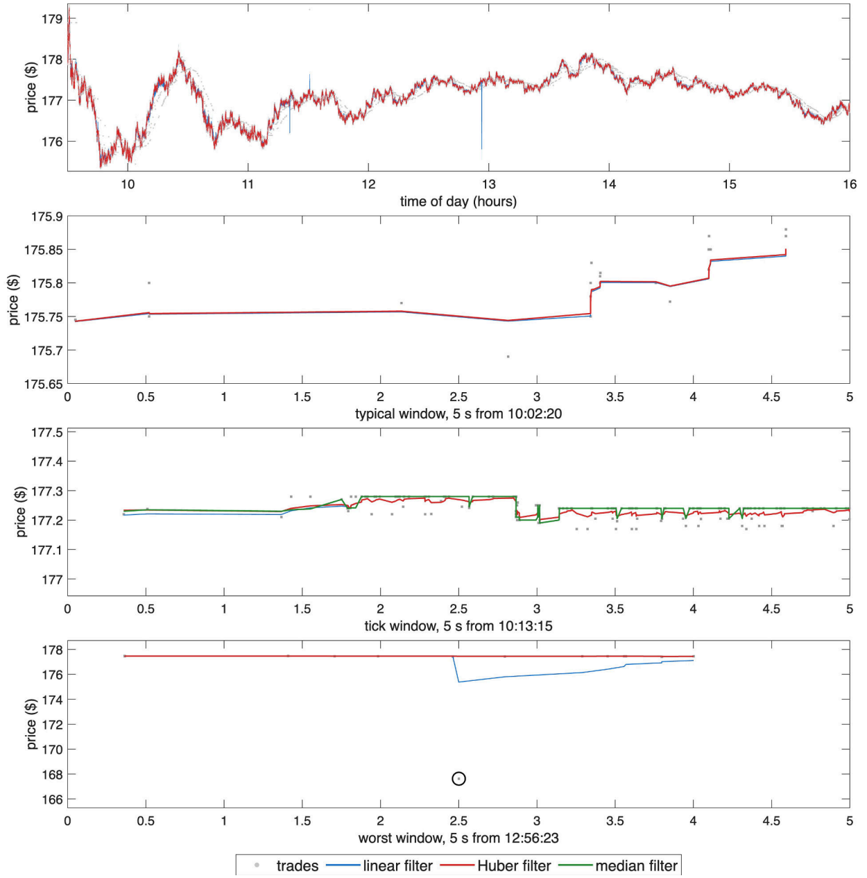
Figure 1: AVGO trades (grey points), the linear filter and the Huber filter, 16 October 2024. Top: full trading day. 2nd: 5-second window at the day's median trade count, from 10:02:20. 3rd: 5-second window at 10:13:15 in which the price reverses direction most often, with the median filter m_t added. Bottom: 5-second window around the largest Huber residual after 09:45, circled.
