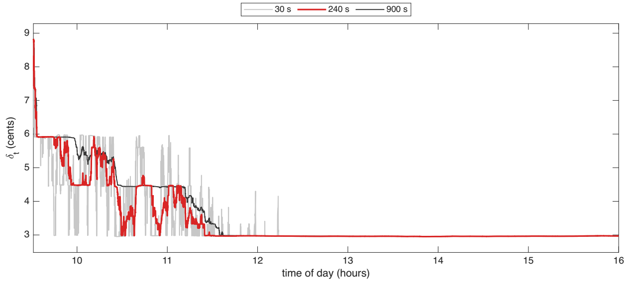
Figure 2: The Huber threshold \delta_t in cents for AVGO on 16 October 2024, with half-lives of 30, 240, 900 seconds. The 240-second half-life, in red, is used.
