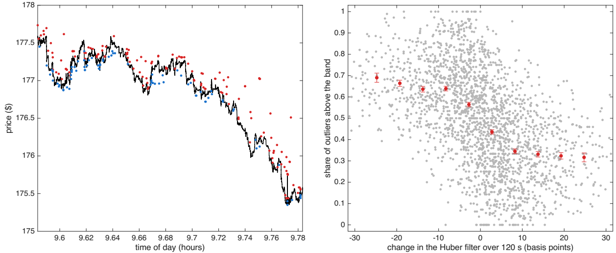
Figure 7: Outliers & robust price for AVGO on 16 October 2024. Left: the 12 minutes with the largest move in the Huber filter that day; outliers above Y_t - \theta_t > \delta_{t-1} in red, outliers below Y_t - \theta_t < -\delta_{t-1} in blue, Huber filter in black. Right: over the 12 trading days, the 120 second empirical conditional probability that outliers are above (rather than below) the Huber band against the 120 second change in the Huber filter in basis points: light points are single bins, the line & bars are means & s.e.
