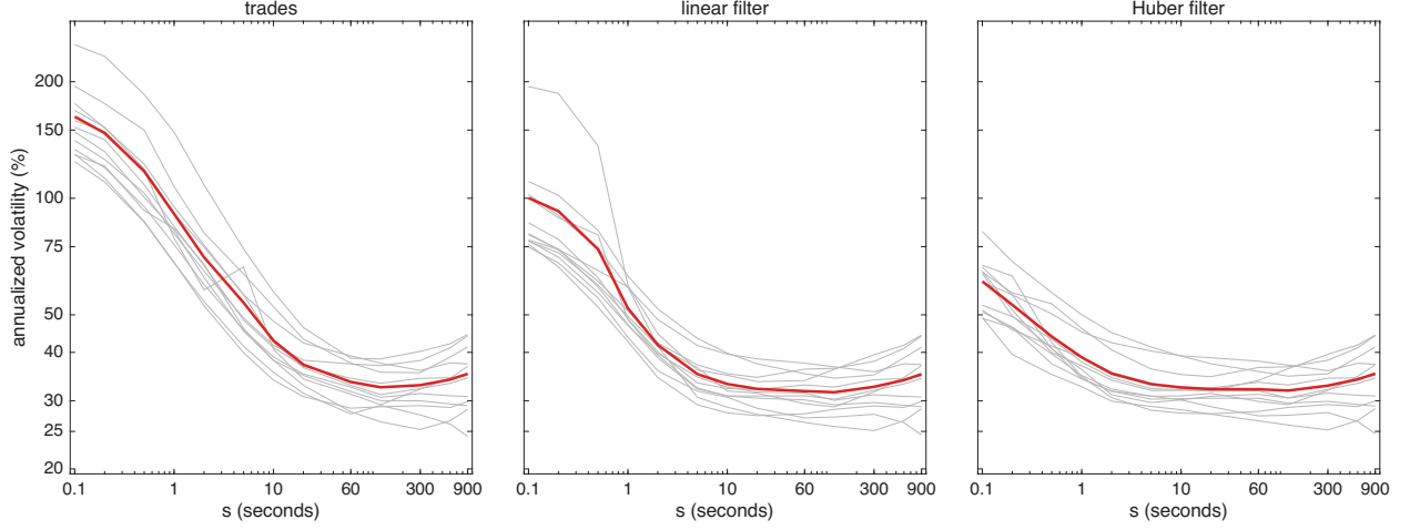
Figure 4: Volatility signature curves for AVGO over the 12 trading days in Oct 2024. The annualized vol \hat{\sigma}100\sqrt{252} from the returns \hat{X}_t - \hat{X}_{t,s} of Table 2, against the lag s in seconds, both axes on log scales, for: raw trades, linear filter & Huber filter. Grey lines are the individual trading days & the red line is the square root of the 12 day average of their squares. The linear & Huber returns carry the finite-sample correction c_{t,s} of the paper; the raw trades are unaffected by it.
