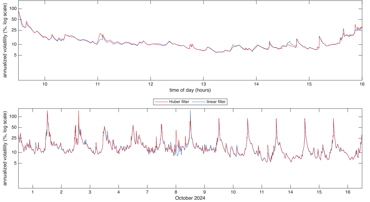
Figure 5: Filtered spot volatility for CALM over 12 trading days in Oct 2024, the diurnally adjusted estimator \hat{\sigma}(u)100\sqrt{252} at s = 1 second with hyperbolic weights, Mandelbrot parameter a = 18 , with the input prices computed using the Huber & linear filters, shown as annualized volatility in percent on a log10 scale. Top: 16 October 2024, bottom: 12 days.
