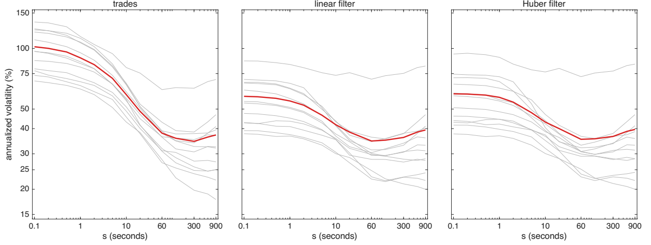
Figure 4: Volatility signature curves for CALM over the 12 trading days in Oct 2024. The annualized vol \hat{\sigma}100\sqrt{252} from the returns \hat{X}_t - \hat{X}_{t,s} of Table 2, against the lag s in seconds, both axes on log scales, for: raw trades, linear filter & Huber filter. Grey lines are the individual trading days & the red line is the square root of the 12 day average of their squares. The linear & Huber returns carry the finite-sample correction c_{t,s} of the paper; the raw trades are unaffected by it.
