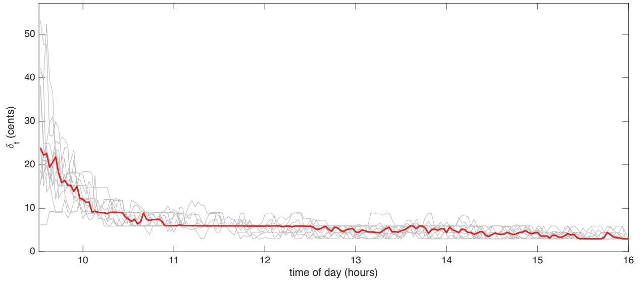
Figure 3: Huber threshold \delta_t in cents through the trading day, for 12 CALM trading days in Oct 2024 (grey lines) and their median (red line).
