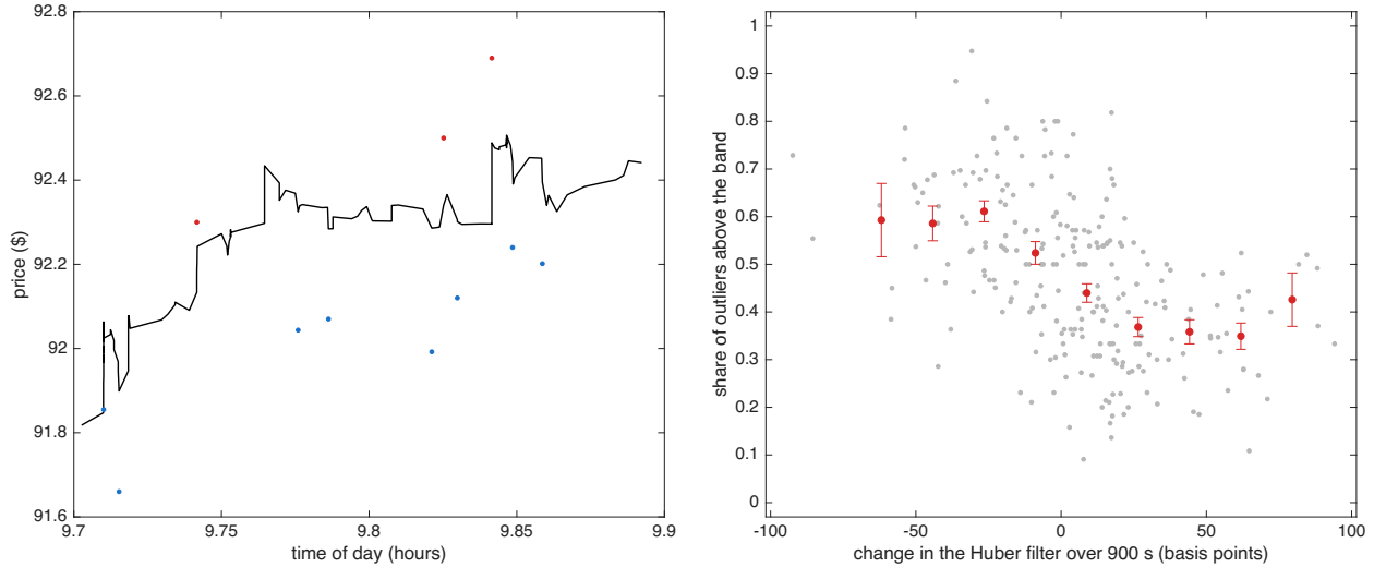
Figure 7: Outliers & robust price for CALM on 16 October 2024. Left: the 12 minutes with the largest move in the Huber filter that day; outliers above Y_t - \theta_t > \delta_{t-1} in red, outliers below Y_t - \theta_t < -\delta_{t-1} in blue, Huber filter in black. Right: over the 12 trading days, the 900 second empirical conditional probability that outliers are above (rather than below) the Huber band against the 900 second change in the Huber filter in basis points: light points are single bins, the line & bars are means & s.e.
