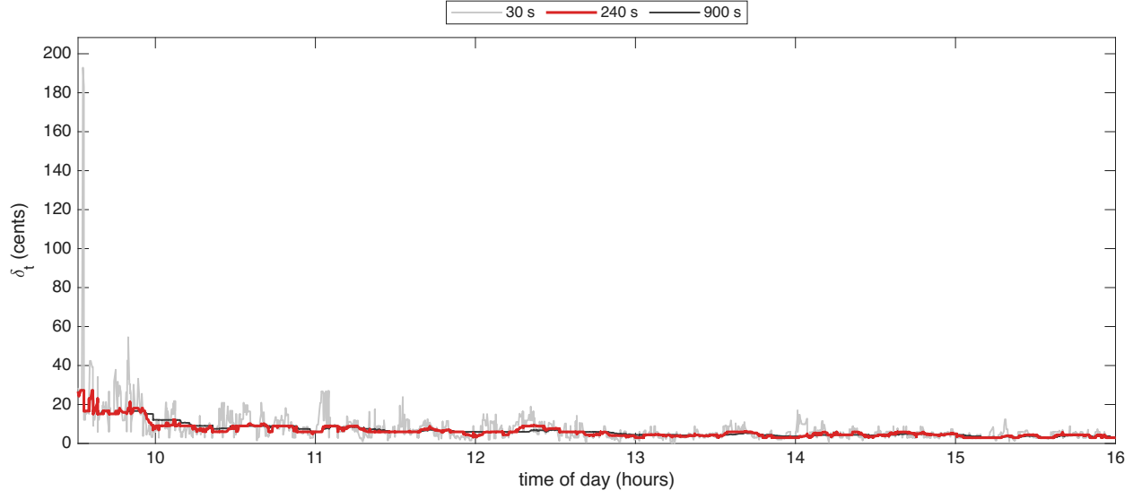
Figure 2: The Huber threshold \delta_t in cents for CALM on 16 October 2024, with half-lives of 30, 240, 900 seconds. The 240-second half-life, in red, is used.
