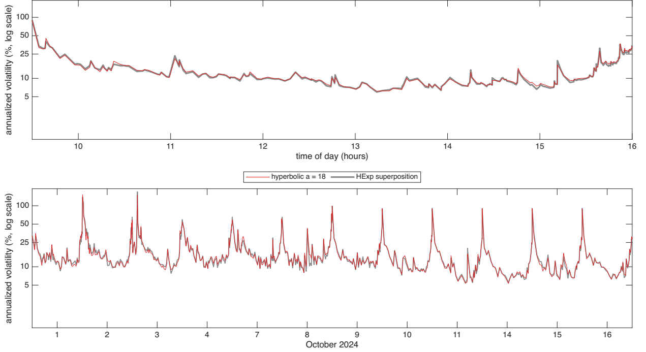
Figure 6: Hyperbolic against superposition weights for CALM over 12 trading days in Oct 2024, the diurnally adjusted \hat{\sigma}(u)100\sqrt{252} at s = 1 second from the Huber filter, shown as annualized vol in % on a log10 scale. The only difference between the 2 paths is the weight function: the hyperbolic weights with a = 18 in red, drawn on top, and the HExp superposition in grey, 4 exponential components with half lives of 10, 100, 1000, 10000 seconds. Hyperparameters minimize the QLIKE objective. Top: 16 October 2024, bottom: 12 days.
