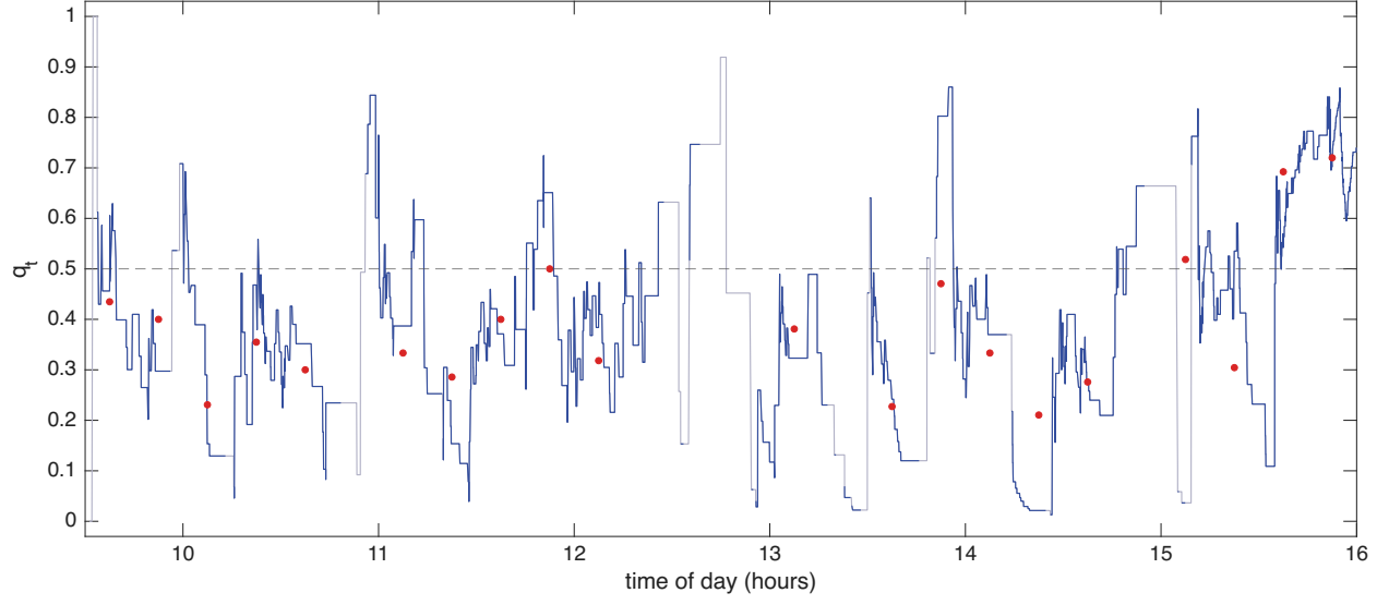
Figure 8: The directional conditional probability for CALM , 16 October 2024. The filtered conditional probability q_t that an outlier lies above the robust Huber band, under exponential weights decaying in clock time with half life of 177 seconds; where fewer than two outliers remain in the weights it is drawn in grey. The dashed line marks 0.5. The red points are the empirical conditional probability using the 900 second bins of the previous figure.
