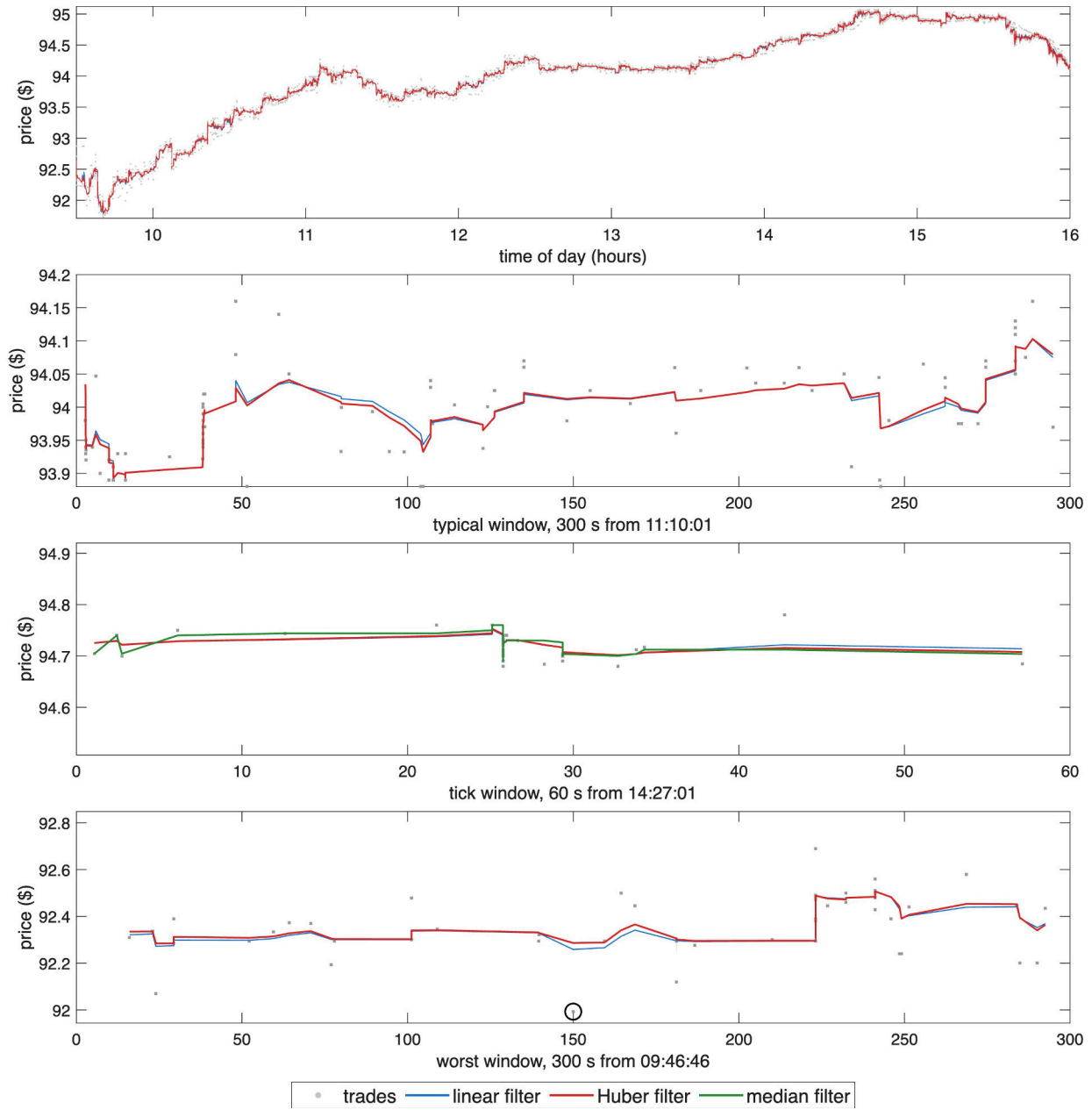
Figure 1: CALM trades (grey points), the linear filter and the Huber filter, 16 October 2024. Top: full trading day. 2nd: 300-second window at the day's median trade count, from 11:10:01. 3rd: 60-second window at 14:27:01 in which the price reverses direction most often, with the median filter m_t added. Bottom: 300-second window around the largest Huber residual after 09:45, circled.
