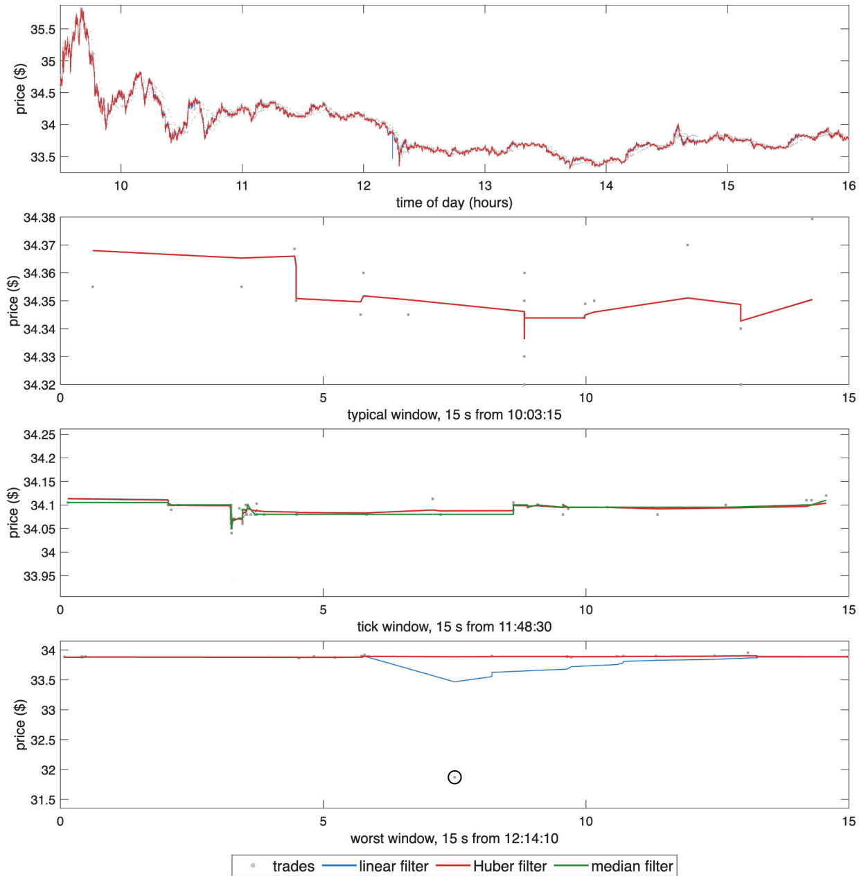
Figure 1: CELH trades (grey points), the linear filter and the Huber filter, 16 October 2024. Top: full trading day. 2nd: 15-second window at the day's median trade count, from 10:03:15. 3rd: 15-second window at 11:48:30 in which the price reverses direction most often, with the median filter m_t added. Bottom: 15-second window around the largest Huber residual after 09:45, circled.
