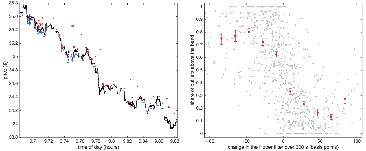
Figure 7: Outliers & robust price for CELH on 16 October 2024. Left: the 12 minutes with the largest move in the Huber filter that day; outliers above Y_t - \theta_t > \delta_{t-1} in red, outliers below Y_t - \theta_t < -\delta_{t-1} in blue, Huber filter in black. Right: over the 12 trading days, the 300 second empirical conditional probability that outliers are above (rather than below) the Huber band against the 300 second change in the Huber filter in basis points: light points are single bins, the line & bars are means & s.e.
