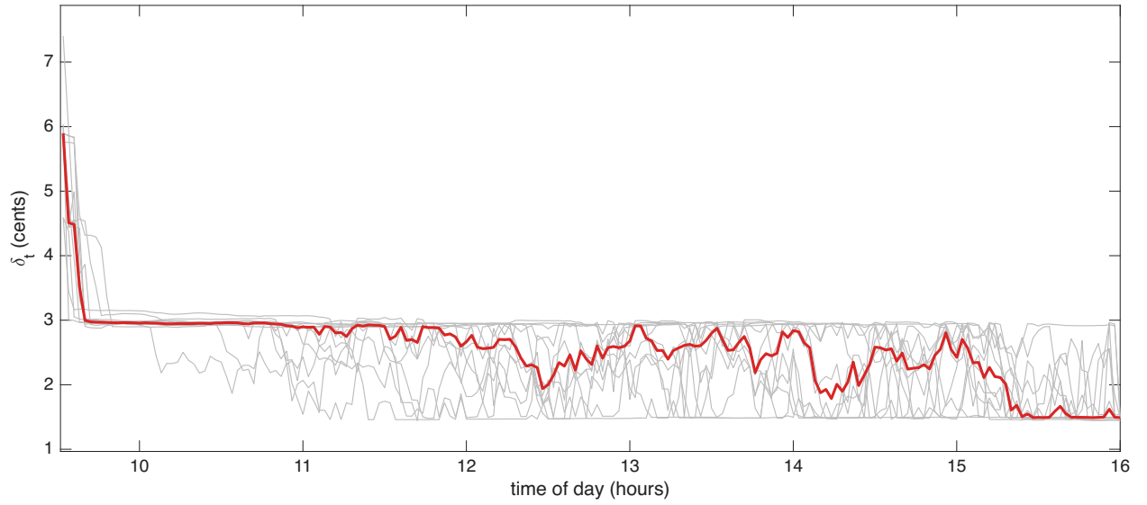
Figure 3: Huber threshold \delta_t in cents through the trading day, for 12 CELH trading days in Oct 2024 (grey lines) and their median (red line).
