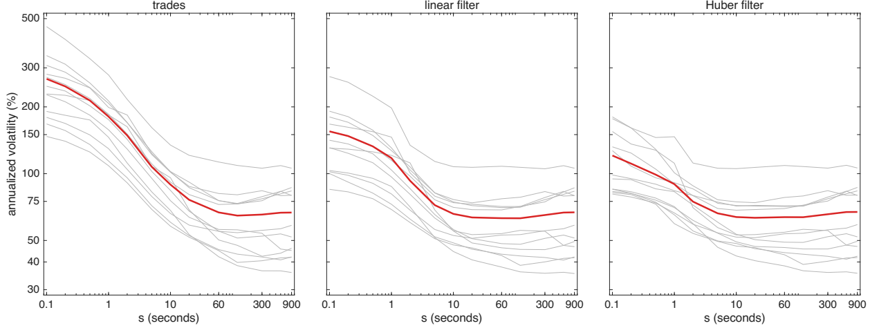
Figure 4: Volatility signature curves for CELH over the 12 trading days in Oct 2024. The annualized vol \hat{\sigma}100\sqrt{252} from the returns \hat{X}_t - \hat{X}_{t,s} of Table 2, against the lag s in seconds, both axes on log scales, for: raw trades, linear filter & Huber filter. Grey lines are the individual trading days & the red line is the square root of the 12 day average of their squares. The linear & Huber returns carry the finite-sample correction c_{t,s} of the paper; the raw trades are unaffected by it.
