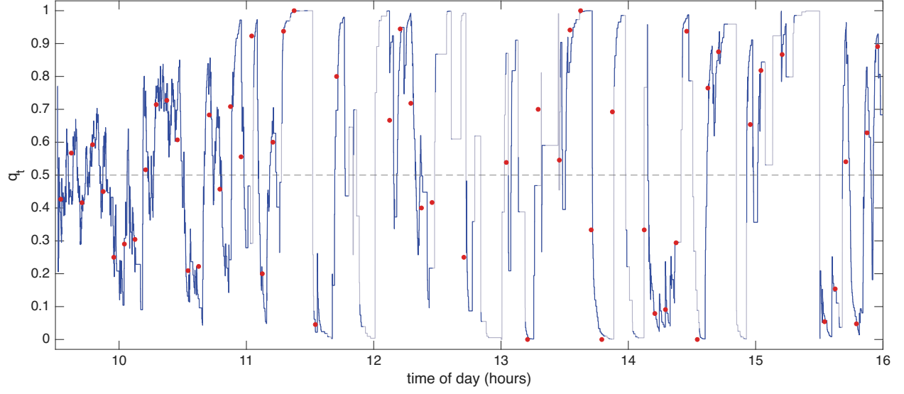
Figure 8: The directional conditional probability for CELH , 16 October 2024. The filtered conditional probability q_t that an outlier lies above the robust Huber band, under exponential weights decaying in clock time with half life of 56 seconds; where fewer than two outliers remain in the weights it is drawn in grey. The dashed line marks 0.5. The red points are the empirical conditional probability using the 300 second bins of the previous figure.
