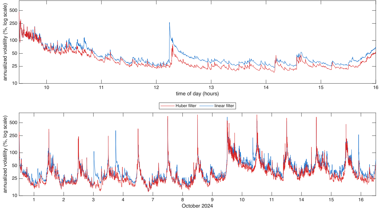
Figure 5: Filtered spot volatility for CELH over 12 trading days in Oct 2024, the diurnally adjusted estimator \hat{\sigma}(u)100\sqrt{252} at s = 1 second with hyperbolic weights, Mandelbrot parameter a = 45 , with the input prices computed using the Huber & linear filters, shown as annualized volatility in percent on a log10 scale. Top: 16 October 2024, bottom: 12 days.
