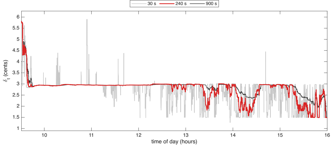
Figure 2: The Huber threshold \delta_t in cents for CELH on 16 October 2024, with half-lives of 30, 240, 900 seconds. The 240-second half-life, in red, is used.
