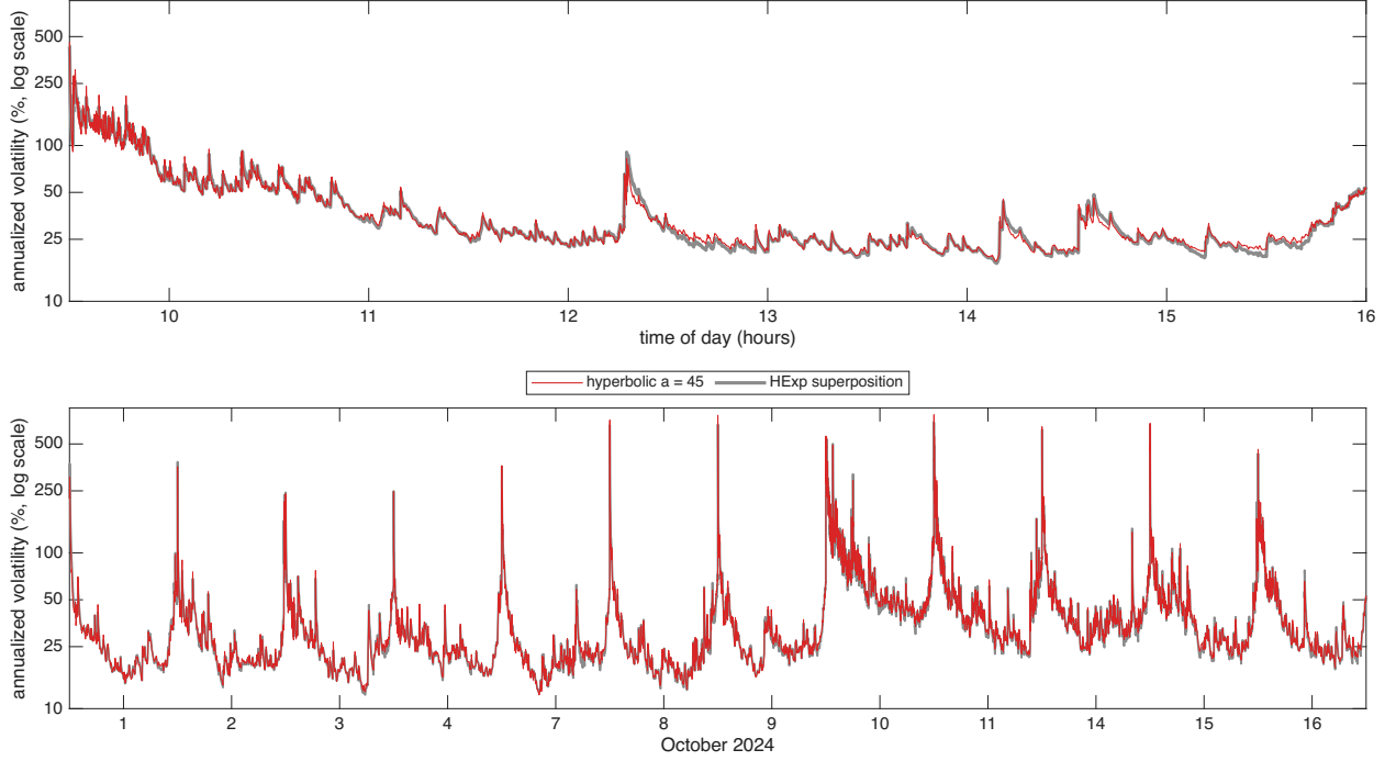
Figure 6: Hyperbolic against superposition weights for CELH over 12 trading days in Oct 2024, the diurnally adjusted \hat{\sigma}(u)100\sqrt{252} at s = 1 second from the Huber filter, shown as annualized vol in % on a log10 scale. The only difference between the 2 paths is the weight function: the hyperbolic weights with a = 45 in red, drawn on top, and the HExp superposition in grey, 4 exponential components with half lives of 10, 100, 1000, 10000 seconds. Hyperparameters minimize the QLIKE objective. Top: 16 October 2024, bottom: 12 days.
