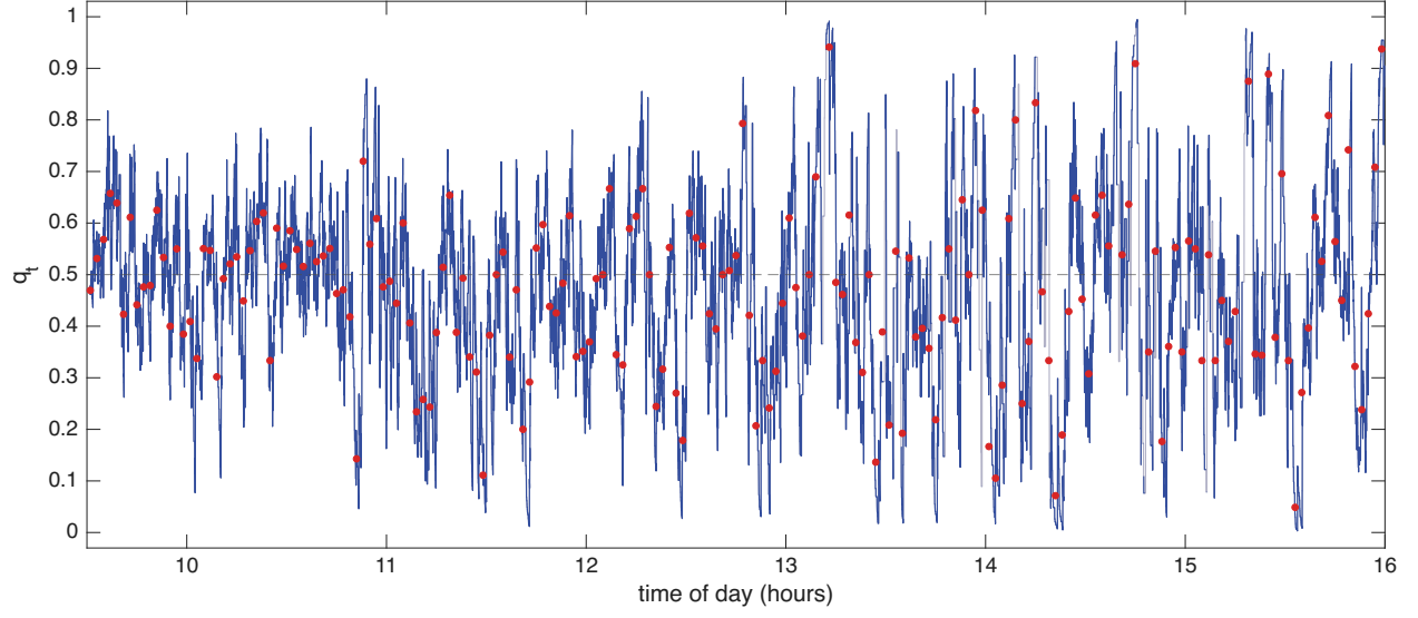
Figure 8: The directional conditional probability for COIN , 16 October 2024. The filtered conditional probability q_t that an outlier lies above the robust Huber band, under exponential weights decaying in clock time with half life of 20 seconds; where fewer than two outliers remain in the weights it is drawn in grey. The dashed line marks 0.5. The red points are the empirical conditional probability using the 120 second bins of the previous figure.
