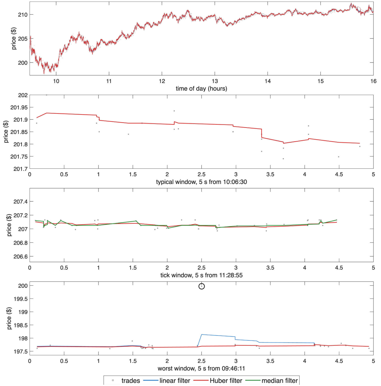
Figure 1: COIN trades (grey points), the linear filter and the Huber filter, 16 October 2024. Top: full trading day. 2nd: 5-second window at the day's median trade count, from 10:06:30. 3rd: 5-second window at 11:28:55 in which the price reverses direction most often, with the median filter m_t added. Bottom: 5-second window around the largest Huber residual after 09:45, circled.
