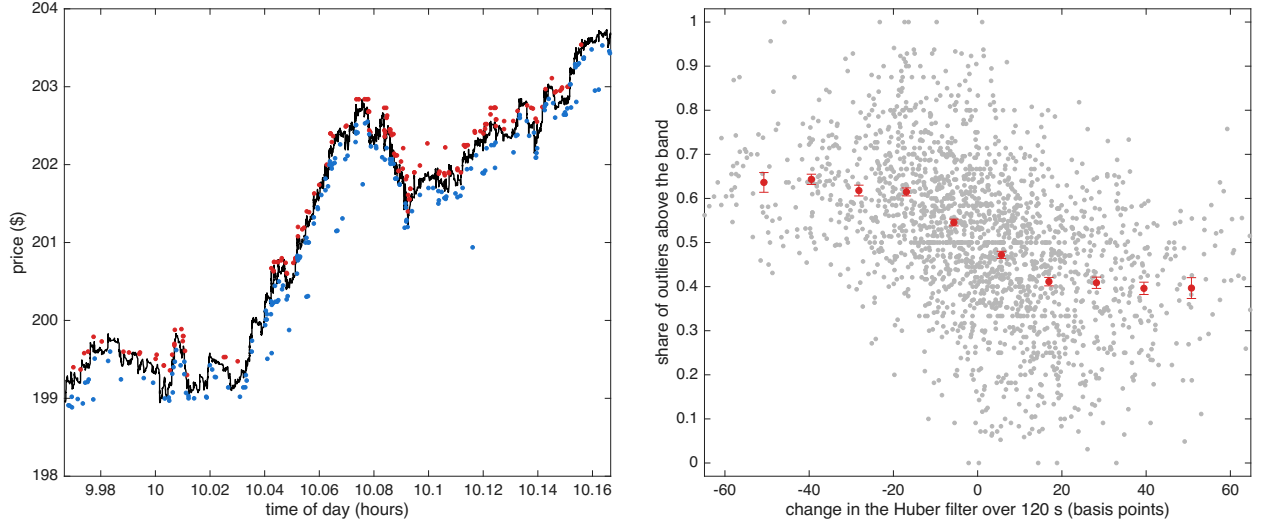
Figure 7: Outliers & robust price for COIN on 16 October 2024. Left: the 12 minutes with the largest move in the Huber filter that day; outliers above Y_t - \theta_t > \delta_{t-1} in red, outliers below Y_t - \theta_t < -\delta_{t-1} in blue, Huber filter in black. Right: over the 12 trading days, the 120 second empirical conditional probability that outliers are above (rather than below) the Huber band against the 120 second change in the Huber filter in basis points: light points are single bins, the line & bars are means & s.e.
