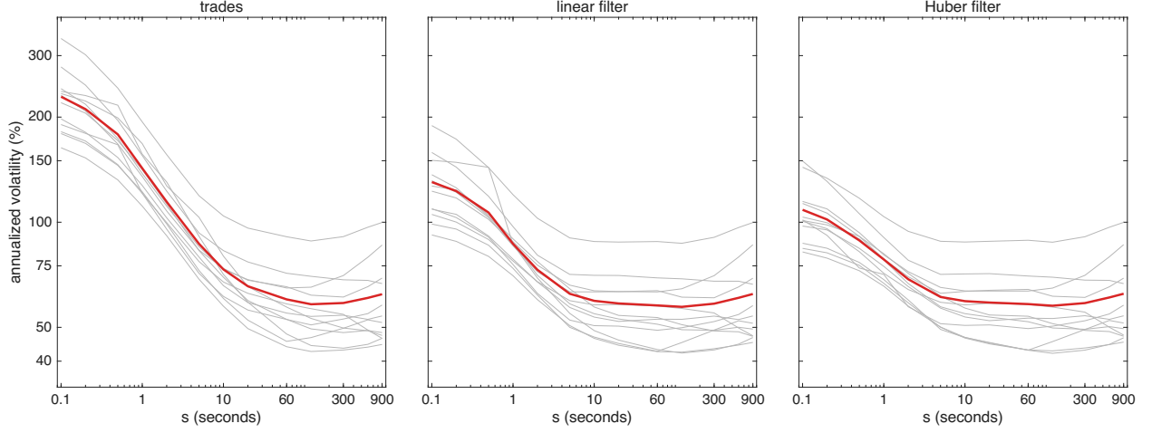
Figure 4: Volatility signature curves for COIN over the 12 trading days in Oct 2024. The annualized vol \hat{\sigma}100\sqrt{252} from the returns \hat{X}_t - \hat{X}_{t,s} of Table 2, against the lag s in seconds, both axes on log scales, for: raw trades, linear filter & Huber filter. Grey lines are the individual trading days & the red line is the square root of the 12 day average of their squares. The linear & Huber returns carry the finite-sample correction c_{t,s} of the paper; the raw trades are unaffected by it.
