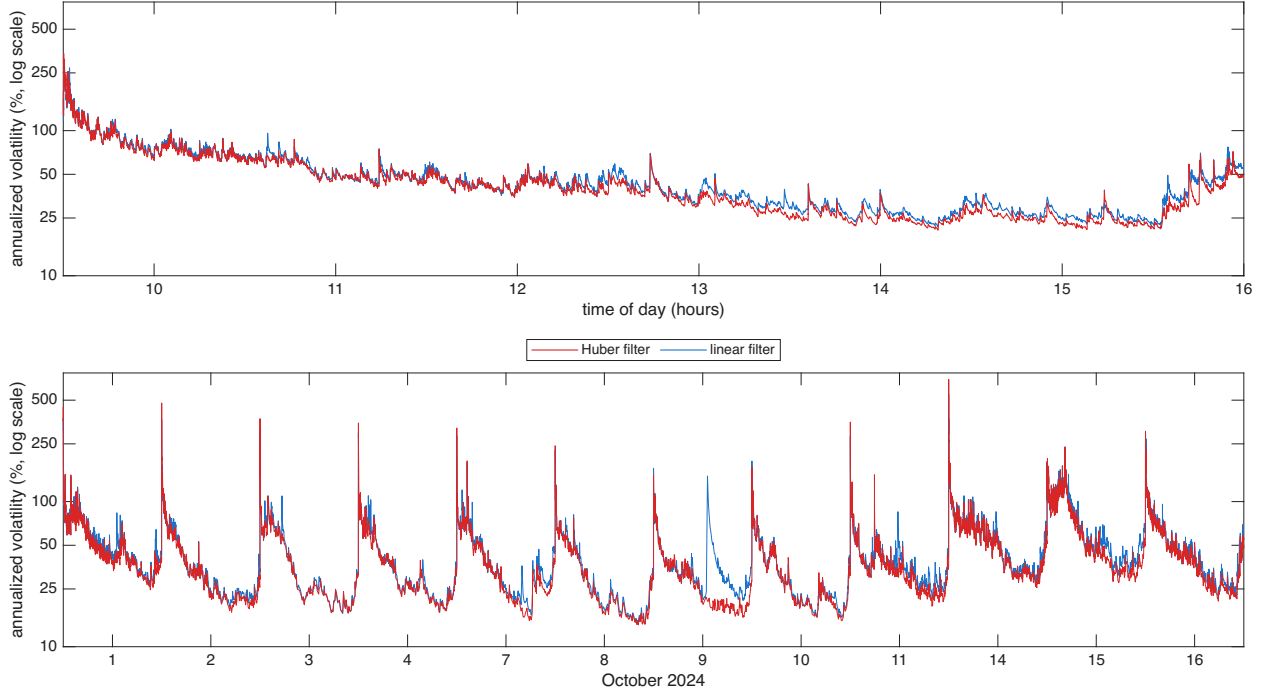
Figure 5: Filtered spot volatility for COIN over 12 trading days in Oct 2024, the diurnally adjusted estimator \hat{\sigma}(u)100\sqrt{252} at s = 1 second with hyperbolic weights, Mandelbrot parameter a = 73 , with the input prices computed using the Huber & linear filters, shown as annualized volatility in percent on a log10 scale. Top: 16 October 2024, bottom: 12 days.
