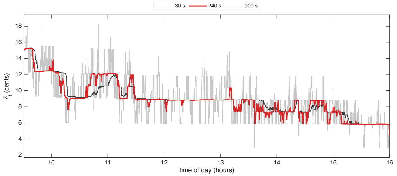
Figure 2: The Huber threshold \delta_t in cents for COIN on 16 October 2024, with half-lives of 30, 240, 900 seconds. The 240-second half-life, in red, is used.
