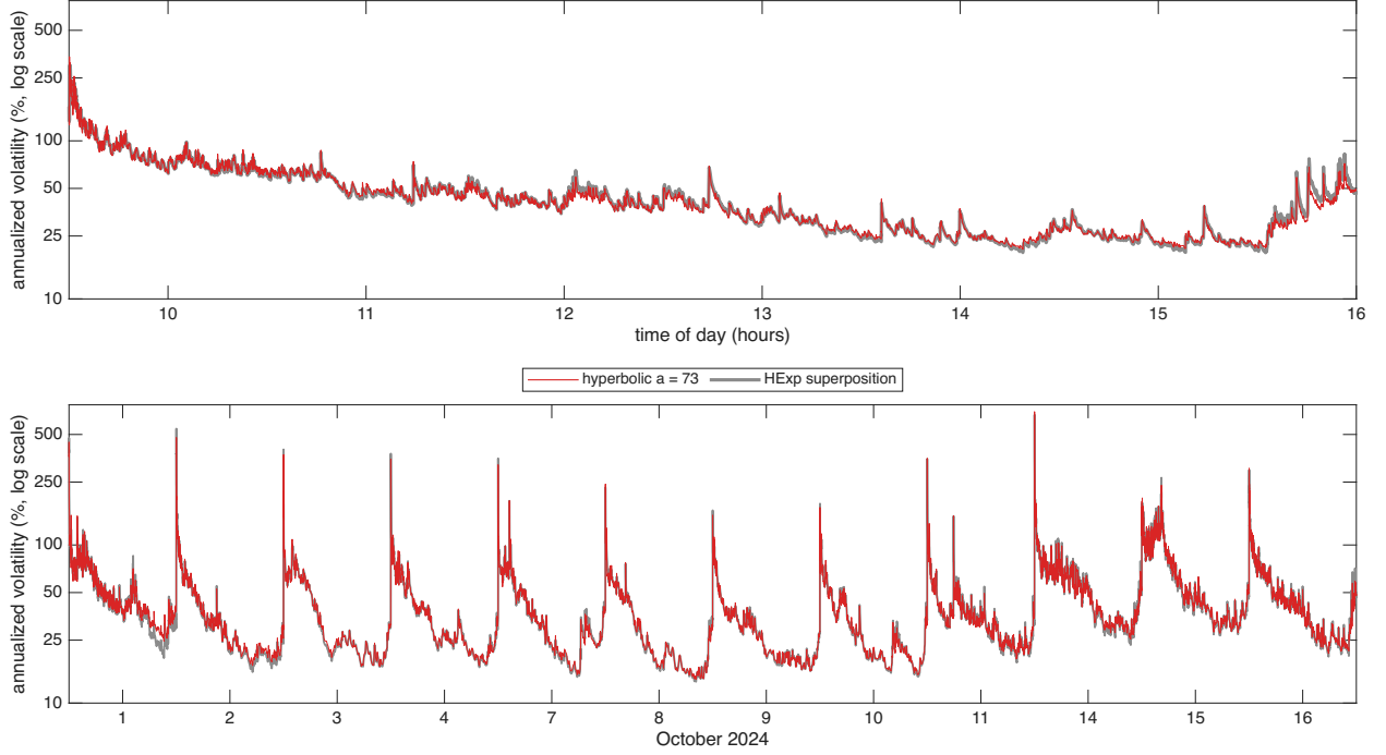
Figure 6: Hyperbolic against superposition weights for COIN over 12 trading days in Oct 2024, the diurnally adjusted \hat{\sigma}(u)100\sqrt{252} at s = 1 second from the Huber filter, shown as annualized vol in % on a log10 scale. The only difference between the 2 paths is the weight function: the hyperbolic weights with a = 73 in red, drawn on top, and the HExp superposition in grey, 4 exponential components with half lives of 2, 20, 200, 2000 seconds. Hyperparameters minimize the QLIKE objective. Top: 16 October 2024, bottom: 12 days.
