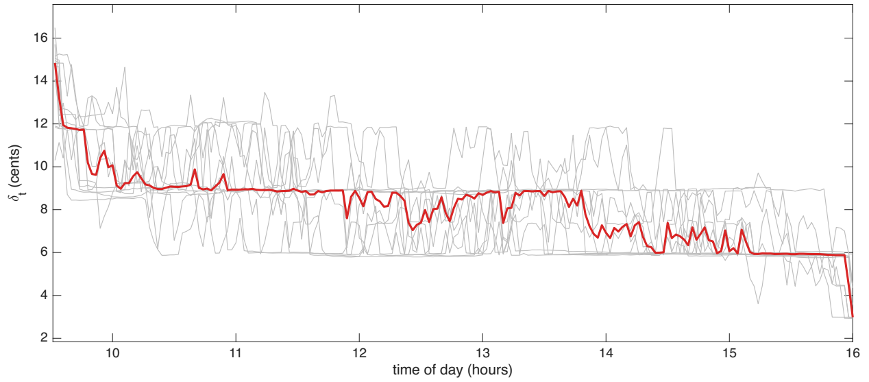
Figure 3: Huber threshold \delta_t in cents through the trading day, for 12 COIN trading days in Oct 2024 (grey lines) and their median (red line).
