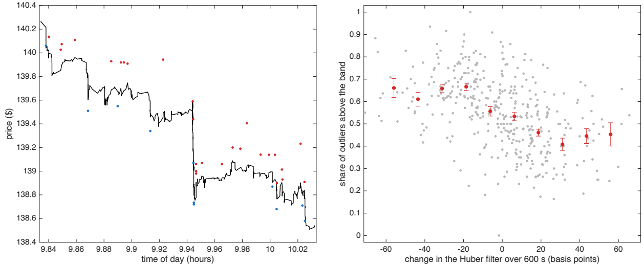
Figure 7: Outliers & robust price for CROX on 16 October 2024. Left: the 12 minutes with the largest move in the Huber filter that day; outliers above Y_t - \theta_t > \delta_{t-1} in red, outliers below Y_t - \theta_t < -\delta_{t-1} in blue, Huber filter in black. Right: over the 12 trading days, the 600 second empirical conditional probability that outliers are above (rather than below) the Huber band against the 600 second change in the Huber filter in basis points: light points are single bins, the line & bars are means & s.e.
