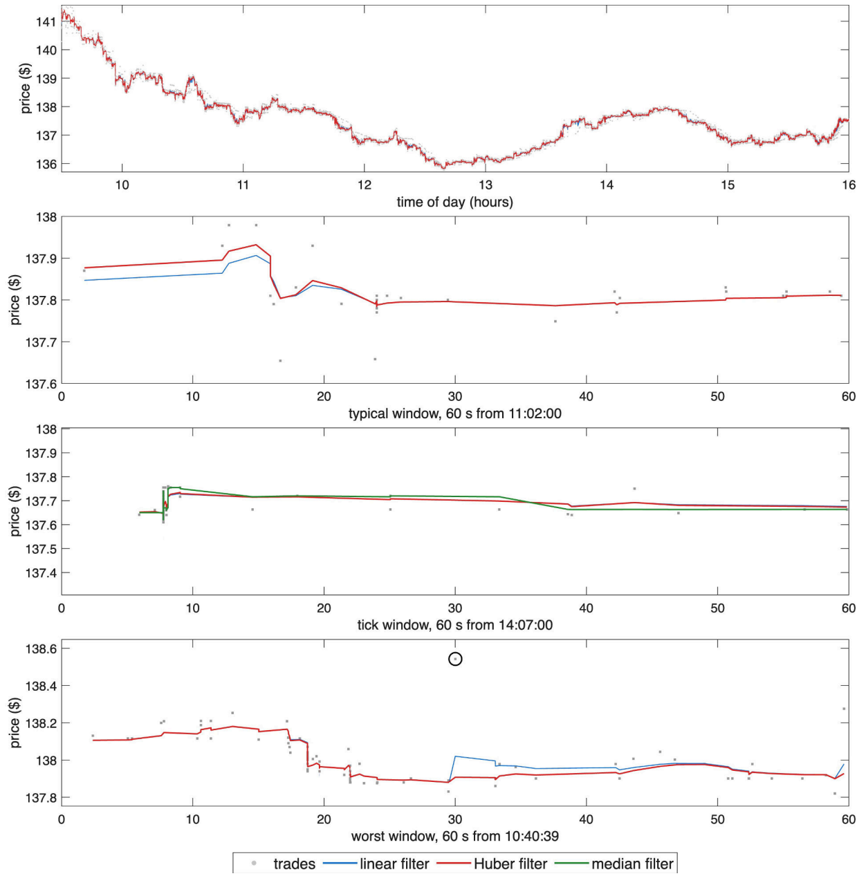
Figure 1: CROX trades (grey points), the linear filter and the Huber filter, 16 October 2024. Top: full trading day. 2nd: 60-second window at the day's median trade count, from 11:02:00. 3rd: 60-second window at 14:07:00 in which the price reverses direction most often, with the median filter m_t added. Bottom: 60-second window around the largest Huber residual after 09:45, circled.
