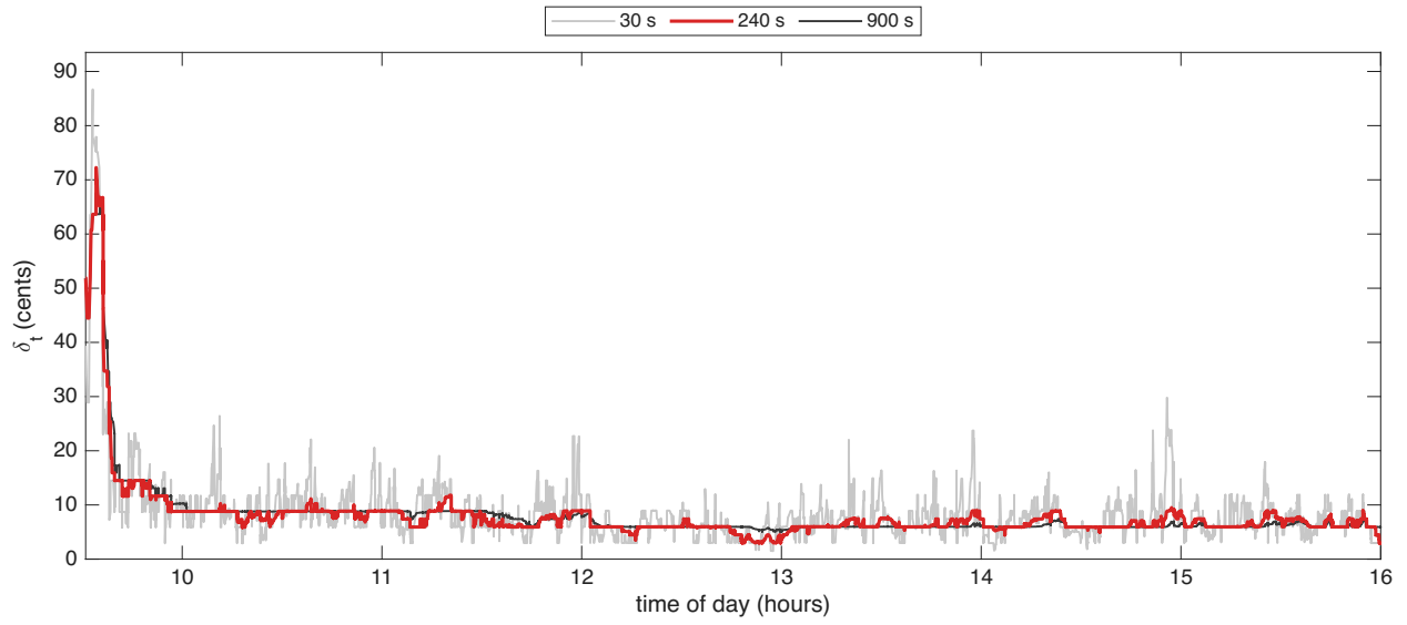
Figure 2: The Huber threshold \delta_t in cents for CROX on 16 October 2024, with half-lives of 30, 240, 900 seconds. The 240-second half-life, in red, is used.
