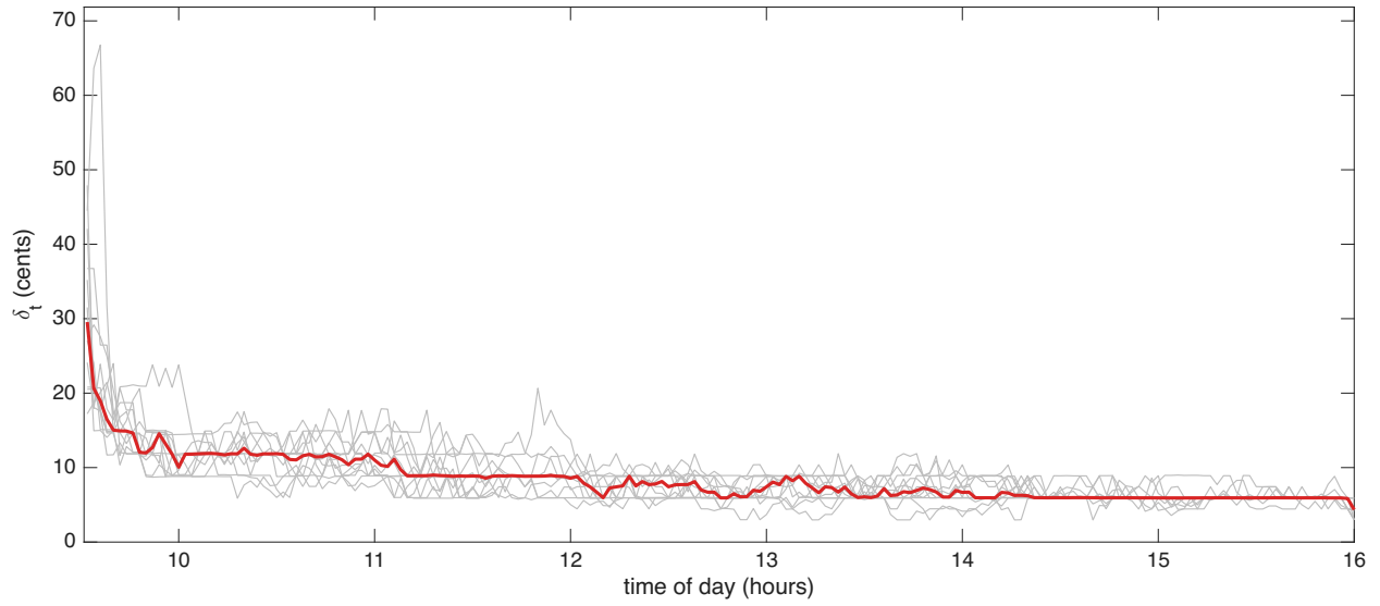
Figure 3: Huber threshold \delta_t in cents through the trading day, for 12 CROX trading days in Oct 2024 (grey lines) and their median (red line).
