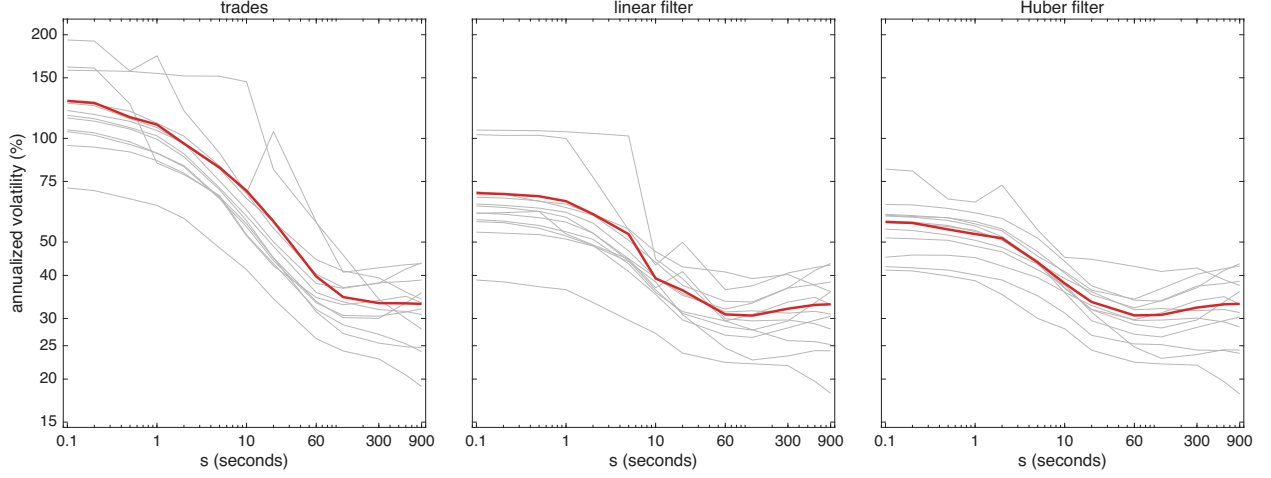
Figure 4: Volatility signature curves for CROX over the 12 trading days in Oct 2024. The annualized vol \hat{\sigma}100\sqrt{252} from the returns \hat{X}_t - \hat{X}_{t,s} of Table 2, against the lag s in seconds, both axes on log scales, for: raw trades, linear filter & Huber filter. Grey lines are the individual trading days & the red line is the square root of the 12 day average of their squares. The linear & Huber returns carry the finite-sample correction c_{t,s} of the paper; the raw trades are unaffected by it.
