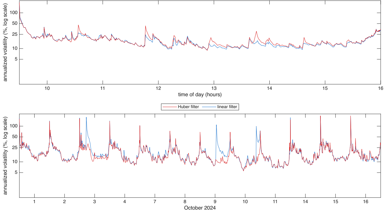
Figure 5: Filtered spot volatility for CROX over 12 trading days in Oct 2024, the diurnally adjusted estimator \hat{\sigma}(u)100\sqrt{252} at s = 1 second with hyperbolic weights, Mandelbrot parameter a = 24 , with the input prices computed using the Huber & linear filters, shown as annualized volatility in percent on a log10 scale. Top: 16 October 2024, bottom: 12 days.
