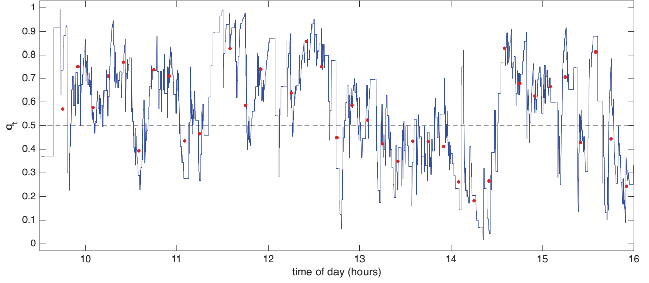
Figure 8: The directional conditional probability for CROX , 16 October 2024. The filtered conditional probability q_t that an outlier lies above the robust Huber band, under exponential weights decaying in clock time with half life of 93 seconds; where fewer than two outliers remain in the weights it is drawn in grey. The dashed line marks 0.5. The red points are the empirical conditional probability using the 600 second bins of the previous figure.
