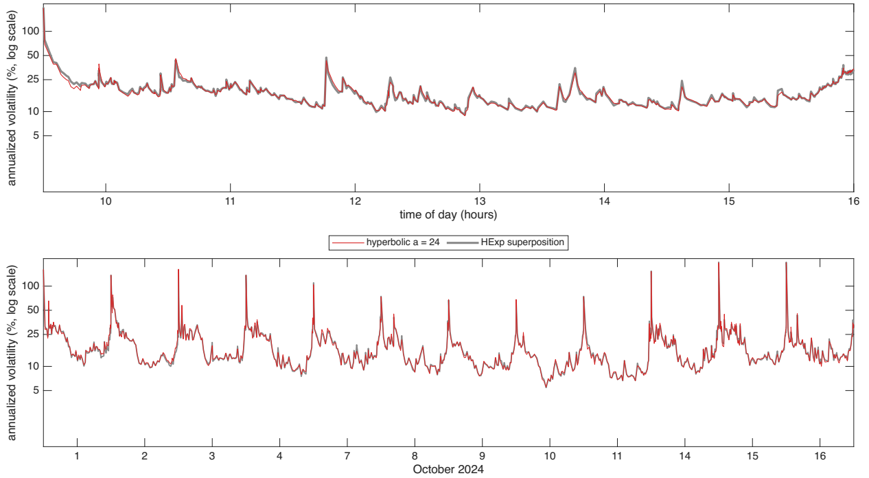
Figure 6: Hyperbolic against superposition weights for CROX over 12 trading days in Oct 2024, the diurnally adjusted \hat{\sigma}(u)100\sqrt{252} at s = 1 second from the Huber filter, shown as annualized vol in % on a log10 scale. The only difference between the 2 paths is the weight function: the hyperbolic weights with a = 24 in red, drawn on top, and the HExp superposition in grey, 4 exponential components with half lives of 2, 20, 200, 2000 seconds. Hyperparameters minimize the QLIKE objective. Top: 16 October 2024, bottom: 12 days.
