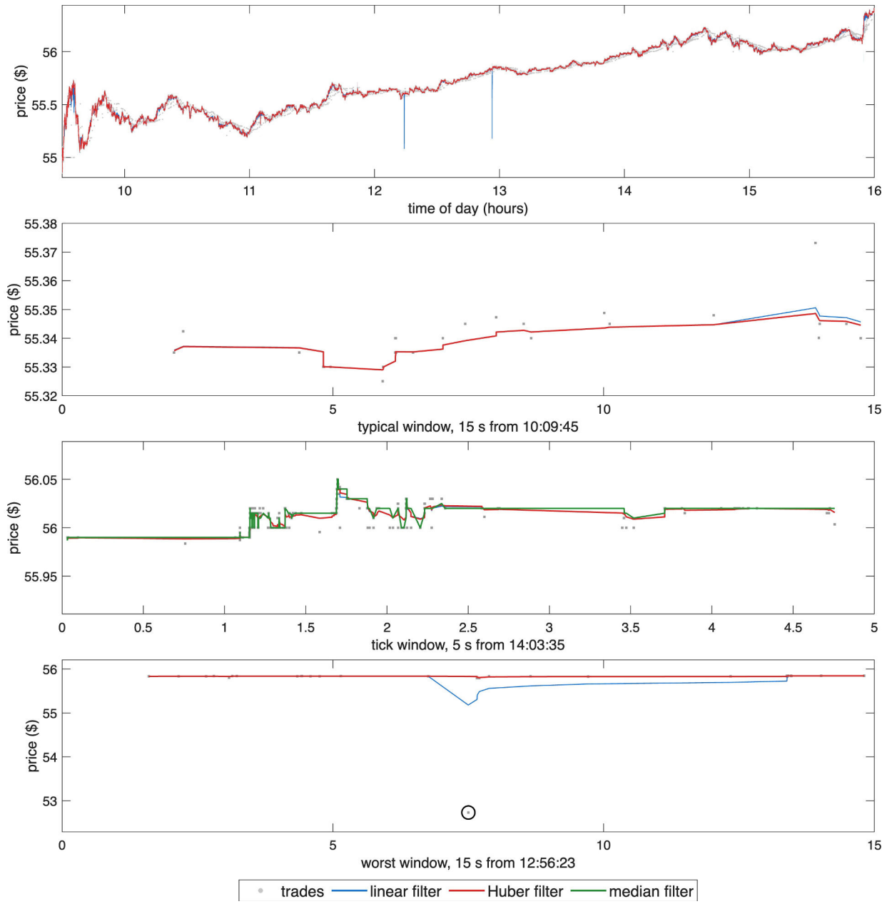
Figure 1: CSC0 trades (grey points), the linear filter and the Huber filter, 16 October 2024. Top: full trading day. 2nd: 15-second window at the day's median trade count, from 10:09:45. 3rd: 5-second window at 14:03:35 in which the price reverses direction most often, with the median filter m_t added. Bottom: 15-second window around the largest Huber residual after 09:45, circled.
