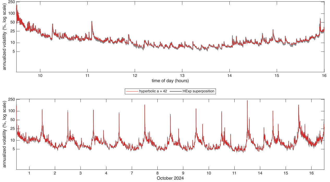
Figure 6: Hyperbolic against superposition weights for CSC0 over 12 trading days in Oct 2024, the diurnally adjusted \hat{\sigma}(u)100\sqrt{252} at s = 1 second from the Huber filter, shown as annualized vol in % on a log10 scale. The only difference between the 2 paths is the weight function: the hyperbolic weights with a = 42 in red, drawn on top, and the HExp superposition in grey, 4 exponential components with half lives of 10, 100, 1000, 10000 seconds. Hyperparameters minimize the QLIKE objective. Top: 16 October 2024, bottom: 12 days.
