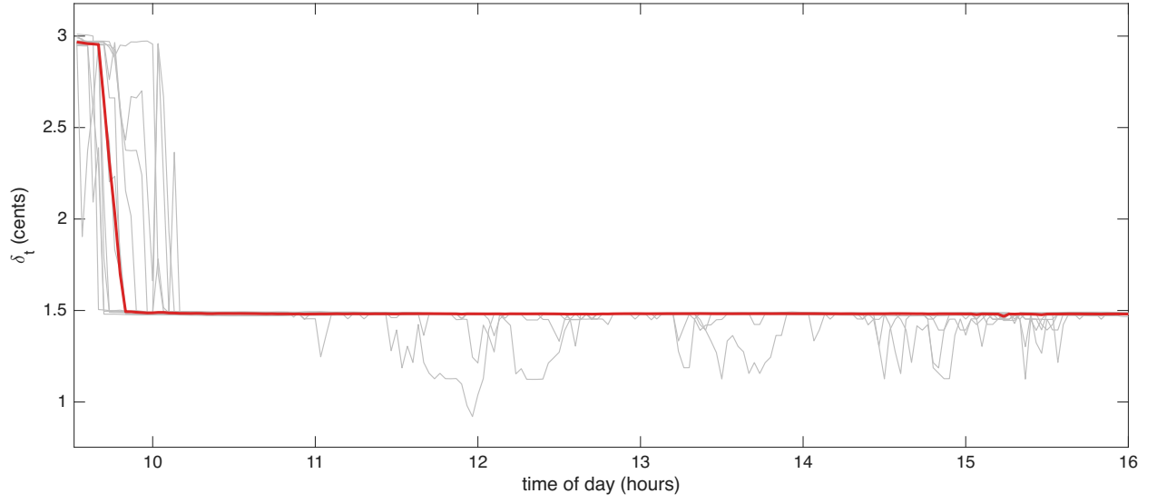
Figure 3: Huber threshold \delta_t in cents through the trading day, for 12 CSC0 trading days in Oct 2024 (grey lines) and their median (red line).
