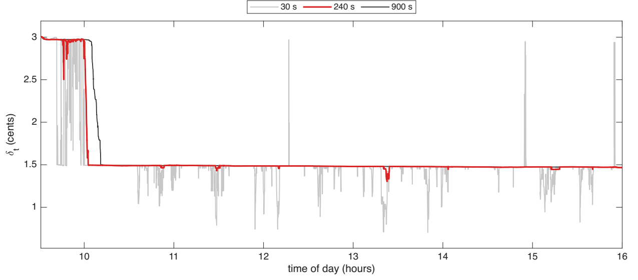
Figure 2: The Huber threshold \delta_t in cents for CSC0 on 16 October 2024, with half-lives of 30, 240, 900 seconds. The 240-second half-life, in red, is used.
