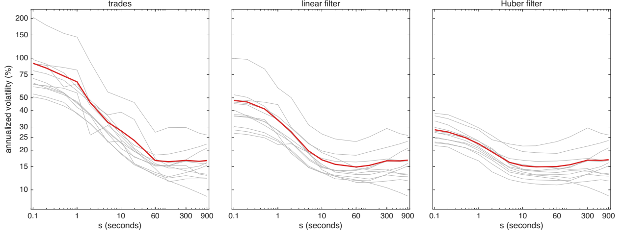
Figure 4: Volatility signature curves for CSC0 over the 12 trading days in Oct 2024. The annualized vol \hat{\sigma}100\sqrt{252} from the returns \hat{X}_t - \hat{X}_{t,s} of Table 2, against the lag s in seconds, both axes on log scales, for: raw trades, linear filter & Huber filter. Grey lines are the individual trading days & the red line is the square root of the 12 day average of their squares. The linear & Huber returns carry the finite-sample correction c_{t,s} of the paper; the raw trades are unaffected by it.
