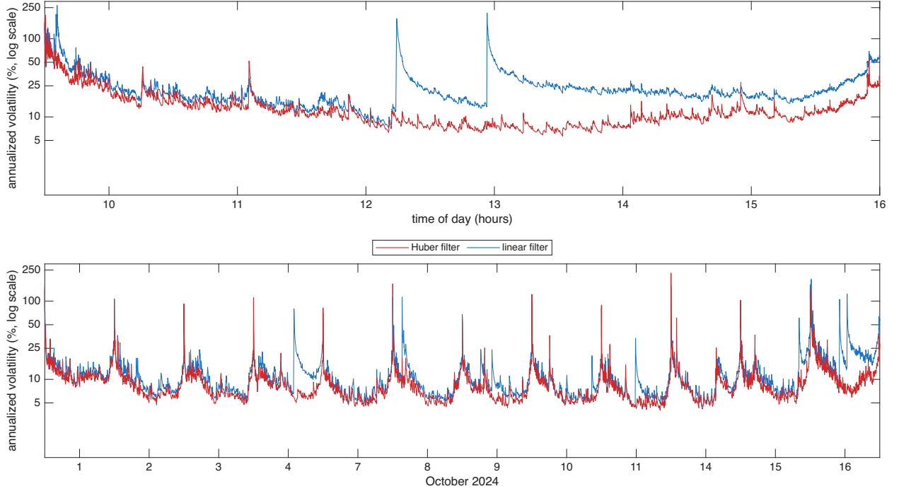
Figure 5: Filtered spot volatility for CSC0 over 12 trading days in Oct 2024, the diurnally adjusted estimator \hat{\sigma}(u)100\sqrt{252} at s = 1 second with hyperbolic weights, Mandelbrot parameter a = 42 , with the input prices computed using the Huber & linear filters, shown as annualized volatility in percent on a log10 scale. Top: 16 October 2024, bottom: 12 days.
