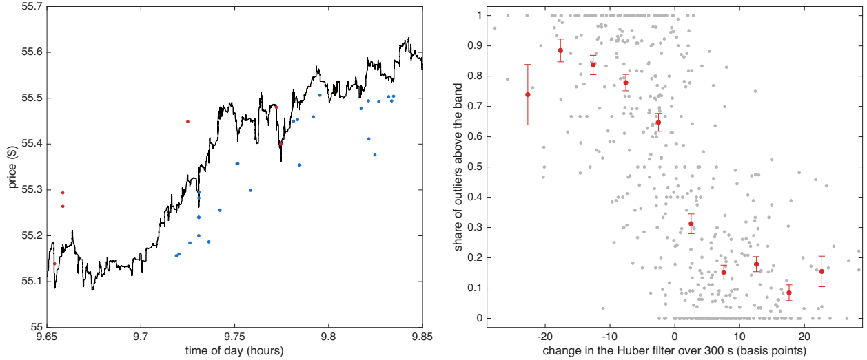
Figure 7: Outliers & robust price for CSC0 on 16 October 2024. Left: the 12 minutes with the largest move in the Huber filter that day; outliers above Y_t - \theta_t > \delta_{t-1} in red, outliers below Y_t - \theta_t < -\delta_{t-1} in blue, Huber filter in black. Right: over the 12 trading days, the 300 second empirical conditional probability that outliers are above (rather than below) the Huber band against the 300 second change in the Huber filter in basis points: light points are single bins, the line & bars are means & s.e.
