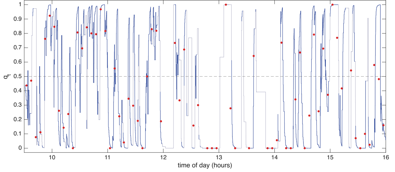
Figure 8: The directional conditional probability for CSC0 , 16 October 2024. The filtered conditional probability q_t that an outlier lies above the robust Huber band, under exponential weights decaying in clock time with half life of 34 seconds; where fewer than two outliers remain in the weights it is drawn in grey. The dashed line marks 0.5. The red points are the empirical conditional probability using the 300 second bins of the previous figure.
