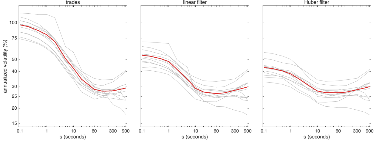
Figure 4: Volatility signature curves for DDOG over the 12 trading days in Oct 2024. The annualized vol \hat{\sigma}100\sqrt{252} from the returns \hat{X}_t - \hat{X}_{t,s} of Table 2, against the lag s in seconds, both axes on log scales, for: raw trades, linear filter & Huber filter. Grey lines are the individual trading days & the red line is the square root of the 12 day average of their squares. The linear & Huber returns carry the finite-sample correction c_{t,s} of the paper; the raw trades are unaffected by it.
