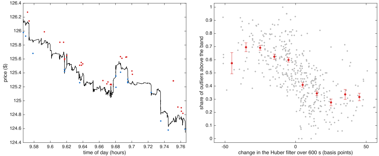
Figure 7: Outliers & robust price for DD0G on 16 October 2024. Left: the 12 minutes with the largest move in the Huber filter that day; outliers above Y_t - \theta_t > \delta_{t-1} in red, outliers below Y_t - \theta_t < -\delta_{t-1} in blue, Huber filter in black. Right: over the 12 trading days, the 600 second empirical conditional probability that outliers are above (rather than below) the Huber band against the 600 second change in the Huber filter in basis points: light points are single bins, the line & bars are means & s.e.
