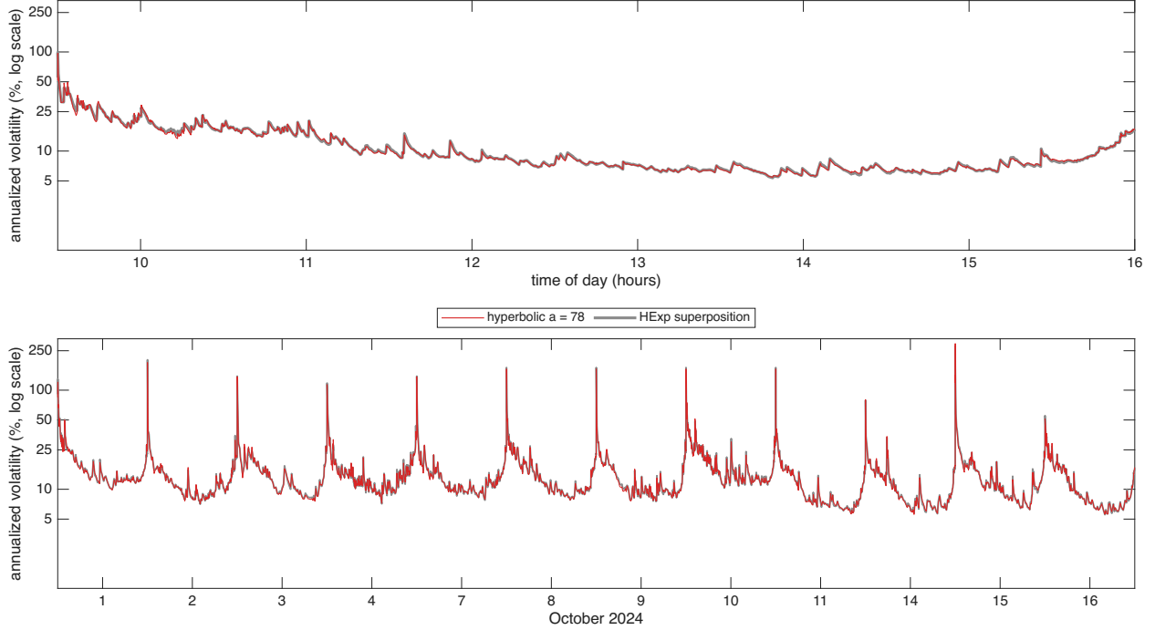
Figure 6: Hyperbolic against superposition weights for DD0G over 12 trading days in Oct 2024, the diurnally adjusted \hat{\sigma}(u)100\sqrt{252} at s = 1 second from the Huber filter, shown as annualized vol in % on a log10 scale. The only difference between the 2 paths is the weight function: the hyperbolic weights with a = 78 in red, drawn on top, and the HExp superposition in grey, 4 exponential components with half lives of 60, 600, 3600, 23400 seconds. Hyperparameters minimize the QLIKE objective. Top: 16 October 2024, bottom: 12 days.
