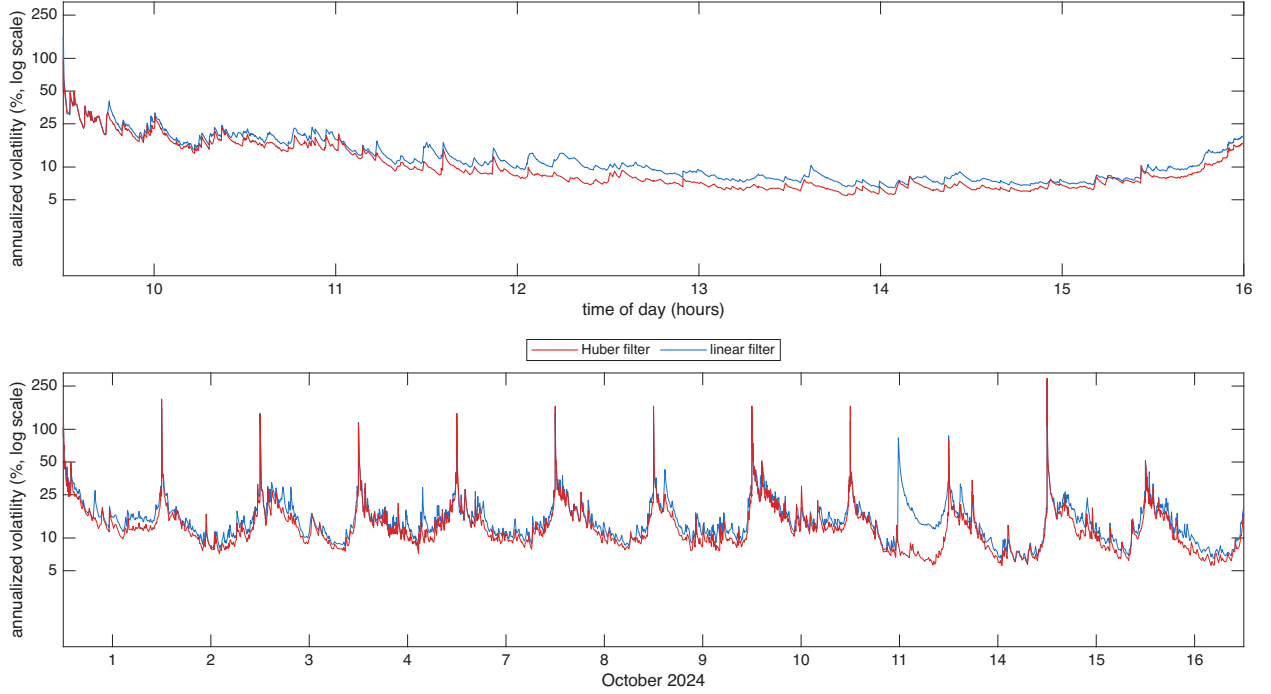
Figure 5: Filtered spot volatility for DDOG over 12 trading days in Oct 2024, the diurnally adjusted estimator \hat{\sigma}(u)100\sqrt{252} at s = 1 second with hyperbolic weights, Mandelbrot parameter a = 78 , with the input prices computed using the Huber & linear filters, shown as annualized volatility in percent on a log10 scale. Top: 16 October 2024, bottom: 12 days.
