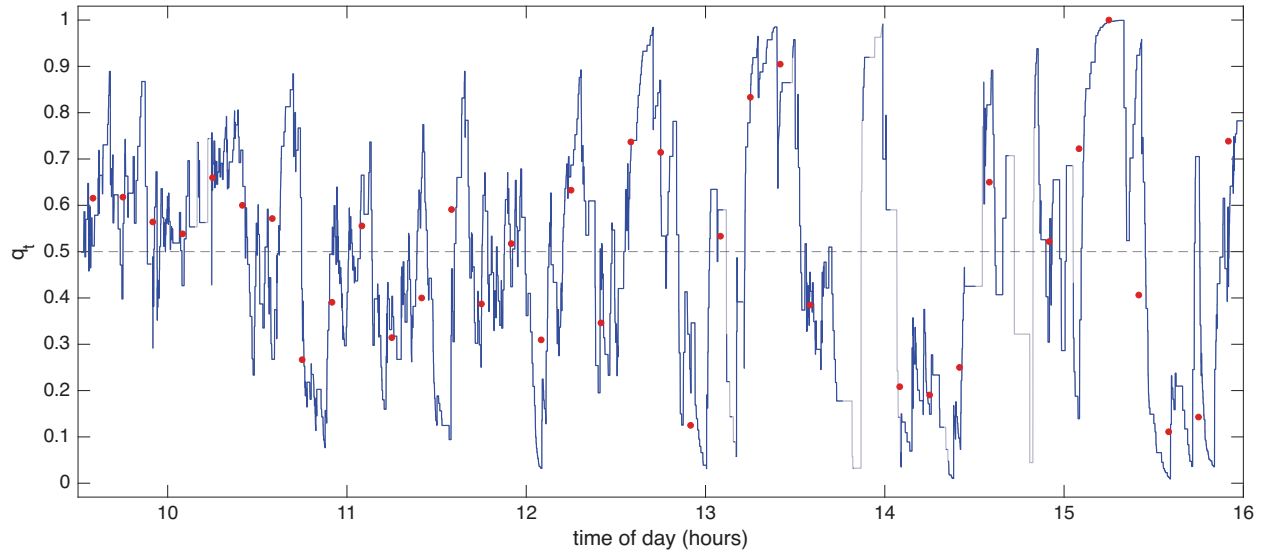
Figure 8: The directional conditional probability for DDOG, 16 October 2024. The filtered conditional probability q_t that an outlier lies above the robust Huber band, under exponential weights decaying in clock time with half life of 88 seconds; where fewer than two outliers remain in the weights it is drawn in grey. The dashed line marks 0.5. The red points are the empirical conditional probability using the 600 second bins of the previous figure.
