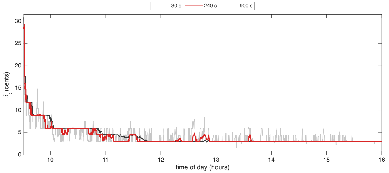
Figure 2: The Huber threshold \delta_t in cents for DDOG on 16 October 2024, with half-lives of 30, 240, 900 seconds. The 240-second half-life, in red, is used.
