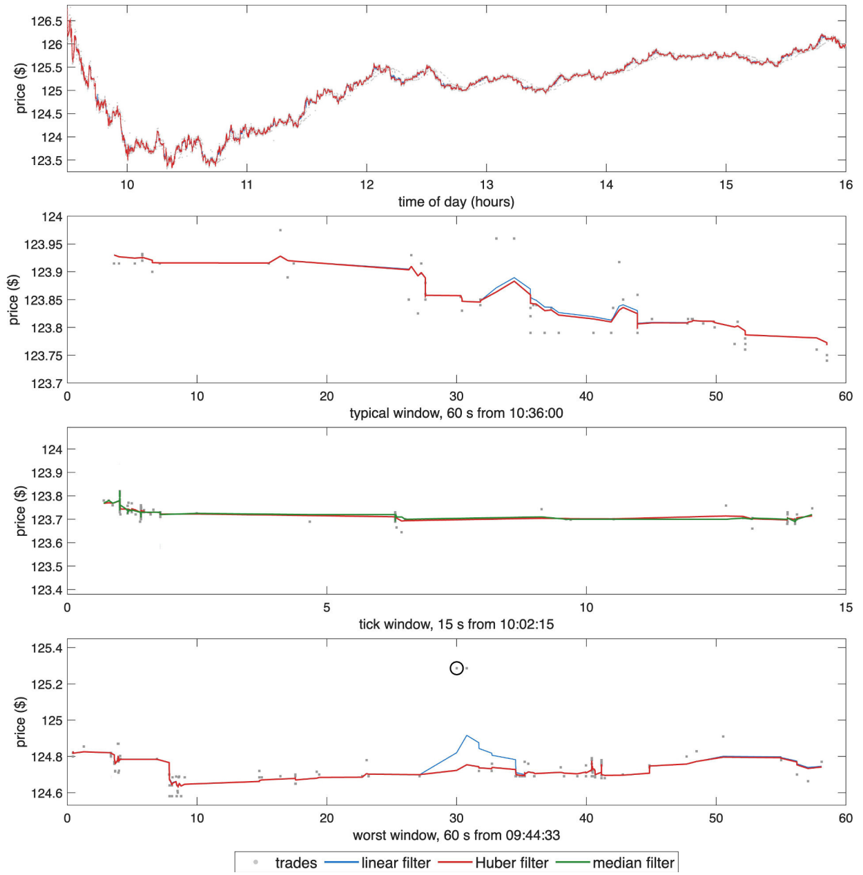
Figure 1: DDOG trades (grey points), the linear filter and the Huber filter, 16 October 2024. Top: full trading day. 2nd: 60-second window at the day's median trade count, from 10:36:00. 3rd: 15-second window at 10:02:15 in which the price reverses direction most often, with the median filter m_t added. Bottom: 60-second window around the largest Huber residual after 09:45, circled.
