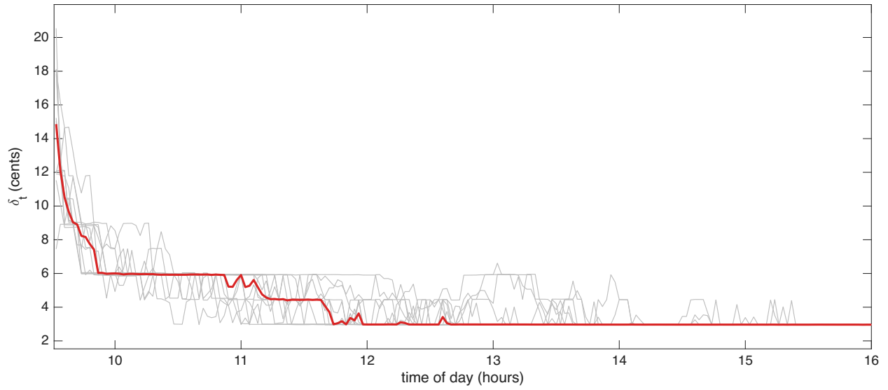
Figure 3: Huber threshold \delta_t in cents through the trading day, for 12 DDOG trading days in Oct 2024 (grey lines) and their median (red line).
