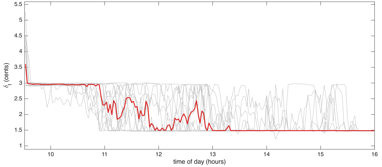
Figure 3: Huber threshold \delta_t in cents through the trading day, for 12 DKNG trading days in Oct 2024 (grey lines) and their median (red line).
