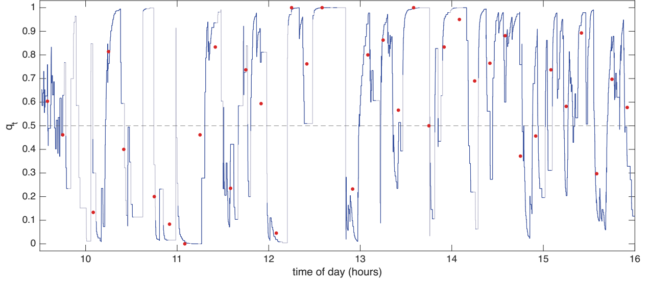
Figure 8: The directional conditional probability for DKNK, 16 October 2024. The filtered conditional probability q_t that an outlier lies above the robust Huber band, under exponential weights decaying in clock time with half life of 68 seconds; where fewer than two outliers remain in the weights it is drawn in grey. The dashed line marks 0.5. The red points are the empirical conditional probability using the 600 second bins of the previous figure.
