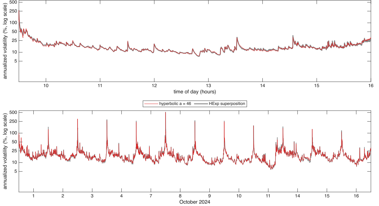
Figure 6: Hyperbolic against superposition weights for DKNV over 12 trading days in Oct 2024, the diurnally adjusted \hat{\sigma}(u)100\sqrt{252} at s = 1 second from the Huber filter, shown as annualized vol in % on a log10 scale. The only difference between the 2 paths is the weight function: the hyperbolic weights with a = 46 in red, drawn on top, and the HExp superposition in grey, 4 exponential components with half lives of 30, 150, 750, 3750 seconds. Hyperparameters minimize the QLIKE objective. Top: 16 October 2024, bottom: 12 days.
