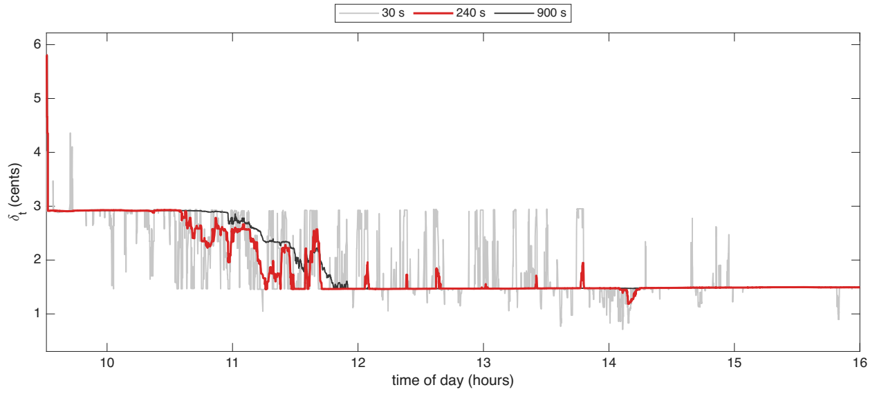
Figure 2: The Huber threshold \delta_t in cents for DKNG on 16 October 2024, with half-lives of 30, 240, 900 seconds. The 240-second half-life, in red, is used.
