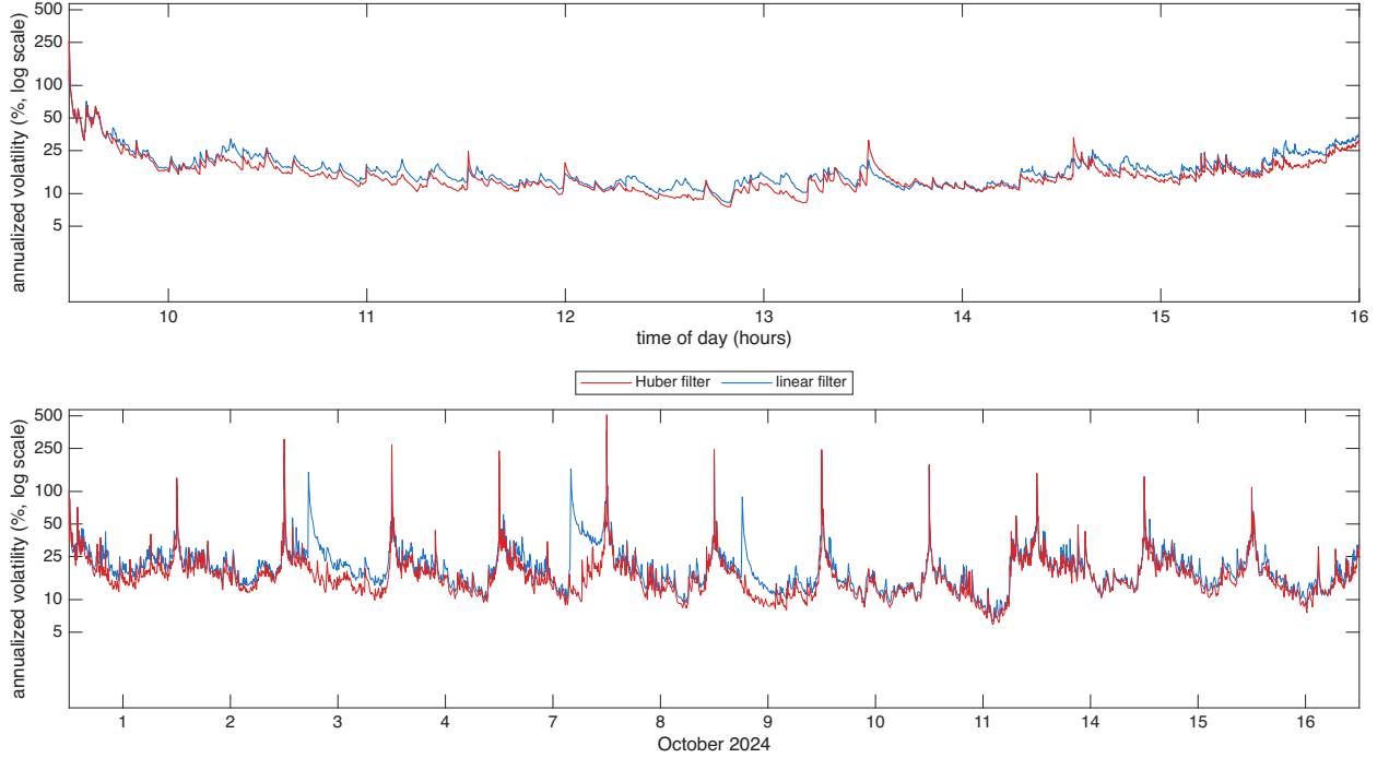
Figure 5: Filtered spot volatility for DKNK over 12 trading days in Oct 2024, the diurnally adjusted estimator \hat{\sigma}(u)100\sqrt{252} at s = 1 second with hyperbolic weights, Mandelbrot parameter a = 46 , with the input prices computed using the Huber & linear filters, shown as annualized volatility in percent on a log10 scale. Top: 16 October 2024, bottom: 12 days.
