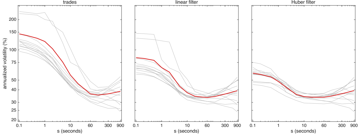
Figure 4: Volatility signature curves for DKNK over the 12 trading days in Oct 2024. The annualized vol \hat{\sigma}100\sqrt{252} from the returns \hat{X}_t - \hat{X}_{t,s} of Table 2, against the lag s in seconds, both axes on log scales, for: raw trades, linear filter & Huber filter. Grey lines are the individual trading days & the red line is the square root of the 12 day average of their squares. The linear & Huber returns carry the finite-sample correction c_{t,s} of the paper; the raw trades are unaffected by it.
