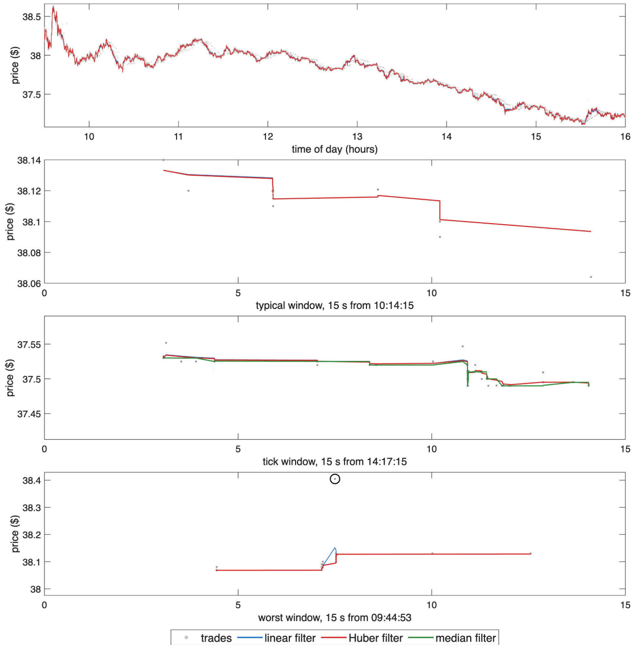
Figure 1: DKNG trades (grey points), the linear filter and the Huber filter, 16 October 2024. Top: full trading day. 2nd: 15-second window at the day's median trade count, from 10:14:15. 3rd: 15-second window at 14:17:15 in which the price reverses direction most often, with the median filter m_t added. Bottom: 15-second window around the largest Huber residual after 09:45, circled.
