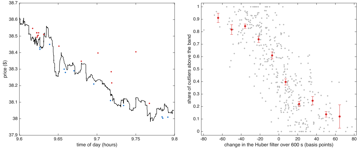
Figure 7: Outliers & robust price for DKNV on 16 October 2024. Left: the 12 minutes with the largest move in the Huber filter that day; outliers above Y_t - \theta_t > \delta_{t-1} in red, outliers below Y_t - \theta_t < -\delta_{t-1} in blue, Huber filter in black. Right: over the 12 trading days, the 600 second empirical conditional probability that outliers are above (rather than below) the Huber band against the 600 second change in the Huber filter in basis points: light points are single bins, the line & bars are means & s.e.
