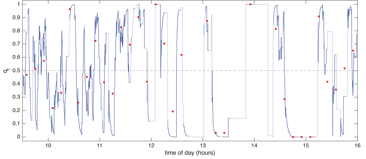
Figure 8: The directional conditional probability for ETSY, 16 October 2024. The filtered conditional probability q_t that an outlier lies above the robust Huber band, under exponential weights decaying in clock time with half life of 62 seconds; where fewer than two outliers remain in the weights it is drawn in grey. The dashed line marks 0.5. The red points are the empirical conditional probability using the 600 second bins of the previous figure.
