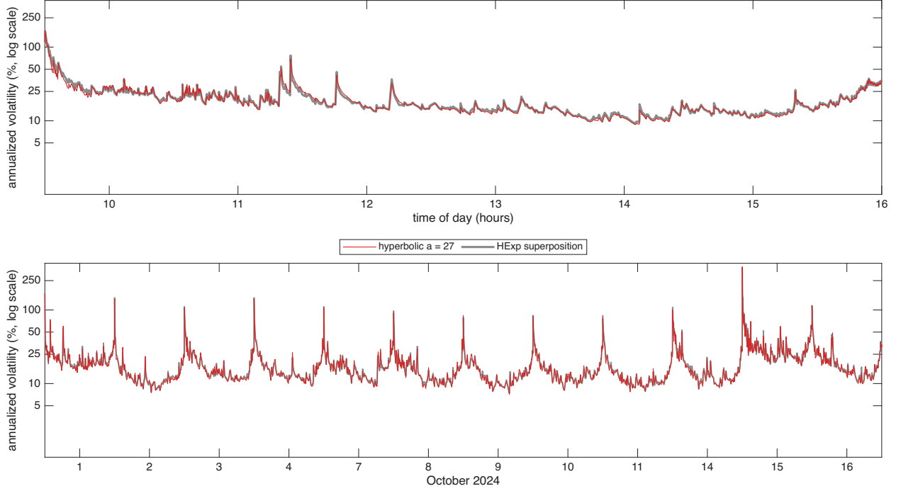
Figure 6: Hyperbolic against superposition weights for ETSY over 12 trading days in Oct 2024, the diurnally adjusted \hat{\sigma}(u)100\sqrt{252} at s = 1 second from the Huber filter, shown as annualized vol in % on a log10 scale. The only difference between the 2 paths is the weight function: the hyperbolic weights with a = 27 in red, drawn on top, and the HExp superposition in grey, 4 exponential components with half lives of 10, 100, 1000, 10000 seconds. Hyperparameters minimize the QLIKE objective. Top: 16 October 2024, bottom: 12 days.
