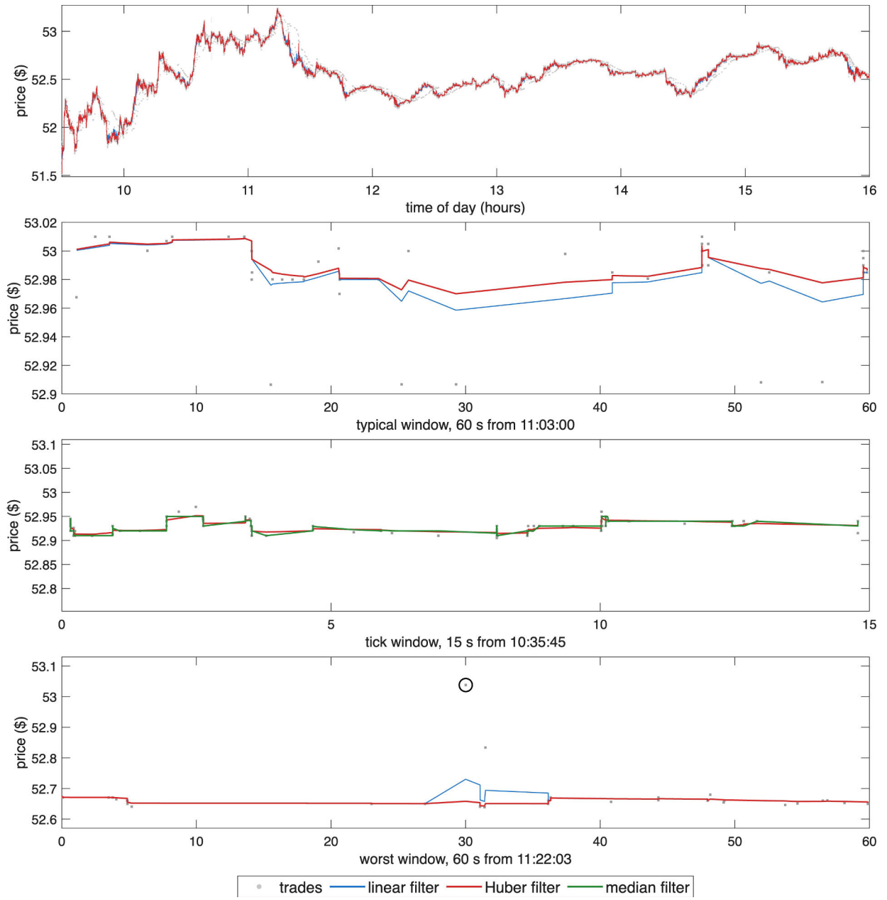
Figure 1: ETSY trades (grey points), the linear filter and the Huber filter, 16 October 2024. Top: full trading day. 2nd: 60-second window at the day's median trade count, from 11:03:00. 3rd: 15-second window at 10:35:45 in which the price reverses direction most often, with the median filter m_t added. Bottom: 60-second window around the largest Huber residual after 09:45, circled.
