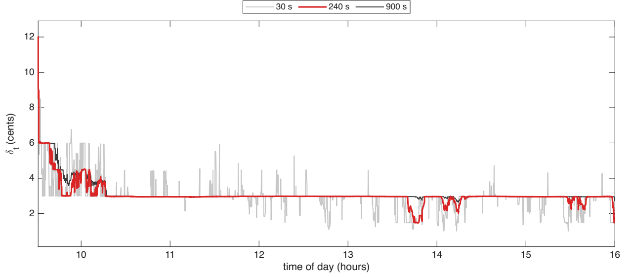
Figure 2: The Huber threshold \delta_t in cents for ETSY on 16 October 2024, with half-lives of 30, 240, 900 seconds. The 240-second half-life, in red, is used.
