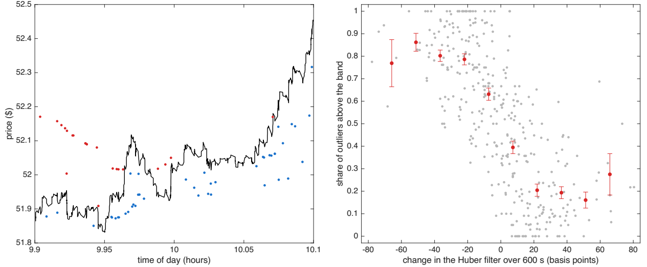
Figure 7: Outliers & robust price for ETSY on 16 October 2024. Left: the 12 minutes with the largest move in the Huber filter that day; outliers above Y_t - \theta_t > \delta_{t-1} in red, outliers below Y_t - \theta_t < -\delta_{t-1} in blue, Huber filter in black. Right: over the 12 trading days, the 600 second empirical conditional probability that outliers are above (rather than below) the Huber band against the 600 second change in the Huber filter in basis points: light points are single bins, the line & bars are means & s.e.
