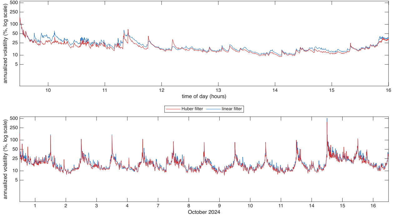
Figure 5: Filtered spot volatility for ETSY over 12 trading days in Oct 2024, the diurnally adjusted estimator \hat{\sigma}(u)100\sqrt{252} at s = 1 second with hyperbolic weights, Mandelbrot parameter a = 27 , with the input prices computed using the Huber & linear filters, shown as annualized volatility in percent on a log10 scale. Top: 16 October 2024, bottom: 12 days.
