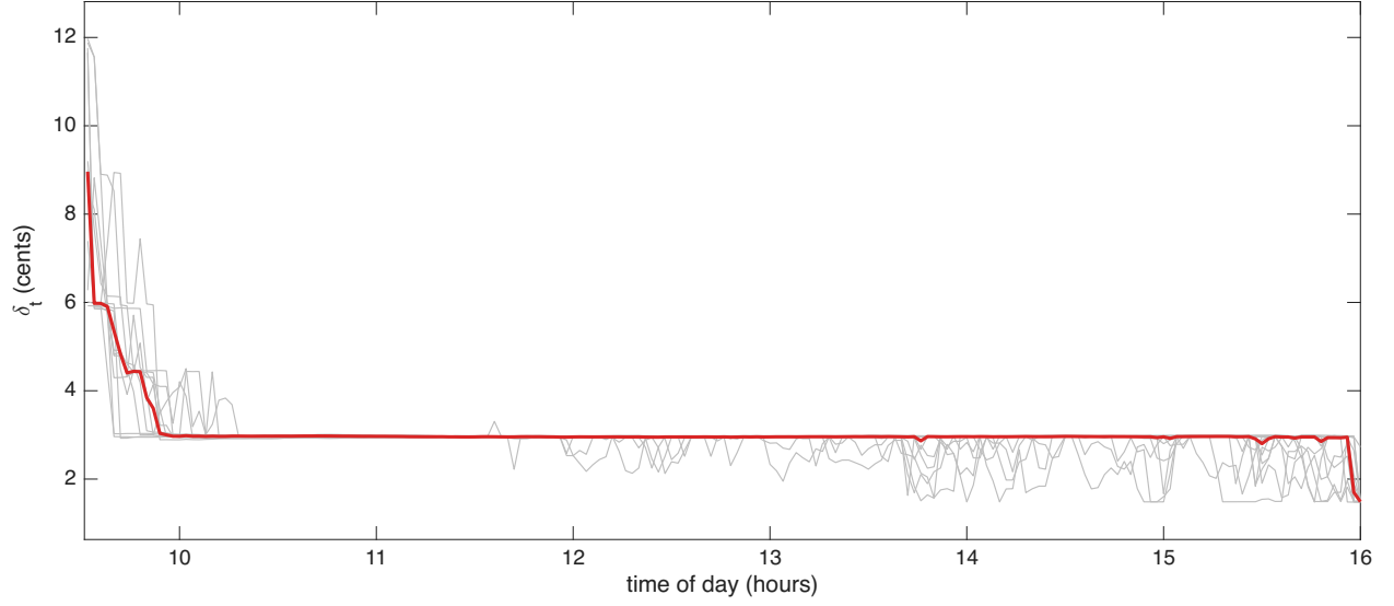
Figure 3: Huber threshold \delta_t in cents through the trading day, for 12 ETSY trading days in Oct 2024 (grey lines) and their median (red line).
