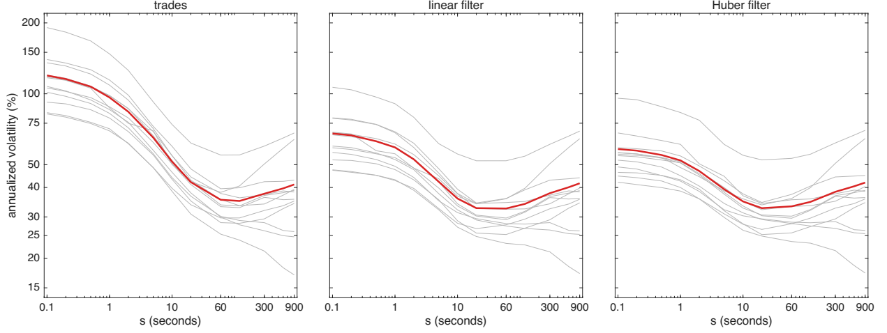
Figure 4: Volatility signature curves for ETSY over the 12 trading days in Oct 2024. The annualized vol \hat{\sigma}100\sqrt{252} from the returns \hat{X}_t - \hat{X}_{t,s} of Table 2, against the lag s in seconds, both axes on log scales, for: raw trades, linear filter & Huber filter. Grey lines are the individual trading days & the red line is the square root of the 12 day average of their squares. The linear & Huber returns carry the finite-sample correction c_{t,s} of the paper; the raw trades are unaffected by it.
