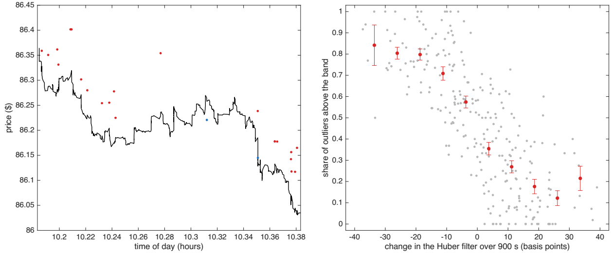
Figure 7: Outliers & robust price for GILD on 16 October 2024. Left: the 12 minutes with the largest move in the Huber filter that day; outliers above Y_t - \theta_t > \delta_{t-1} in red, outliers below Y_t - \theta_t < -\delta_{t-1} in blue, Huber filter in black. Right: over the 12 trading days, the 900 second empirical conditional probability that outliers are above (rather than below) the Huber band against the 900 second change in the Huber filter in basis points: light points are single bins, the line & bars are means & s.e.
