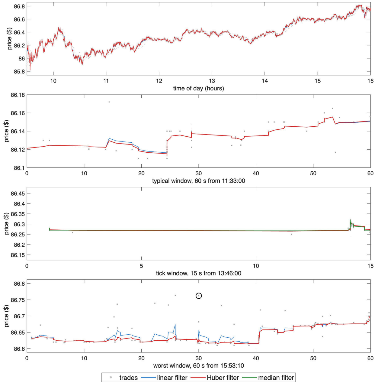
Figure 1: GILD trades (grey points), the linear filter and the Huber filter, 16 October 2024. Top: full trading day. 2nd: 60-second window at the day's median trade count, from 11:33:00. 3rd: 15-second window at 13:46:00 in which the price reverses direction most often, with the median filter m_t added. Bottom: 60-second window around the largest Huber residual after 09:45, circled.
