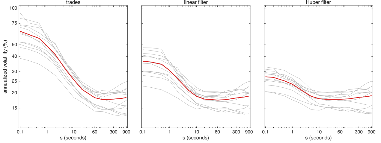
Figure 4: Volatility signature curves for GILD over the 12 trading days in Oct 2024. The annualized vol \hat{\sigma}100\sqrt{252} from the returns \hat{X}_t - \hat{X}_{t,s} of Table 2, against the lag s in seconds, both axes on log scales, for: raw trades, linear filter & Huber filter. Grey lines are the individual trading days & the red line is the square root of the 12 day average of their squares. The linear & Huber returns carry the finite-sample correction c_{t,s} of the paper; the raw trades are unaffected by it.
