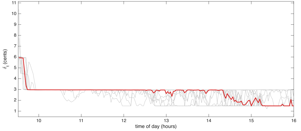
Figure 3: Huber threshold \delta_t in cents through the trading day, for 12 GILD trading days in Oct 2024 (grey lines) and their median (red line).
