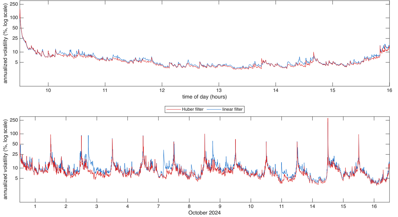
Figure 5: Filtered spot volatility for GILD over 12 trading days in Oct 2024, the diurnally adjusted estimator \hat{\sigma}(u)100\sqrt{252} at s = 1 second with hyperbolic weights, Mandelbrot parameter a = 25 , with the input prices computed using the Huber & linear filters, shown as annualized volatility in percent on a log10 scale. Top: 16 October 2024, bottom: 12 days.
