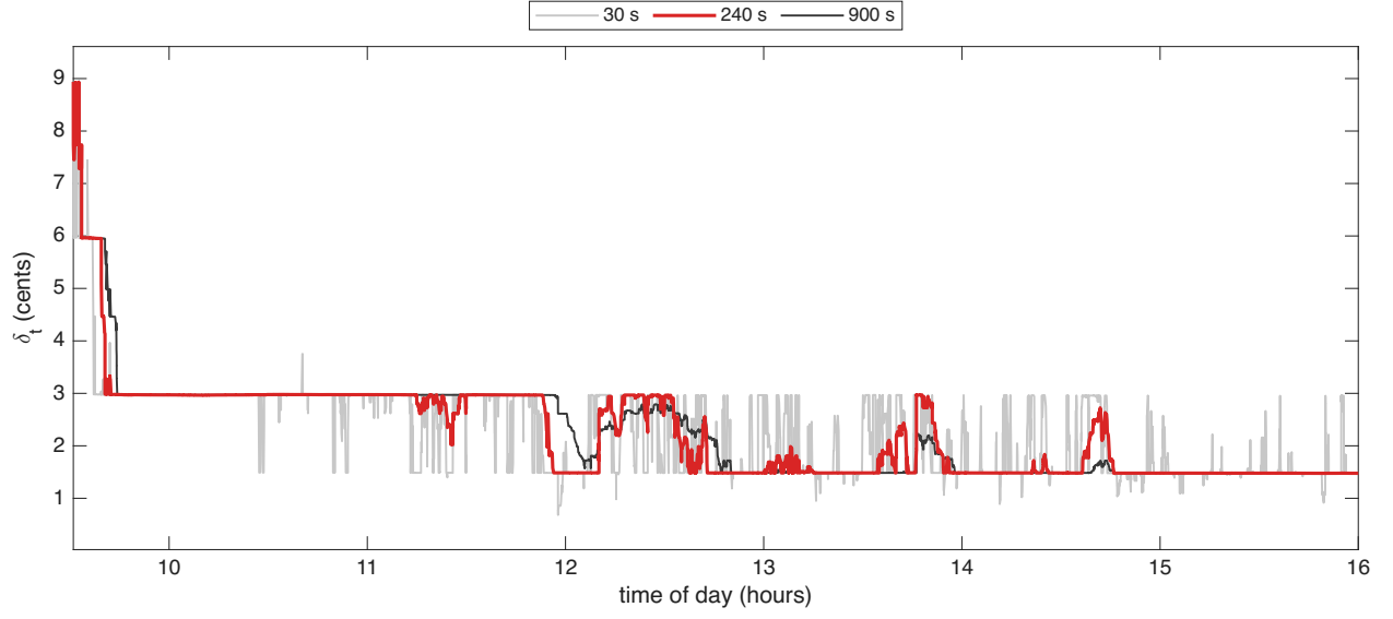
Figure 2: The Huber threshold \delta_t in cents for GILD on 16 October 2024, with half-lives of 30, 240, 900 seconds. The 240-second half-life, in red, is used.
