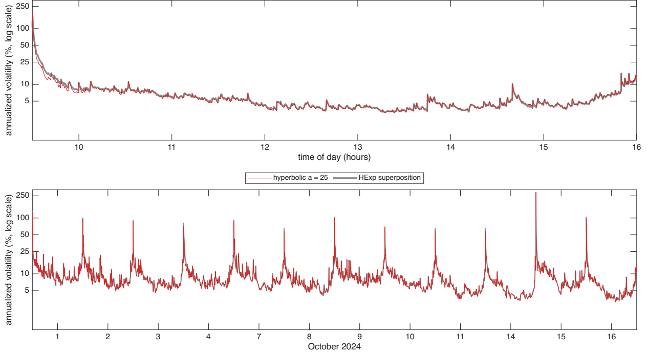
Figure 6: Hyperbolic against superposition weights for GILD over 12 trading days in Oct 2024, the diurnally adjusted \hat{\sigma}(u)100\sqrt{252} at s = 1 second from the Huber filter, shown as annualized vol in % on a log10 scale. The only difference between the 2 paths is the weight function: the hyperbolic weights with a = 25 in red, drawn on top, and the HExp superposition in grey, 4 exponential components with half lives of 10, 100, 1000, 10000 seconds. Hyperparameters minimize the QLIKE objective. Top: 16 October 2024, bottom: 12 days.
