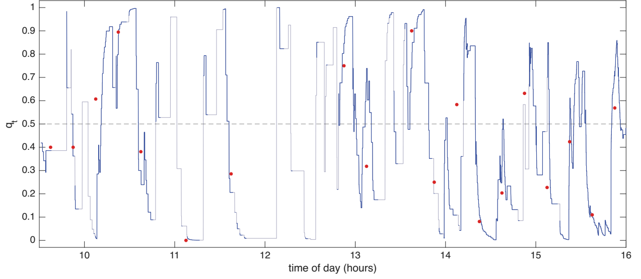
Figure 8: The directional conditional probability for GILD, 16 October 2024. The filtered conditional probability q_t that an outlier lies above the robust Huber band, under exponential weights decaying in clock time with half life of 116 seconds; where fewer than two outliers remain in the weights it is drawn in grey. The dashed line marks 0.5. The red points are the empirical conditional probability using the 900 second bins of the previous figure.
