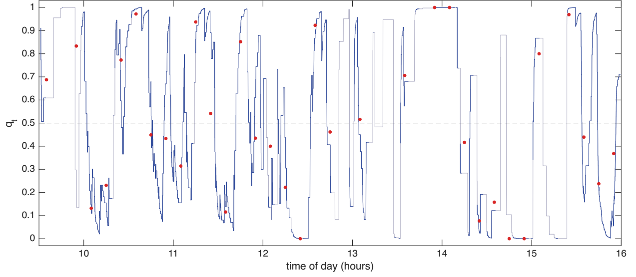
Figure 8: The directional conditional probability for H00D, 16 October 2024. The filtered conditional probability q_t that an outlier lies above the robust Huber band, under exponential weights decaying in clock time with half life of 76 seconds; where fewer than two outliers remain in the weights it is drawn in grey. The dashed line marks 0.5. The red points are the empirical conditional probability using the 600 second bins of the previous figure.
