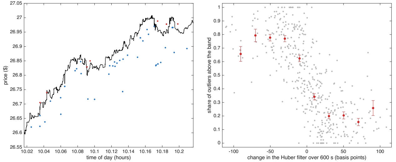
Figure 7: Outliers & robust price for H00D on 16 October 2024. Left: the 12 minutes with the largest move in the Huber filter that day; outliers above Y_t - \theta_t > \delta_{t-1} in red, outliers below Y_t - \theta_t < -\delta_{t-1} in blue, Huber filter in black. Right: over the 12 trading days, the 600 second empirical conditional probability that outliers are above (rather than below) the Huber band against the 600 second change in the Huber filter in basis points: light points are single bins, the line & bars are means & s.e.
