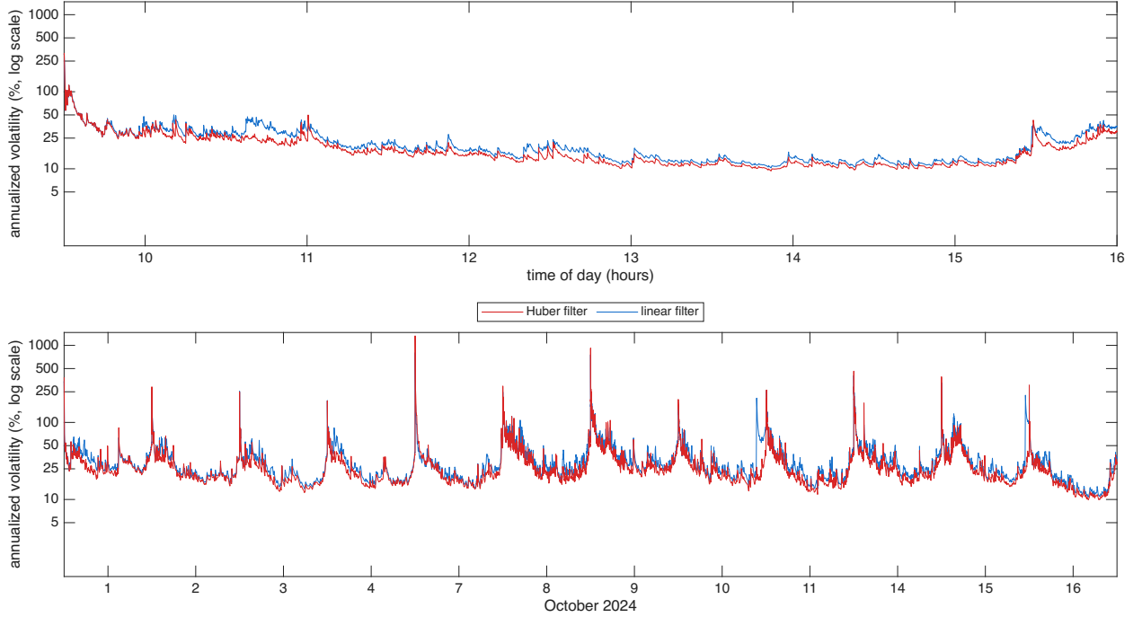
Figure 5: Filtered spot volatility for HOOD over 12 trading days in Oct 2024, the diurnally adjusted estimator \hat{\sigma}(u)100\sqrt{252} at s = 1 second with hyperbolic weights, Mandelbrot parameter a = 54 , with the input prices computed using the Huber & linear filters, shown as annualized volatility in percent on a log10 scale. Top: 16 October 2024, bottom: 12 days.
