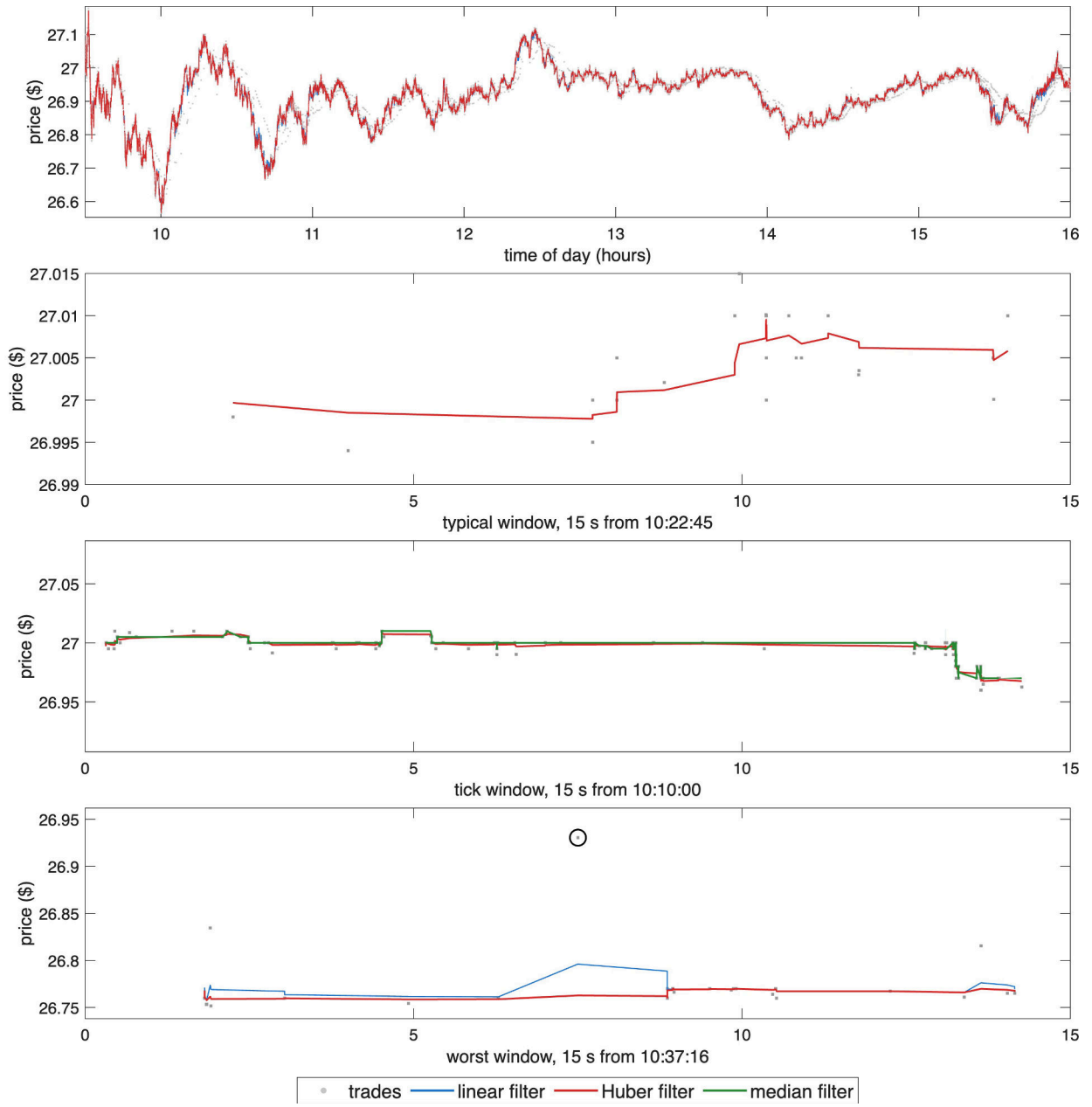
Figure 1: HOOD trades (grey points), the linear filter and the Huber filter, 16 October 2024. Top: full trading day. 2nd: 15-second window at the day's median trade count, from 10:22:45. 3rd: 15-second window at 10:10:00 in which the price reverses direction most often, with the median filter m_t added. Bottom: 15-second window around the largest Huber residual after 09:45, circled.
