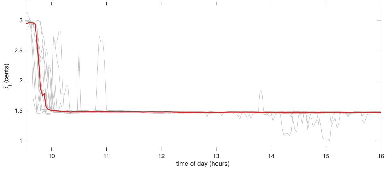
Figure 3: Huber threshold \delta_t in cents through the trading day, for 12 HOOD trading days in Oct 2024 (grey lines) and their median (red line).
