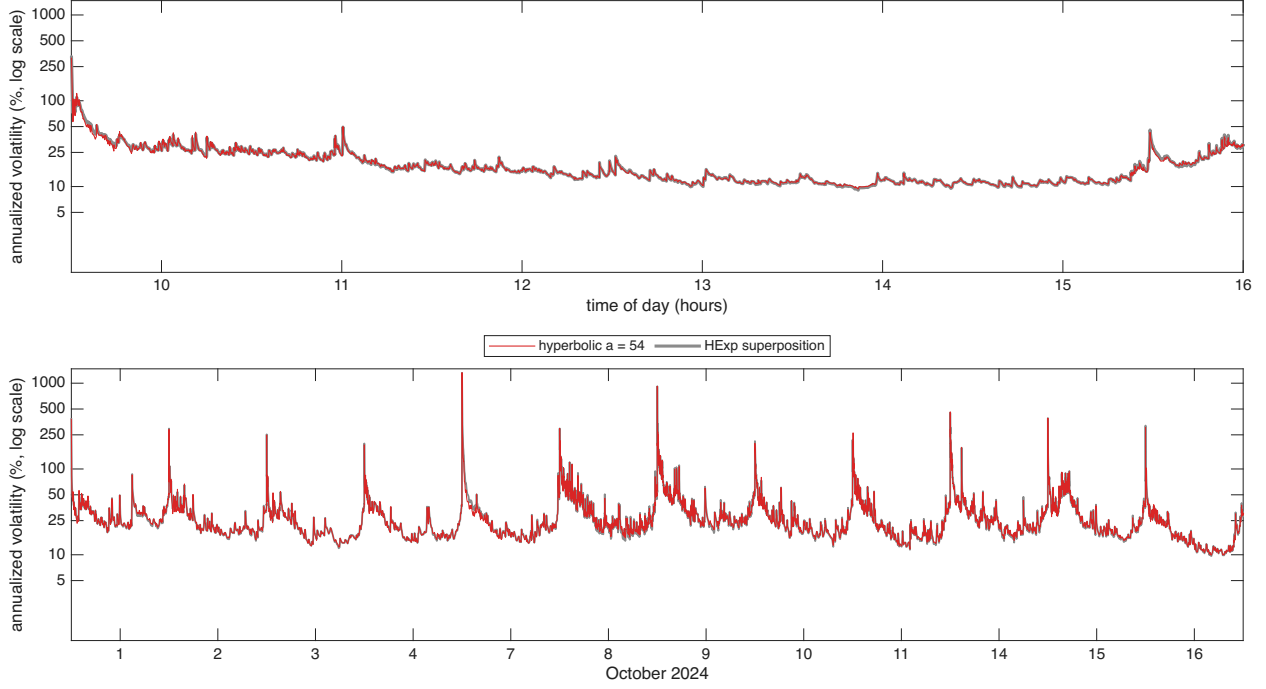
Figure 6: Hyperbolic against superposition weights for H00D over 12 trading days in Oct 2024, the diurnally adjusted \hat{\sigma}(u)100\sqrt{252} at s = 1 second from the Huber filter, shown as annualized vol in % on a log10 scale. The only difference between the 2 paths is the weight function: the hyperbolic weights with a = 54 in red, drawn on top, and the HExp superposition in grey, 4 exponential components with half lives of 10, 100, 1000, 10000 seconds. Hyperparameters minimize the QLIKE objective. Top: 16 October 2024, bottom: 12 days.
