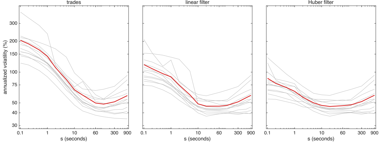
Figure 4: Volatility signature curves for HOOD over the 12 trading days in Oct 2024. The annualized vol \hat{\sigma}100\sqrt{252} from the returns \hat{X}_t - \hat{X}_{t,s} of Table 2, against the lag s in seconds, both axes on log scales, for: raw trades, linear filter & Huber filter. Grey lines are the individual trading days & the red line is the square root of the 12 day average of their squares. The linear & Huber returns carry the finite-sample correction c_{t,s} of the paper; the raw trades are unaffected by it.
