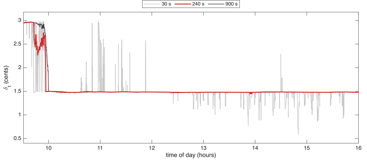
Figure 2: The Huber threshold \delta_t in cents for HOOD on 16 October 2024, with half-lives of 30, 240, 900 seconds. The 240-second half-life, in red, is used.
