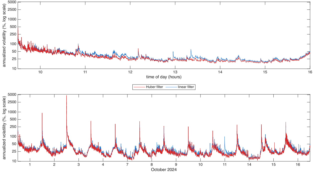
Figure 5: Filtered spot volatility for INTC over 12 trading days in Oct 2024, the diurnally adjusted estimator \hat{\sigma}(u)100\sqrt{252} at s = 1 second with hyperbolic weights, Mandelbrot parameter a = 59 , with the input prices computed using the Huber & linear filters, shown as annualized volatility in percent on a log10 scale. Top: 16 October 2024, bottom: 12 days.
