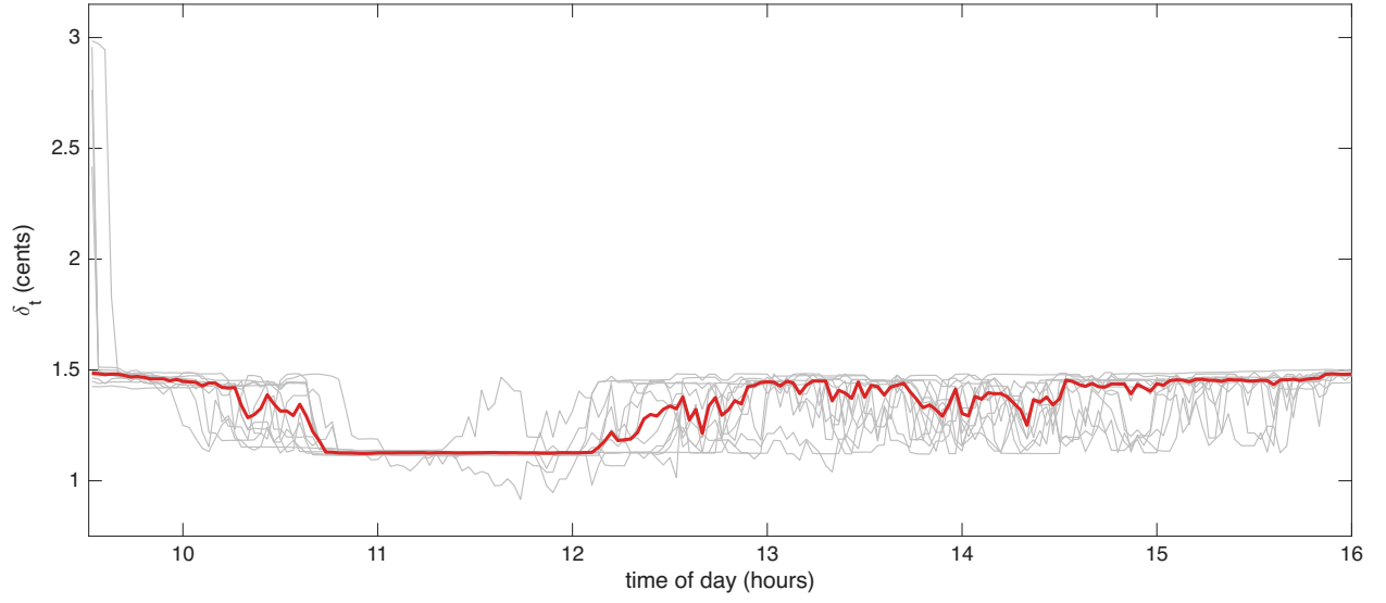
Figure 3: Huber threshold \delta_t in cents through the trading day, for 12 INTC trading days in Oct 2024 (grey lines) and their median (red line).
