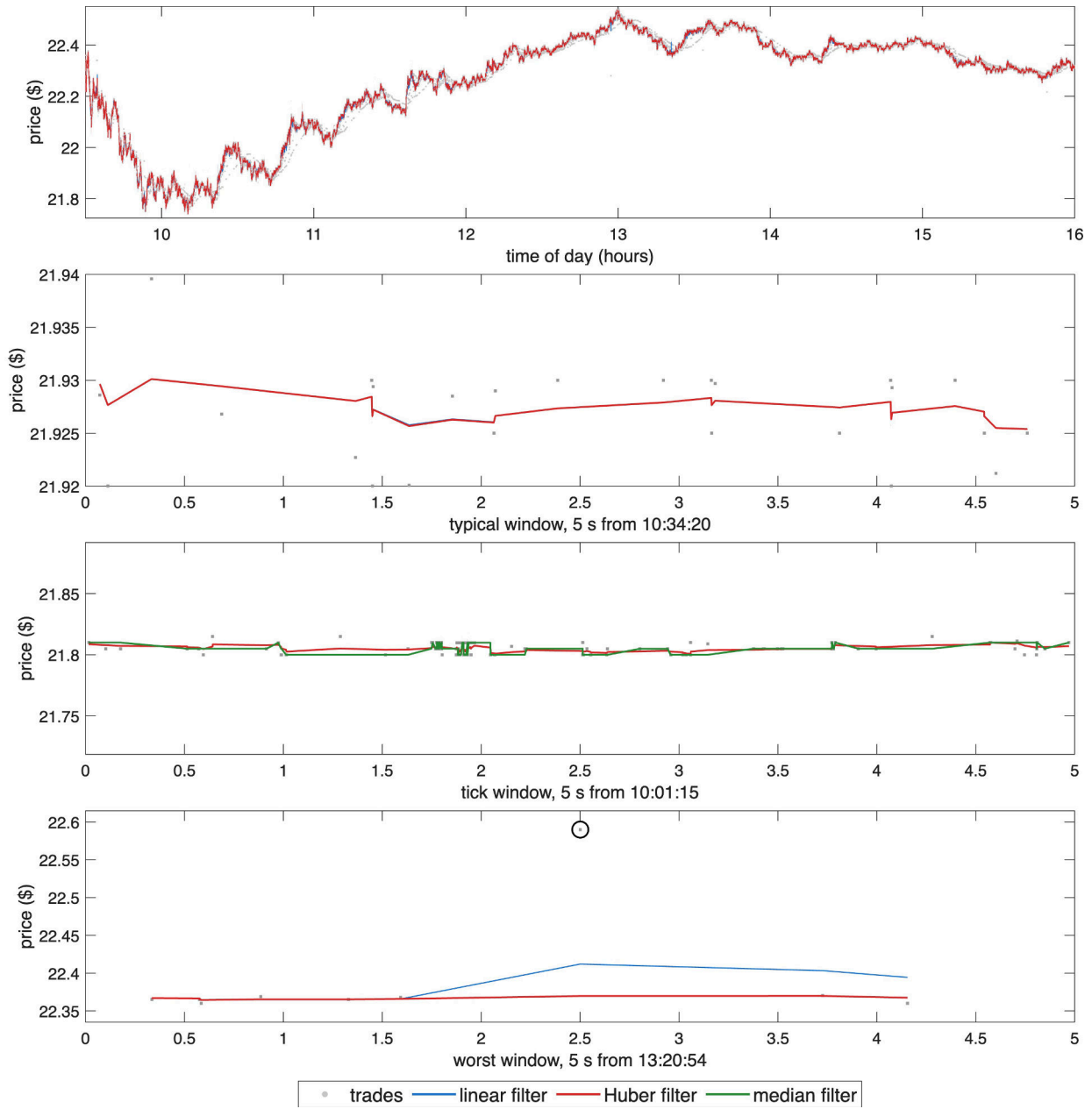
Figure 1: INTC trades (grey points), the linear filter and the Huber filter, 16 October 2024. Top: full trading day. 2nd: 5-second window at the day's median trade count, from 10:34:20. 3rd: 5-second window at 10:01:15 in which the price reverses direction most often, with the median filter m_t added. Bottom: 5-second window around the largest Huber residual after 09:45, circled.
