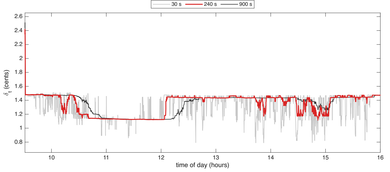
Figure 2: The Huber threshold \delta_t in cents for INTC on 16 October 2024, with half-lives of 30, 240, 900 seconds. The 240-second half-life, in red, is used.
