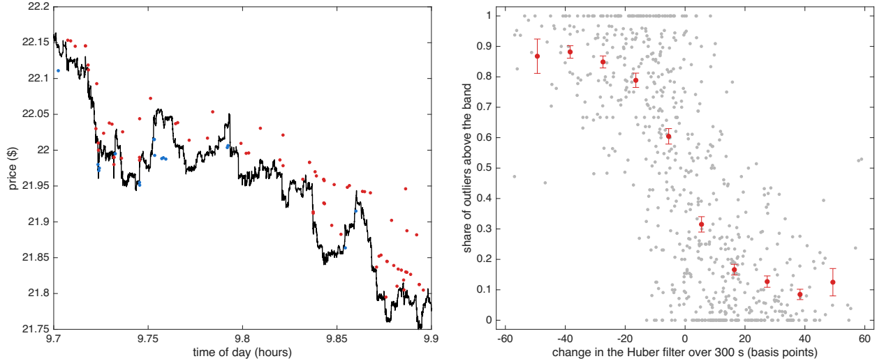
Figure 7: Outliers & robust price for INTC on 16 October 2024. Left: the 12 minutes with the largest move in the Huber filter that day; outliers above Y_t - \theta_t > \delta_{t-1} in red, outliers below Y_t - \theta_t < -\delta_{t-1} in blue, Huber filter in black. Right: over the 12 trading days, the 300 second empirical conditional probability that outliers are above (rather than below) the Huber band against the 300 second change in the Huber filter in basis points: light points are single bins, the line & bars are means & s.e.
