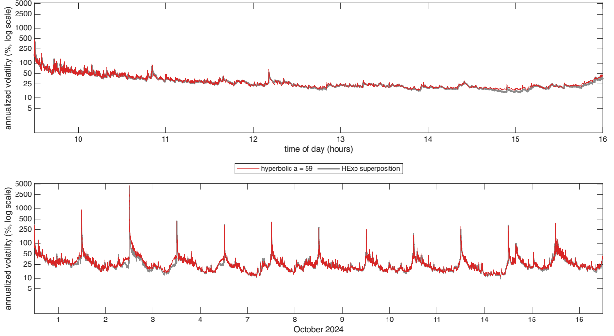
Figure 6: Hyperbolic against superposition weights for INTC over 12 trading days in Oct 2024, the diurnally adjusted \hat{\sigma}(u)100\sqrt{252} at s = 1 second from the Huber filter, shown as annualized vol in % on a log10 scale. The only difference between the 2 paths is the weight function: the hyperbolic weights with a = 59 in red, drawn on top, and the HExp superposition in grey, 4 exponential components with half lives of 2, 20, 200, 2000 seconds. Hyperparameters minimize the QLIKE objective. Top: 16 October 2024, bottom: 12 days.
