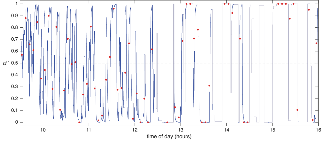
Figure 8: The directional conditional probability for INTG, 16 October 2024. The filtered conditional probability q_t that an outlier lies above the robust Huber band, under exponential weights decaying in clock time with half life of 34 seconds; where fewer than two outliers remain in the weights it is drawn in grey. The dashed line marks 0.5. The red points are the empirical conditional probability using the 300 second bins of the previous figure.
