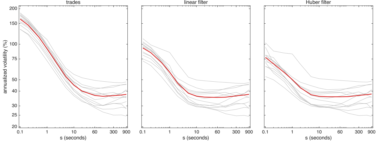
Figure 4: Volatility signature curves for INTC over the 12 trading days in Oct 2024. The annualized vol \hat{\sigma}100\sqrt{252} from the returns \hat{X}_t - \hat{X}_{t,s} of Table 2, against the lag s in seconds, both axes on log scales, for: raw trades, linear filter & Huber filter. Grey lines are the individual trading days & the red line is the square root of the 12 day average of their squares. The linear & Huber returns carry the finite-sample correction c_{t,s} of the paper; the raw trades are unaffected by it.
