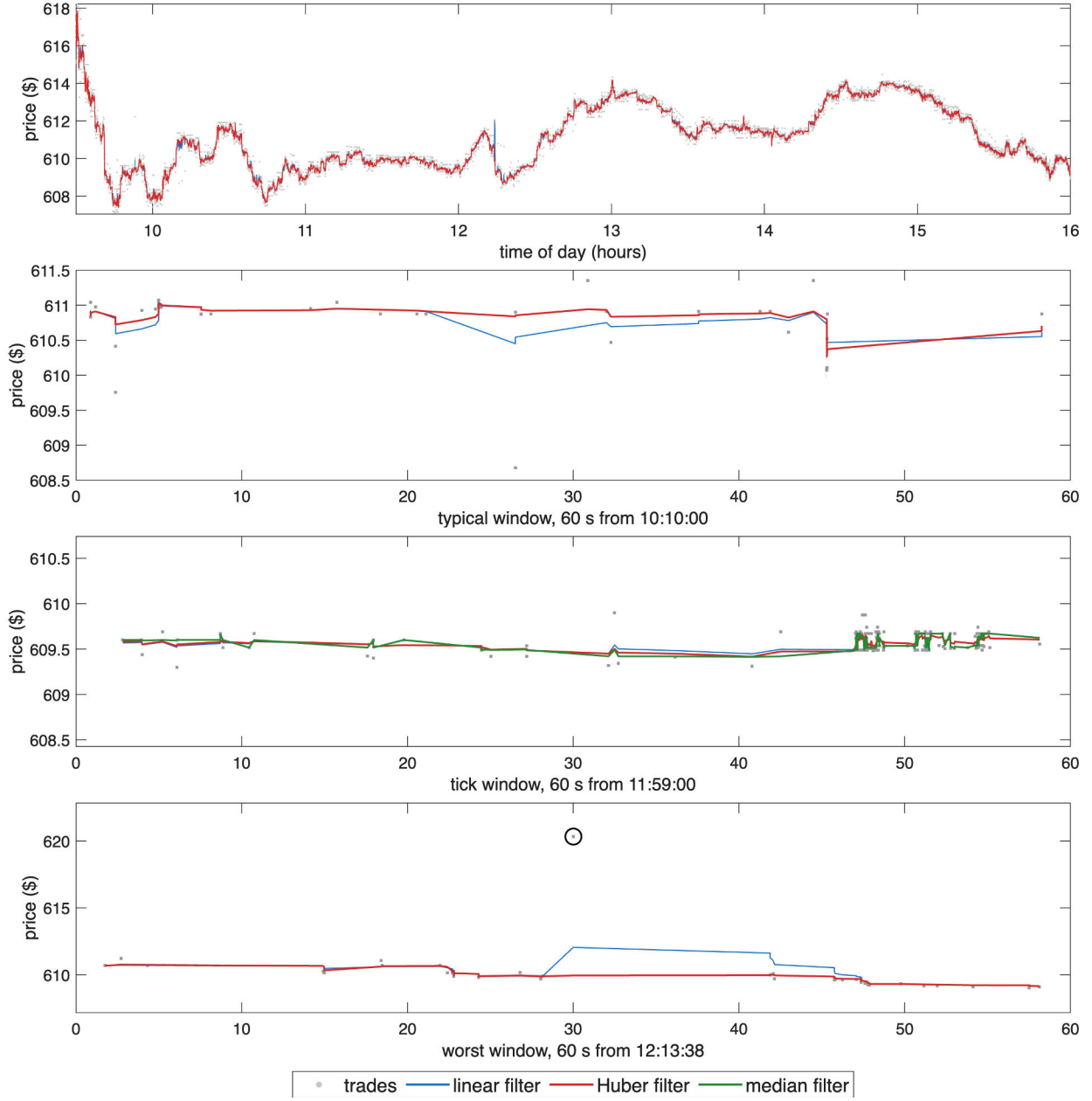
Figure 1: INTU trades (grey points), the linear filter and the Huber filter, 16 October 2024. Top: full trading day. 2nd: 60-second window at the day's median trade count, from 10:10:00. 3rd: 60-second window at 11:59:00 in which the price reverses direction most often, with the median filter m_t added. Bottom: 60-second window around the largest Huber residual after 09:45, circled.
