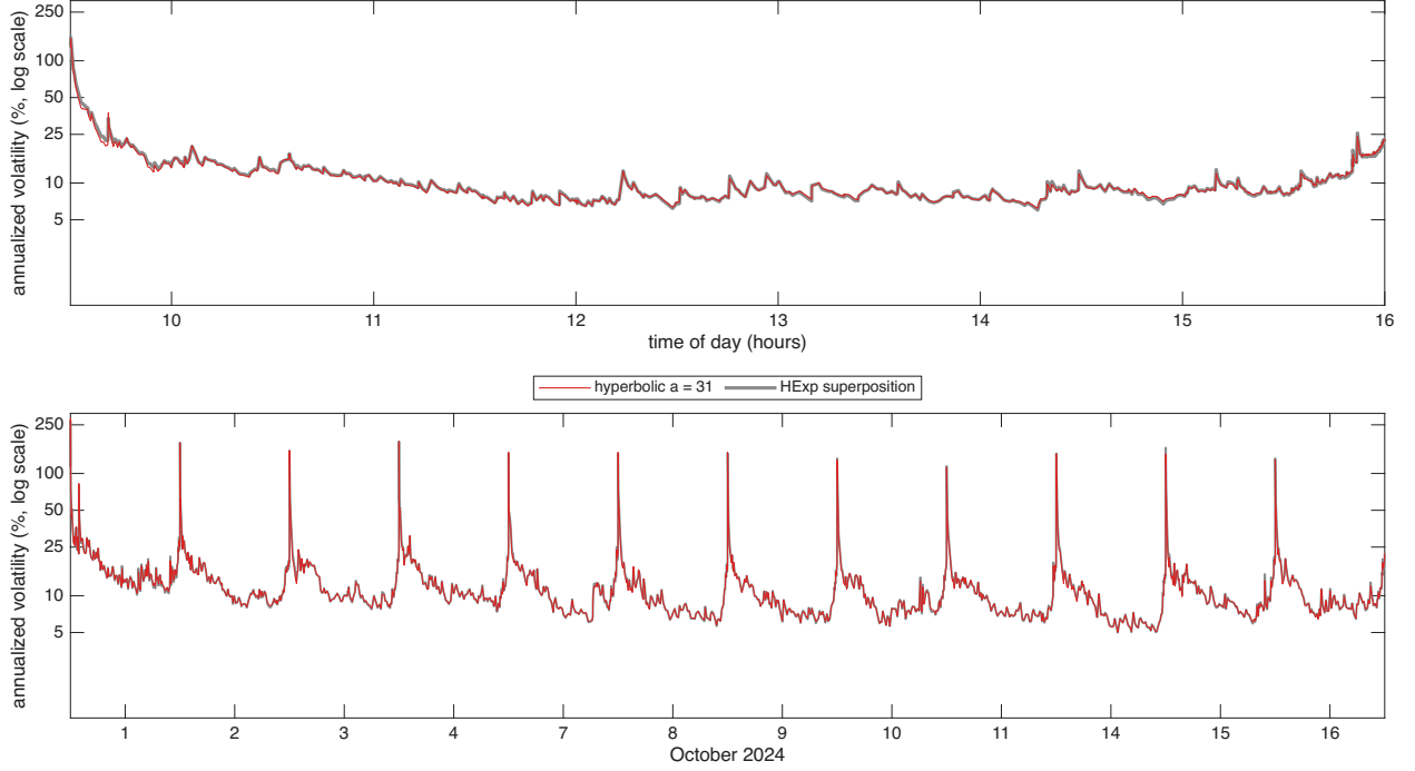
Figure 6: Hyperbolic against superposition weights for INTU over 12 trading days in Oct 2024, the diurnally adjusted \hat{\sigma}(u)100\sqrt{252} at s = 1 second from the Huber filter, shown as annualized vol in % on a log10 scale. The only difference between the 2 paths is the weight function: the hyperbolic weights with a = 31 in red, drawn on top, and the HExp superposition in grey, 4 exponential components with half lives of 10, 100, 1000, 10000 seconds. Hyperparameters minimize the QLIKE objective. Top: 16 October 2024, bottom: 12 days.
