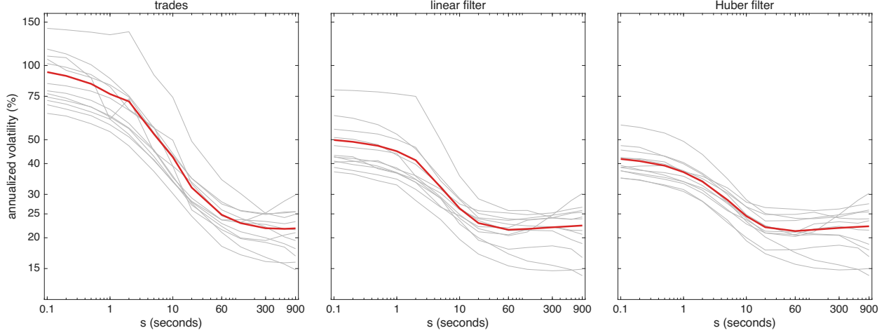
Figure 4: Volatility signature curves for INTU over the 12 trading days in Oct 2024. The annualized vol \hat{\sigma}100\sqrt{252} from the returns \hat{X}_t - \hat{X}_{t,s} of Table 2, against the lag s in seconds, both axes on log scales, for: raw trades, linear filter & Huber filter. Grey lines are the individual trading days & the red line is the square root of the 12 day average of their squares. The linear & Huber returns carry the finite-sample correction c_{t,s} of the paper; the raw trades are unaffected by it.
