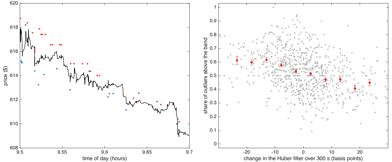
Figure 7: Outliers & robust price for INTU on 16 October 2024. Left: the 12 minutes with the largest move in the Huber filter that day; outliers above Y_t - \theta_t > \delta_{t-1} in red, outliers below Y_t - \theta_t < -\delta_{t-1} in blue, Huber filter in black. Right: over the 12 trading days, the 300 second empirical conditional probability that outliers are above (rather than below) the Huber band against the 300 second change in the Huber filter in basis points: light points are single bins, the line & bars are means & s.e.
