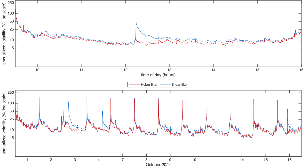
Figure 5: Filtered spot volatility for INTU over 12 trading days in Oct 2024, the diurnally adjusted estimator \hat{\sigma}(u)100\sqrt{252} at s = 1 second with hyperbolic weights, Mandelbrot parameter a = 31 , with the input prices computed using the Huber & linear filters, shown as annualized volatility in percent on a log10 scale. Top: 16 October 2024, bottom: 12 days.
