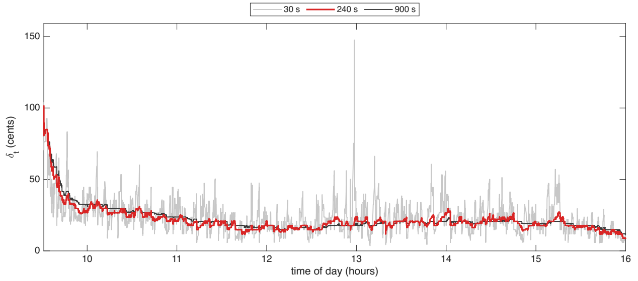
Figure 2: The Huber threshold \delta_t in cents for INTU on 16 October 2024, with half-lives of 30, 240, 900 seconds. The 240-second half-life, in red, is used.
