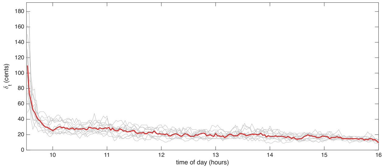
Figure 3: Huber threshold \delta_t in cents through the trading day, for 12 INTU trading days in Oct 2024 (grey lines) and their median (red line).
