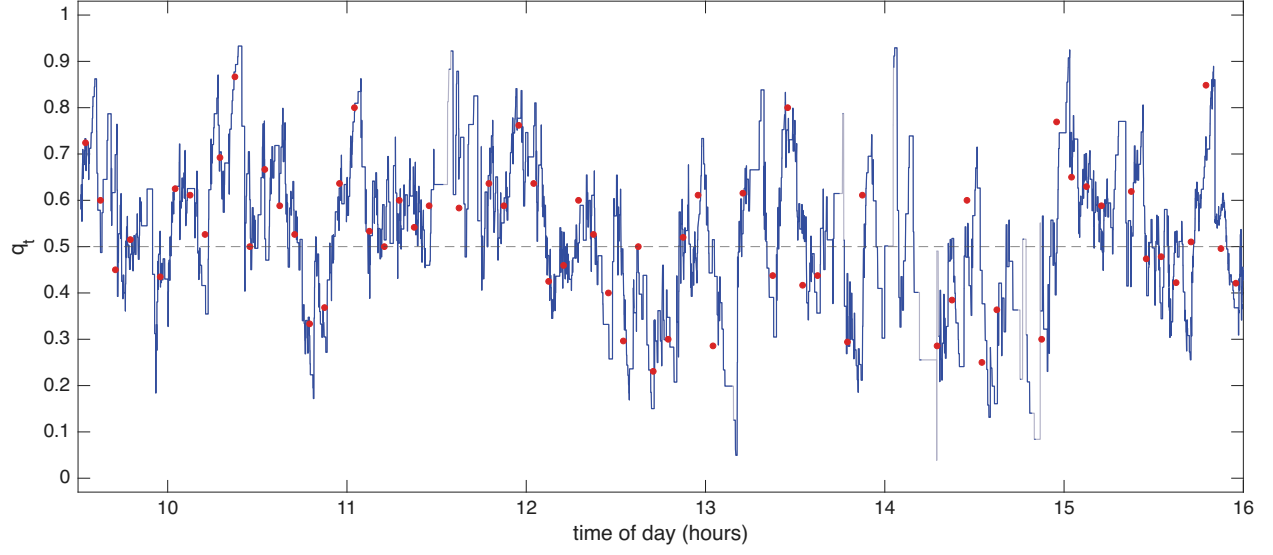
Figure 8: The directional conditional probability for INTU, 16 October 2024. The filtered conditional probability q_t that an outlier lies above the robust Huber band, under exponential weights decaying in clock time with half life of 87 seconds; where fewer than two outliers remain in the weights it is drawn in grey. The dashed line marks 0.5. The red points are the empirical conditional probability using the 300 second bins of the previous figure.
