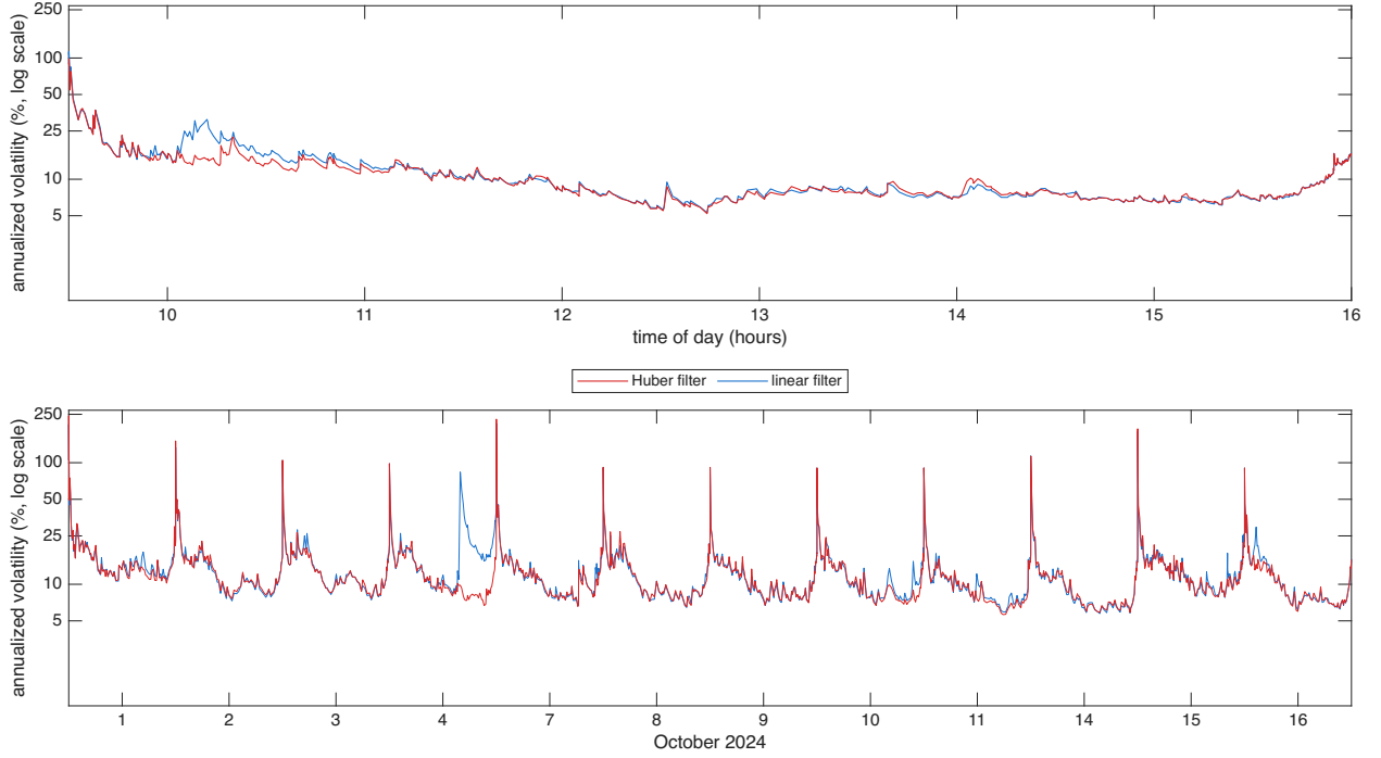
Figure 5: Filtered spot volatility for ISRG over 12 trading days in Oct 2024, the diurnally adjusted estimator \hat{\sigma}(u)100\sqrt{252} at s = 1 second with hyperbolic weights, Mandelbrot parameter a = 28 , with the input prices computed using the Huber & linear filters, shown as annualized volatility in percent on a log10 scale. Top: 16 October 2024, bottom: 12 days.
