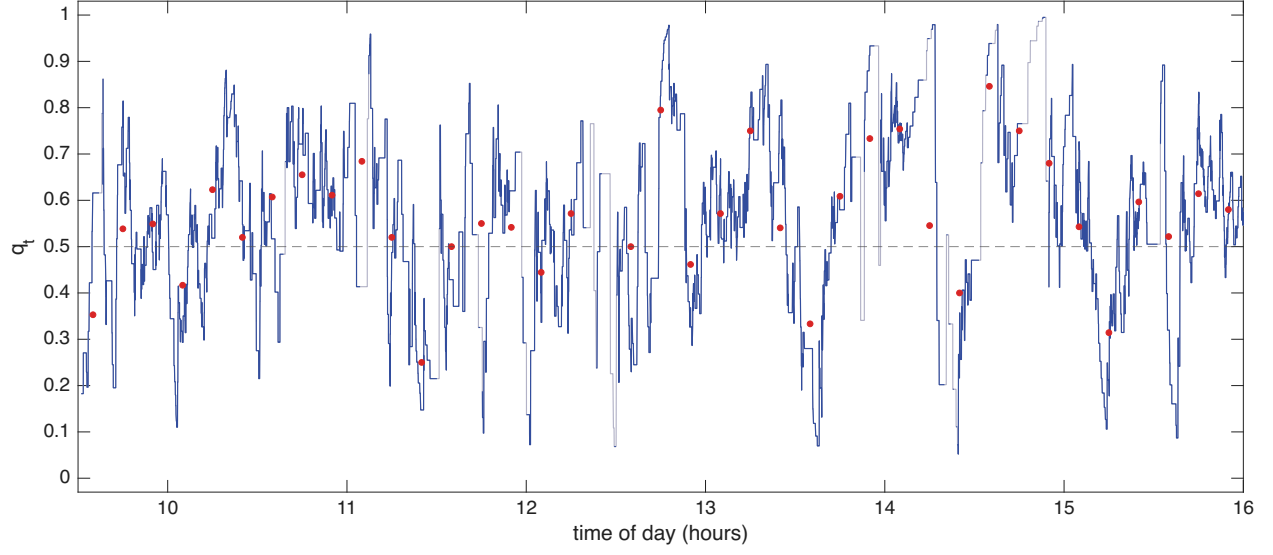
Figure 8: The directional conditional probability for ISRG, 16 October 2024. The filtered conditional probability q_t that an outlier lies above the robust Huber band, under exponential weights decaying in clock time with half life of 84 seconds; where fewer than two outliers remain in the weights it is drawn in grey. The dashed line marks 0.5. The red points are the empirical conditional probability using the 600 second bins of the previous figure.
