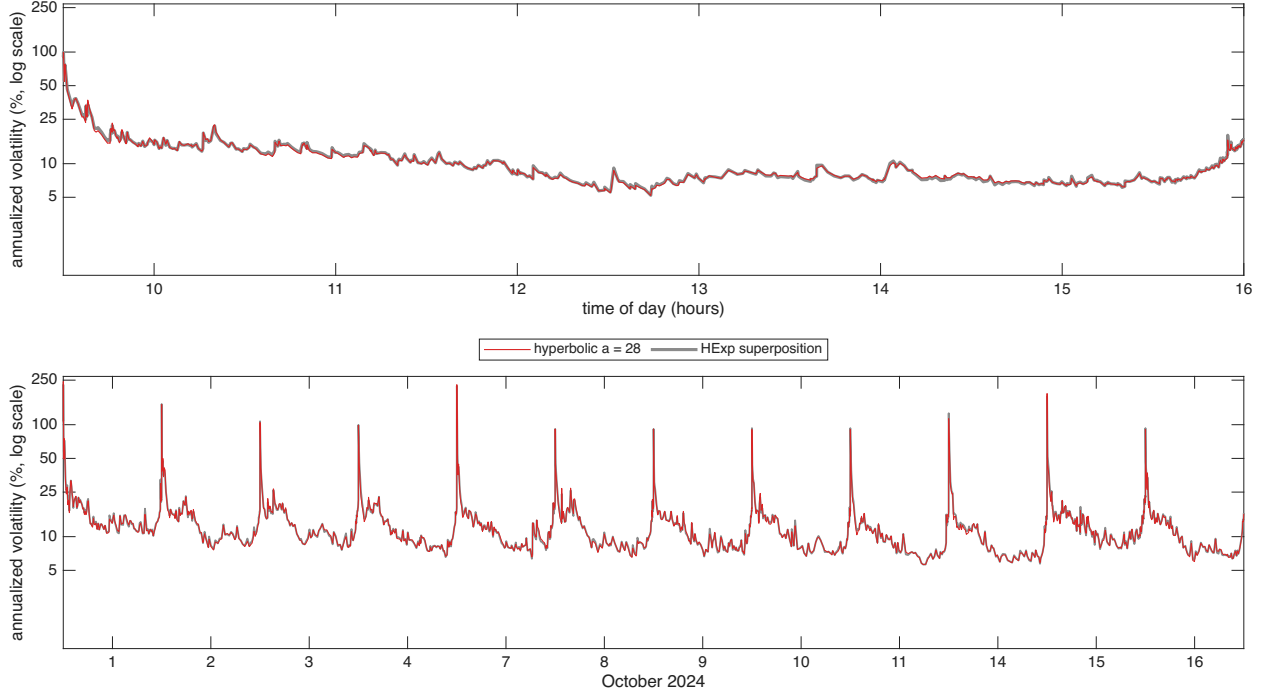
Figure 6: Hyperbolic against superposition weights for ISRG over 12 trading days in Oct 2024, the diurnally adjusted \hat{\sigma}(u)100\sqrt{252} at s = 1 second from the Huber filter, shown as annualized vol in % on a log10 scale. The only difference between the 2 paths is the weight function: the hyperbolic weights with a = 28 in red, drawn on top, and the HExp superposition in grey, 4 exponential components with half lives of 10, 100, 1000, 10000 seconds. Hyperparameters minimize the QLIKE objective. Top: 16 October 2024, bottom: 12 days.
