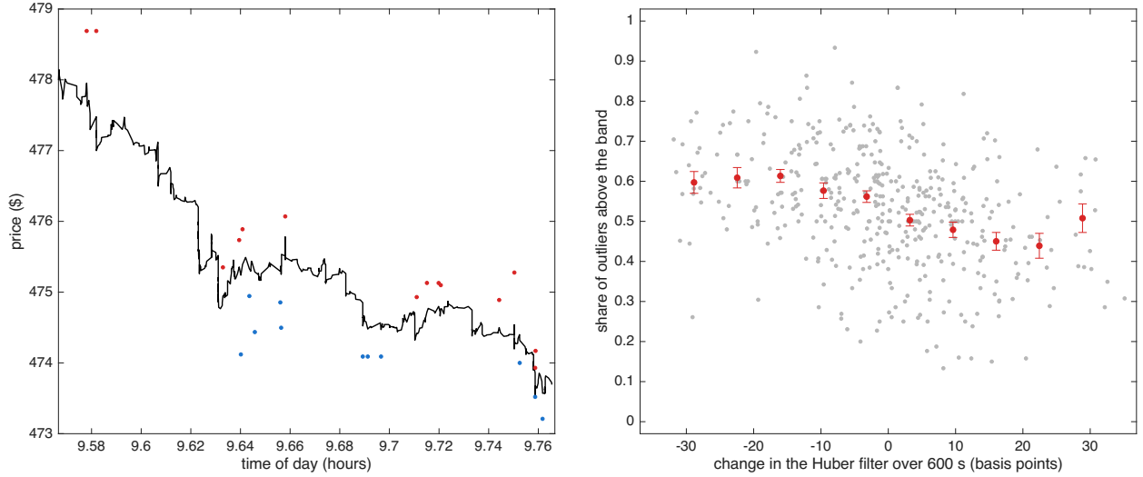
Figure 7: Outliers & robust price for ISRG on 16 October 2024. Left: the 12 minutes with the largest move in the Huber filter that day; outliers above Y_t - \theta_t > \delta_{t-1} in red, outliers below Y_t - \theta_t < -\delta_{t-1} in blue, Huber filter in black. Right: over the 12 trading days, the 600 second empirical conditional probability that outliers are above (rather than below) the Huber band against the 600 second change in the Huber filter in basis points: light points are single bins, the line & bars are means & s.e.
