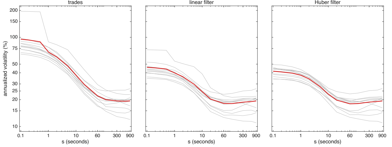
Figure 4: Volatility signature curves for ISRG over the 12 trading days in Oct 2024. The annualized vol \hat{\sigma}100\sqrt{252} from the returns \hat{X}_t - \hat{X}_{t,s} of Table 2, against the lag s in seconds, both axes on log scales, for: raw trades, linear filter & Huber filter. Grey lines are the individual trading days & the red line is the square root of the 12 day average of their squares. The linear & Huber returns carry the finite-sample correction c_{t,s} of the paper; the raw trades are unaffected by it.
