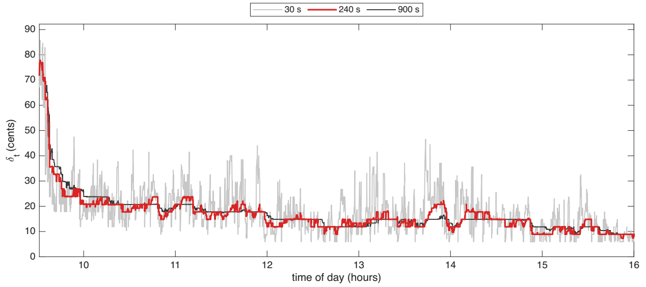
Figure 2: The Huber threshold \delta_t in cents for ISRG on 16 October 2024, with half-lives of 30, 240, 900 seconds. The 240-second half-life, in red, is used.
