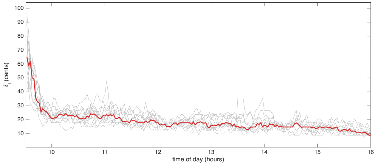
Figure 3: Huber threshold \delta_t in cents through the trading day, for 12 ISRG trading days in Oct 2024 (grey lines) and their median (red line).
