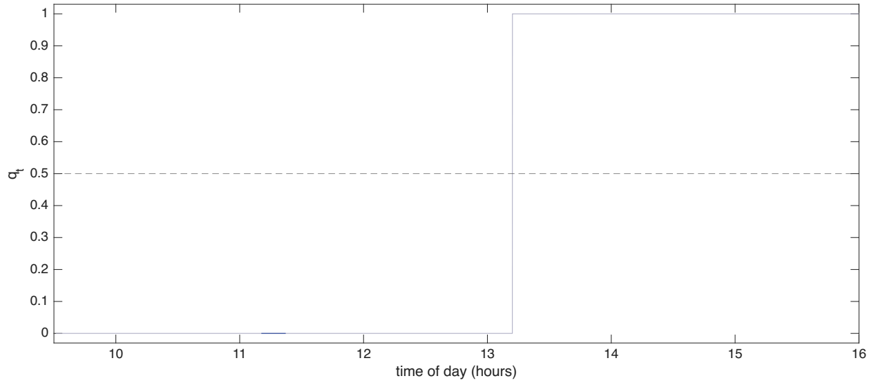
Figure 8: The directional conditional probability for LCID, 16 October 2024. The filtered conditional probability q_t that an outlier lies above the robust Huber band, under exponential weights decaying in clock time with half life of 415 seconds; where fewer than two outliers remain in the weights it is drawn in grey. The dashed line marks 0.5. The red points are the empirical conditional probability using the 1800 second bins of the previous figure.
