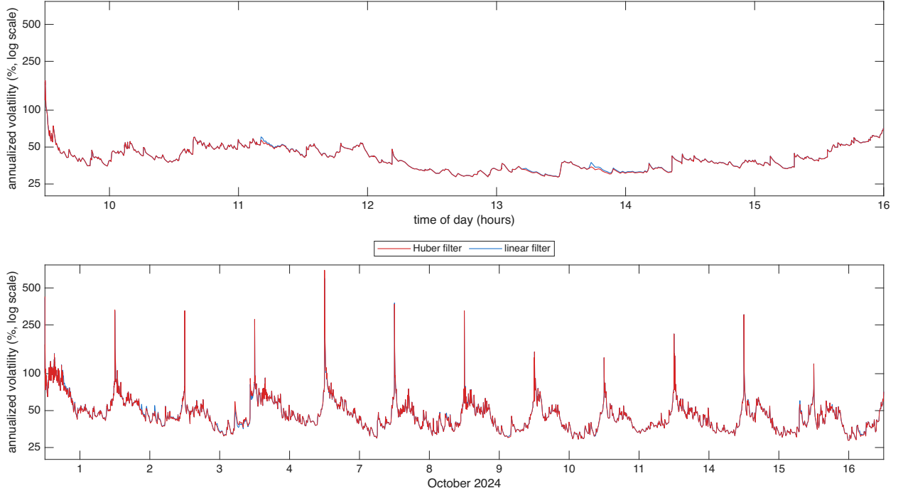
Figure 5: Filtered spot volatility for LCID over 12 trading days in Oct 2024, the diurnally adjusted estimator \hat{\sigma}(u)100\sqrt{252} at s = 1 second with hyperbolic weights, Mandelbrot parameter a = 74 , with the input prices computed using the Huber & linear filters, shown as annualized volatility in percent on a log10 scale. Top: 16 October 2024, bottom: 12 days.
