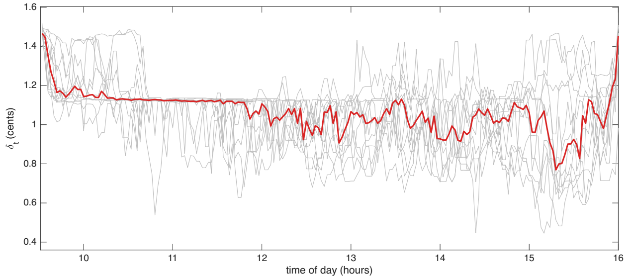
Figure 3: Huber threshold \delta_t in cents through the trading day, for 12 LCID trading days in Oct 2024 (grey lines) and their median (red line).
