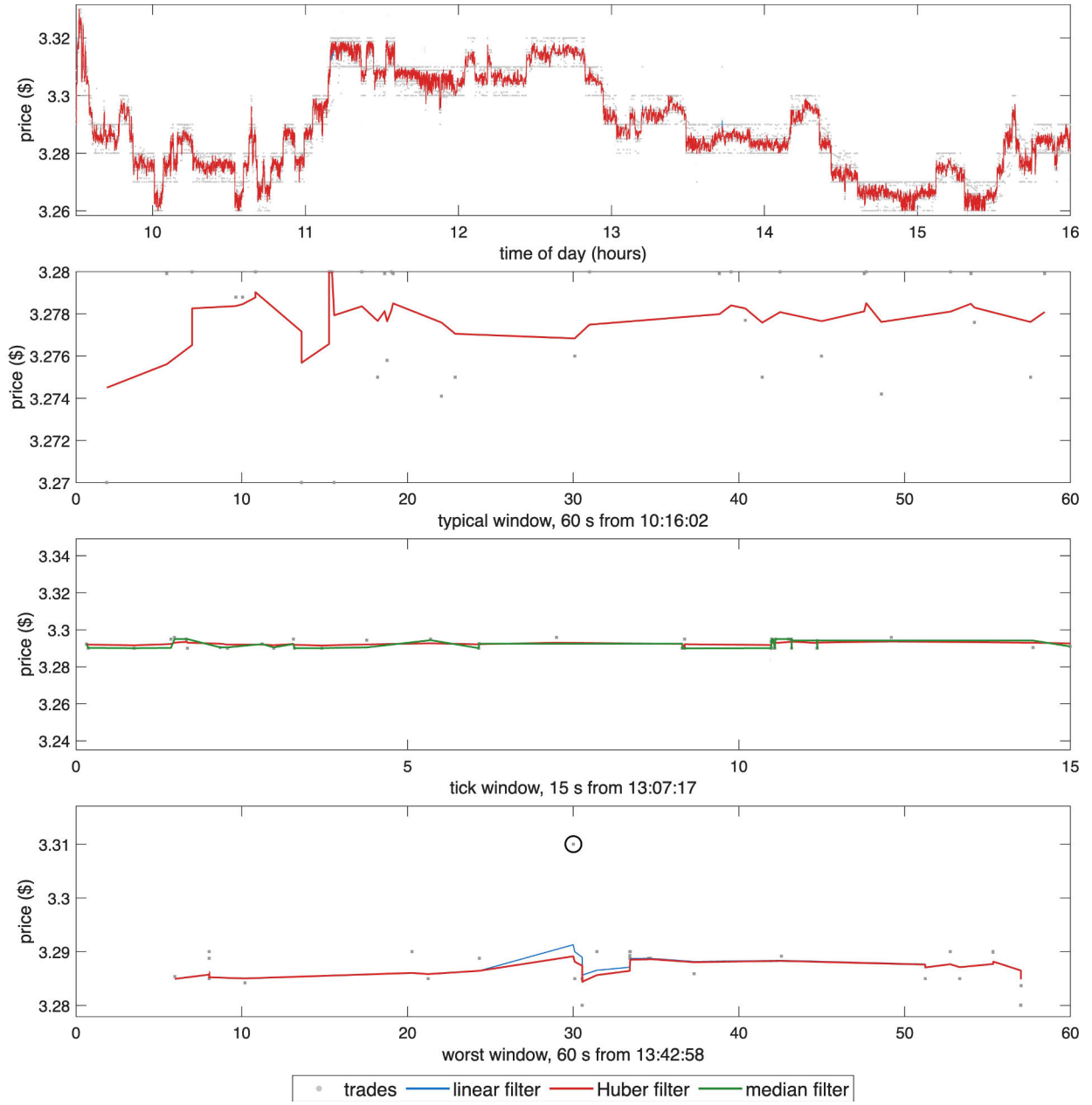
Figure 1: LCID trades (grey points), the linear filter and the Huber filter, 16 October 2024. Top: full trading day. 2nd: 60-second window at the day's median trade count, from 10:16:02. 3rd: 15-second window at 13:07:17 in which the price reverses direction most often, with the median filter m_t added. Bottom: 60-second window around the largest Huber residual after 09:45, circled.
