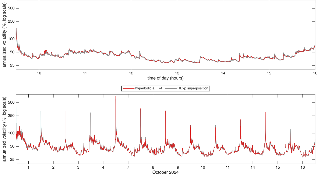
Figure 6: Hyperbolic against superposition weights for LCID over 12 trading days in Oct 2024, the diurnally adjusted \hat{\sigma}(u)100\sqrt{252} at s = 1 second from the Huber filter, shown as annualized vol in % on a log10 scale. The only difference between the 2 paths is the weight function: the hyperbolic weights with a = 74 in red, drawn on top, and the HExp superposition in grey, 4 exponential components with half lives of 10, 100, 1000, 10000 seconds. Hyperparameters minimize the QLIKE objective. Top: 16 October 2024, bottom: 12 days.
