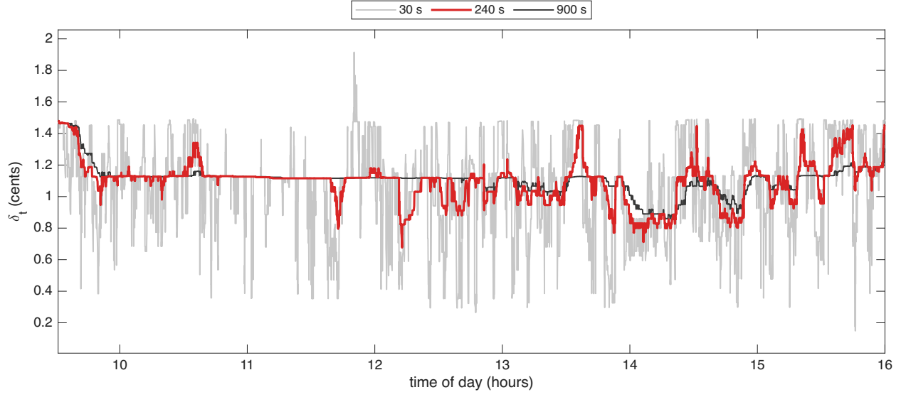
Figure 2: The Huber threshold \delta_t in cents for LCID on 16 October 2024, with half-lives of 30, 240, 900 seconds. The 240-second half-life, in red, is used.
