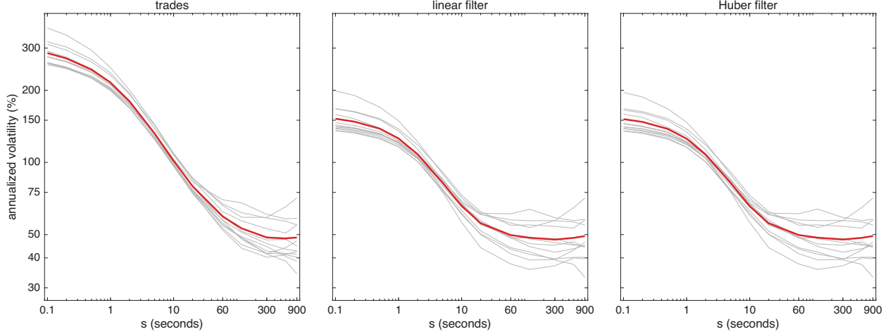
Figure 4: Volatility signature curves for LCID over the 12 trading days in Oct 2024. The annualized vol \hat{\sigma}100\sqrt{252} from the returns \hat{X}_t - \hat{X}_{t,s} of Table 2, against the lag s in seconds, both axes on log scales, for: raw trades, linear filter & Huber filter. Grey lines are the individual trading days & the red line is the square root of the 12 day average of their squares. The linear & Huber returns carry the finite-sample correction c_{t,s} of the paper; the raw trades are unaffected by it.
