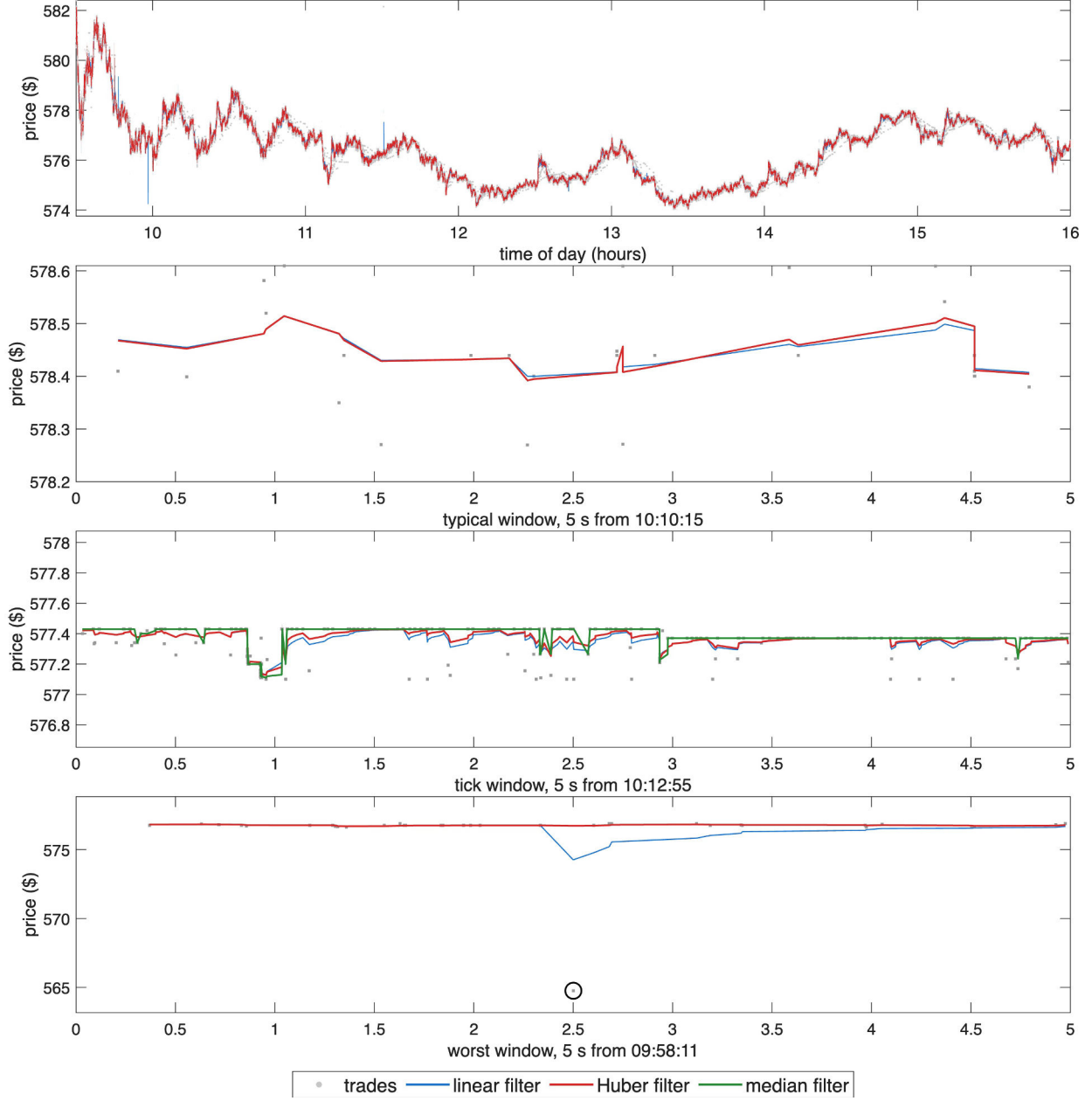
Figure 1: META trades (grey points), the linear filter and the Huber filter, 16 October 2024. Top: full trading day. 2nd: 5-second window at the day's median trade count, from 10:10:15. 3rd: 5-second window at 10:12:55 in which the price reverses direction most often, with the median filter m_t added. Bottom: 5-second window around the largest Huber residual after 09:45, circled.
