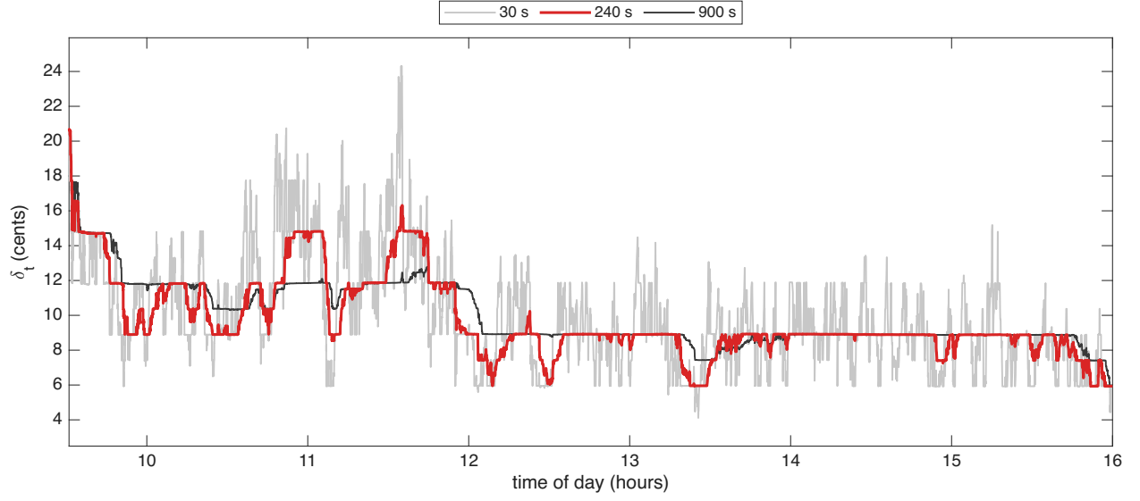
Figure 2: The Huber threshold \delta_t in cents for META on 16 October 2024, with half-lives of 30, 240, 900 seconds. The 240-second half-life, in red, is used.
