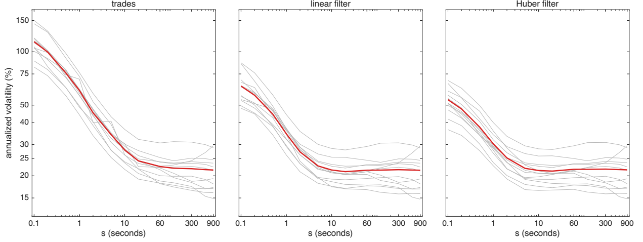
Figure 4: Volatility signature curves for META over the 12 trading days in Oct 2024. The annualized vol \hat{\sigma}100\sqrt{252} from the returns \hat{X}_t - \hat{X}_{t,s} of Table 2, against the lag s in seconds, both axes on log scales, for: raw trades, linear filter & Huber filter. Grey lines are the individual trading days & the red line is the square root of the 12 day average of their squares. The linear & Huber returns carry the finite-sample correction c_{t,s} of the paper; the raw trades are unaffected by it.
