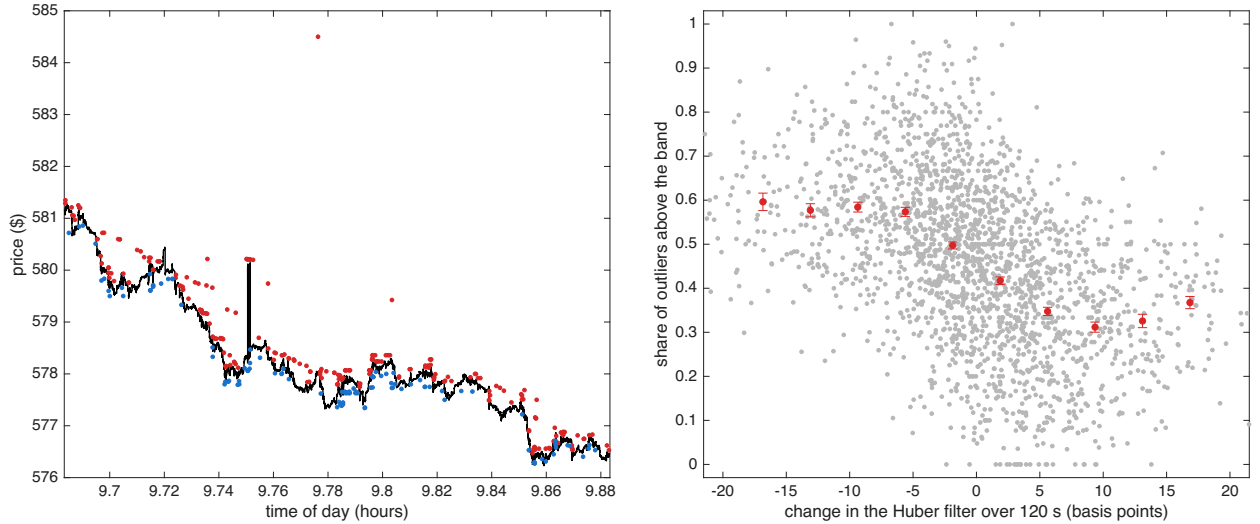
Figure 7: Outliers & robust price for META on 16 October 2024. Left: the 12 minutes with the largest move in the Huber filter that day; outliers above Y_t - \theta_t > \delta_{t-1} in red, outliers below Y_t - \theta_t < -\delta_{t-1} in blue, Huber filter in black. Right: over the 12 trading days, the 120 second empirical conditional probability that outliers are above (rather than below) the Huber band against the 120 second change in the Huber filter in basis points: light points are single bins, the line & bars are means & s.e.
