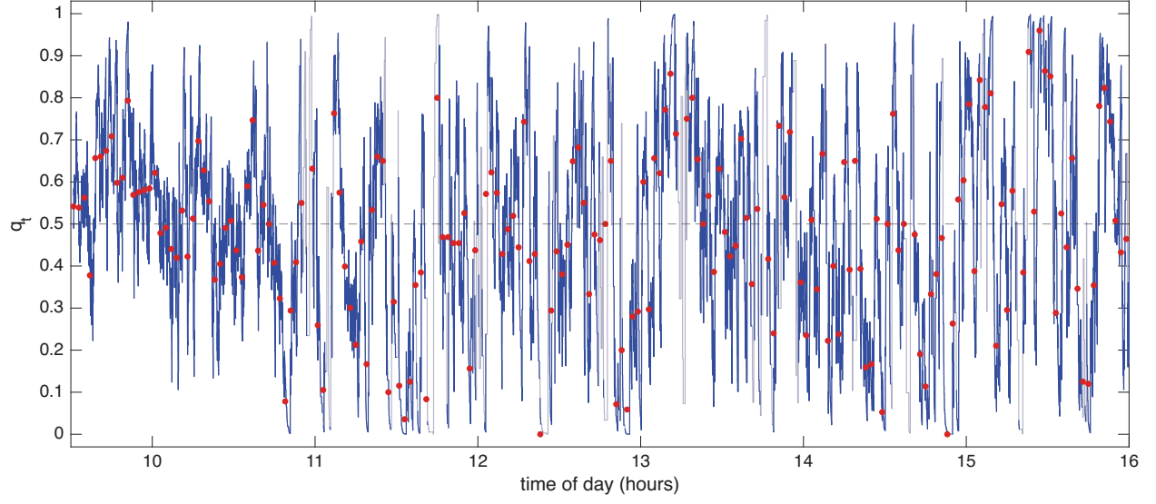
Figure 8: The directional conditional probability for META, 16 October 2024. The filtered conditional probability q_t that an outlier lies above the robust Huber band, under exponential weights decaying in clock time with half life of 14 seconds; where fewer than two outliers remain in the weights it is drawn in grey. The dashed line marks 0.5. The red points are the empirical conditional probability using the 120 second bins of the previous figure.
