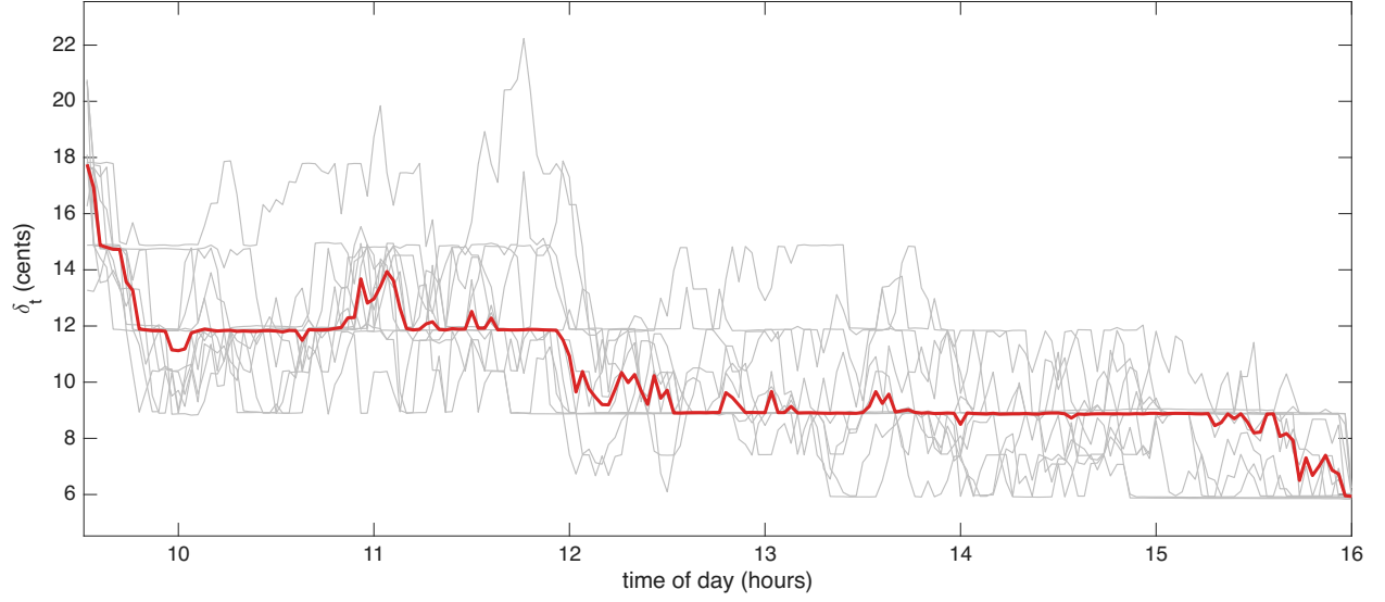
Figure 3: Huber threshold \delta_t in cents through the trading day, for 12 META trading days in Oct 2024 (grey lines) and their median (red line).
