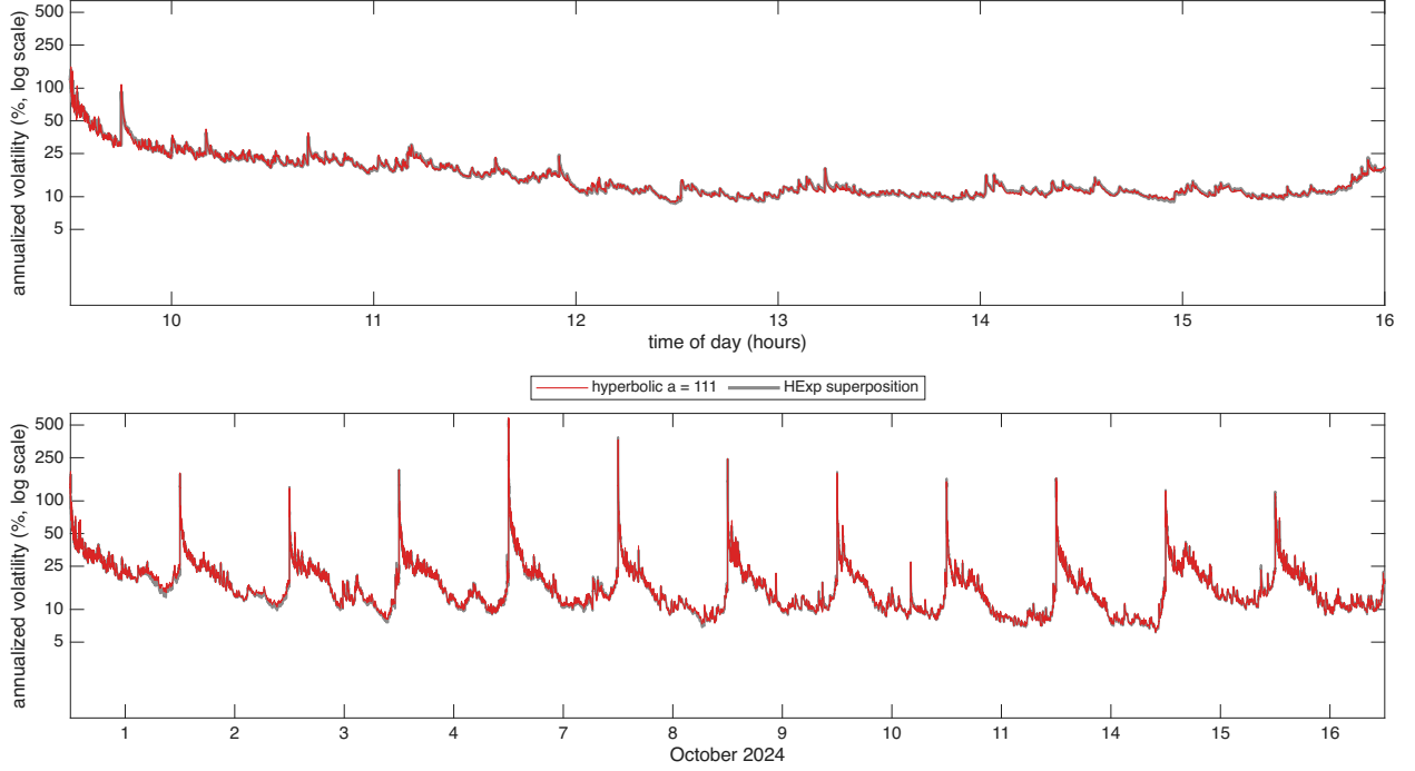
Figure 6: Hyperbolic against superposition weights for META over 12 trading days in Oct 2024, the diurnally adjusted \hat{\sigma}(u)100\sqrt{252} at s = 1 second from the Huber filter, shown as annualized vol in % on a log10 scale. The only difference between the 2 paths is the weight function: the hyperbolic weights with a = 111 in red, drawn on top, and the HExp superposition in grey, 4 exponential components with half lives of 2, 20, 200, 2000 seconds. Hyperparameters minimize the QLIKE objective. Top: 16 October 2024, bottom: 12 days.
