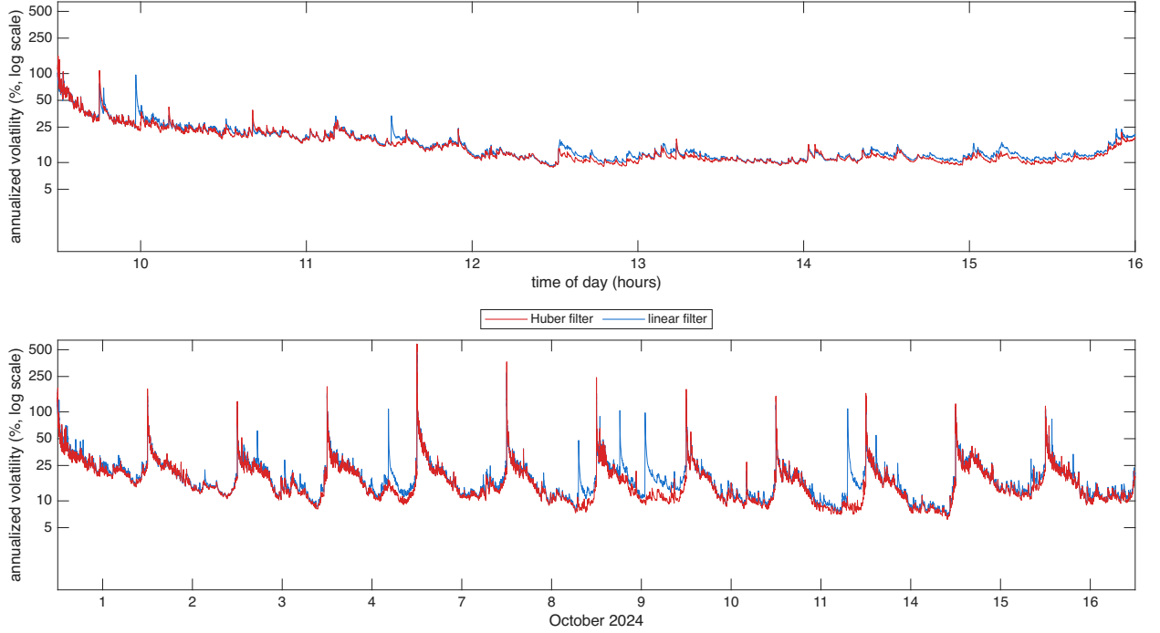
Figure 5: Filtered spot volatility for META over 12 trading days in Oct 2024, the diurnally adjusted estimator \hat{\sigma}(u)100\sqrt{252} at s = 1 second with hyperbolic weights, Mandelbrot parameter a = 111 , with the input prices computed using the Huber & linear filters, shown as annualized volatility in percent on a log10 scale. Top: 16 October 2024, bottom: 12 days.
