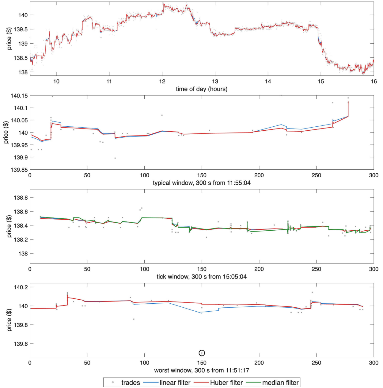
Figure 1: MIDD trades (grey points), the linear filter and the Huber filter, 16 October 2024. Top: full trading day. 2nd: 300-second window at the day's median trade count, from 11:55:04. 3rd: 300-second window at 15:05:04 in which the price reverses direction most often, with the median filter m_t added. Bottom: 300-second window around the largest Huber residual after 09:45, circled.
