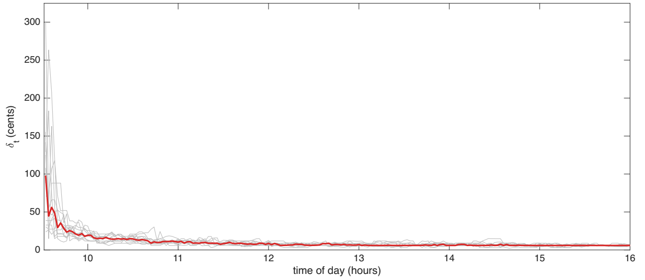
Figure 3: Huber threshold \delta_t in cents through the trading day, for 12 MIDD trading days in Oct 2024 (grey lines) and their median (red line).
