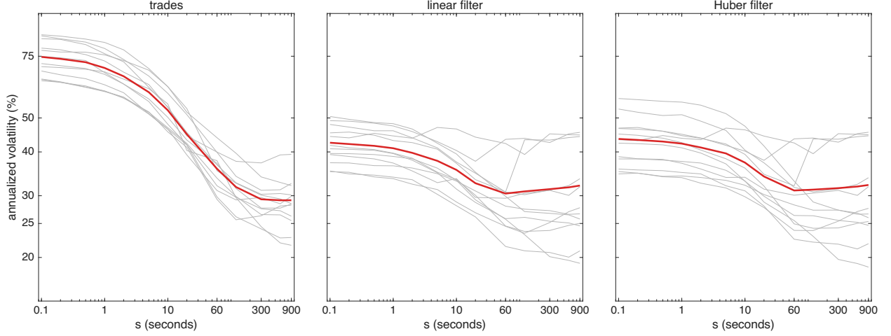
Figure 4: Volatility signature curves for MIDD over the 12 trading days in Oct 2024. The annualized vol \hat{\sigma}100\sqrt{252} from the returns \hat{X}_t - \hat{X}_{t,s} of Table 2, against the lag s in seconds, both axes on log scales, for: raw trades, linear filter & Huber filter. Grey lines are the individual trading days & the red line is the square root of the 12 day average of their squares. The linear & Huber returns carry the finite-sample correction c_{t,s} of the paper; the raw trades are unaffected by it.
