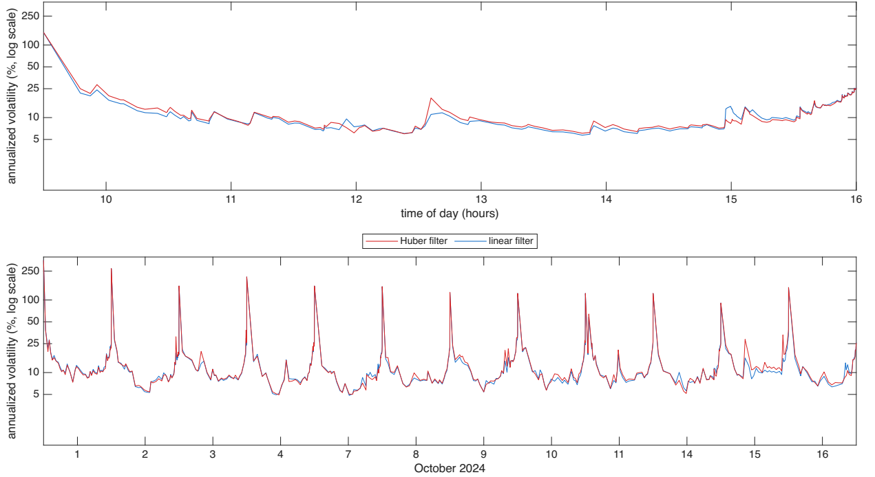
Figure 5: Filtered spot volatility for MIDD over 12 trading days in Oct 2024, the diurnally adjusted estimator \hat{\sigma}(u)100\sqrt{252} at s = 1 second with hyperbolic weights, Mandelbrot parameter a = 21 , with the input prices computed using the Huber & linear filters, shown as annualized volatility in percent on a log10 scale. Top: 16 October 2024, bottom: 12 days.
