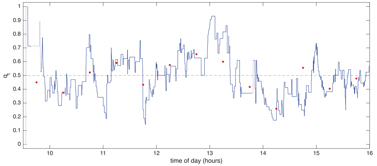
Figure 8: The directional conditional probability for MIDD, 16 October 2024. The filtered conditional probability q_t that an outlier lies above the robust Huber band, under exponential weights decaying in clock time with half life of 315 seconds; where fewer than two outliers remain in the weights it is drawn in grey. The dashed line marks 0.5. The red points are the empirical conditional probability using the 1800 second bins of the previous figure.
