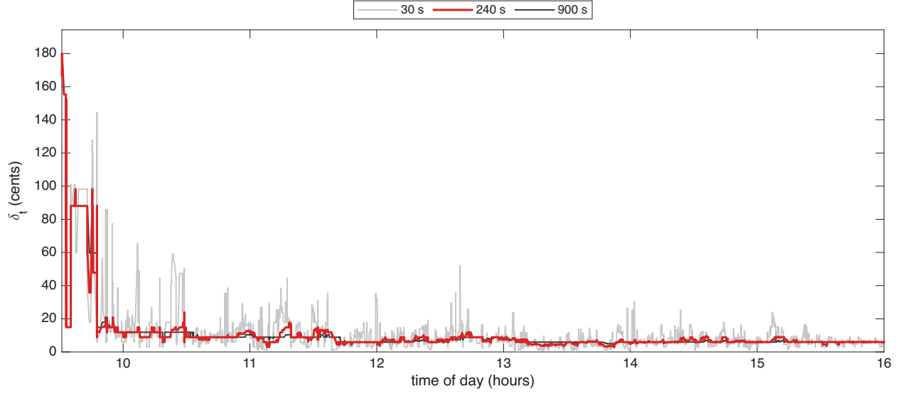
Figure 2: The Huber threshold \delta_t in cents for MIDD on 16 October 2024, with half-lives of 30, 240, 900 seconds. The 240-second half-life, in red, is used.
