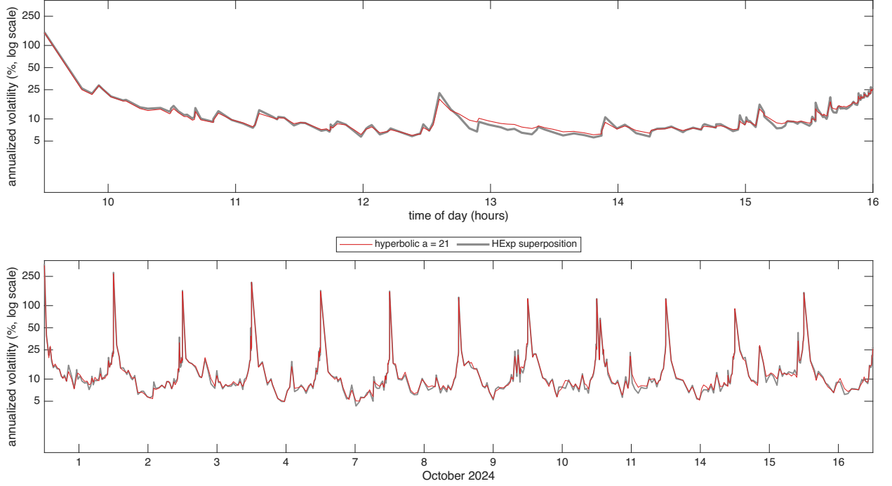
Figure 6: Hyperbolic against superposition weights for MIDD over 12 trading days in Oct 2024, the diurnally adjusted \hat{\sigma}(u)100\sqrt{252} at s = 1 second from the Huber filter, shown as annualized vol in % on a log10 scale. The only difference between the 2 paths is the weight function: the hyperbolic weights with a = 21 in red, drawn on top, and the HExp superposition in grey, 4 exponential components with half lives of 60, 600, 3600, 23400 seconds. Hyperparameters minimize the QLIKE objective. Top: 16 October 2024, bottom: 12 days.
