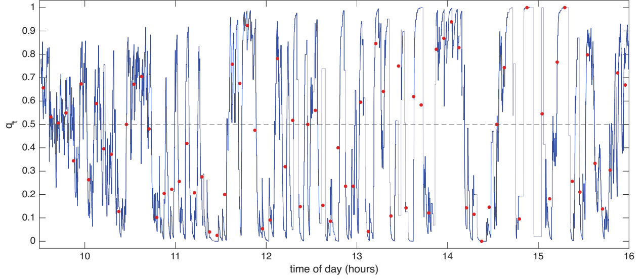
Figure 8: The directional conditional probability for MRVL, 16 October 2024. The filtered conditional probability q_t that an outlier lies above the robust Huber band, under exponential weights decaying in clock time with half life of 31 seconds; where fewer than two outliers remain in the weights it is drawn in grey. The dashed line marks 0.5. The red points are the empirical conditional probability using the 300 second bins of the previous figure.
