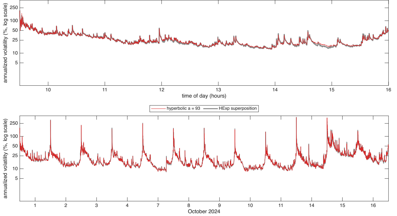
Figure 6: Hyperbolic against superposition weights for MRVL over 12 trading days in Oct 2024, the diurnally adjusted \hat{\sigma}(u)100\sqrt{252} at s = 1 second from the Huber filter, shown as annualized vol in % on a log10 scale. The only difference between the 2 paths is the weight function: the hyperbolic weights with a = 93 in red, drawn on top, and the HExp superposition in grey, 4 exponential components with half lives of 10, 100, 1000, 10000 seconds. Hyperparameters minimize the QLIKE objective. Top: 16 October 2024, bottom: 12 days.
