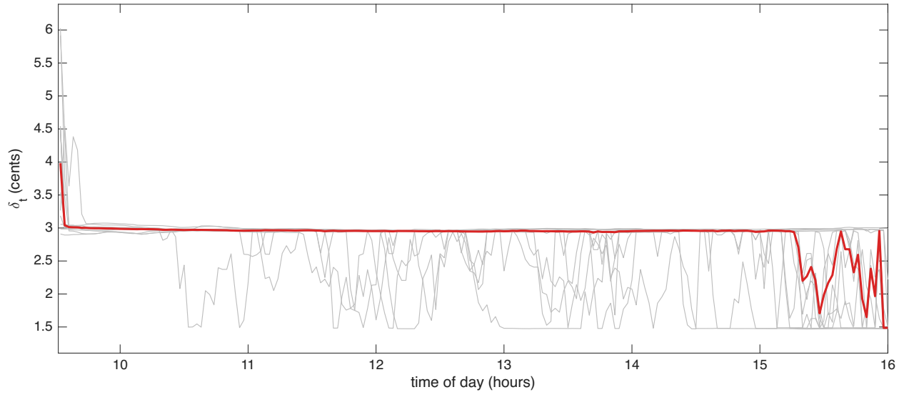
Figure 3: Huber threshold \delta_t in cents through the trading day, for 12 MRVL trading days in Oct 2024 (grey lines) and their median (red line).
