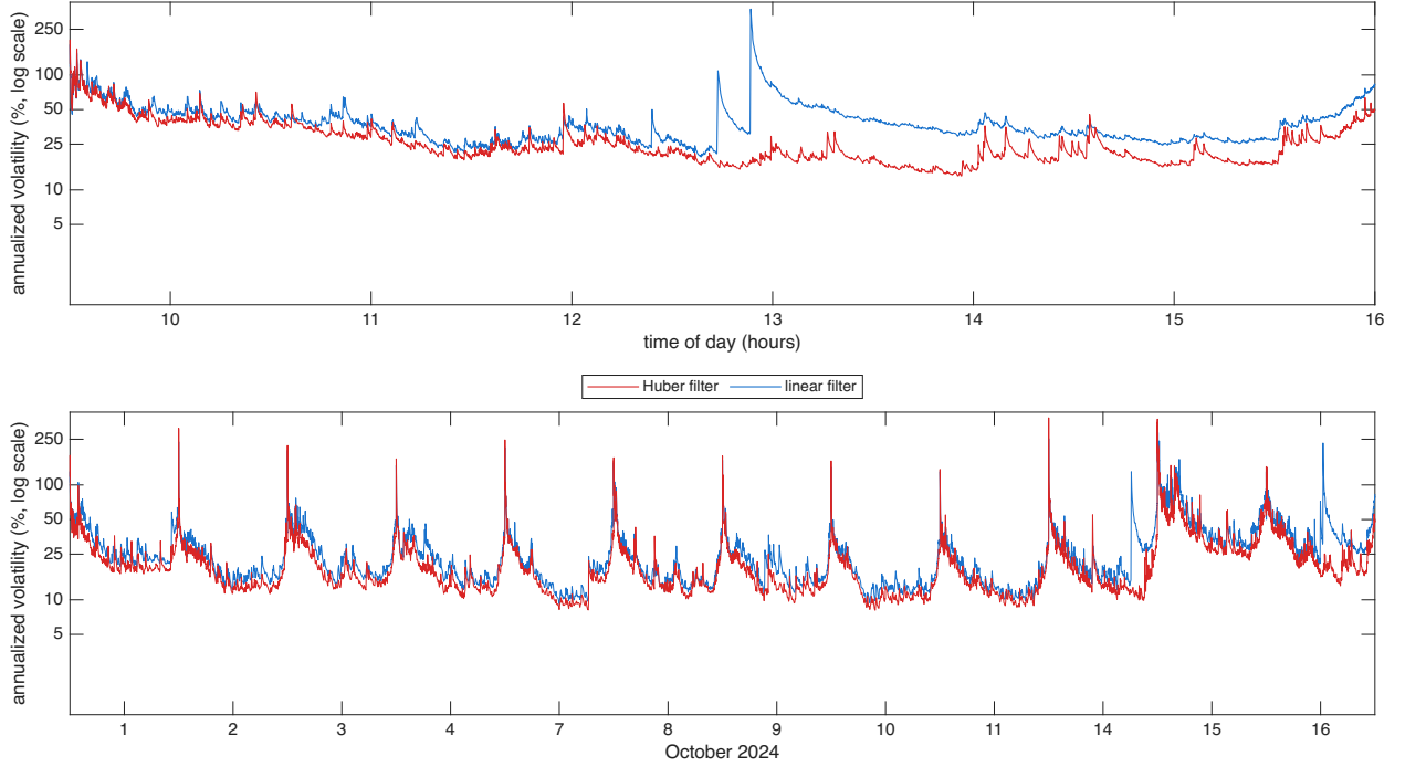
Figure 5: Filtered spot volatility for MRVL over 12 trading days in Oct 2024, the diurnally adjusted estimator \hat{\sigma}(u)100\sqrt{252} at s = 1 second with hyperbolic weights, Mandelbrot parameter a = 93 , with the input prices computed using the Huber & linear filters, shown as annualized volatility in percent on a log10 scale. Top: 16 October 2024, bottom: 12 days.
