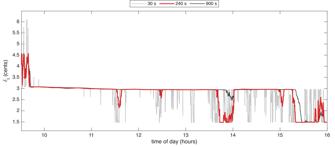
Figure 2: The Huber threshold \delta_t in cents for MRVL on 16 October 2024, with half-lives of 30, 240, 900 seconds. The 240-second half-life, in red, is used.
