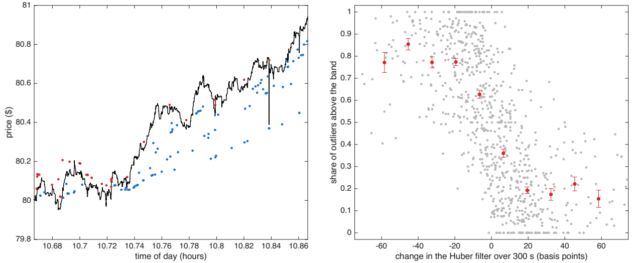
Figure 7: Outliers & robust price for MRVL on 16 October 2024. Left: the 12 minutes with the largest move in the Huber filter that day; outliers above Y_t - \theta_t > \delta_{t-1} in red, outliers below Y_t - \theta_t < -\delta_{t-1} in blue, Huber filter in black. Right: over the 12 trading days, the 300 second empirical conditional probability that outliers are above (rather than below) the Huber band against the 300 second change in the Huber filter in basis points: light points are single bins, the line & bars are means & s.e.
