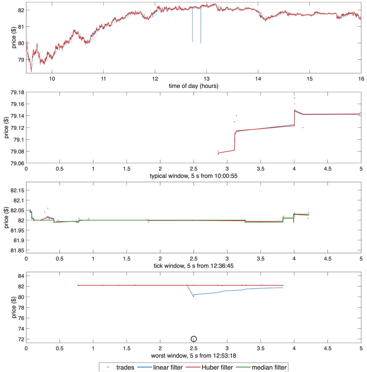
Figure 1: MRVL trades (grey points), the linear filter and the Huber filter, 16 October 2024. Top: full trading day. 2nd: 5-second window at the day's median trade count, from 10:00:55. 3rd: 5-second window at 12:36:45 in which the price reverses direction most often, with the median filter m_t added. Bottom: 5-second window around the largest Huber residual after 09:45, circled.
