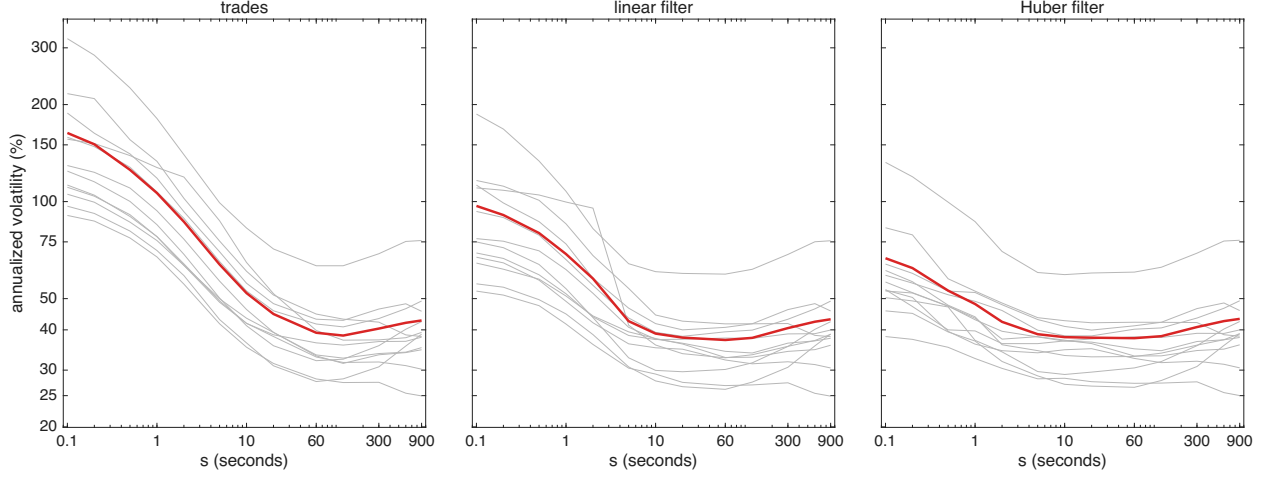
Figure 4: Volatility signature curves for MRVL over the 12 trading days in Oct 2024. The annualized vol \hat{\sigma}100\sqrt{252} from the returns \hat{X}_t - \hat{X}_{t,s} of Table 2, against the lag s in seconds, both axes on log scales, for: raw trades, linear filter & Huber filter. Grey lines are the individual trading days & the red line is the square root of the 12 day average of their squares. The linear & Huber returns carry the finite-sample correction c_{t,s} of the paper; the raw trades are unaffected by it.
