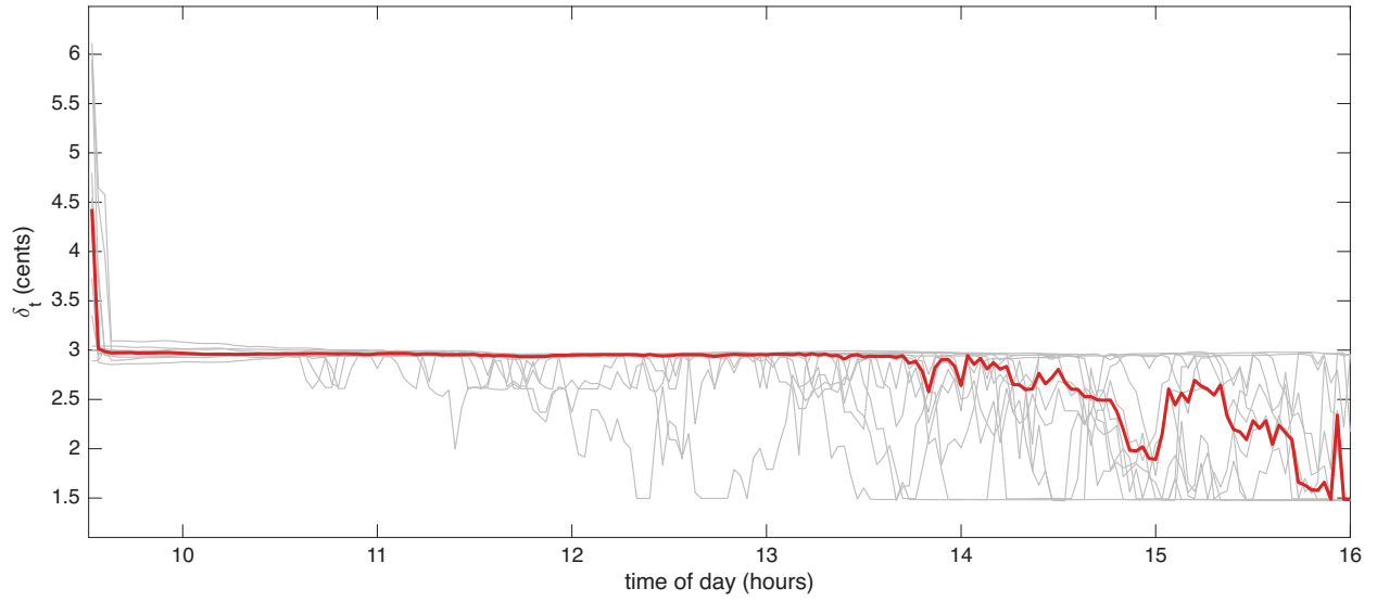
Figure 3: Huber threshold \delta_t in cents through the trading day, for 12 MU trading days in Oct 2024 (grey lines) and their median (red line).
