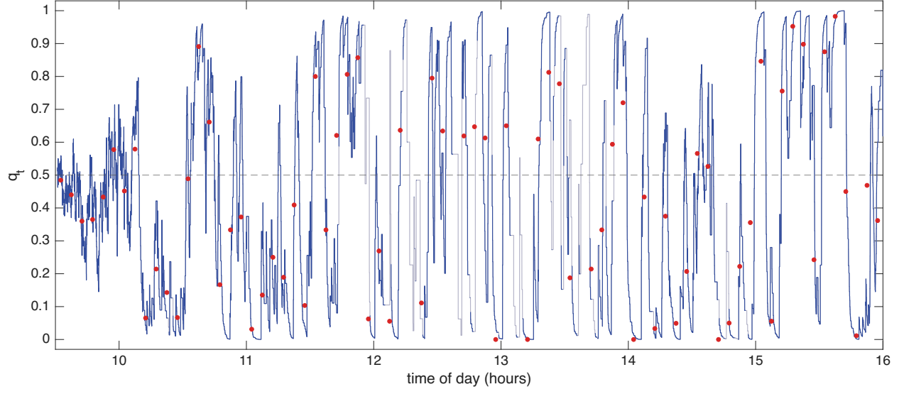
Figure 8: The directional conditional probability for MU, 16 October 2024. The filtered conditional probability q_t that an outlier lies above the robust Huber band, under exponential weights decaying in clock time with half life of 36 seconds; where fewer than two outliers remain in the weights it is drawn in grey. The dashed line marks 0.5. The red points are the empirical conditional probability using the 300 second bins of the previous figure.
