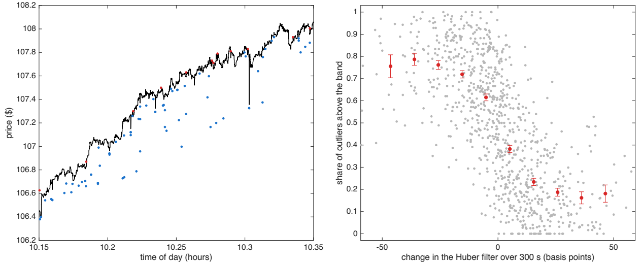
Figure 7: Outliers & robust price for MU on 16 October 2024. Left: the 12 minutes with the largest move in the Huber filter that day; outliers above Y_t - \theta_t > \delta_{t-1} in red, outliers below Y_t - \theta_t < -\delta_{t-1} in blue, Huber filter in black. Right: over the 12 trading days, the 300 second empirical conditional probability that outliers are above (rather than below) the Huber band against the 300 second change in the Huber filter in basis points: light points are single bins, the line & bars are means & s.e.
