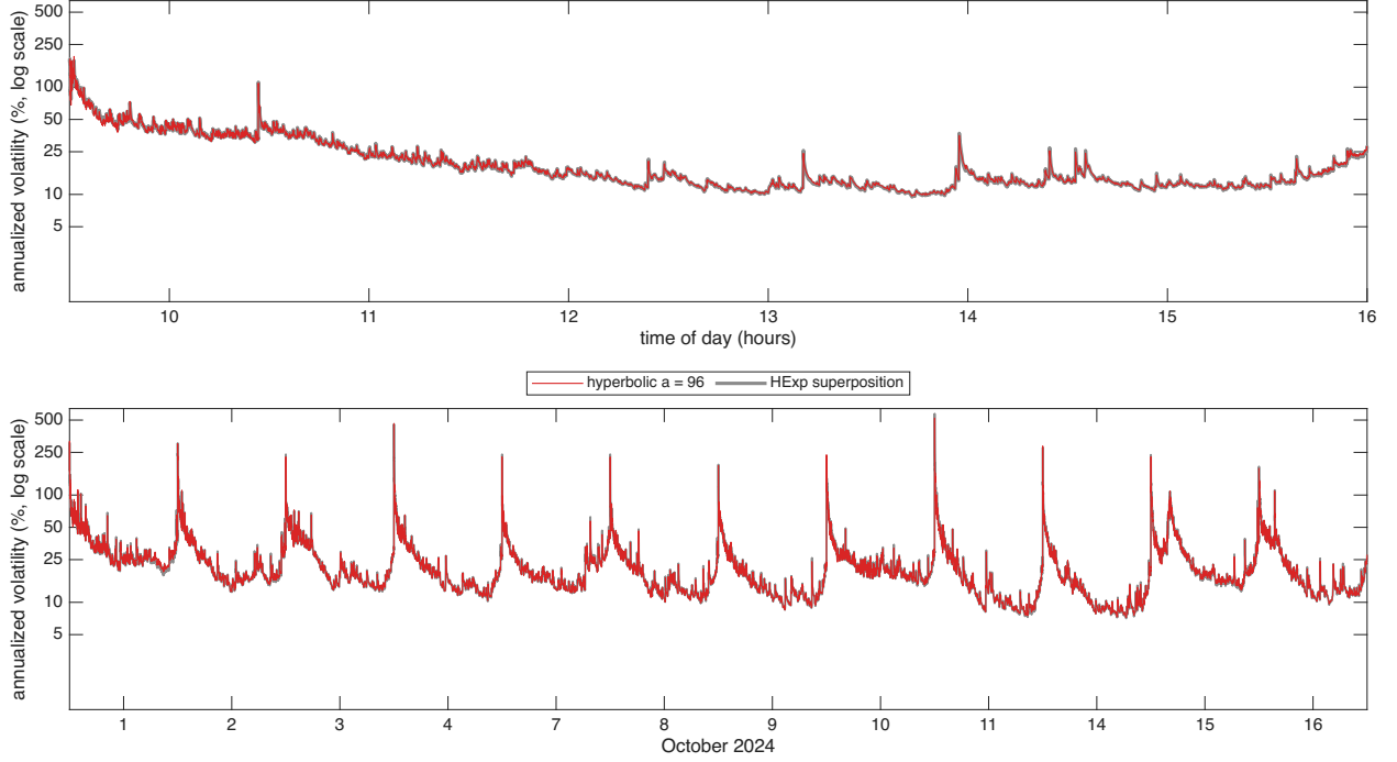
Figure 6: Hyperbolic against superposition weights for MU over 12 trading days in Oct 2024, the diurnally adjusted \hat{\sigma}(u)100\sqrt{252} at s = 1 second from the Huber filter, shown as annualized vol in % on a log10 scale. The only difference between the 2 paths is the weight function: the hyperbolic weights with a = 96 in red, drawn on top, and the HExp superposition in grey, 4 exponential components with half lives of 10, 100, 1000, 10000 seconds. Hyperparameters minimize the QLIKE objective. Top: 16 October 2024, bottom: 12 days.
