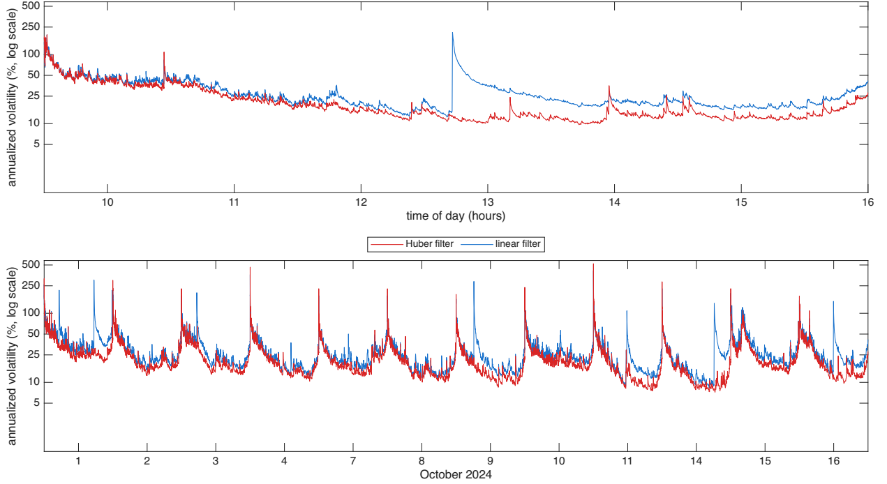
Figure 5: Filtered spot volatility for MU over 12 trading days in Oct 2024, the diurnally adjusted estimator \hat{\sigma}(u)100\sqrt{252} at s = 1 second with hyperbolic weights, Mandelbrot parameter a = 96 , with the input prices computed using the Huber & linear filters, shown as annualized volatility in percent on a log10 scale. Top: 16 October 2024, bottom: 12 days.
