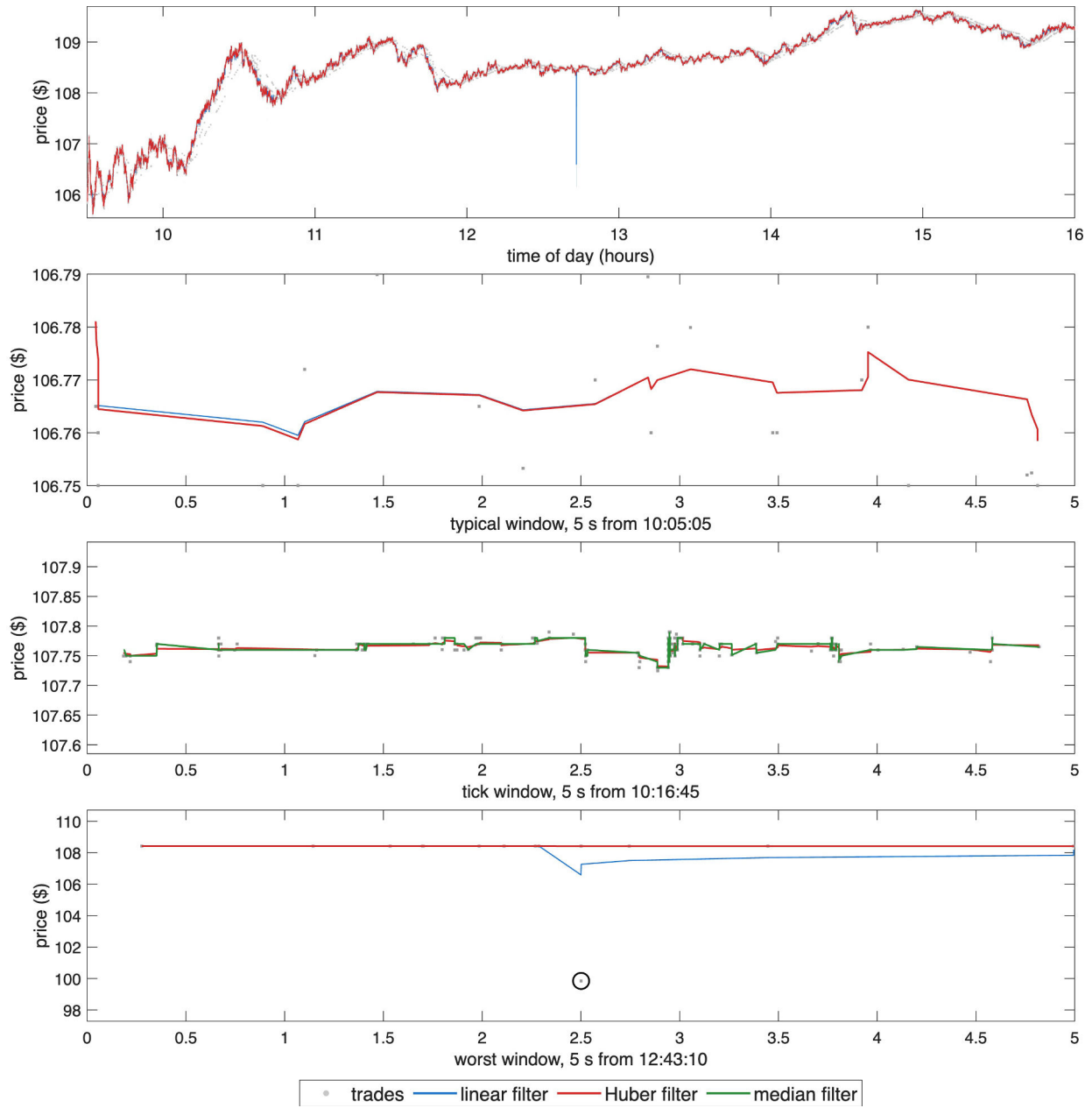
Figure 1: MU trades (grey points), the linear filter and the Huber filter, 16 October 2024. Top: full trading day. 2nd: 5-second window at the day's median trade count, from 10:05:05. 3rd: 5-second window at 10:16:45 in which the price reverses direction most often, with the median filter m_t added. Bottom: 5-second window around the largest Huber residual after 09:45, circled.
