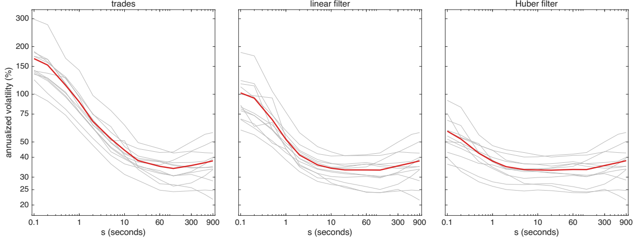
Figure 4: Volatility signature curves for MU over the 12 trading days in Oct 2024. The annualized vol \hat{\sigma}100\sqrt{252} from the returns \hat{X}_t - \hat{X}_{t,s} of Table 2, against the lag s in seconds, both axes on log scales, for: raw trades, linear filter & Huber filter. Grey lines are the individual trading days & the red line is the square root of the 12 day average of their squares. The linear & Huber returns carry the finite-sample correction c_{t,s} of the paper; the raw trades are unaffected by it.
