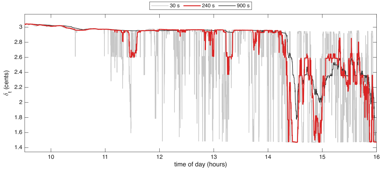
Figure 2: The Huber threshold \delta_t in cents for MU on 16 October 2024, with half-lives of 30, 240, 900 seconds. The 240-second half-life, in red, is used.
