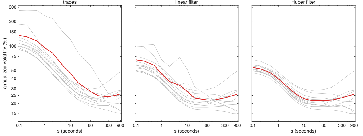
Figure 4: Volatility signature curves for NFLX over the 12 trading days in Oct 2024. The annualized vol \hat{\sigma}100\sqrt{252} from the returns \hat{X}_t - \hat{X}_{t,s} of Table 2, against the lag s in seconds, both axes on log scales, for: raw trades, linear filter & Huber filter. Grey lines are the individual trading days & the red line is the square root of the 12 day average of their squares. The linear & Huber returns carry the finite-sample correction c_{t,s} of the paper; the raw trades are unaffected by it.
