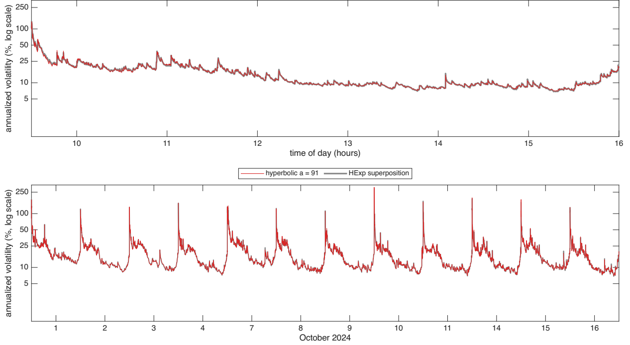
Figure 6: Hyperbolic against superposition weights for NFLX over 12 trading days in Oct 2024, the diurnally adjusted \hat{\sigma}(u)100\sqrt{252} at s = 1 second from the Huber filter, shown as annualized vol in % on a log10 scale. The only difference between the 2 paths is the weight function: the hyperbolic weights with a = 91 in red, drawn on top, and the HExp superposition in grey, 4 exponential components with half lives of 10, 100, 1000, 10000 seconds. Hyperparameters minimize the QLIKE objective. Top: 16 October 2024, bottom: 12 days.
