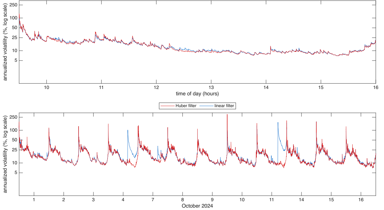
Figure 5: Filtered spot volatility for NFLX over 12 trading days in Oct 2024, the diurnally adjusted estimator \hat{\sigma}(u)100\sqrt{252} at s = 1 second with hyperbolic weights, Mandelbrot parameter a = 91 , with the input prices computed using the Huber & linear filters, shown as annualized volatility in percent on a log10 scale. Top: 16 October 2024, bottom: 12 days.
