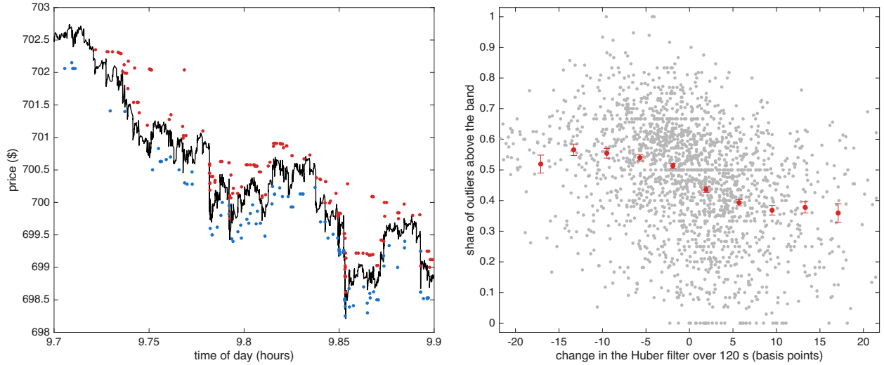
Figure 7: Outliers & robust price for NFLX on 16 October 2024. Left: the 12 minutes with the largest move in the Huber filter that day; outliers above Y_t - \theta_t > \delta_{t-1} in red, outliers below Y_t - \theta_t < -\delta_{t-1} in blue, Huber filter in black. Right: over the 12 trading days, the 120 second empirical conditional probability that outliers are above (rather than below) the Huber band against the 120 second change in the Huber filter in basis points: light points are single bins, the line & bars are means & s.e.
