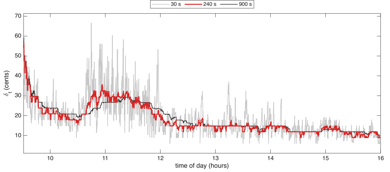
Figure 2: The Huber threshold \delta_t in cents for NFLX on 16 October 2024, with half-lives of 30, 240, 900 seconds. The 240-second half-life, in red, is used.
