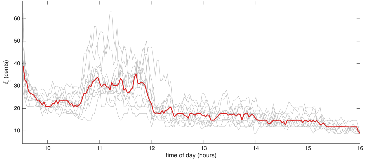
Figure 3: Huber threshold \delta_t in cents through the trading day, for 12 NFLX trading days in Oct 2024 (grey lines) and their median (red line).
