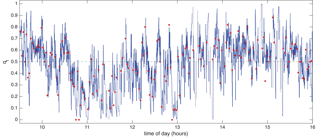
Figure 8: The directional conditional probability for NFLX, 16 October 2024. The filtered conditional probability q_t that an outlier lies above the robust Huber band, under exponential weights decaying in clock time with half life of 30 seconds; where fewer than two outliers remain in the weights it is drawn in grey. The dashed line marks 0.5. The red points are the empirical conditional probability using the 120 second bins of the previous figure.
