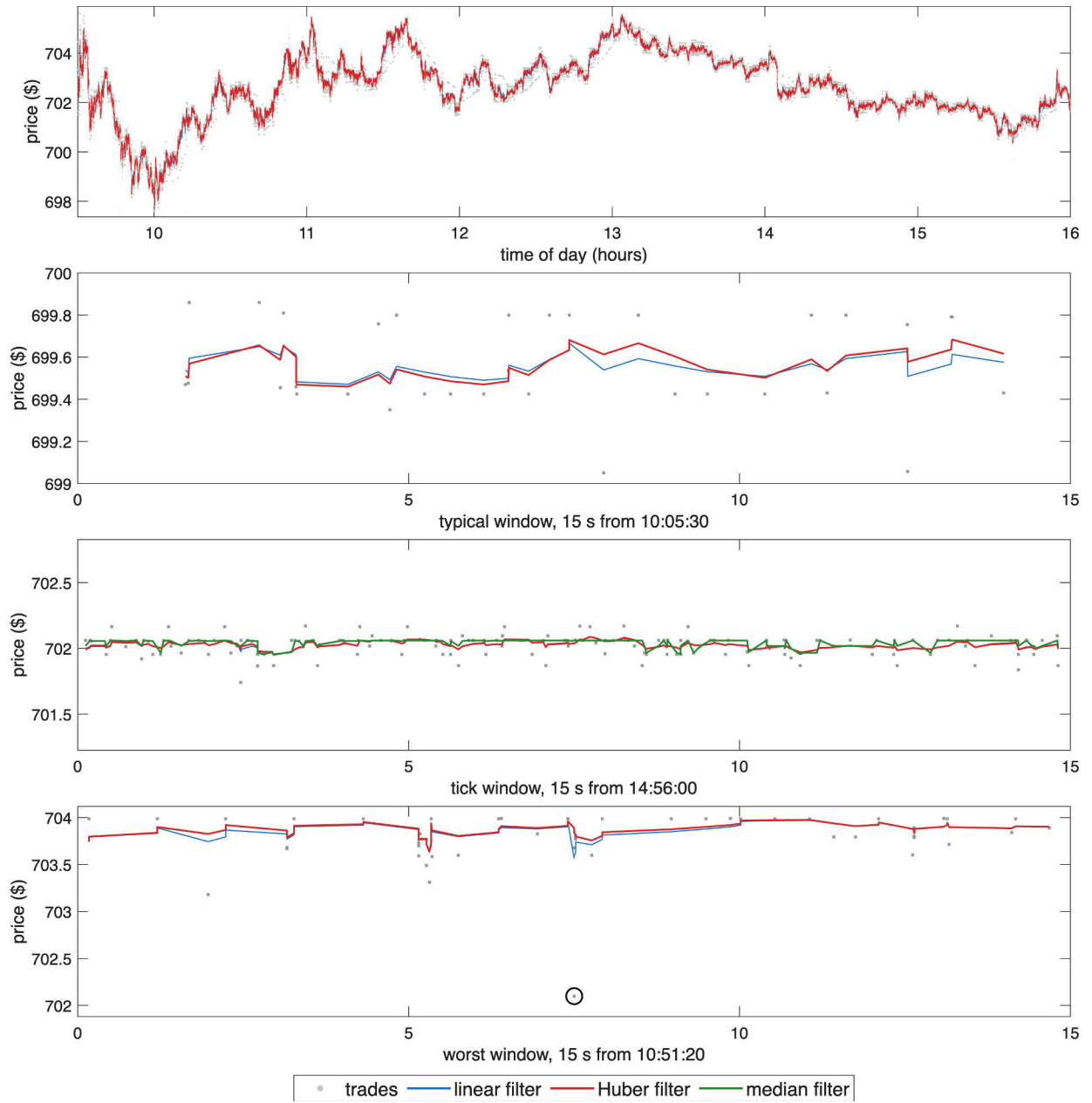
Figure 1: NFLX trades (grey points), the linear filter and the Huber filter, 16 October 2024. Top: full trading day. 2nd: 15-second window at the day's median trade count, from 10:05:30. 3rd: 15-second window at 14:56:00 in which the price reverses direction most often, with the median filter m_t added. Bottom: 15-second window around the largest Huber residual after 09:45, circled.
