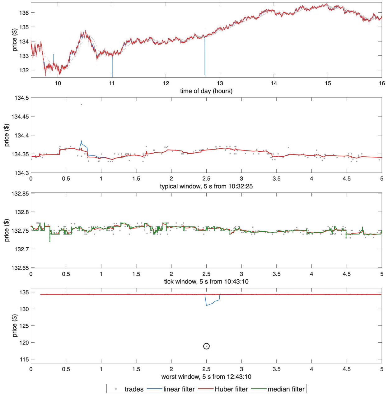
Figure 1: NVDA trades (grey points), the linear filter and the Huber filter, 16 October 2024. Top: full trading day. 2nd: 5-second window at the day's median trade count, from 10:32:25. 3rd: 5-second window at 10:43:10 in which the price reverses direction most often, with the median filter m_t added. Bottom: 5-second window around the largest Huber residual after 09:45, circled.
