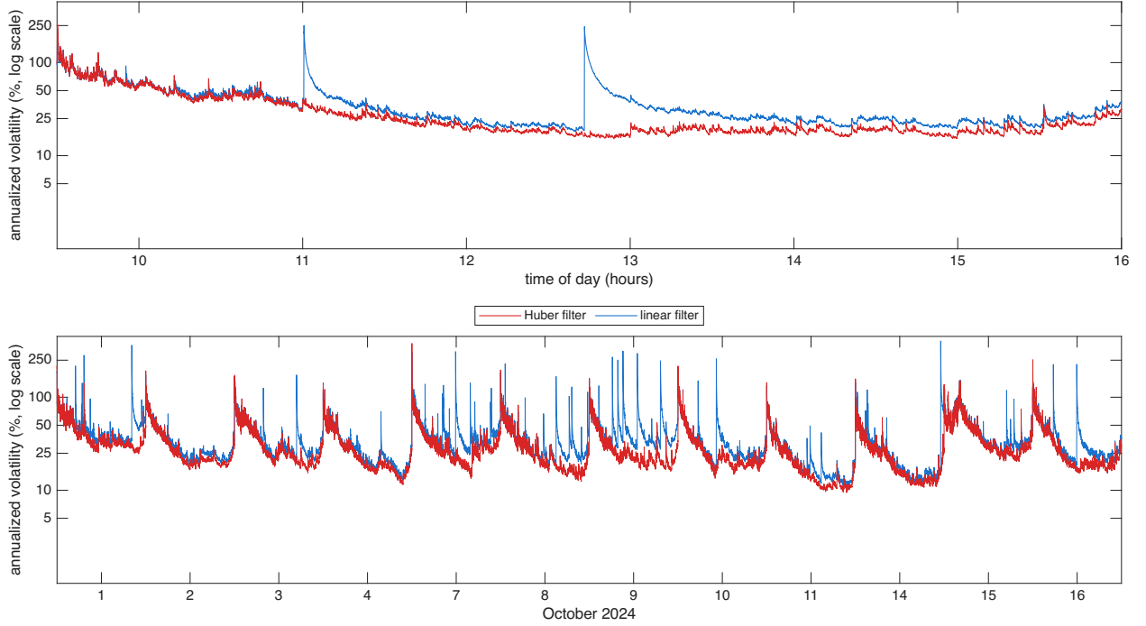
Figure 5: Filtered spot volatility for NVDA over 12 trading days in Oct 2024, the diurnally adjusted estimator \hat{\sigma}(u)100\sqrt{252} at s = 1 second with hyperbolic weights, Mandelbrot parameter a = 563 , with the input prices computed using the Huber & linear filters, shown as annualized volatility in percent on a log10 scale. Top: 16 October 2024, bottom: 12 days.
