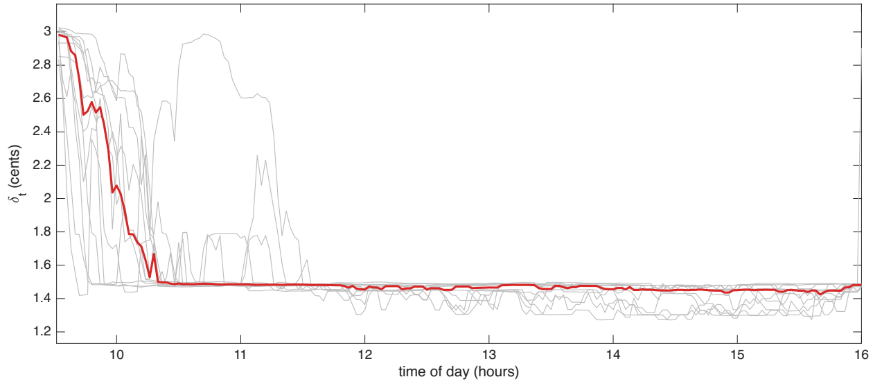
Figure 3: Huber threshold \delta_t in cents through the trading day, for 12 NVDA trading days in Oct 2024 (grey lines) and their median (red line).
