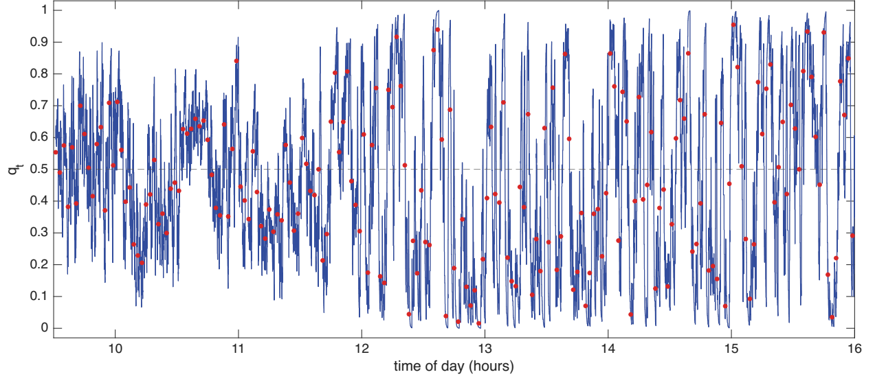
Figure 8: The directional conditional probability for NVDA, 16 October 2024. The filtered conditional probability q_t that an outlier lies above the robust Huber band, under exponential weights decaying in clock time with half life of 13 seconds; where fewer than two outliers remain in the weights it is drawn in grey. The dashed line marks 0.5. The red points are the empirical conditional probability using the 120 second bins of the previous figure.
