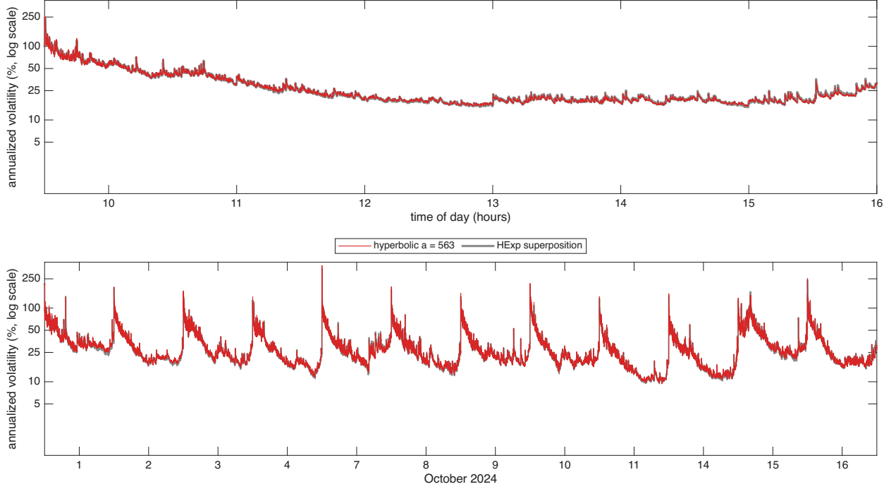
Figure 6: Hyperbolic against superposition weights for NVDA over 12 trading days in Oct 2024, the diurnally adjusted \hat{\sigma}(u)100\sqrt{252} at s = 1 second from the Huber filter, shown as annualized vol in % on a log10 scale. The only difference between the 2 paths is the weight function: the hyperbolic weights with a = 563 in red, drawn on top, and the HExp superposition in grey, 4 exponential components with half lives of 2, 20, 200, 2000 seconds. Hyperparameters minimize the QLIKE objective. Top: 16 October 2024, bottom: 12 days.
