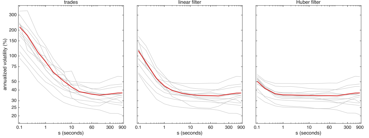
Figure 4: Volatility signature curves for NVDA over the 12 trading days in Oct 2024. The annualized vol \hat{\sigma}100\sqrt{252} from the returns \hat{X}_t - \hat{X}_{t,s} of Table 2, against the lag s in seconds, both axes on log scales, for: raw trades, linear filter & Huber filter. Grey lines are the individual trading days & the red line is the square root of the 12 day average of their squares. The linear & Huber returns carry the finite-sample correction c_{t,s} of the paper; the raw trades are unaffected by it.
