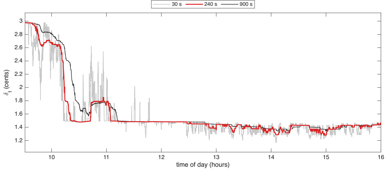
Figure 2: The Huber threshold \delta_t in cents for NVDA on 16 October 2024, with half-lives of 30, 240, 900 seconds. The 240-second half-life, in red, is used.
