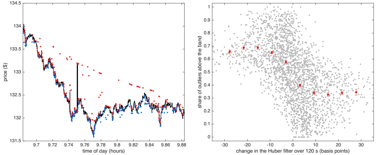
Figure 7: Outliers & robust price for NVDA on 16 October 2024. Left: the 12 minutes with the largest move in the Huber filter that day; outliers above Y_t - \theta_t > \delta_{t-1} in red, outliers below Y_t - \theta_t < -\delta_{t-1} in blue, Huber filter in black. Right: over the 12 trading days, the 120 second empirical conditional probability that outliers are above (rather than below) the Huber band against the 120 second change in the Huber filter in basis points: light points are single bins, the line & bars are means & s.e.
