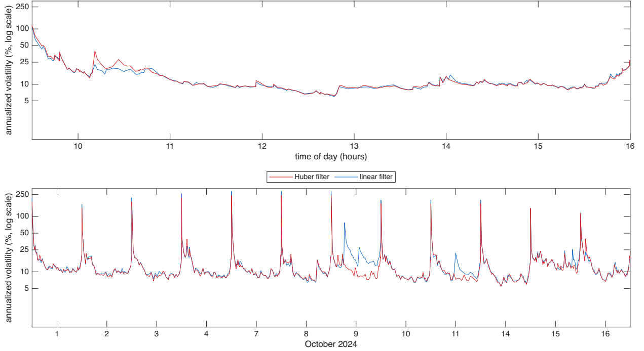
Figure 5: Filtered spot volatility for ORLY over 12 trading days in Oct 2024, the diurnally adjusted estimator \hat{\sigma}(u)100\sqrt{252} at s = 1 second with hyperbolic weights, Mandelbrot parameter a = 23 , with the input prices computed using the Huber & linear filters, shown as annualized volatility in percent on a log10 scale. Top: 16 October 2024, bottom: 12 days.
