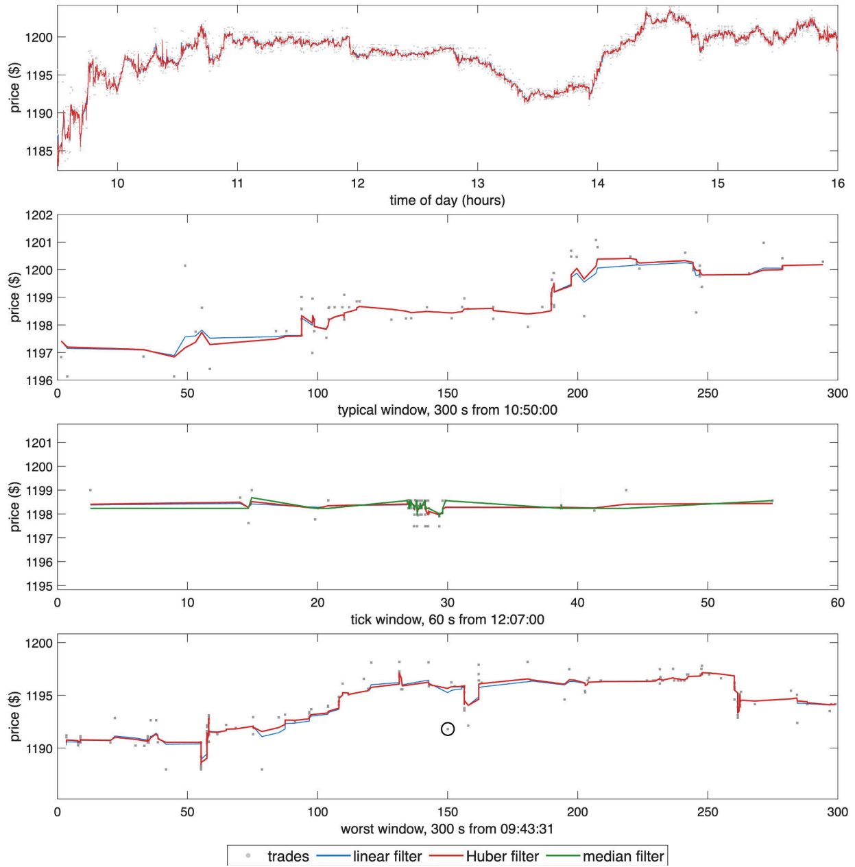
Figure 1: ORLY trades (grey points), the linear filter and the Huber filter, 16 October 2024. Top: full trading day. 2nd: 300-second window at the day's median trade count, from 10:50:00. 3rd: 60-second window at 12:07:00 in which the price reverses direction most often, with the median filter m_t added. Bottom: 300-second window around the largest Huber residual after 09:45, circled.
