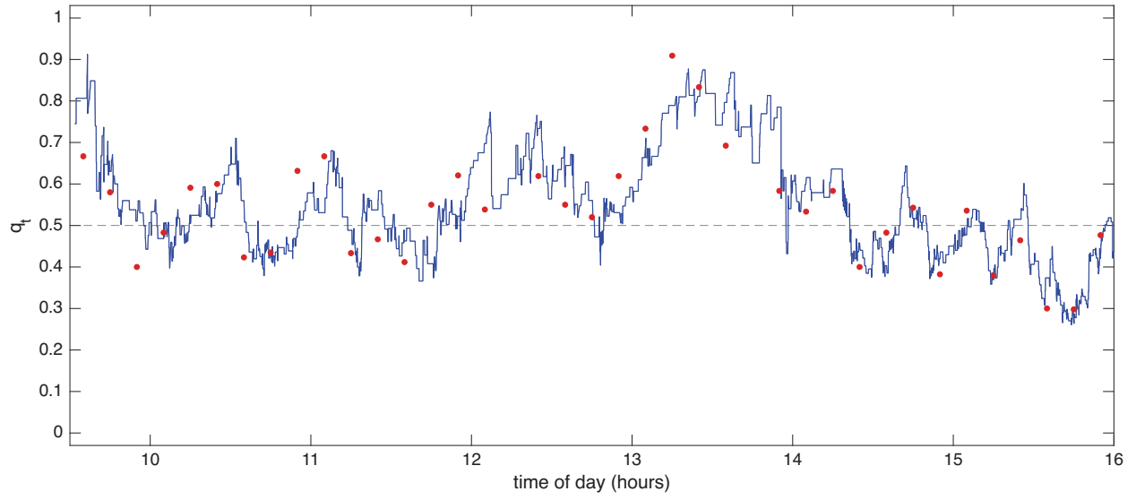
Figure 8: The directional conditional probability for ORLY , 16 October 2024. The filtered conditional probability q_t that an outlier lies above the robust Huber band, under exponential weights decaying in clock time with half life of 335 seconds; where fewer than two outliers remain in the weights it is drawn in grey. The dashed line marks 0.5. The red points are the empirical conditional probability using the 600 second bins of the previous figure.
