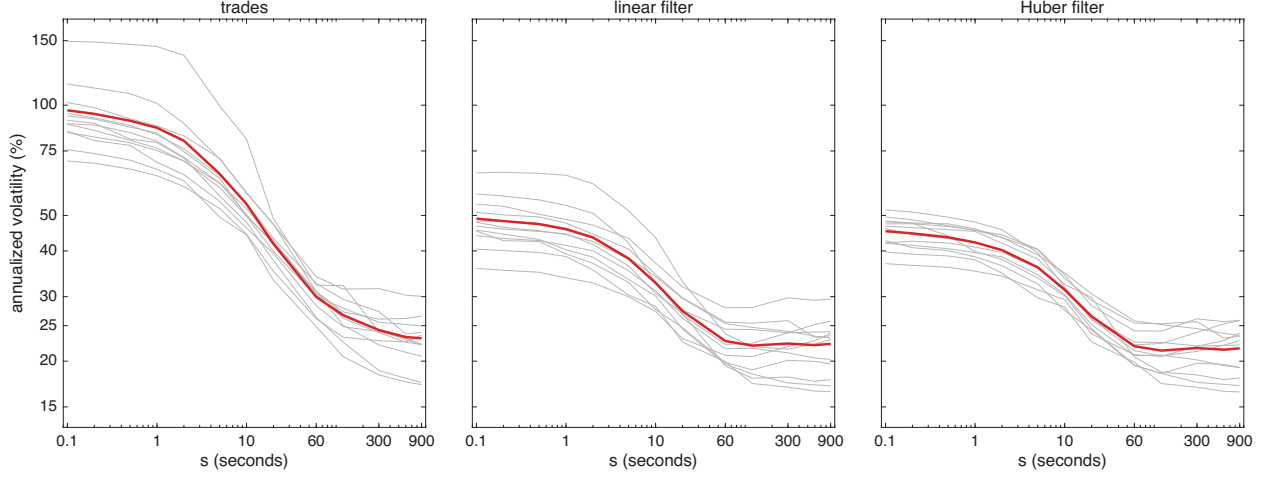
Figure 4: Volatility signature curves for ORLY over the 12 trading days in Oct 2024. The annualized vol \hat{\sigma}100\sqrt{252} from the returns \hat{X}_t - \hat{X}_{t,s} of Table 2, against the lag s in seconds, both axes on log scales, for: raw trades, linear filter & Huber filter. Grey lines are the individual trading days & the red line is the square root of the 12 day average of their squares. The linear & Huber returns carry the finite-sample correction c_{t,s} of the paper; the raw trades are unaffected by it.
