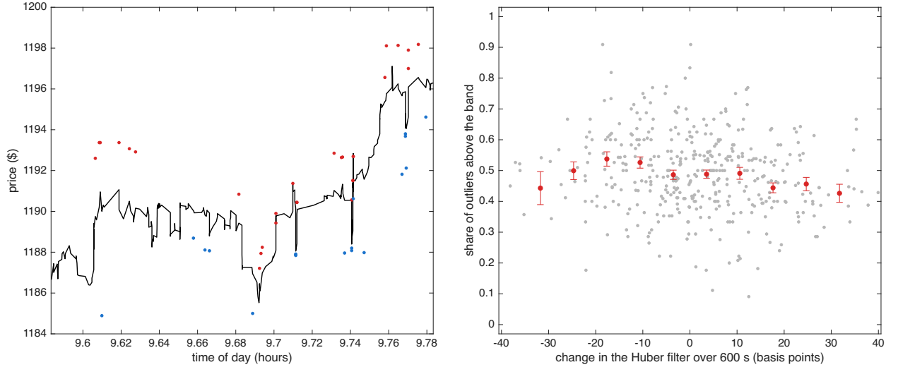
Figure 7: Outliers & robust price for ORLY on 16 October 2024. Left: the 12 minutes with the largest move in the Huber filter that day; outliers above Y_t - \theta_t > \delta_{t-1} in red, outliers below Y_t - \theta_t < -\delta_{t-1} in blue, Huber filter in black. Right: over the 12 trading days, the 600 second empirical conditional probability that outliers are above (rather than below) the Huber band against the 600 second change in the Huber filter in basis points: light points are single bins, the line & bars are means & s.e.
