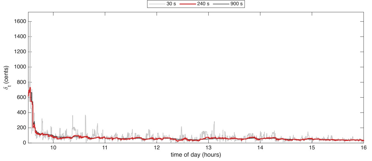
Figure 2: The Huber threshold \delta_t in cents for ORLY on 16 October 2024, with half-lives of 30, 240, 900 seconds. The 240-second half-life, in red, is used.
