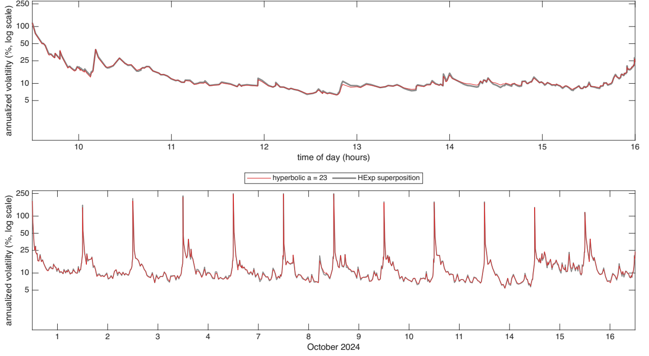
Figure 6: Hyperbolic against superposition weights for ORLY over 12 trading days in Oct 2024, the diurnally adjusted \hat{\sigma}(u)100\sqrt{252} at s = 1 second from the Huber filter, shown as annualized vol in % on a log10 scale. The only difference between the 2 paths is the weight function: the hyperbolic weights with a = 23 in red, drawn on top, and the HExp superposition in grey, 4 exponential components with half lives of 10, 100, 1000, 10000 seconds. Hyperparameters minimize the QLIKE objective. Top: 16 October 2024, bottom: 12 days.
