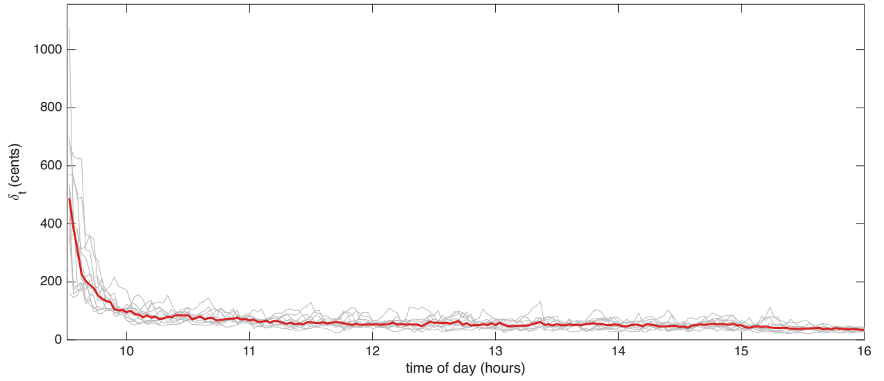
Figure 3: Huber threshold \delta_t in cents through the trading day, for 12 ORLY trading days in Oct 2024 (grey lines) and their median (red line).
