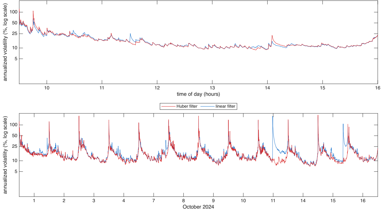
Figure 5: Filtered spot volatility for PANW over 12 trading days in Oct 2024, the diurnally adjusted estimator \hat{\sigma}(u)100\sqrt{252} at s = 1 second with hyperbolic weights, Mandelbrot parameter a = 59 , with the input prices computed using the Huber & linear filters, shown as annualized volatility in percent on a log10 scale. Top: 16 October 2024, bottom: 12 days.
