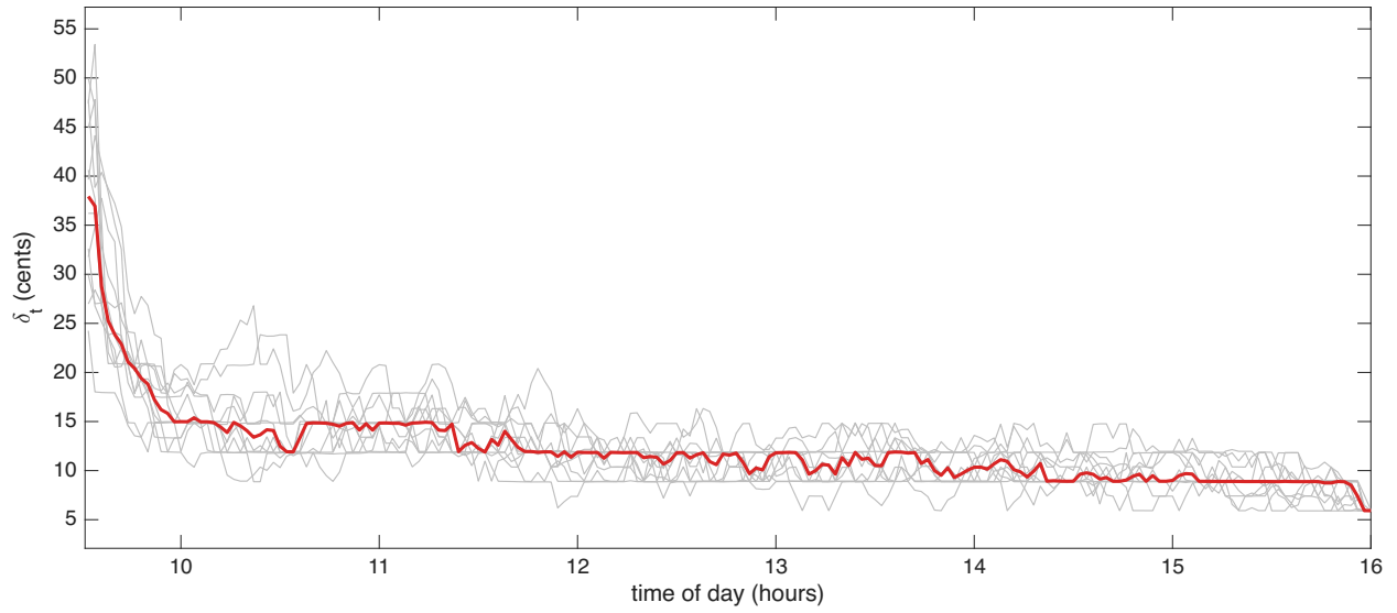
Figure 3: Huber threshold \delta_t in cents through the trading day, for 12 PANW trading days in Oct 2024 (grey lines) and their median (red line).
