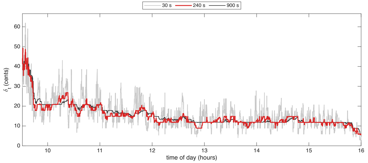
Figure 2: The Huber threshold \delta_t in cents for PANW on 16 October 2024, with half-lives of 30, 240, 900 seconds. The 240-second half-life, in red, is used.
