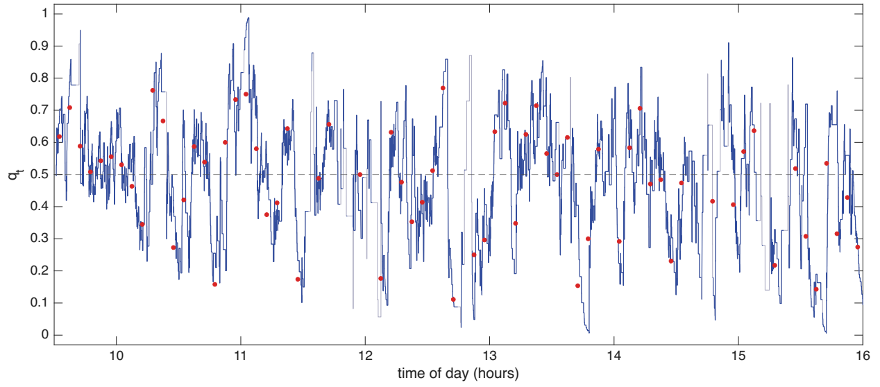
Figure 8: The directional conditional probability for PANW, 16 October 2024. The filtered conditional probability q_t that an outlier lies above the robust Huber band, under exponential weights decaying in clock time with half life of 60 seconds; where fewer than two outliers remain in the weights it is drawn in grey. The dashed line marks 0.5. The red points are the empirical conditional probability using the 300 second bins of the previous figure.
