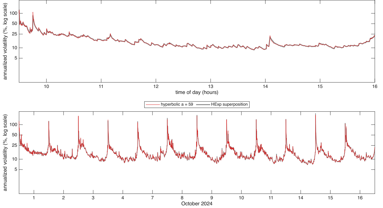
Figure 6: Hyperbolic against superposition weights for PANW over 12 trading days in Oct 2024, the diurnally adjusted \hat{\sigma}(u)100\sqrt{252} at s = 1 second from the Huber filter, shown as annualized vol in % on a log10 scale. The only difference between the 2 paths is the weight function: the hyperbolic weights with a = 59 in red, drawn on top, and the HExp superposition in grey, 4 exponential components with half lives of 60, 600, 3600, 23400 seconds. Hyperparameters minimize the QLIKE objective. Top: 16 October 2024, bottom: 12 days.
