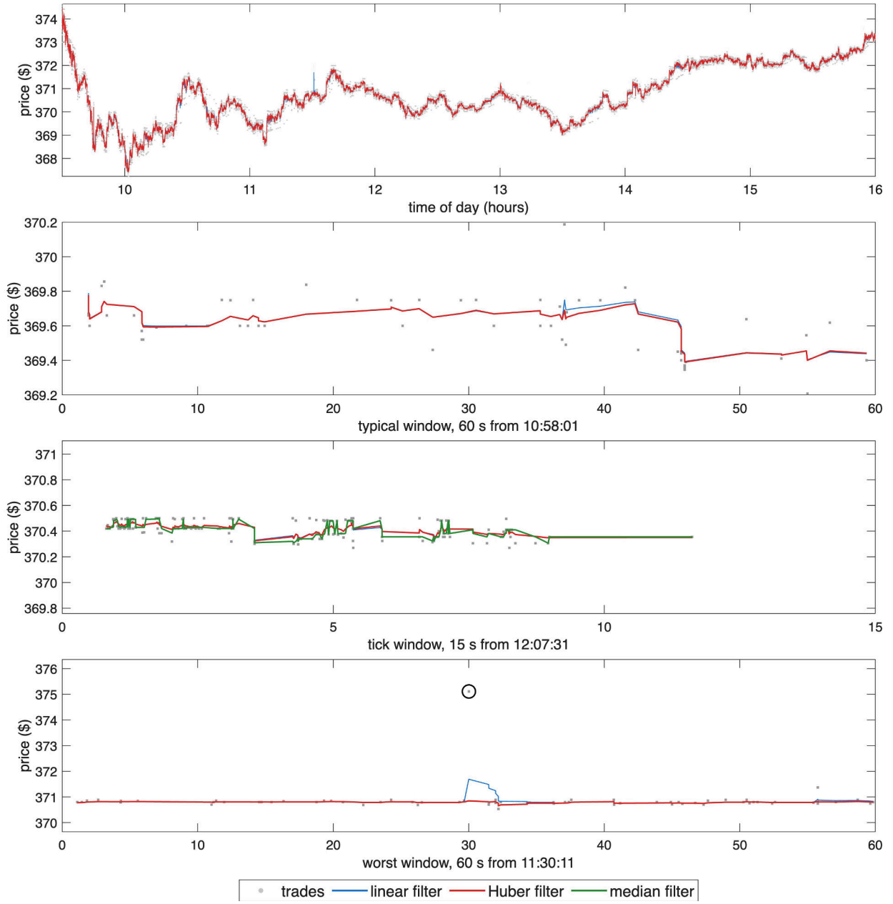
Figure 1: PANW trades (grey points), the linear filter and the Huber filter, 16 October 2024. Top: full trading day. 2nd: 60-second window at the day's median trade count, from 10:58:01. 3rd: 15-second window at 12:07:31 in which the price reverses direction most often, with the median filter m_t added. Bottom: 60-second window around the largest Huber residual after 09:45, circled.
