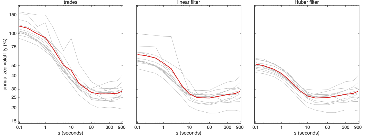
Figure 4: Volatility signature curves for PANW over the 12 trading days in Oct 2024. The annualized vol \hat{\sigma}100\sqrt{252} from the returns \hat{X}_t - \hat{X}_{t,s} of Table 2, against the lag s in seconds, both axes on log scales, for: raw trades, linear filter & Huber filter. Grey lines are the individual trading days & the red line is the square root of the 12 day average of their squares. The linear & Huber returns carry the finite-sample correction c_{t,s} of the paper; the raw trades are unaffected by it.
