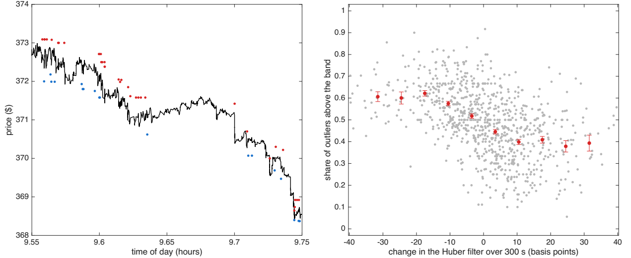
Figure 7: Outliers & robust price for PANW on 16 October 2024. Left: the 12 minutes with the largest move in the Huber filter that day; outliers above Y_t - \theta_t > \delta_{t-1} in red, outliers below Y_t - \theta_t < -\delta_{t-1} in blue, Huber filter in black. Right: over the 12 trading days, the 300 second empirical conditional probability that outliers are above (rather than below) the Huber band against the 300 second change in the Huber filter in basis points: light points are single bins, the line & bars are means & s.e.
