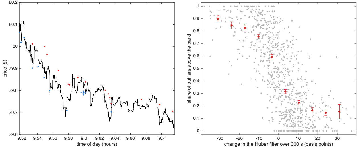
Figure 7: Outliers & robust price for PYPL on 16 October 2024. Left: the 12 minutes with the largest move in the Huber filter that day; outliers above Y_t - \theta_t > \delta_{t-1} in red, outliers below Y_t - \theta_t < -\delta_{t-1} in blue, Huber filter in black. Right: over the 12 trading days, the 300 second empirical conditional probability that outliers are above (rather than below) the Huber band against the 300 second change in the Huber filter in basis points: light points are single bins, the line & bars are means & s.e.
