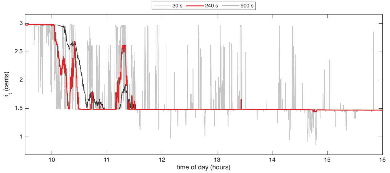
Figure 2: The Huber threshold \delta_t in cents for PYPL on 16 October 2024, with half-lives of 30, 240, 900 seconds. The 240-second half-life, in red, is used.
