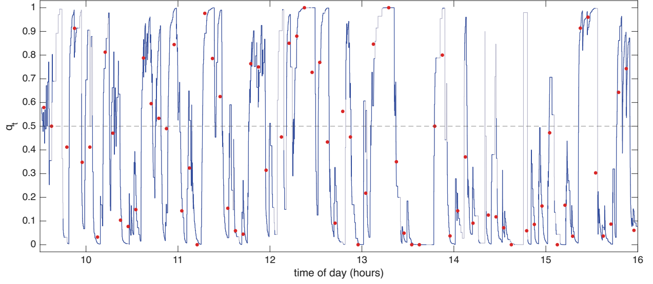
Figure 8: The directional conditional probability for PYPL, 16 October 2024. The filtered conditional probability q_t that an outlier lies above the robust Huber band, under exponential weights decaying in clock time with half life of 42 seconds; where fewer than two outliers remain in the weights it is drawn in grey. The dashed line marks 0.5. The red points are the empirical conditional probability using the 300 second bins of the previous figure.
