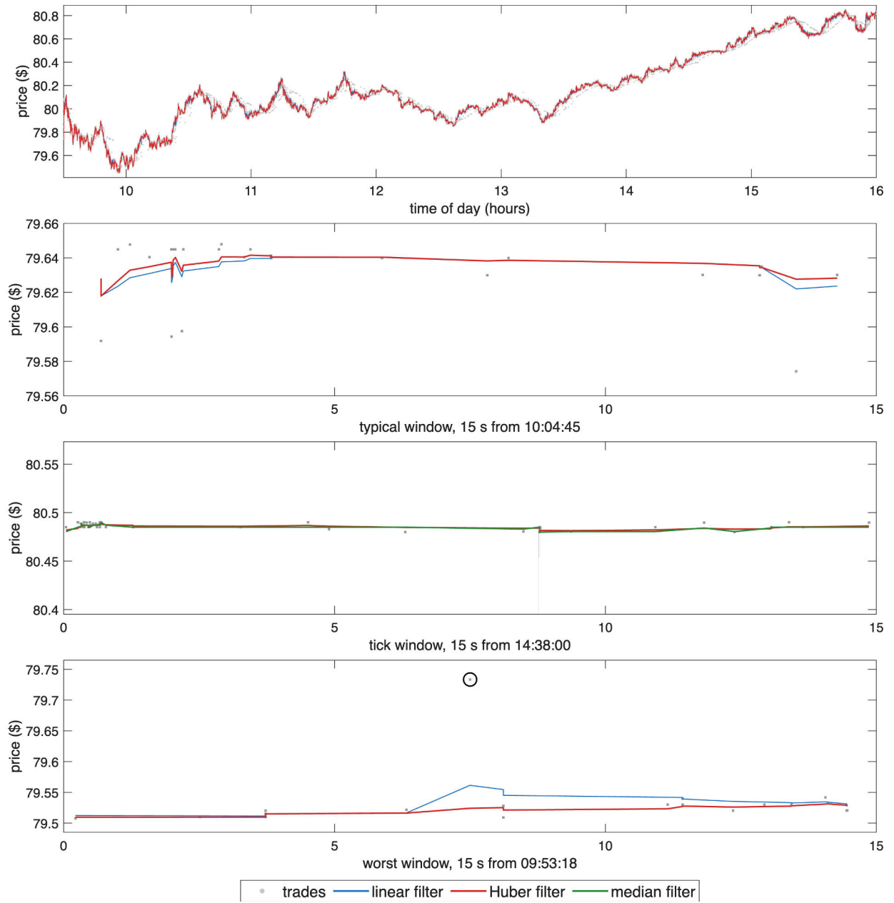
Figure 1: PYPL trades (grey points), the linear filter and the Huber filter, 16 October 2024. Top: full trading day. 2nd: 15-second window at the day's median trade count, from 10:04:45. 3rd: 15-second window at 14:38:00 in which the price reverses direction most often, with the median filter m_t added. Bottom: 15-second window around the largest Huber residual after 09:45, circled.
