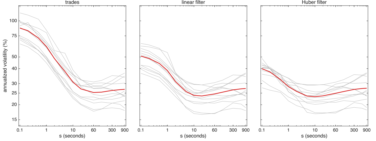
Figure 4: Volatility signature curves for PYPL over the 12 trading days in Oct 2024. The annualized vol \hat{\sigma}100\sqrt{252} from the returns \hat{X}_t - \hat{X}_{t,s} of Table 2, against the lag s in seconds, both axes on log scales, for: raw trades, linear filter & Huber filter. Grey lines are the individual trading days & the red line is the square root of the 12 day average of their squares. The linear & Huber returns carry the finite-sample correction c_{t,s} of the paper; the raw trades are unaffected by it.
