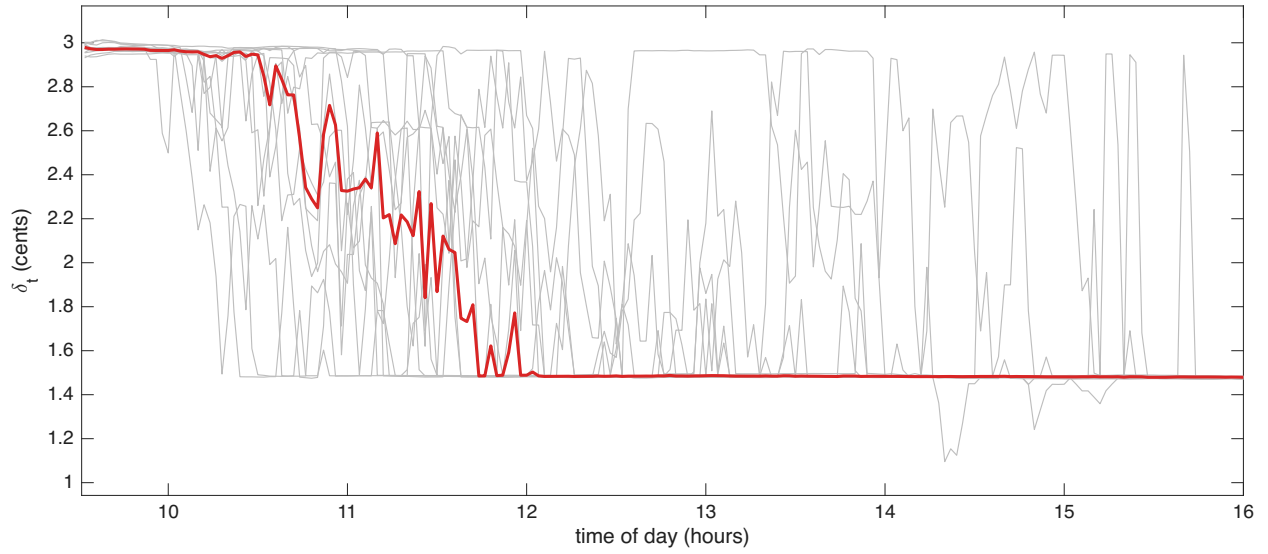
Figure 3: Huber threshold \delta_t in cents through the trading day, for 12 PYPL trading days in Oct 2024 (grey lines) and their median (red line).
