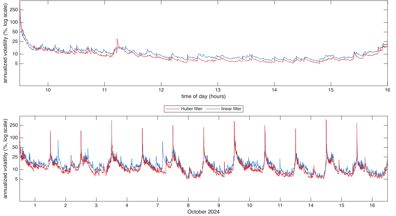
Figure 5: Filtered spot volatility for PYPL over 12 trading days in Oct 2024, the diurnally adjusted estimator \hat{\sigma}(u)100\sqrt{252} at s = 1 second with hyperbolic weights, Mandelbrot parameter a = 95 , with the input prices computed using the Huber & linear filters, shown as annualized volatility in percent on a log10 scale. Top: 16 October 2024, bottom: 12 days.
