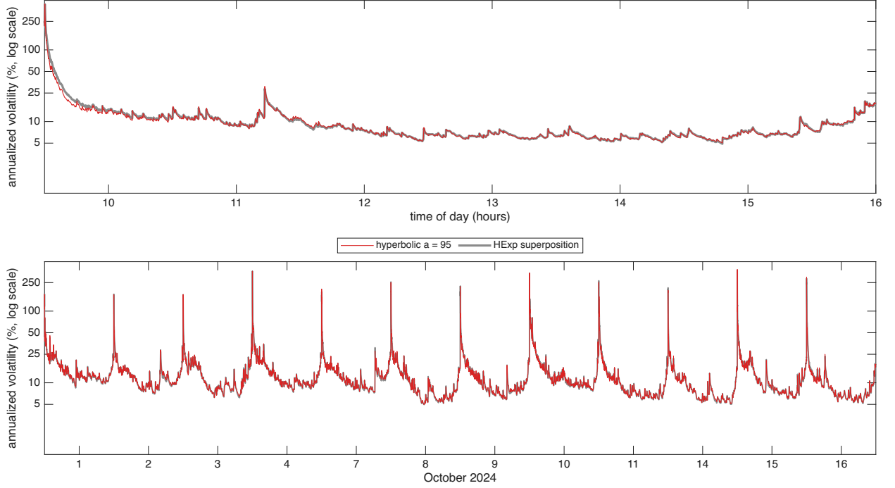
Figure 6: Hyperbolic against superposition weights for PYPL over 12 trading days in Oct 2024, the diurnally adjusted \hat{\sigma}(u)100\sqrt{252} at s = 1 second from the Huber filter, shown as annualized vol in % on a log10 scale. The only difference between the 2 paths is the weight function: the hyperbolic weights with a = 95 in red, drawn on top, and the HExp superposition in grey, 4 exponential components with half lives of 10, 100, 1000, 10000 seconds. Hyperparameters minimize the QLIKE objective. Top: 16 October 2024, bottom: 12 days.
