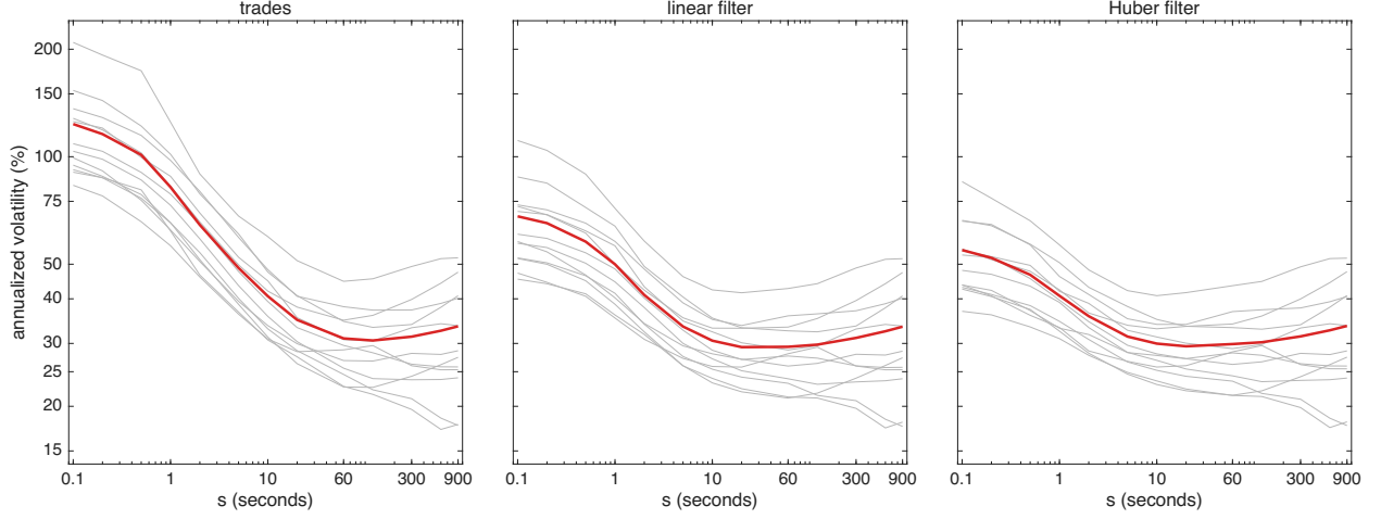
Figure 4: Volatility signature curves for QCOM over the 12 trading days in Oct 2024. The annualized vol \hat{\sigma}100\sqrt{252} from the returns \hat{X}_t - \hat{X}_{t,s} of Table 2, against the lag s in seconds, both axes on log scales, for: raw trades, linear filter & Huber filter. Grey lines are the individual trading days & the red line is the square root of the 12 day average of their squares. The linear & Huber returns carry the finite-sample correction c_{t,s} of the paper; the raw trades are unaffected by it.
