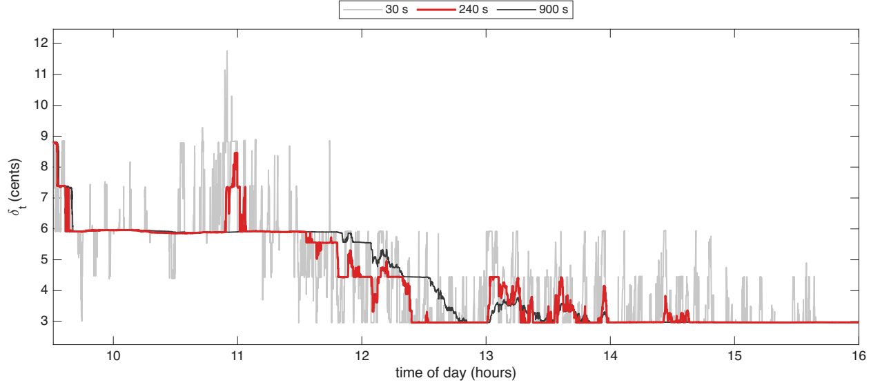
Figure 2: The Huber threshold \delta_t in cents for QCOM on 16 October 2024, with half-lives of 30, 240, 900 seconds. The 240-second half-life, in red, is used.
