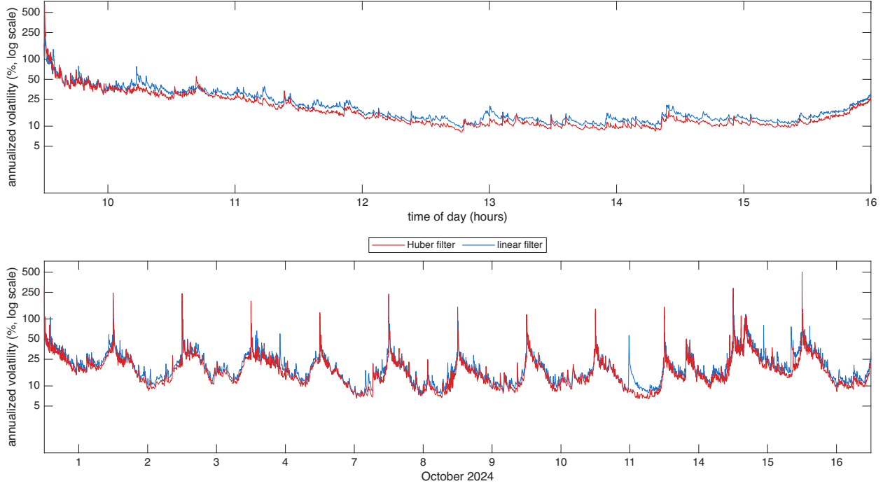
Figure 5: Filtered spot volatility for QCOM over 12 trading days in Oct 2024, the diurnally adjusted estimator \hat{\sigma}(u)100\sqrt{252} at s = 1 second with hyperbolic weights, Mandelbrot parameter a = 39 , with the input prices computed using the Huber & linear filters, shown as annualized volatility in percent on a log10 scale. Top: 16 October 2024, bottom: 12 days.
