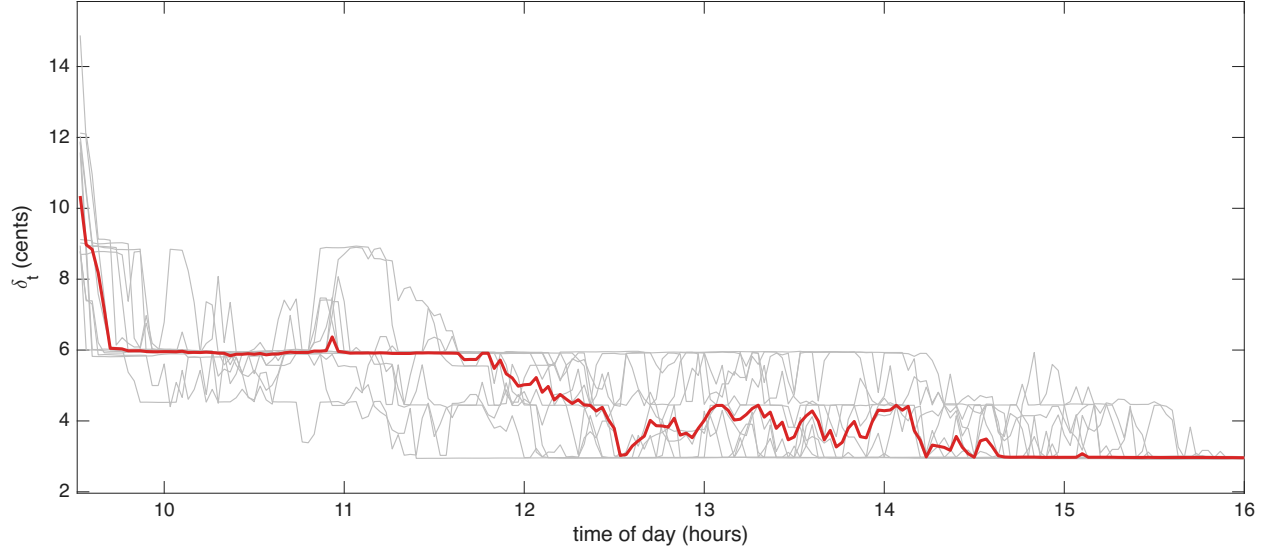
Figure 3: Huber threshold \delta_t in cents through the trading day, for 12 QCOM trading days in Oct 2024 (grey lines) and their median (red line).
