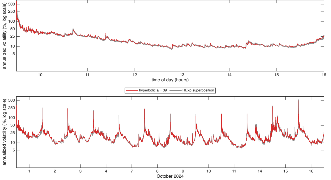
Figure 6: Hyperbolic against superposition weights for QCOM over 12 trading days in Oct 2024, the diurnally adjusted \hat{\sigma}(u)100\sqrt{252} at s = 1 second from the Huber filter, shown as annualized vol in % on a log10 scale. The only difference between the 2 paths is the weight function: the hyperbolic weights with a = 39 in red, drawn on top, and the HExp superposition in grey, 4 exponential components with half lives of 30, 150, 750, 3750 seconds. Hyperparameters minimize the QLIKE objective. Top: 16 October 2024, bottom: 12 days.
