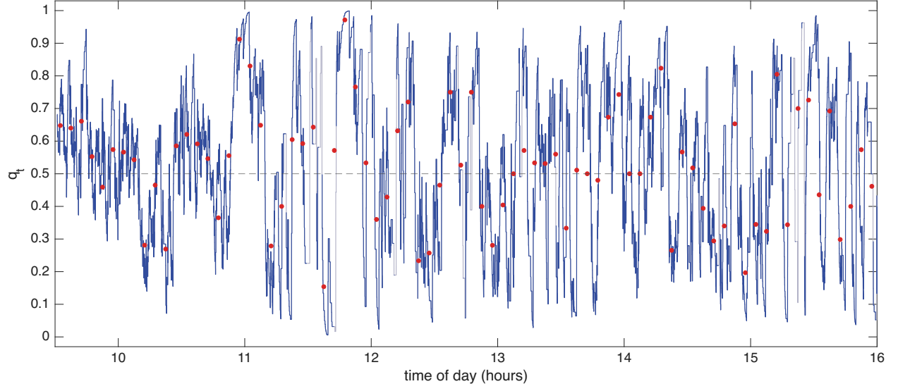
Figure 8: The directional conditional probability for QCOM , 16 October 2024. The filtered conditional probability q_t that an outlier lies above the robust Huber band, under exponential weights decaying in clock time with half life of 33 seconds; where fewer than two outliers remain in the weights it is drawn in grey. The dashed line marks 0.5. The red points are the empirical conditional probability using the 300 second bins of the previous figure.
