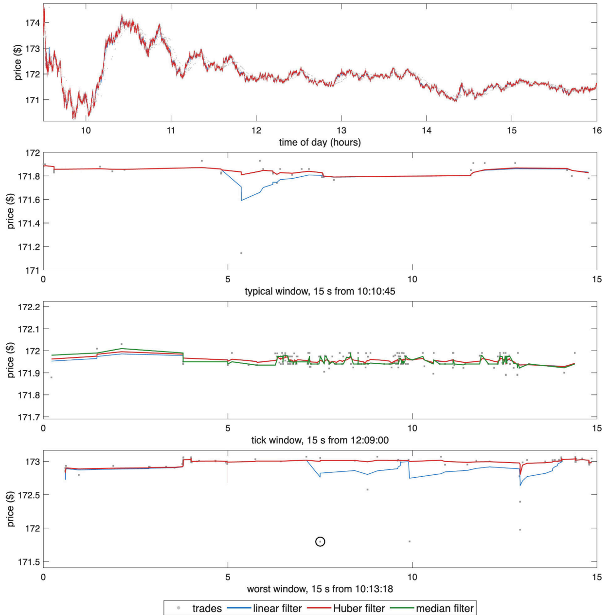
Figure 1: QCOM trades (grey points), the linear filter and the Huber filter, 16 October 2024. Top: full trading day. 2nd: 15-second window at the day's median trade count, from 10:10:45. 3rd: 15-second window at 12:09:00 in which the price reverses direction most often, with the median filter m_t added. Bottom: 15-second window around the largest Huber residual after 09:45, circled.
