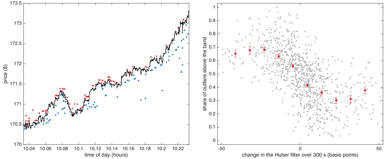
Figure 7: Outliers & robust price for QCOM on 16 October 2024. Left: the 12 minutes with the largest move in the Huber filter that day; outliers above Y_t - \theta_t > \delta_{t-1} in red, outliers below Y_t - \theta_t < -\delta_{t-1} in blue, Huber filter in black. Right: over the 12 trading days, the 300 second empirical conditional probability that outliers are above (rather than below) the Huber band against the 300 second change in the Huber filter in basis points: light points are single bins, the line & bars are means & s.e.
