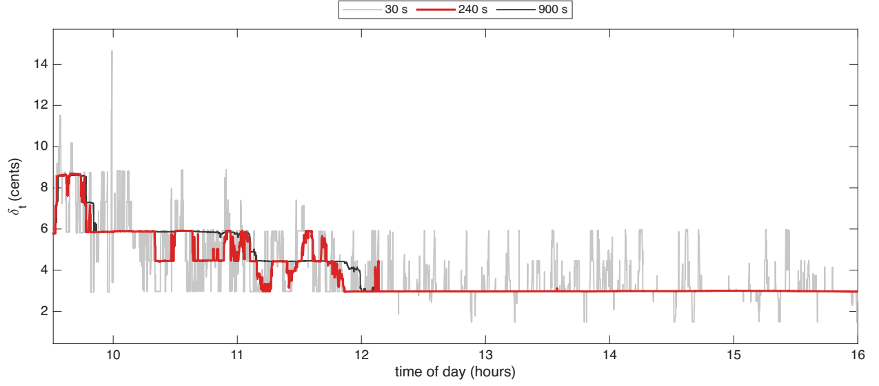
Figure 2: The Huber threshold \delta_t in cents for ROKU on 16 October 2024, with half-lives of 30, 240, 900 seconds. The 240-second half-life, in red, is used.
