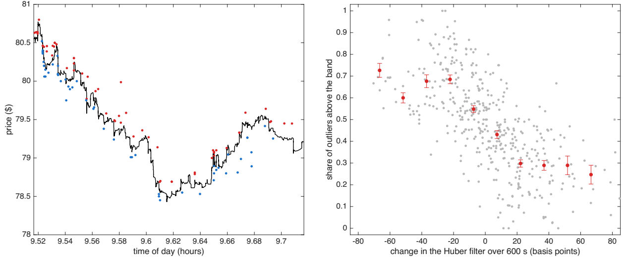
Figure 7: Outliers & robust price for ROKU on 16 October 2024. Left: the 12 minutes with the largest move in the Huber filter that day; outliers above Y_t - \theta_t > \delta_{t-1} in red, outliers below Y_t - \theta_t < -\delta_{t-1} in blue, Huber filter in black. Right: over the 12 trading days, the 600 second empirical conditional probability that outliers are above (rather than below) the Huber band against the 600 second change in the Huber filter in basis points: light points are single bins, the line & bars are means & s.e.
