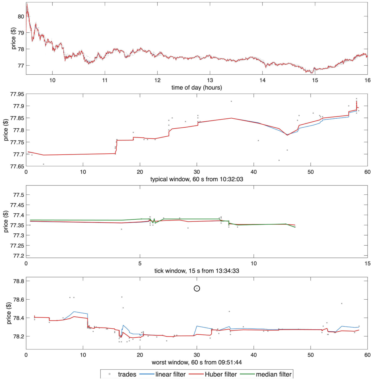
Figure 1: ROKU trades (grey points), the linear filter and the Huber filter, 16 October 2024. Top: full trading day. 2nd: 60-second window at the day's median trade count, from 10:32:03. 3rd: 15-second window at 13:34:33 in which the price reverses direction most often, with the median filter m_t added. Bottom: 60-second window around the largest Huber residual after 09:45, circled.
