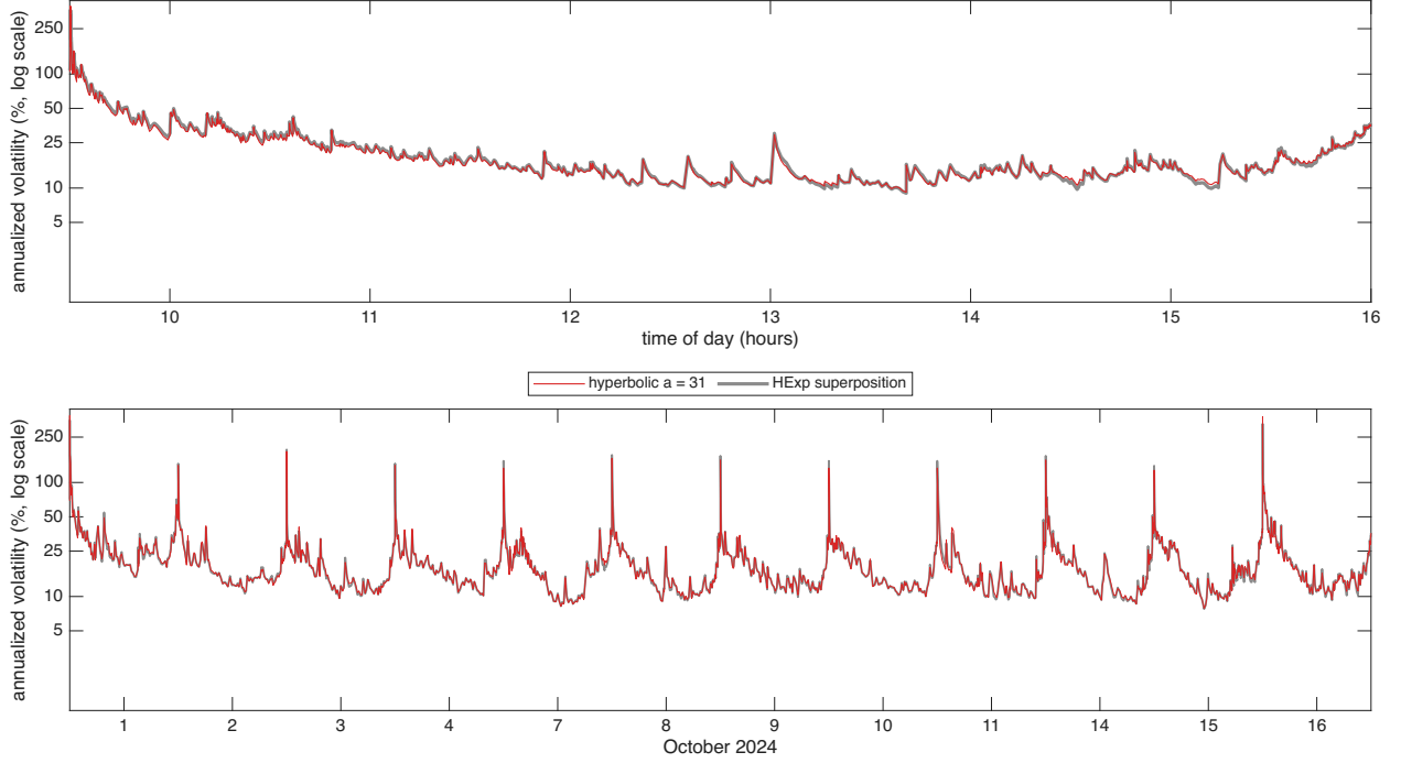
Figure 6: Hyperbolic against superposition weights for ROKU over 12 trading days in Oct 2024, the diurnally adjusted \hat{\sigma}(u)100\sqrt{252} at s = 1 second from the Huber filter, shown as annualized vol in % on a log10 scale. The only difference between the 2 paths is the weight function: the hyperbolic weights with a = 31 in red, drawn on top, and the HExp superposition in grey, 4 exponential components with half lives of 10, 100, 1000, 10000 seconds. Hyperparameters minimize the QLIKE objective. Top: 16 October 2024, bottom: 12 days.
