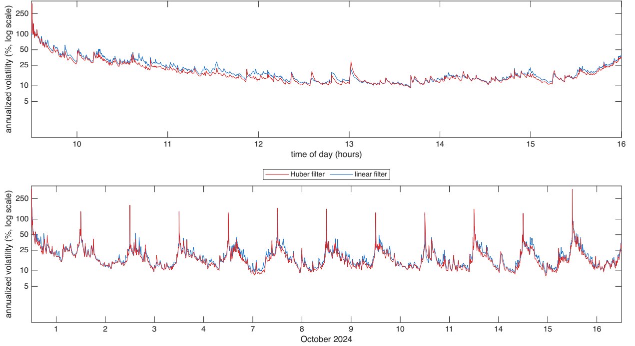
Figure 5: Filtered spot volatility for ROKU over 12 trading days in Oct 2024, the diurnally adjusted estimator \hat{\sigma}(u)100\sqrt{252} at s = 1 second with hyperbolic weights, Mandelbrot parameter a = 31 , with the input prices computed using the Huber & linear filters, shown as annualized volatility in percent on a log10 scale. Top: 16 October 2024, bottom: 12 days.
