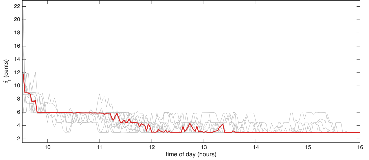
Figure 3: Huber threshold \delta_t in cents through the trading day, for 12 ROKU trading days in Oct 2024 (grey lines) and their median (red line).
