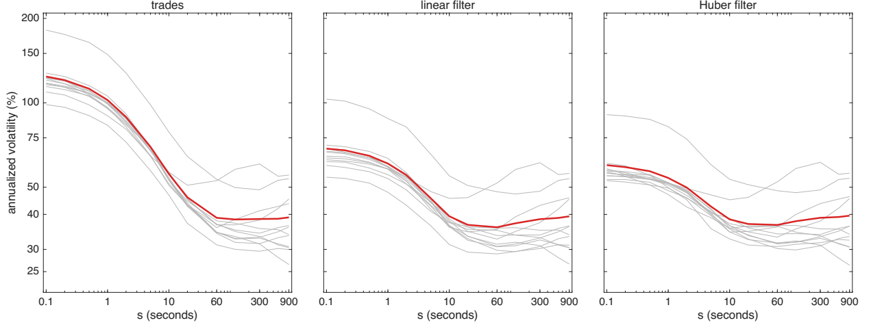
Figure 4: Volatility signature curves for ROKU over the 12 trading days in Oct 2024. The annualized vol \hat{\sigma}100\sqrt{252} from the returns \hat{X}_t - \hat{X}_{t,s} of Table 2, against the lag s in seconds, both axes on log scales, for: raw trades, linear filter & Huber filter. Grey lines are the individual trading days & the red line is the square root of the 12 day average of their squares. The linear & Huber returns carry the finite-sample correction c_{t,s} of the paper; the raw trades are unaffected by it.
