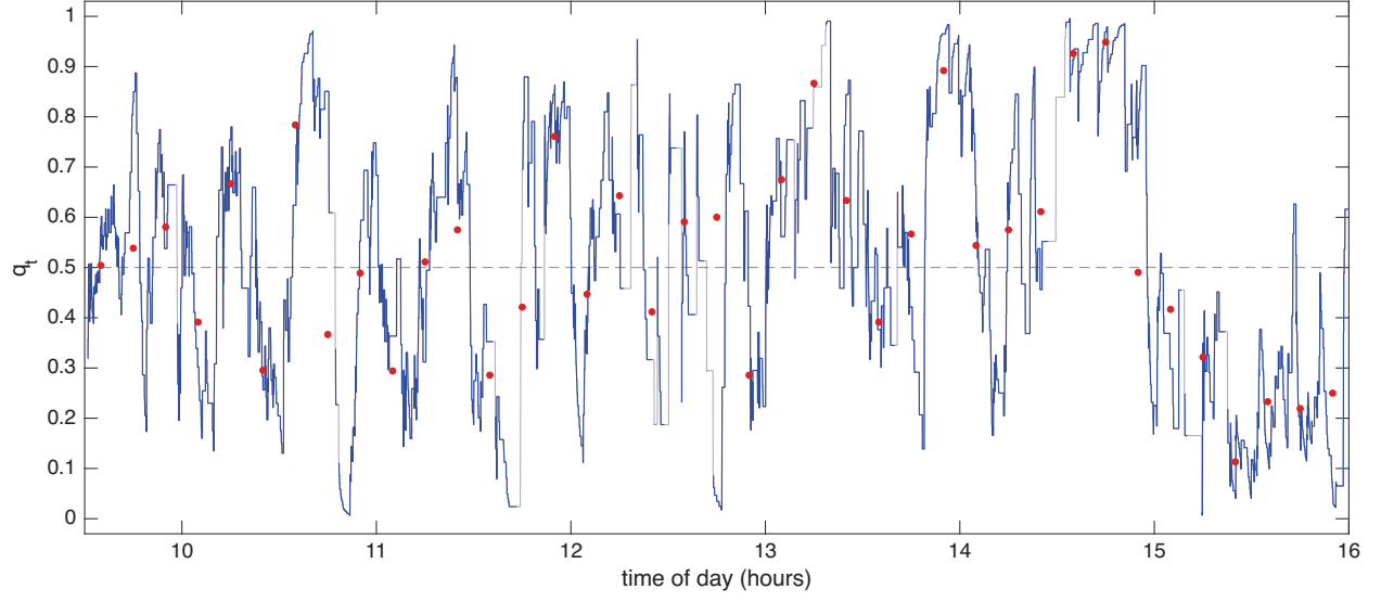
Figure 8: The directional conditional probability for ROKU, 16 October 2024. The filtered conditional probability q_t that an outlier lies above the robust Huber band, under exponential weights decaying in clock time with half life of 77 seconds; where fewer than two outliers remain in the weights it is drawn in grey. The dashed line marks 0.5. The red points are the empirical conditional probability using the 600 second bins of the previous figure.
