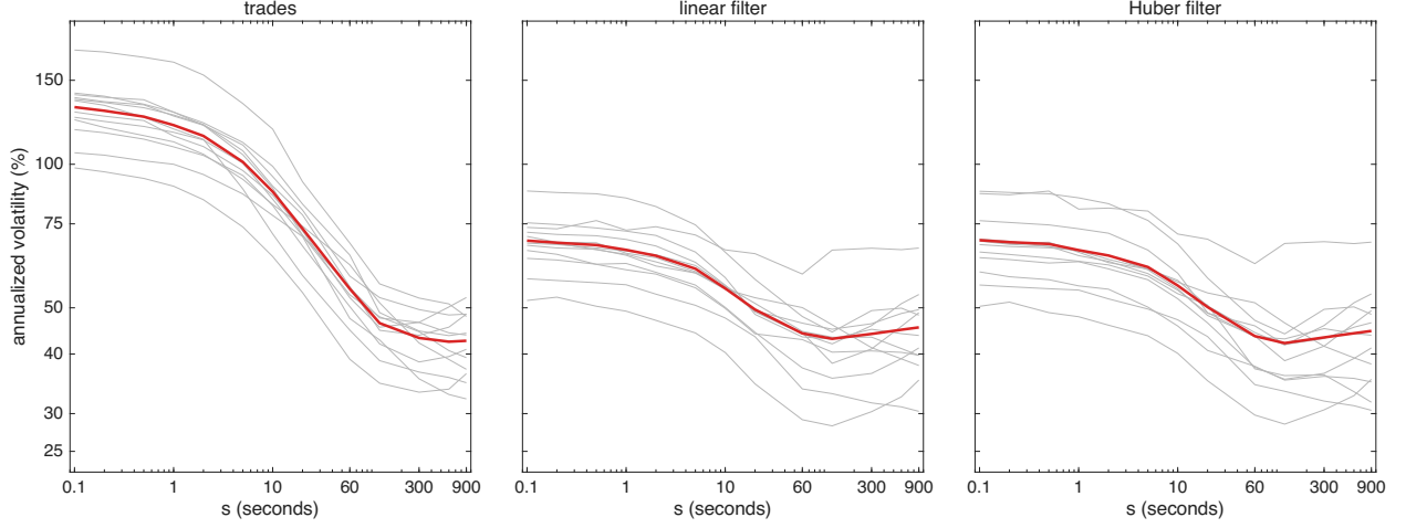
Figure 4: Volatility signature curves for SAIA over the 12 trading days in Oct 2024. The annualized vol \hat{\sigma}100\sqrt{252} from the returns \hat{X}_t - \hat{X}_{t,s} of Table 2, against the lag s in seconds, both axes on log scales, for: raw trades, linear filter & Huber filter. Grey lines are the individual trading days & the red line is the square root of the 12 day average of their squares. The linear & Huber returns carry the finite-sample correction c_{t,s} of the paper; the raw trades are unaffected by it.
