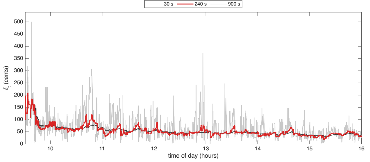
Figure 2: The Huber threshold \delta_t in cents for SAIA on 16 October 2024, with half-lives of 30, 240, 900 seconds. The 240-second half-life, in red, is used.
