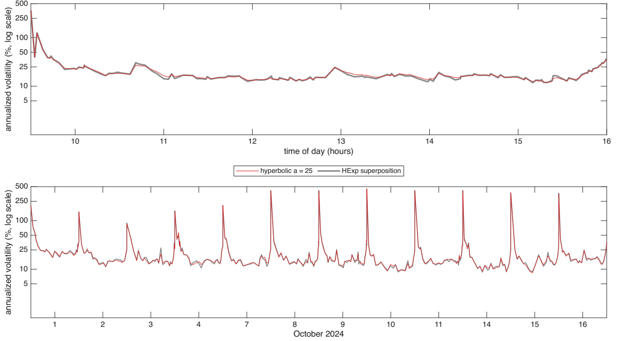
Figure 6: Hyperbolic against superposition weights for SAIA over 12 trading days in Oct 2024, the diurnally adjusted \hat{\sigma}(u)100\sqrt{252} at s = 1 second from the Huber filter, shown as annualized vol in % on a log10 scale. The only difference between the 2 paths is the weight function: the hyperbolic weights with a = 25 in red, drawn on top, and the HExp superposition in grey, 4 exponential components with half lives of 10, 100, 1000, 10000 seconds. Hyperparameters minimize the QLIKE objective. Top: 16 October 2024, bottom: 12 days.
