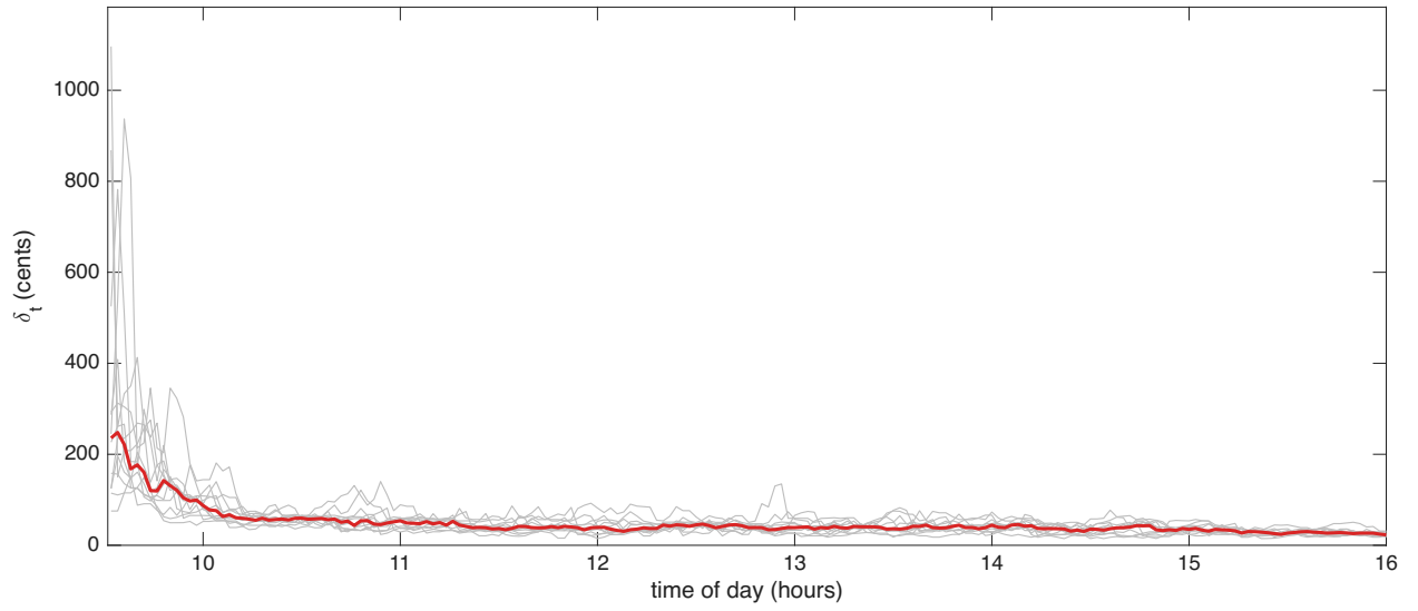
Figure 3: Huber threshold \delta_t in cents through the trading day, for 12 SAIA trading days in Oct 2024 (grey lines) and their median (red line).
