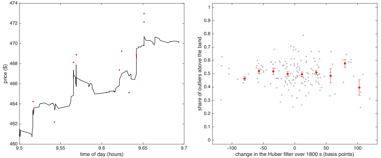
Figure 7: Outliers & robust price for SAIA on 16 October 2024. Left: the 12 minutes with the largest move in the Huber filter that day; outliers above Y_t - \theta_t > \delta_{t-1} in red, outliers below Y_t - \theta_t < -\delta_{t-1} in blue, Huber filter in black. Right: over the 12 trading days, the 1800 second empirical conditional probability that outliers are above (rather than below) the Huber band against the 1800 second change in the Huber filter in basis points: light points are single bins, the line & bars are means & s.e.
