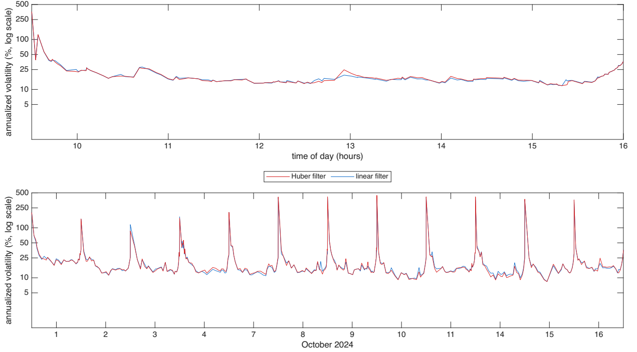
Figure 5: Filtered spot volatility for SAIA over 12 trading days in Oct 2024, the diurnally adjusted estimator \hat{\sigma}(u)100\sqrt{252} at s = 1 second with hyperbolic weights, Mandelbrot parameter a = 25 , with the input prices computed using the Huber & linear filters, shown as annualized volatility in percent on a log10 scale. Top: 16 October 2024, bottom: 12 days.
