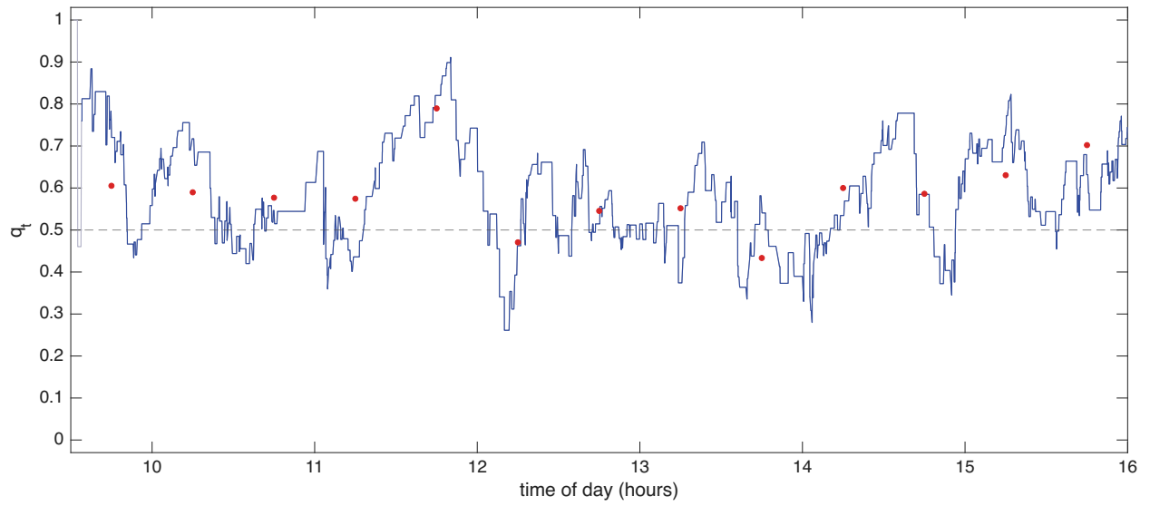
Figure 8: The directional conditional probability for SAIA, 16 October 2024. The filtered conditional probability q_t that an outlier lies above the robust Huber band, under exponential weights decaying in clock time with half life of 405 seconds; where fewer than two outliers remain in the weights it is drawn in grey. The dashed line marks 0.5. The red points are the empirical conditional probability using the 1800 second bins of the previous figure.
