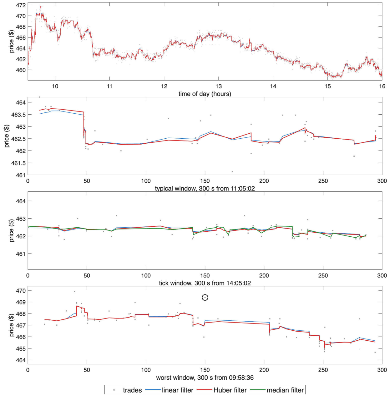
Figure 1: SAIA trades (grey points), the linear filter and the Huber filter, 16 October 2024. Top: full trading day. 2nd: 300-second window at the day's median trade count, from 11:05:02. 3rd: 300-second window at 14:05:02 in which the price reverses direction most often, with the median filter m_t added. Bottom: 300-second window around the largest Huber residual after 09:45, circled.
