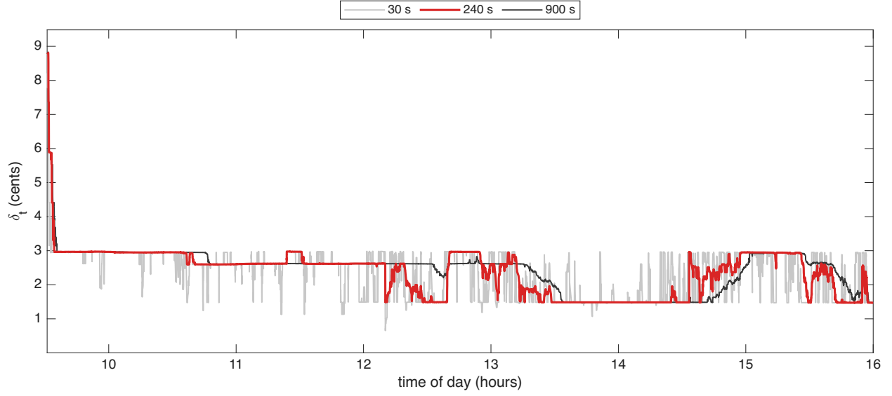
Figure 2: The Huber threshold \delta_t in cents for SBUX on 16 October 2024, with half-lives of 30, 240, 900 seconds. The 240-second half-life, in red, is used.
