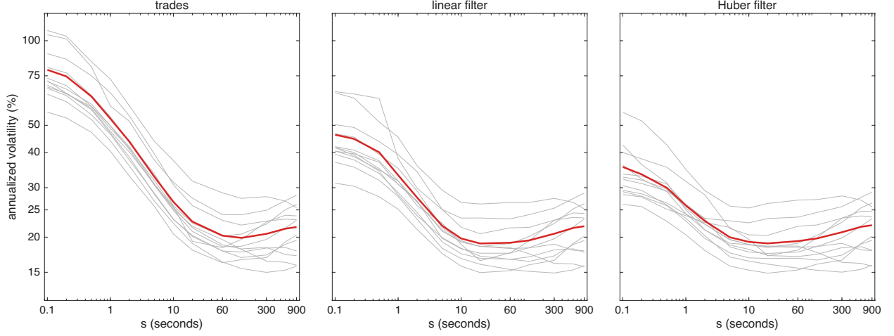
Figure 4: Volatility signature curves for SBUX over the 12 trading days in Oct 2024. The annualized vol \hat{\sigma}100\sqrt{252} from the returns \hat{X}_t - \hat{X}_{t,s} of Table 2, against the lag s in seconds, both axes on log scales, for: raw trades, linear filter & Huber filter. Grey lines are the individual trading days & the red line is the square root of the 12 day average of their squares. The linear & Huber returns carry the finite-sample correction c_{t,s} of the paper; the raw trades are unaffected by it.
