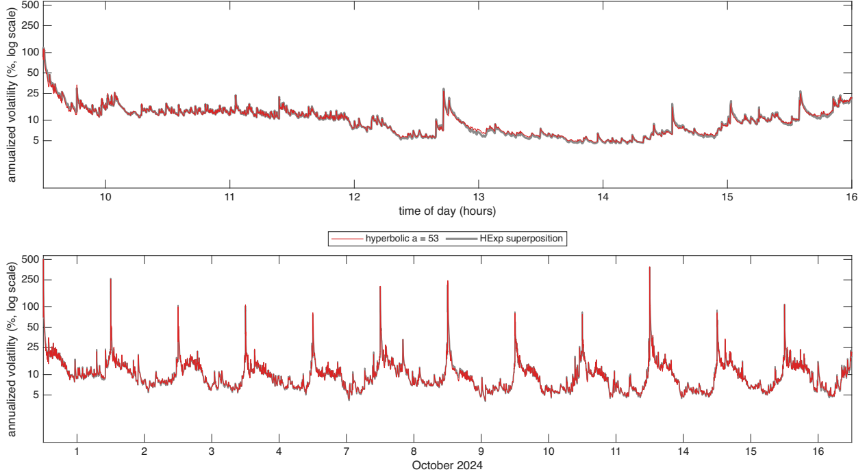
Figure 6: Hyperbolic against superposition weights for SBUX over 12 trading days in Oct 2024, the diurnally adjusted \hat{\sigma}(u)100\sqrt{252} at s = 1 second from the Huber filter, shown as annualized vol in % on a log10 scale. The only difference between the 2 paths is the weight function: the hyperbolic weights with a = 53 in red, drawn on top, and the HExp superposition in grey, 4 exponential components with half lives of 10, 100, 1000, 10000 seconds. Hyperparameters minimize the QLIKE objective. Top: 16 October 2024, bottom: 12 days.
