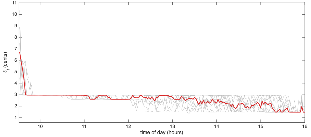
Figure 3: Huber threshold \delta_t in cents through the trading day, for 12 SBUX trading days in Oct 2024 (grey lines) and their median (red line).
