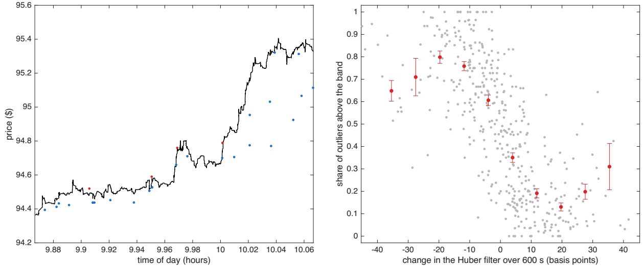
Figure 7: Outliers & robust price for SBUX on 16 October 2024. Left: the 12 minutes with the largest move in the Huber filter that day; outliers above Y_t - \theta_t > \delta_{t-1} in red, outliers below Y_t - \theta_t < -\delta_{t-1} in blue, Huber filter in black. Right: over the 12 trading days, the 600 second empirical conditional probability that outliers are above (rather than below) the Huber band against the 600 second change in the Huber filter in basis points: light points are single bins, the line & bars are means & s.e.
