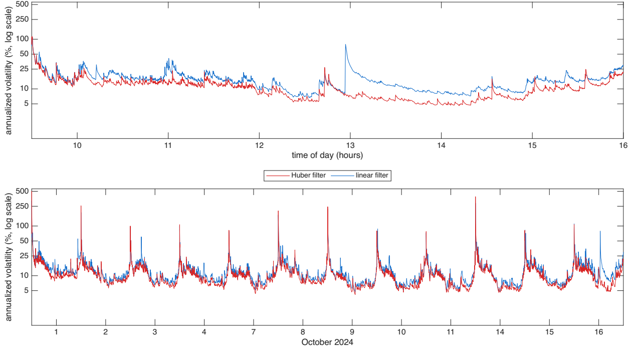
Figure 5: Filtered spot volatility for SBUX over 12 trading days in Oct 2024, the diurnally adjusted estimator \hat{\sigma}(u)100\sqrt{252} at s = 1 second with hyperbolic weights, Mandelbrot parameter a = 53 , with the input prices computed using the Huber & linear filters, shown as annualized volatility in percent on a log10 scale. Top: 16 October 2024, bottom: 12 days.
