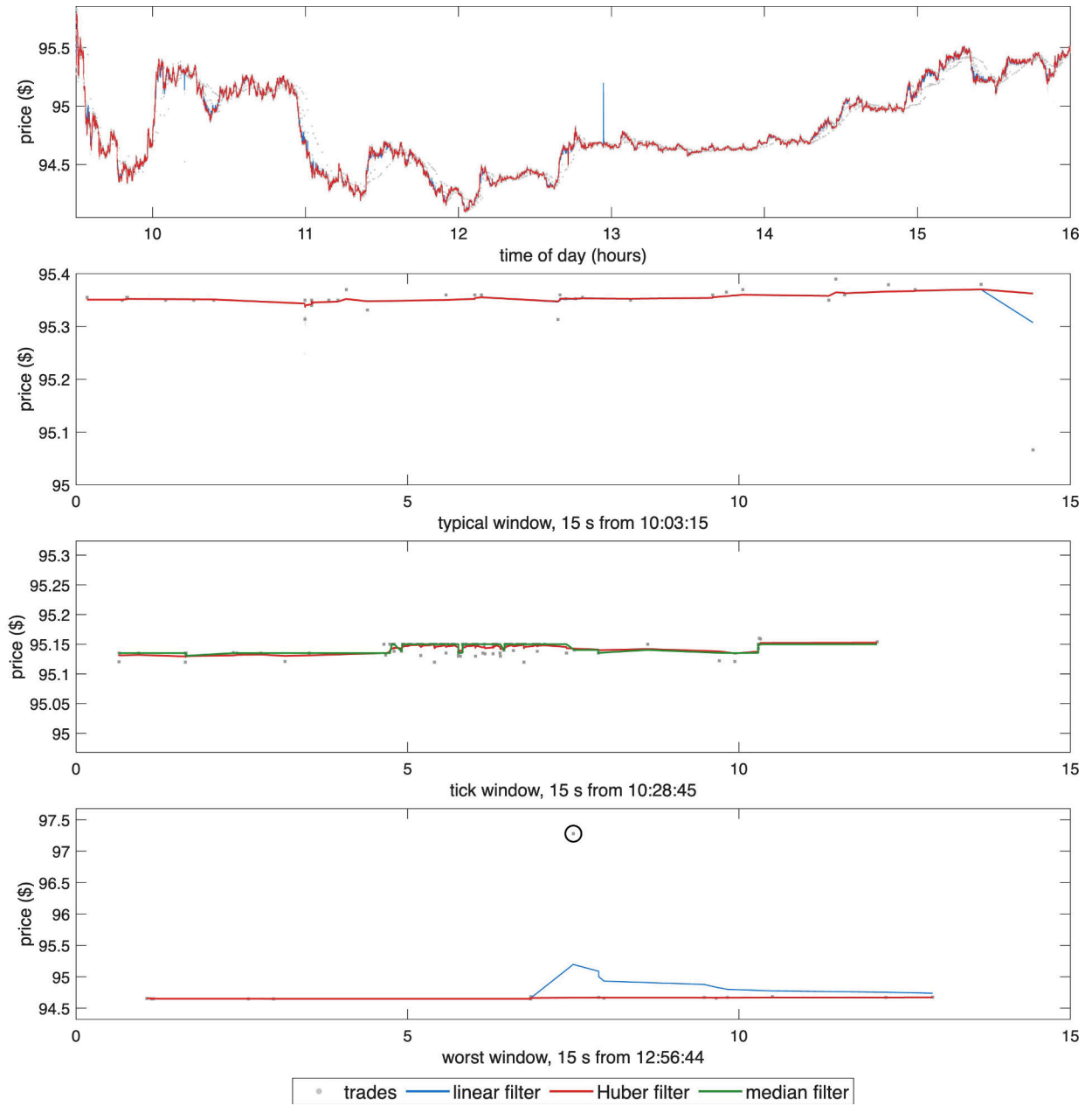
Figure 1: SBUX trades (grey points), the linear filter and the Huber filter, 16 October 2024. Top: full trading day. 2nd: 15-second window at the day's median trade count, from 10:03:15. 3rd: 15-second window at 10:28:45 in which the price reverses direction most often, with the median filter m_t added. Bottom: 15-second window around the largest Huber residual after 09:45, circled.
