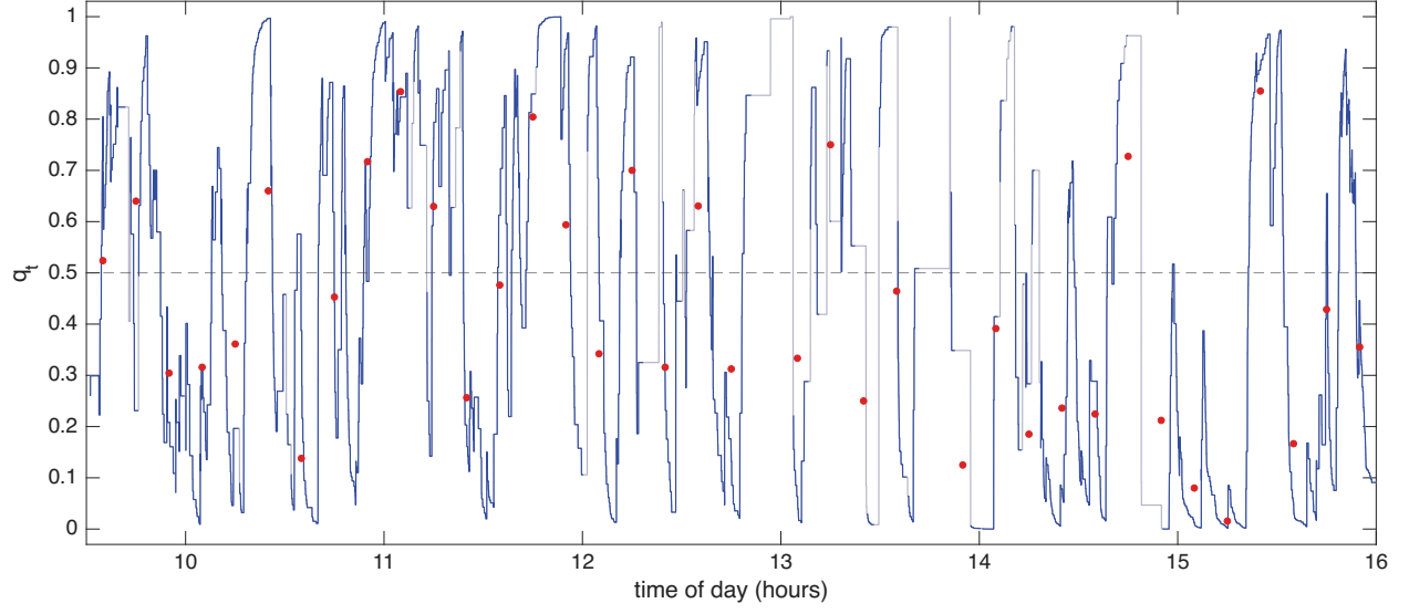
Figure 8: The directional conditional probability for SBUX, 16 October 2024. The filtered conditional probability q_t that an outlier lies above the robust Huber band, under exponential weights decaying in clock time with half life of 57 seconds; where fewer than two outliers remain in the weights it is drawn in grey. The dashed line marks 0.5. The red points are the empirical conditional probability using the 600 second bins of the previous figure.
