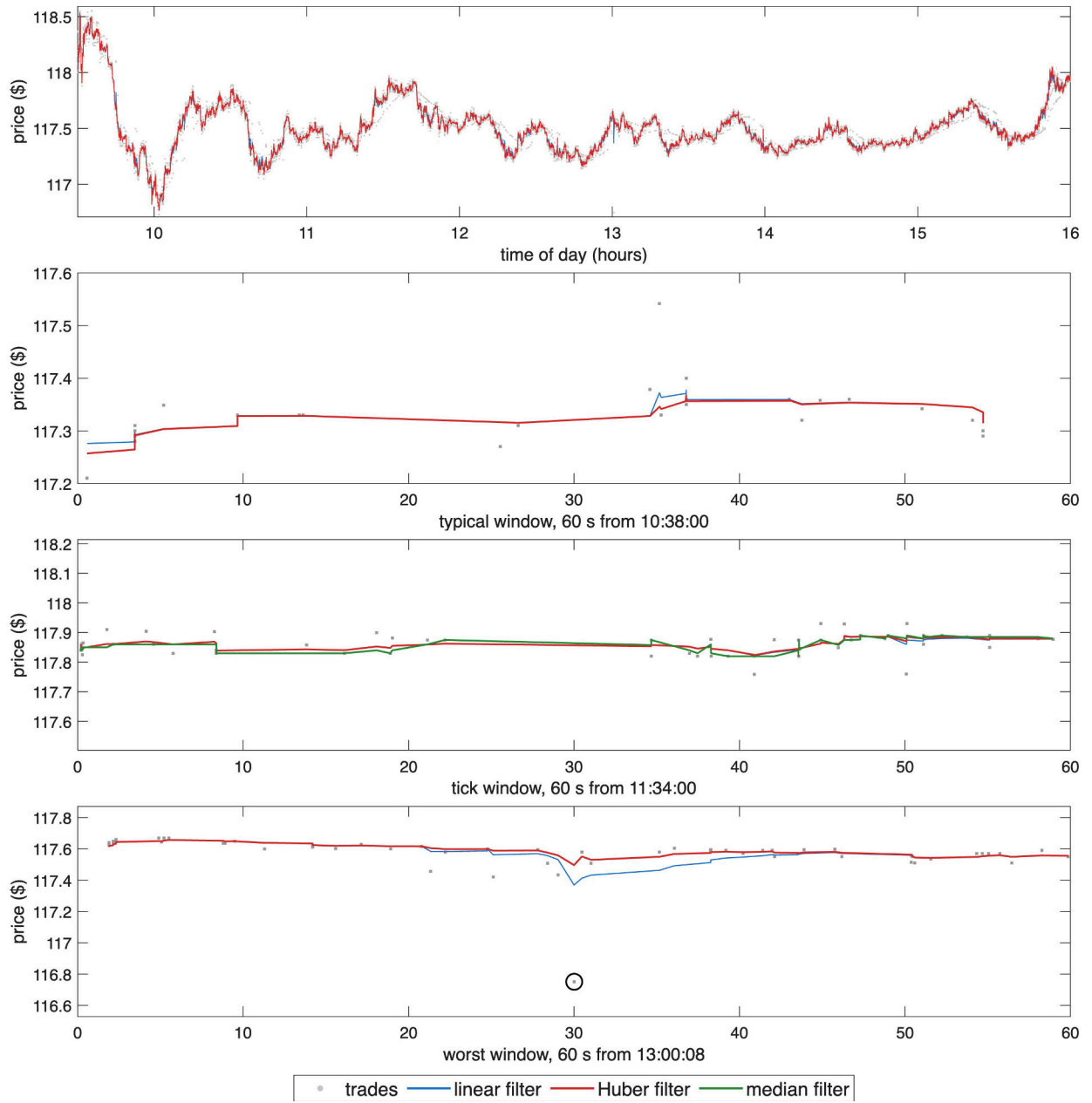
Figure 1: TTD trades (grey points), the linear filter and the Huber filter, 16 October 2024. Top: full trading day. 2nd: 60-second window at the day's median trade count, from 10:38:00. 3rd: 60-second window at 11:34:00 in which the price reverses direction most often, with the median filter m_t added. Bottom: 60-second window around the largest Huber residual after 09:45, circled.
