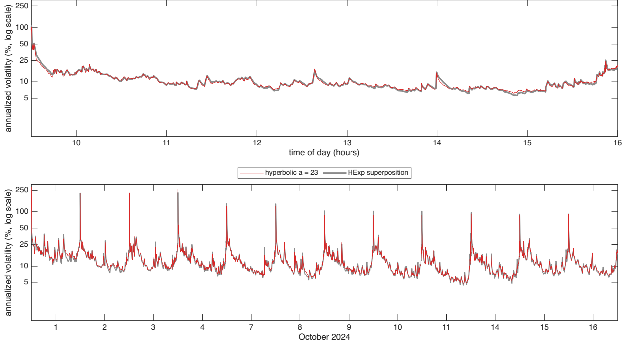
Figure 6: Hyperbolic against superposition weights for TTD over 12 trading days in Oct 2024, the diurnally adjusted \hat{\sigma}(u)100\sqrt{252} at s = 1 second from the Huber filter, shown as annualized vol in % on a log10 scale. The only difference between the 2 paths is the weight function: the hyperbolic weights with a = 23 in red, drawn on top, and the HExp superposition in grey, 4 exponential components with half lives of 10, 100, 1000, 10000 seconds. Hyperparameters minimize the QLIKE objective. Top: 16 October 2024, bottom: 12 days.
