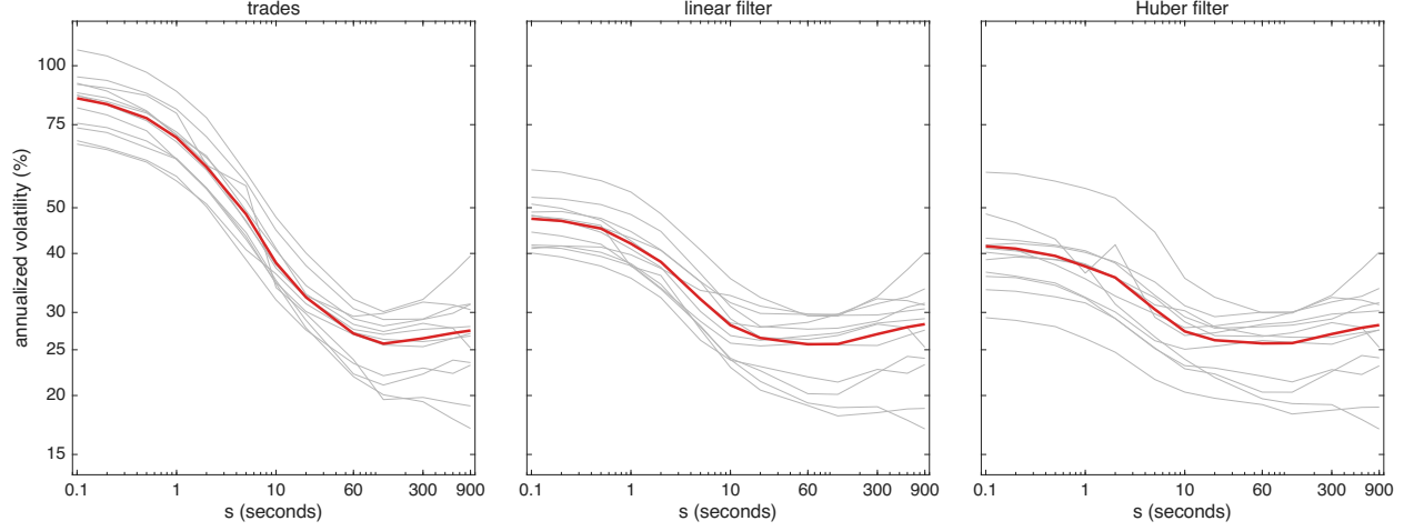
Figure 4: Volatility signature curves for TTD over the 12 trading days in Oct 2024. The annualized vol \hat{\sigma}100\sqrt{252} from the returns \hat{X}_t - \hat{X}_{t,s} of Table 2, against the lag s in seconds, both axes on log scales, for: raw trades, linear filter & Huber filter. Grey lines are the individual trading days & the red line is the square root of the 12 day average of their squares. The linear & Huber returns carry the finite-sample correction c_{t,s} of the paper; the raw trades are unaffected by it.
