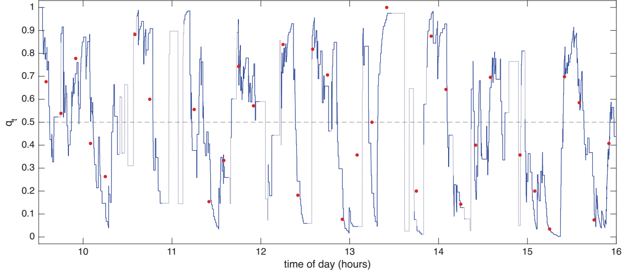
Figure 8: The directional conditional probability for TTD, 16 October 2024. The filtered conditional probability q_t that an outlier lies above the robust Huber band, under exponential weights decaying in clock time with half life of 100 seconds; where fewer than two outliers remain in the weights it is drawn in grey. The dashed line marks 0.5. The red points are the empirical conditional probability using the 600 second bins of the previous figure.
