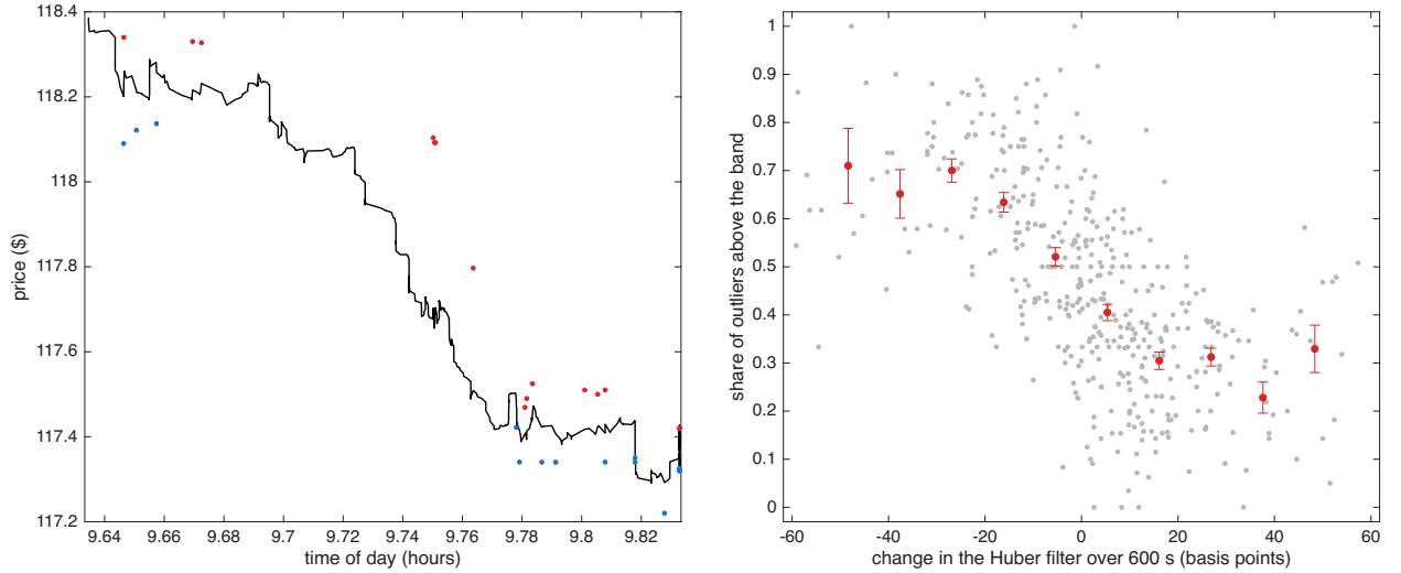
Figure 7: Outliers & robust price for TTD on 16 October 2024. Left: the 12 minutes with the largest move in the Huber filter that day; outliers above Y_t - \theta_t > \delta_{t-1} in red, outliers below Y_t - \theta_t < -\delta_{t-1} in blue, Huber filter in black. Right: over the 12 trading days, the 600 second empirical conditional probability that outliers are above (rather than below) the Huber band against the 600 second change in the Huber filter in basis points: light points are single bins, the line & bars are means & s.e.
