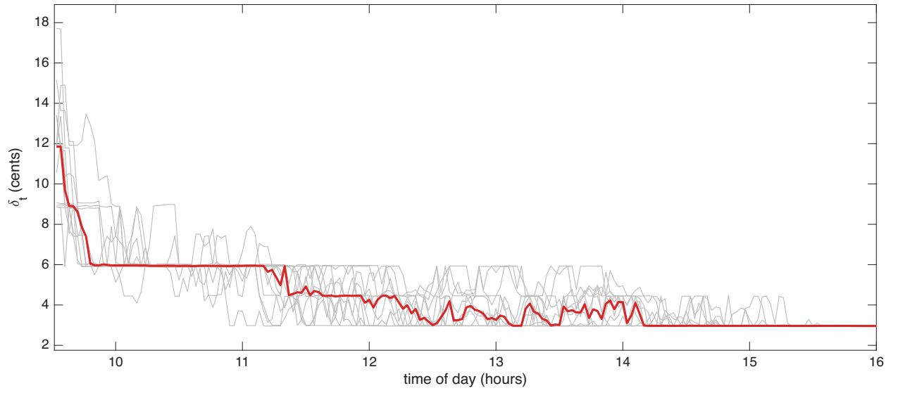
Figure 3: Huber threshold \delta_t in cents through the trading day, for 12 TTD trading days in Oct 2024 (grey lines) and their median (red line).
