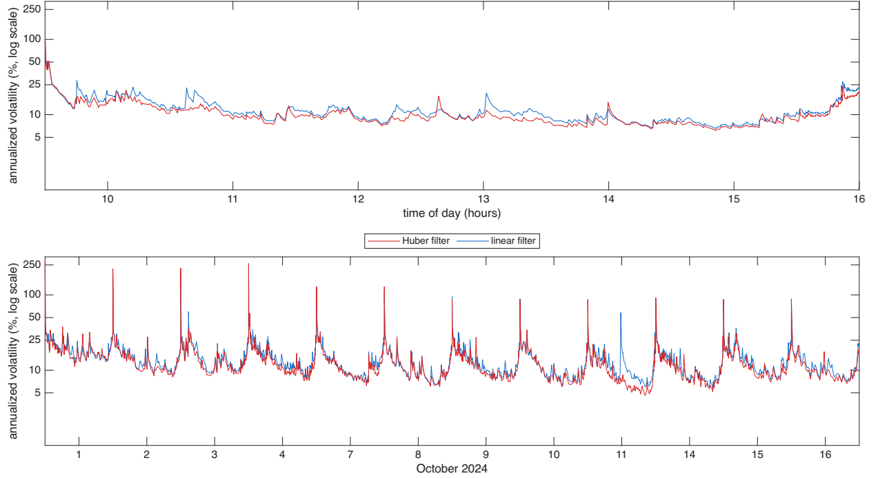
Figure 5: Filtered spot volatility for TTD over 12 trading days in Oct 2024, the diurnally adjusted estimator \hat{\sigma}(u)100\sqrt{252} at s = 1 second with hyperbolic weights, Mandelbrot parameter a = 23 , with the input prices computed using the Huber & linear filters, shown as annualized volatility in percent on a log10 scale. Top: 16 October 2024, bottom: 12 days.
