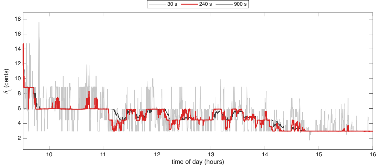
Figure 2: The Huber threshold \delta_t in cents for TTD on 16 October 2024, with half-lives of 30, 240, 900 seconds. The 240-second half-life, in red, is used.
