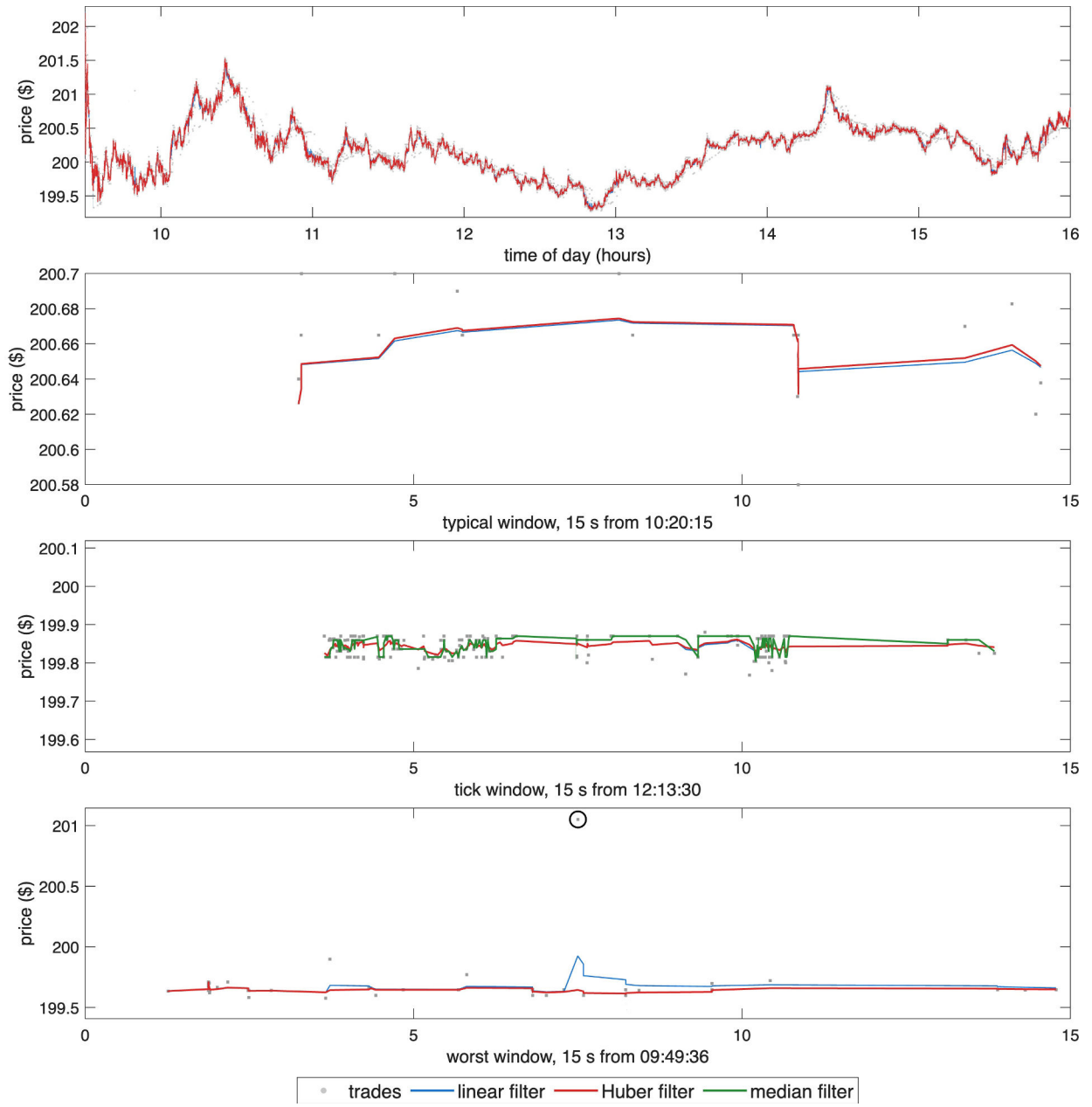
Figure 1: TXN trades (grey points), the linear filter and the Huber filter, 16 October 2024. Top: full trading day. 2nd: 15-second window at the day's median trade count, from 10:20:15. 3rd: 15-second window at 12:13:30 in which the price reverses direction most often, with the median filter m_t added. Bottom: 15-second window around the largest Huber residual after 09:45, circled.
