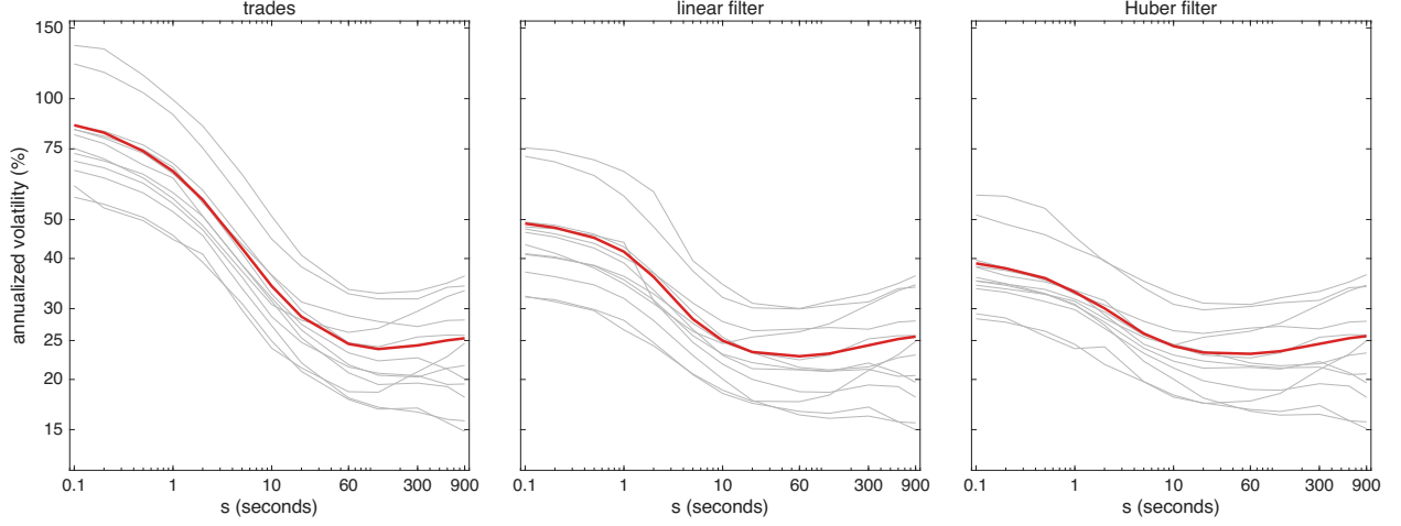
Figure 4: Volatility signature curves for TXN over the 12 trading days in Oct 2024. The annualized vol \hat{\sigma}100\sqrt{252} from the returns \hat{X}_t - \hat{X}_{t,s} of Table 2, against the lag s in seconds, both axes on log scales, for: raw trades, linear filter & Huber filter. Grey lines are the individual trading days & the red line is the square root of the 12 day average of their squares. The linear & Huber returns carry the finite-sample correction c_{t,s} of the paper; the raw trades are unaffected by it.
