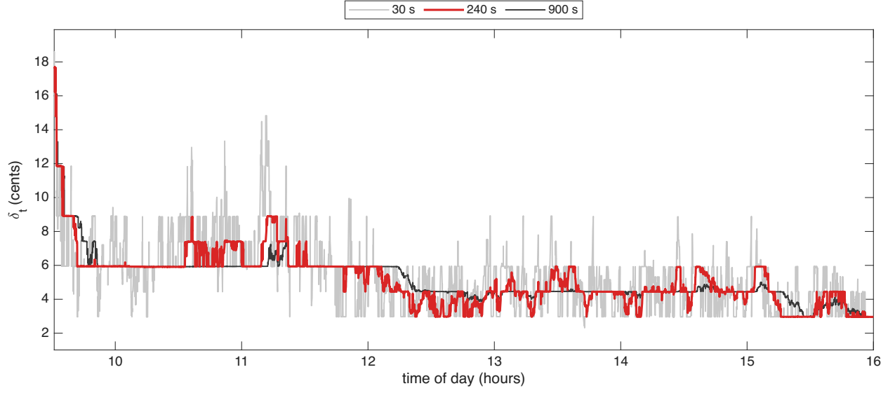
Figure 2: The Huber threshold \delta_t in cents for TXN on 16 October 2024, with half-lives of 30, 240, 900 seconds. The 240-second half-life, in red, is used.
