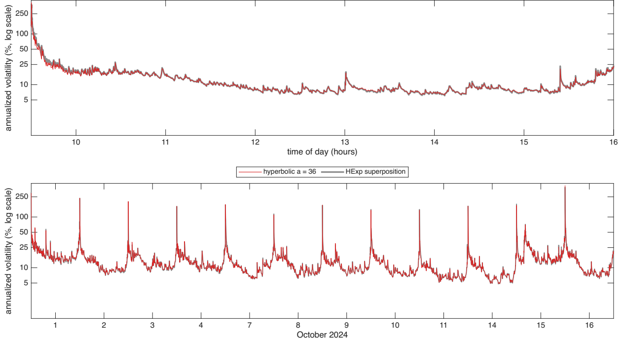
Figure 6: Hyperbolic against superposition weights for TXN over 12 trading days in Oct 2024, the diurnally adjusted \hat{\sigma}(u)100\sqrt{252} at s = 1 second from the Huber filter, shown as annualized vol in % on a log10 scale. The only difference between the 2 paths is the weight function: the hyperbolic weights with a = 36 in red, drawn on top, and the HExp superposition in grey, 4 exponential components with half lives of 10, 100, 1000, 10000 seconds. Hyperparameters minimize the QLIKE objective. Top: 16 October 2024, bottom: 12 days.
