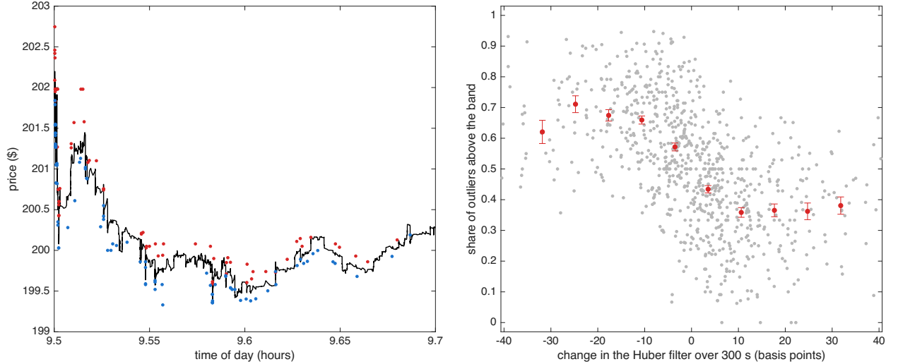
Figure 7: Outliers & robust price for TXN on 16 October 2024. Left: the 12 minutes with the largest move in the Huber filter that day; outliers above Y_t - \theta_t > \delta_{t-1} in red, outliers below Y_t - \theta_t < -\delta_{t-1} in blue, Huber filter in black. Right: over the 12 trading days, the 300 second empirical conditional probability that outliers are above (rather than below) the Huber band against the 300 second change in the Huber filter in basis points: light points are single bins, the line & bars are means & s.e.
