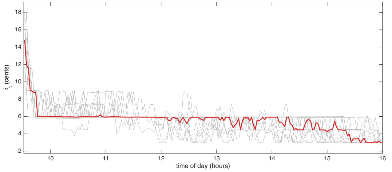
Figure 3: Huber threshold \delta_t in cents through the trading day, for 12 TXN trading days in Oct 2024 (grey lines) and their median (red line).
