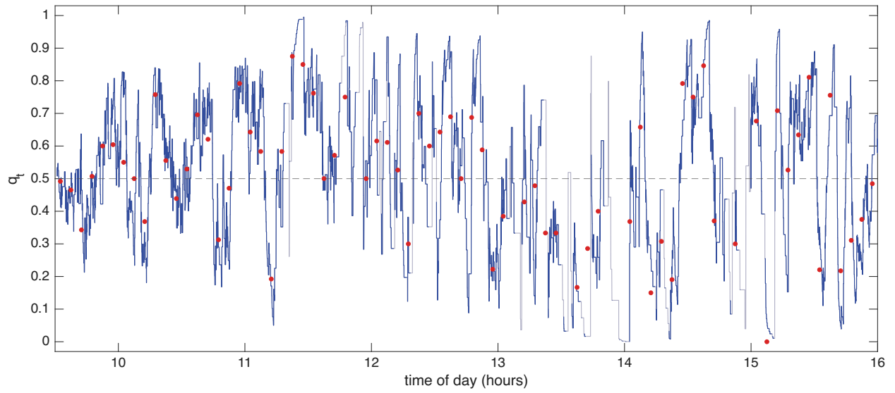
Figure 8: The directional conditional probability for TXN, 16 October 2024. The filtered conditional probability q_t that an outlier lies above the robust Huber band, under exponential weights decaying in clock time with half life of 51 seconds; where fewer than two outliers remain in the weights it is drawn in grey. The dashed line marks 0.5. The red points are the empirical conditional probability using the 300 second bins of the previous figure.
