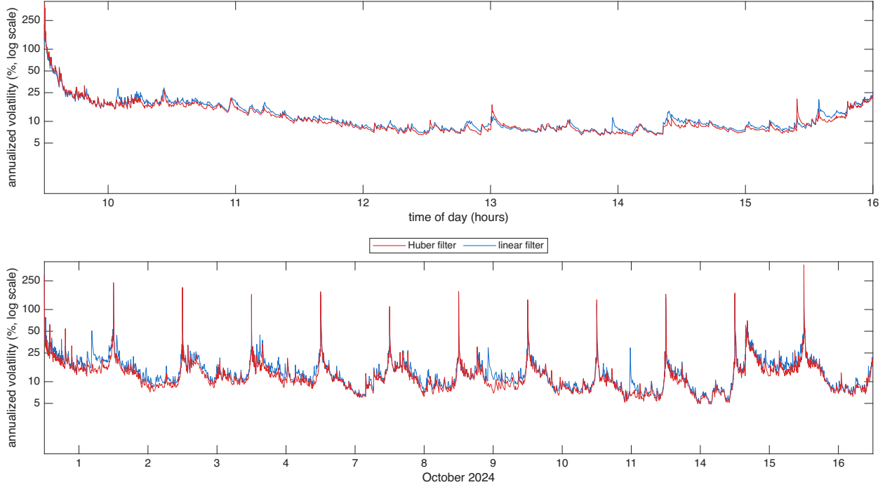
Figure 5: Filtered spot volatility for TXN over 12 trading days in Oct 2024, the diurnally adjusted estimator \hat{\sigma}(u)100\sqrt{252} at s = 1 second with hyperbolic weights, Mandelbrot parameter a = 36 , with the input prices computed using the Huber & linear filters, shown as annualized volatility in percent on a log10 scale. Top: 16 October 2024, bottom: 12 days.
