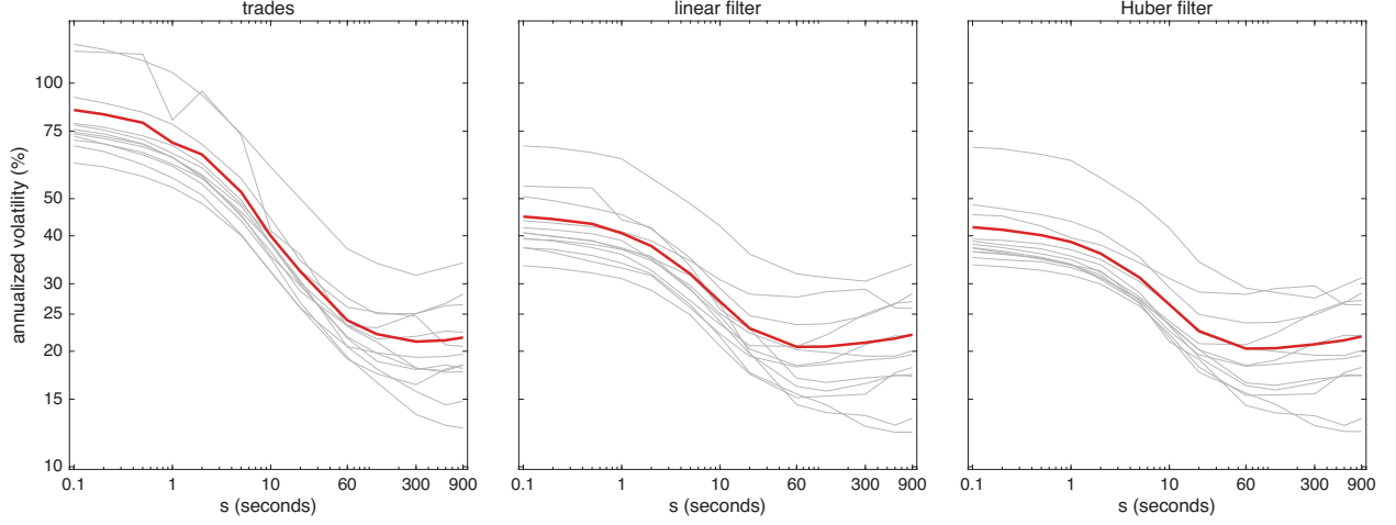
Figure 4: Volatility signature curves for VRTX over the 12 trading days in Oct 2024. The annualized vol \hat{\sigma}100\sqrt{252} from the returns \hat{X}_t - \hat{X}_{t,s} of Table 2, against the lag s in seconds, both axes on log scales, for: raw trades, linear filter & Huber filter. Grey lines are the individual trading days & the red line is the square root of the 12 day average of their squares. The linear & Huber returns carry the finite-sample correction c_{t,s} of the paper; the raw trades are unaffected by it.
