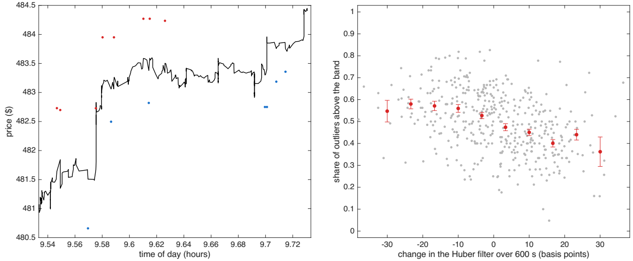
Figure 7: Outliers & robust price for VRTX on 16 October 2024. Left: the 12 minutes with the largest move in the Huber filter that day; outliers above Y_t - \theta_t > \delta_{t-1} in red, outliers below Y_t - \theta_t < -\delta_{t-1} in blue, Huber filter in black. Right: over the 12 trading days, the 600 second empirical conditional probability that outliers are above (rather than below) the Huber band against the 600 second change in the Huber filter in basis points: light points are single bins, the line & bars are means & s.e.
