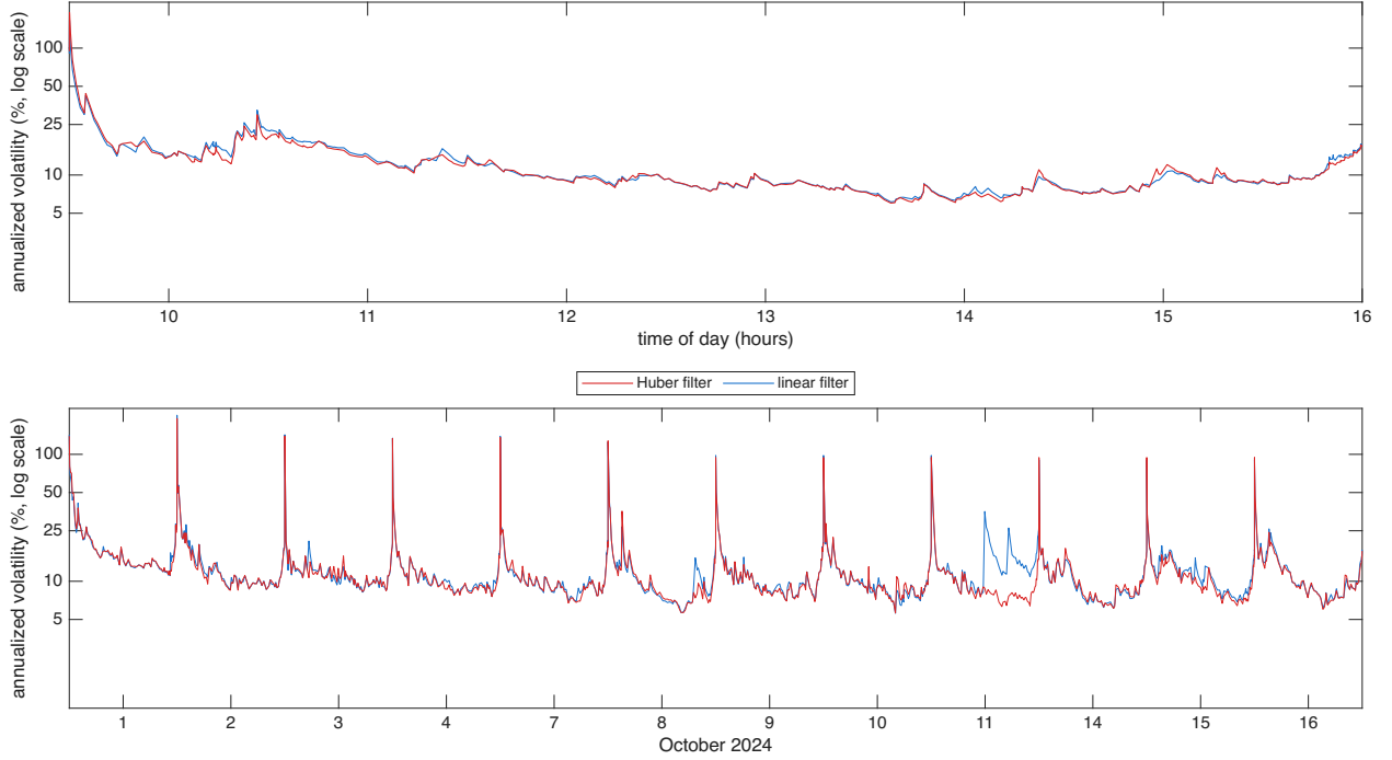
Figure 5: Filtered spot volatility for VRTX over 12 trading days in Oct 2024, the diurnally adjusted estimator \hat{\sigma}(u)100\sqrt{252} at s = 1 second with hyperbolic weights, Mandelbrot parameter a = 50 , with the input prices computed using the Huber & linear filters, shown as annualized volatility in percent on a log10 scale. Top: 16 October 2024, bottom: 12 days.
