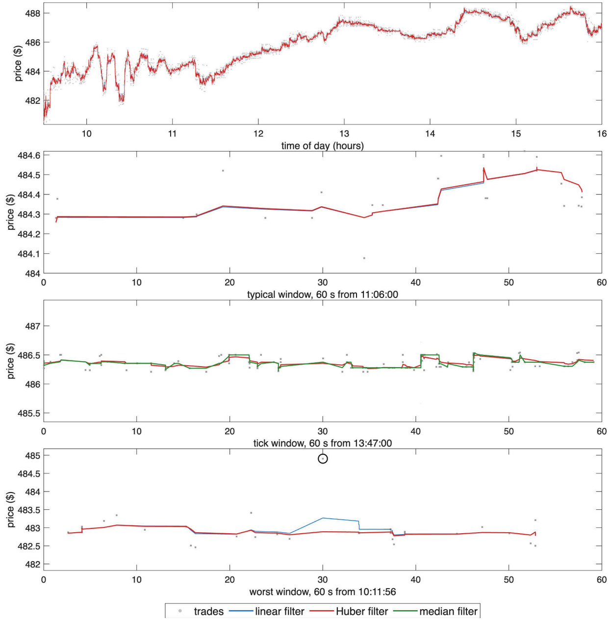
Figure 1: VRTX trades (grey points), the linear filter and the Huber filter, 16 October 2024. Top: full trading day. 2nd: 60-second window at the day's median trade count, from 11:06:00. 3rd: 60-second window at 13:47:00 in which the price reverses direction most often, with the median filter m_t added. Bottom: 60-second window around the largest Huber residual after 09:45, circled.
