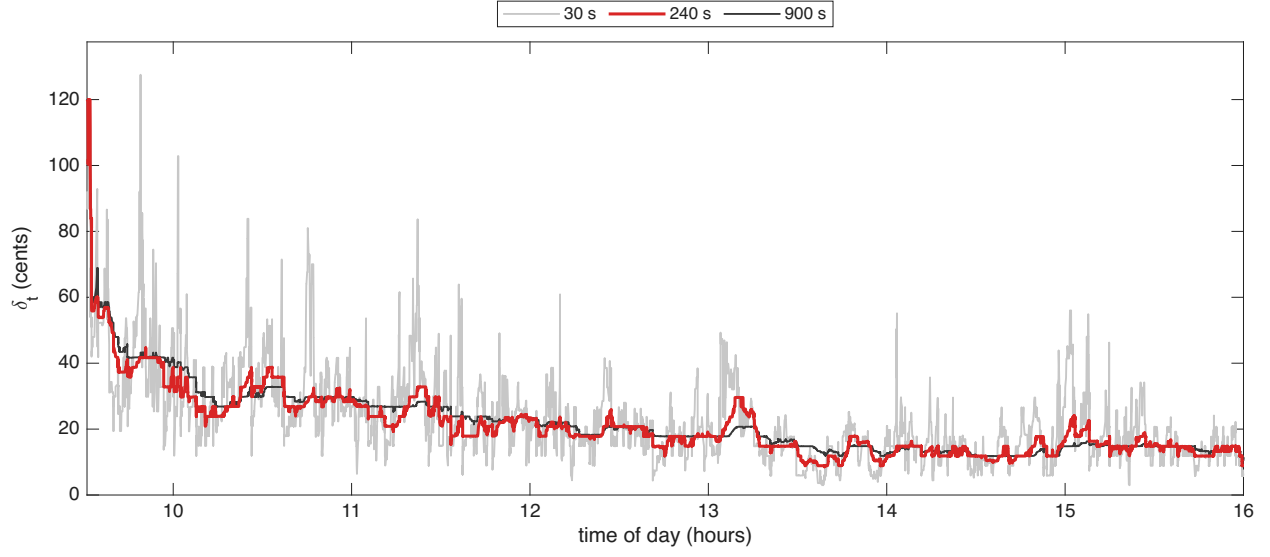
Figure 2: The Huber threshold \delta_t in cents for VRTX on 16 October 2024, with half-lives of 30, 240, 900 seconds. The 240-second half-life, in red, is used.
