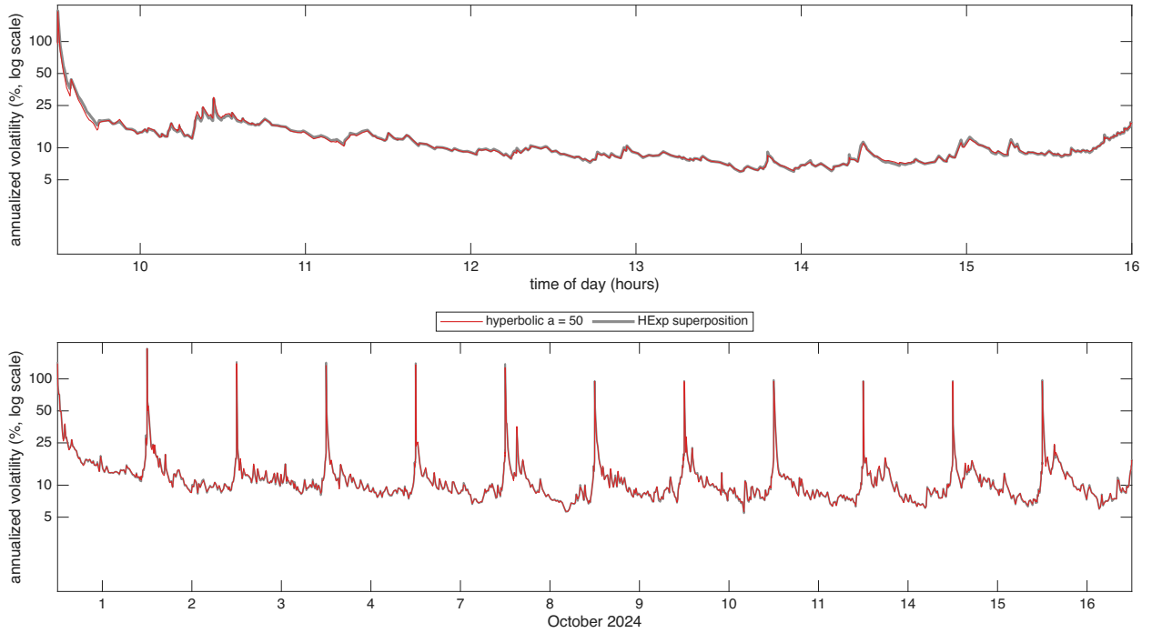
Figure 6: Hyperbolic against superposition weights for VRTX over 12 trading days in Oct 2024, the diurnally adjusted \hat{\sigma}(u)100\sqrt{252} at s = 1 second from the Huber filter, shown as annualized vol in % on a log10 scale. The only difference between the 2 paths is the weight function: the hyperbolic weights with a = 50 in red, drawn on top, and the HExp superposition in grey, 4 exponential components with half lives of 10, 100, 1000, 10000 seconds. Hyperparameters minimize the QLIKE objective. Top: 16 October 2024, bottom: 12 days.
