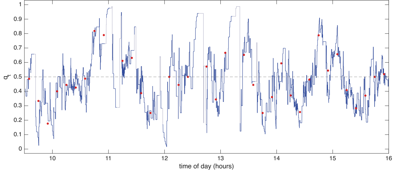
Figure 8: The directional conditional probability for VRTX, 16 October 2024. The filtered conditional probability q_t that an outlier lies above the robust Huber band, under exponential weights decaying in clock time with half life of 101 seconds; where fewer than two outliers remain in the weights it is drawn in grey. The dashed line marks 0.5. The red points are the empirical conditional probability using the 600 second bins of the previous figure.
