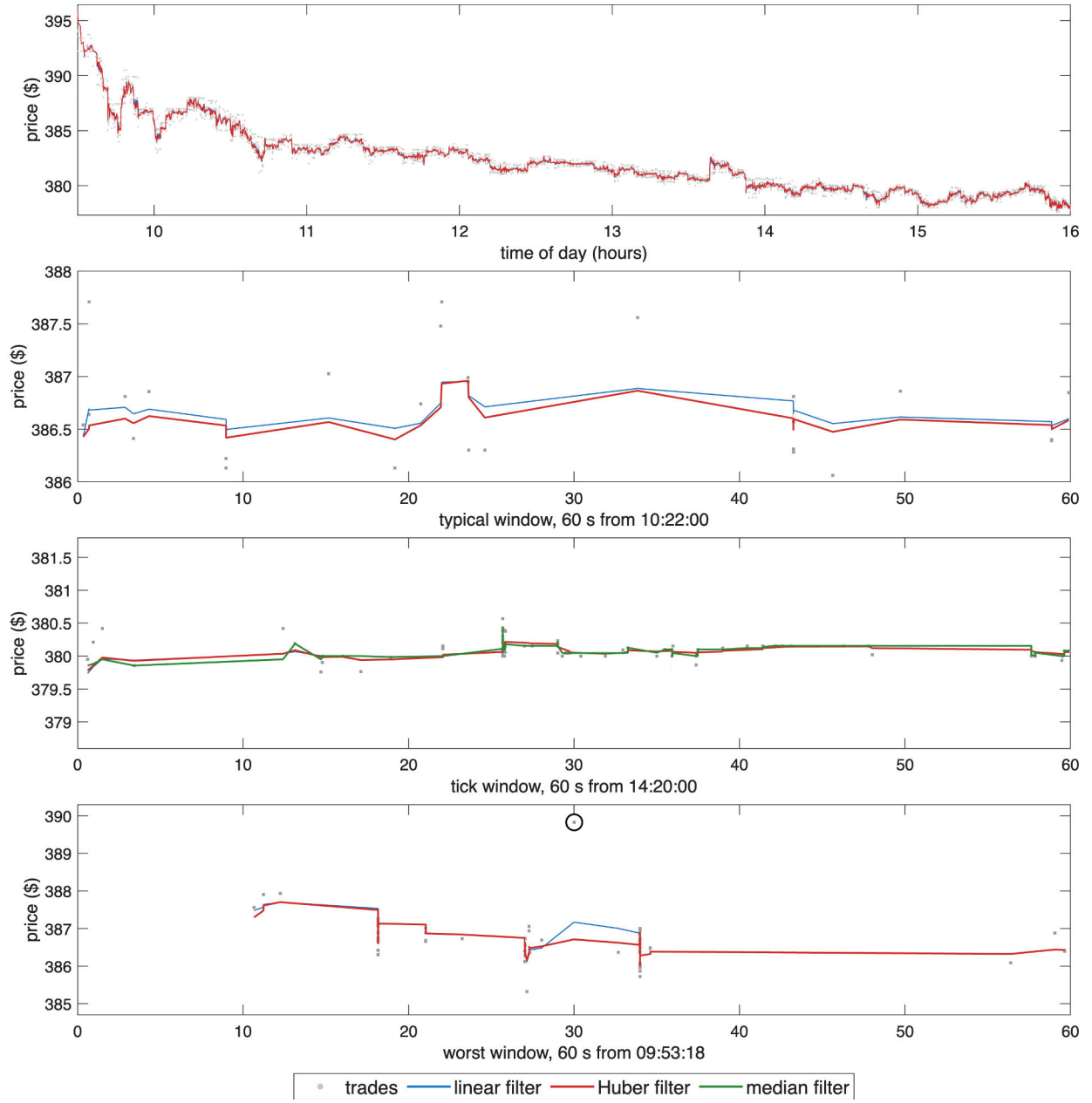
Figure 1: WING trades (grey points), the linear filter and the Huber filter, 16 October 2024. Top: full trading day. 2nd: 60-second window at the day's median trade count, from 10:22:00. 3rd: 60-second window at 14:20:00 in which the price reverses direction most often, with the median filter m_t added. Bottom: 60-second window around the largest Huber residual after 09:45, circled.
