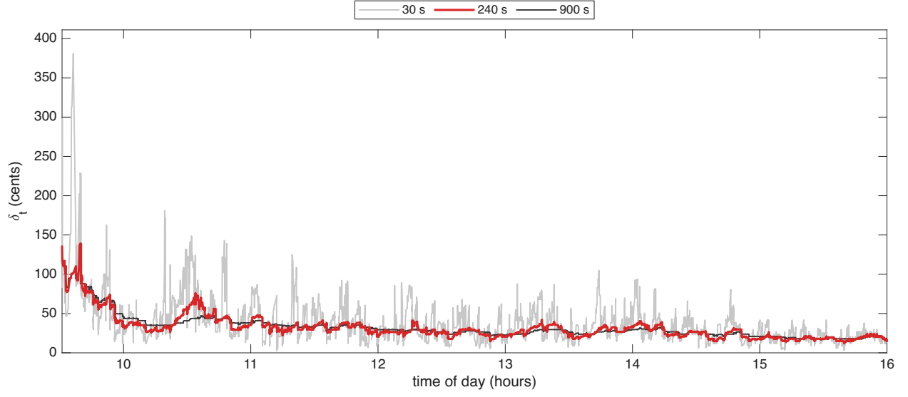
Figure 2: The Huber threshold \delta_t in cents for WING on 16 October 2024, with half-lives of 30, 240, 900 seconds. The 240-second half-life, in red, is used.
