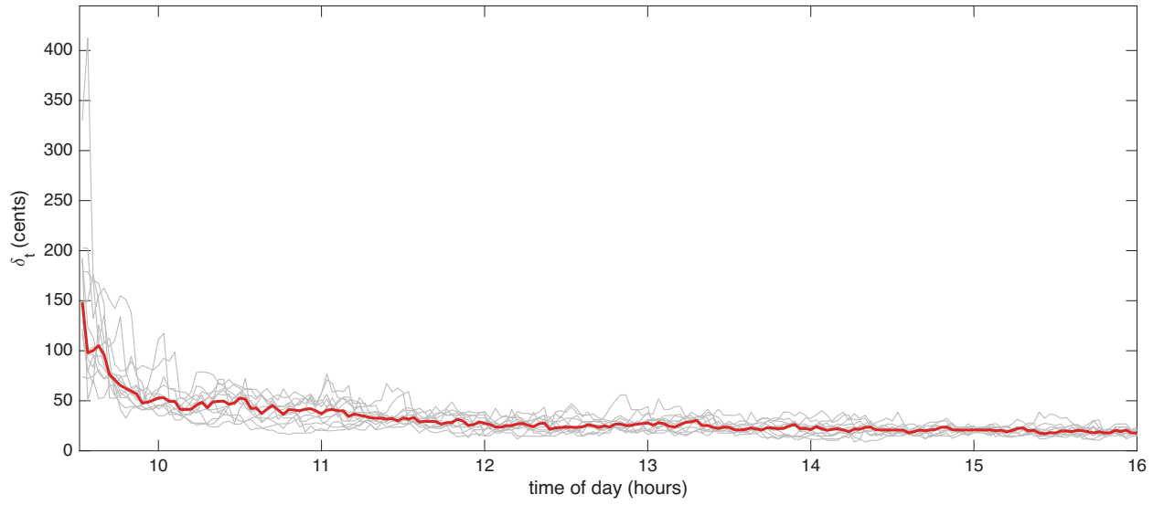
Figure 3: Huber threshold \delta_t in cents through the trading day, for 12 WING trading days in Oct 2024 (grey lines) and their median (red line).
