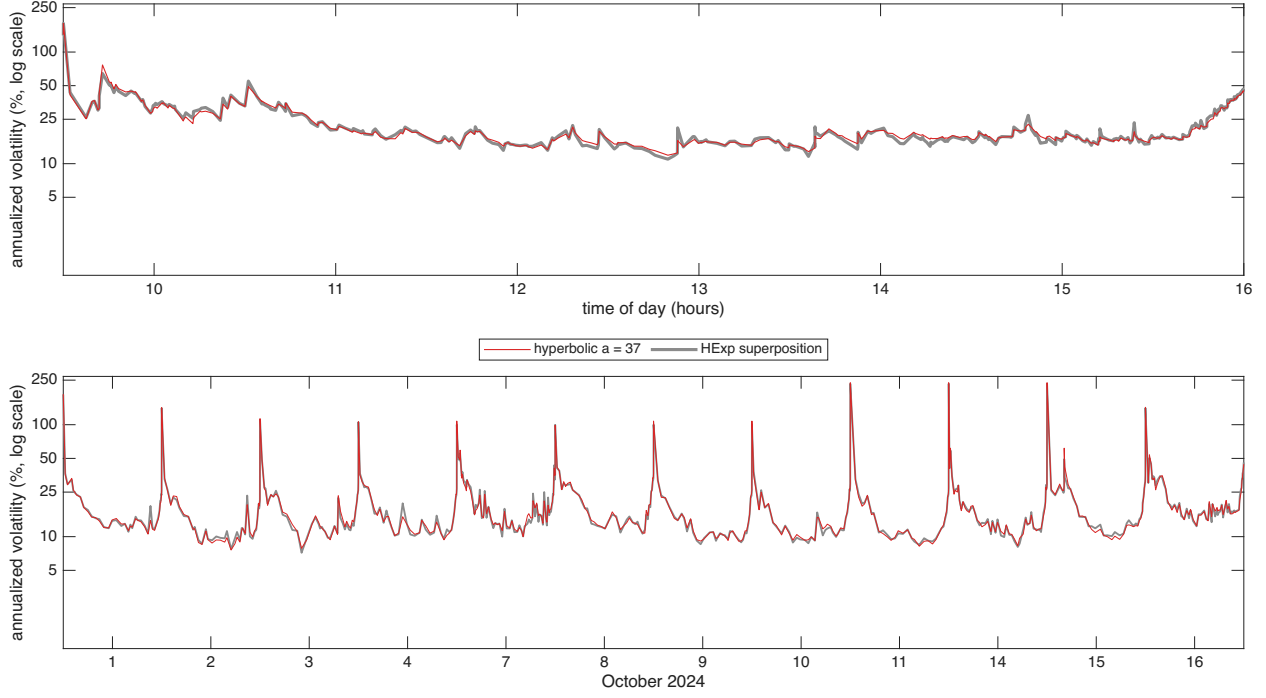
Figure 6: Hyperbolic against superposition weights for WING over 12 trading days in Oct 2024, the diurnally adjusted \hat{\sigma}(u)100\sqrt{252} at s = 1 second from the Huber filter, shown as annualized vol in % on a log10 scale. The only difference between the 2 paths is the weight function: the hyperbolic weights with a = 37 in red, drawn on top, and the HExp superposition in grey, 4 exponential components with half lives of 10, 100, 1000, 10000 seconds. Hyperparameters minimize the QLIKE objective. Top: 16 October 2024, bottom: 12 days.
