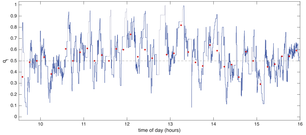
Figure 8: The directional conditional probability for WING, 16 October 2024. The filtered conditional probability q_t that an outlier lies above the robust Huber band, under exponential weights decaying in clock time with half life of 90 seconds; where fewer than two outliers remain in the weights it is drawn in grey. The dashed line marks 0.5. The red points are the empirical conditional probability using the 600 second bins of the previous figure.
