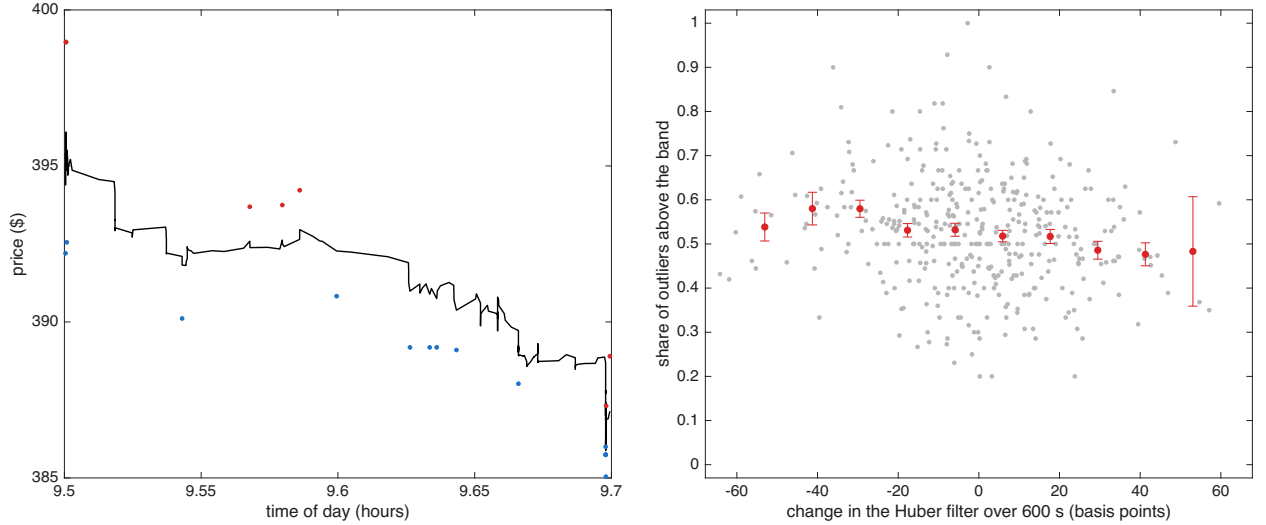
Figure 7: Outliers & robust price for WING on 16 October 2024. Left: the 12 minutes with the largest move in the Huber filter that day; outliers above Y_t - \theta_t > \delta_{t-1} in red, outliers below Y_t - \theta_t < -\delta_{t-1} in blue, Huber filter in black. Right: over the 12 trading days, the 600 second empirical conditional probability that outliers are above (rather than below) the Huber band against the 600 second change in the Huber filter in basis points: light points are single bins, the line & bars are means & s.e.
