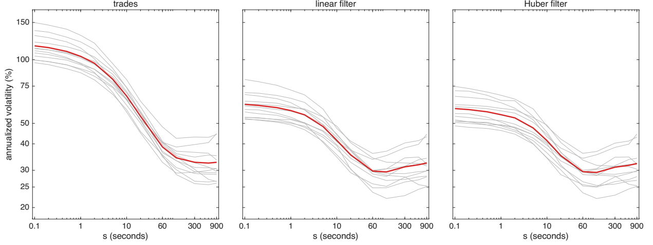
Figure 4: Volatility signature curves for WING over the 12 trading days in Oct 2024. The annualized vol \hat{\sigma}100\sqrt{252} from the returns \hat{X}_t - \hat{X}_{t,s} of Table 2, against the lag s in seconds, both axes on log scales, for: raw trades, linear filter & Huber filter. Grey lines are the individual trading days & the red line is the square root of the 12 day average of their squares. The linear & Huber returns carry the finite-sample correction c_{t,s} of the paper; the raw trades are unaffected by it.
