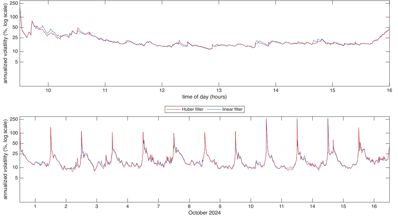
Figure 5: Filtered spot volatility for WING over 12 trading days in Oct 2024, the diurnally adjusted estimator \hat{\sigma}(u)100\sqrt{252} at s = 1 second with hyperbolic weights, Mandelbrot parameter a = 37 , with the input prices computed using the Huber & linear filters, shown as annualized volatility in percent on a log10 scale. Top: 16 October 2024, bottom: 12 days.
